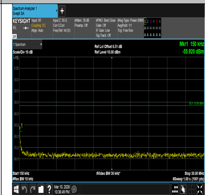
Band4-1.4MHz-QPSK-19957-6RB#0-0.15~30-PASS
