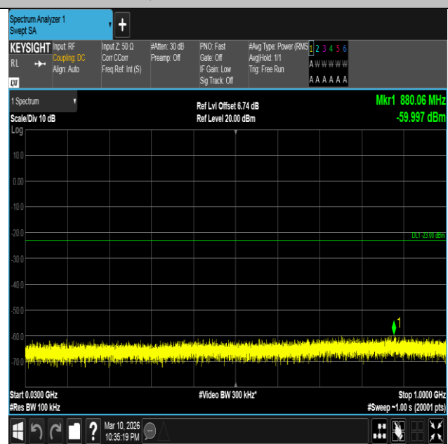
Band4-1.4MHz-QPSK-19957-1RB#5-30~1000-PASS
