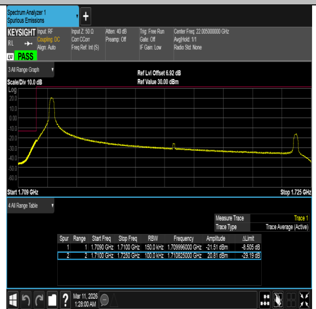
Band4-15MHz-16QAM-20025-1RB#0-PASS
