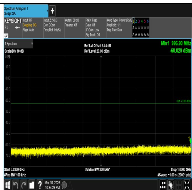
Band4-1.4MHz-16QAM-19957-1RB#0-30~1000-PASS
