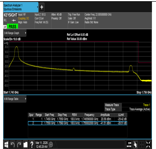
Band4-10MHz-16QAM-20350-1RB#0-PASS
