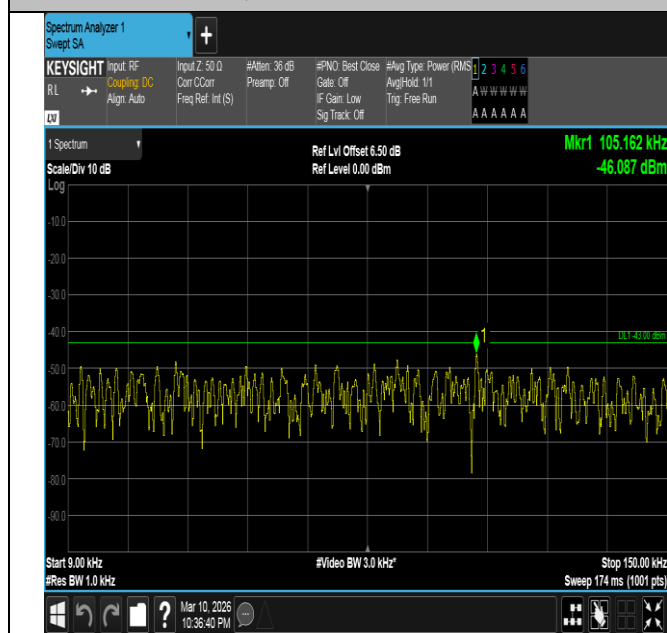
Band4-1.4MHz-QPSK-19957-6RB#0-0.009~0.15-PASS
