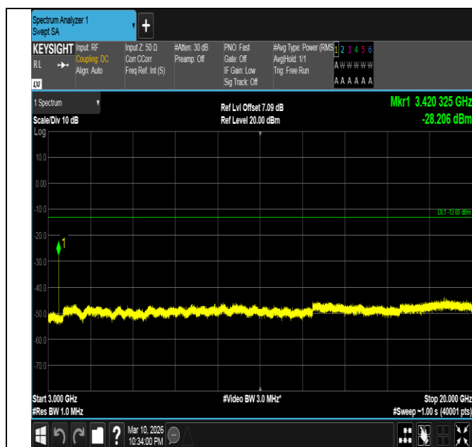
Band4-1.4MHz-QPSK-19957-1RB#0-3000~20000-PASS
