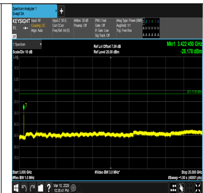
Band4-1.4MHz-QPSK-19957-1RB#5-3000~20000-PASS
