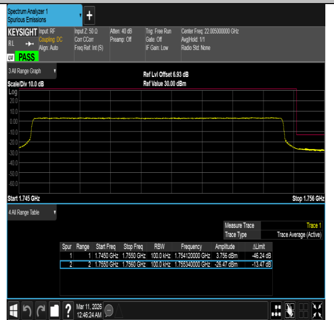
Band4-10MHz-16QAM-20350-50RB#0-PASS
