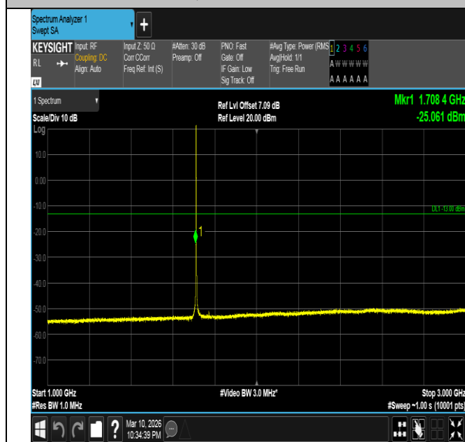
Band4-1.4MHz-16QAM-19957-1RB#0-1000~3000-PASS
