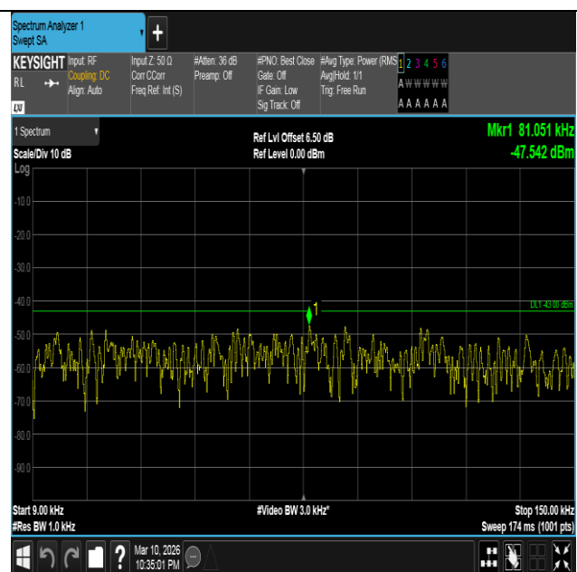
Band4-1.4MHz-QPSK-19957-1RB#5-0.009~0.15-PASS
