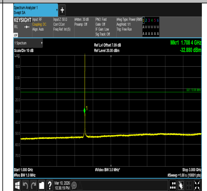
Band4-1.4MHz-16QAM-19957-1RB#5-1000~3000-PASS
