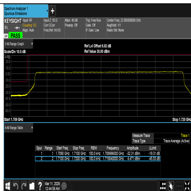
Band4-10MHz-16QAM-20000-50RB#0-PASS
