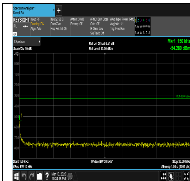
Band4-1.4MHz-16QAM-19957-1RB#0-0.15~30-PASS
