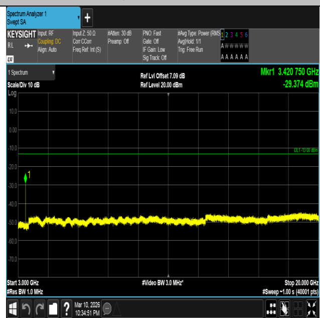
Band4-1.4MHz-16QAM-19957-1RB#0-3000~20000-PASS
