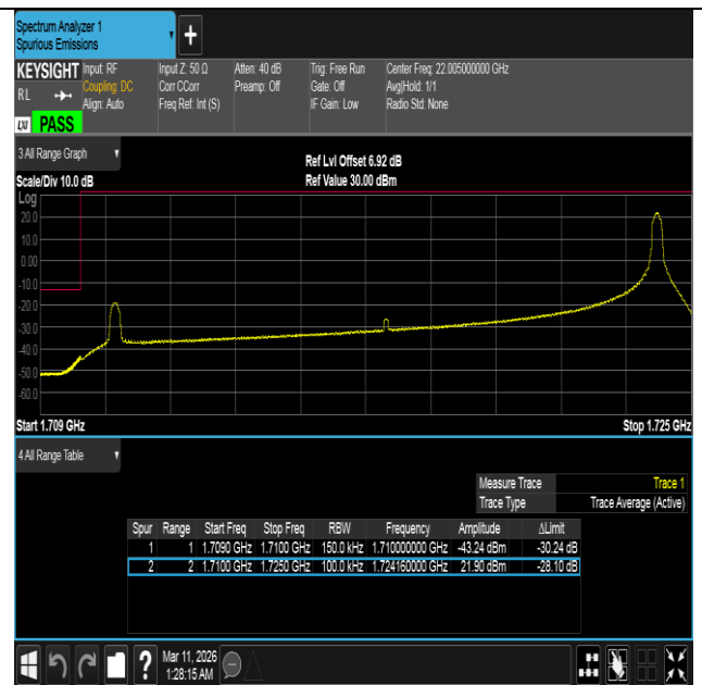
Band4-15MHz-QPSK-20025-1RB#74-PASS
