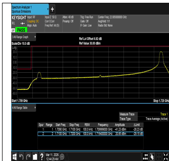
Band4-10MHz-16QAM-20000-1RB#49-PASS
