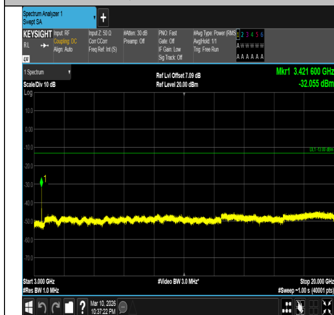
Band4-1.4MHz-QPSK-19957-6RB#0-3000~20000-PASS
