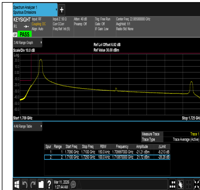
Band4-15MHz-QPSK-20025-1RB#0-PASS
