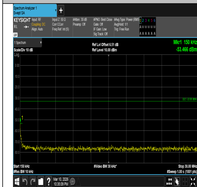
Band4-1.4MHz-QPSK-19957-1RB#5-0.15~30-PASS
