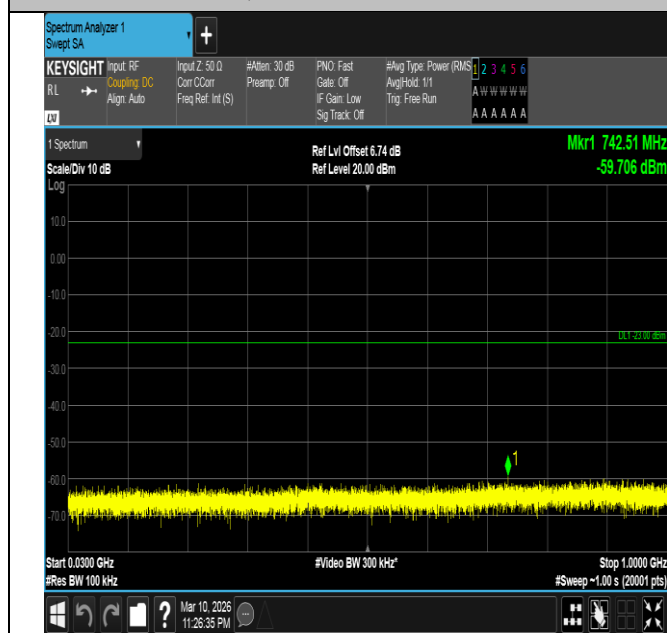
Band4-3MHz-16QAM-20175-1RB#14-30~1000-PASS
