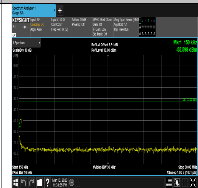
Band4-3MHz-16QAM-20385-1RB#14-0.15~30-PASS
