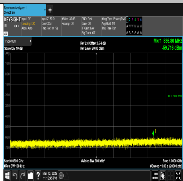
Band4-3MHz-16QAM-19965-1RB#0-30~1000-PASS
