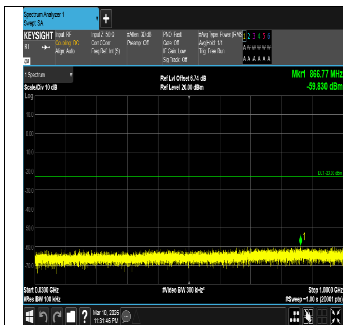
Band4-3MHz-16QAM-20385-1RB#14-30~1000-PASS
