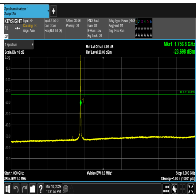
Band4-3MHz-16QAM-20385-1RB#14-1000~3000-PASS
