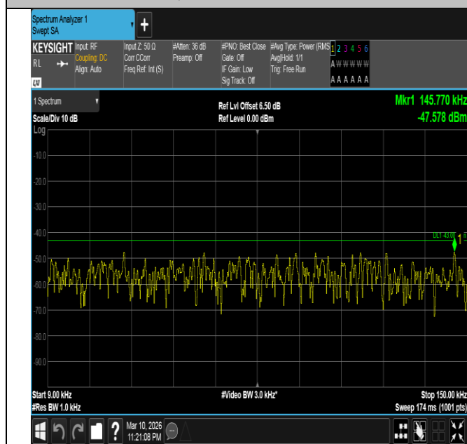
Band4-3MHz-16QAM-19965-1RB#14-0.009~0.15-PASS
