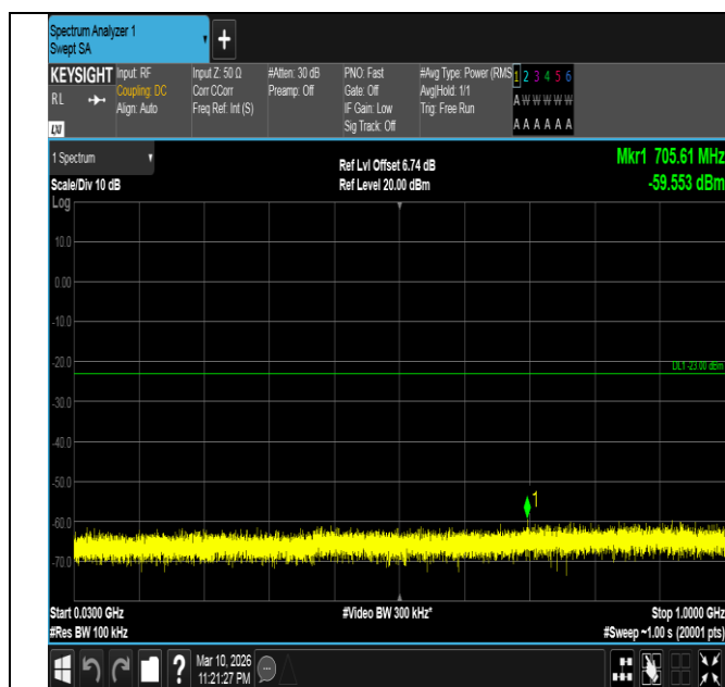
Band4-3MHz-16QAM-19965-1RB#14-30~1000-PASS
