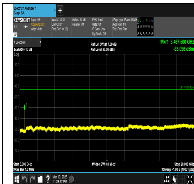
Band4-3MHz-16QAM-20175-1RB#14-3000~20000-PASS
