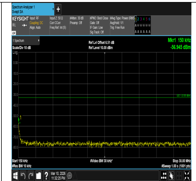
Band4-3MHz-QPSK-20385-15RB#0-0.15~30-PASS
