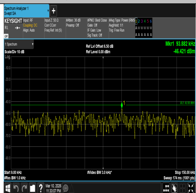
Band4-3MHz-16QAM-20385-15RB#0-0.009~0.15-PASS
