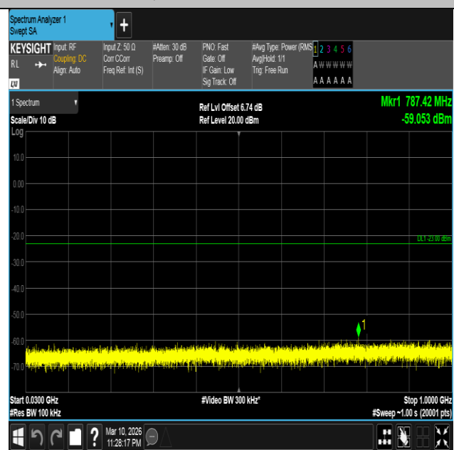
Band4-3MHz-16QAM-20175-15RB#0-30~1000-PASS
