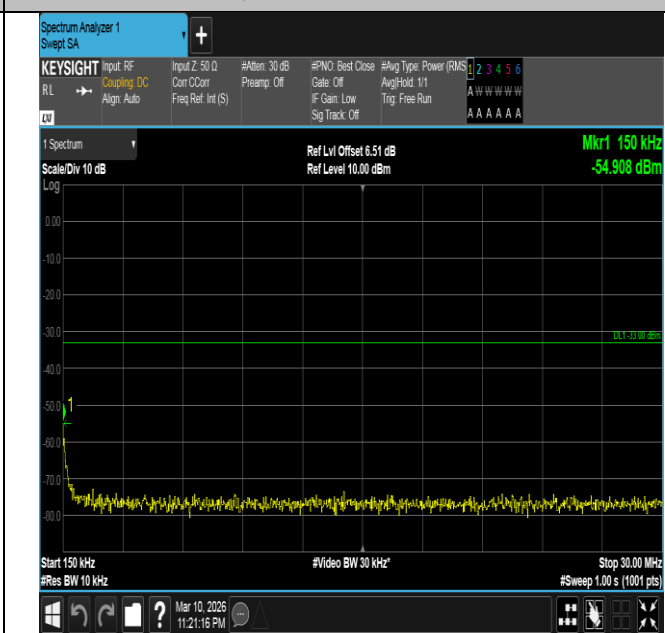
Band4-3MHz-16QAM-19965-1RB#14-0.15~30-PASS
