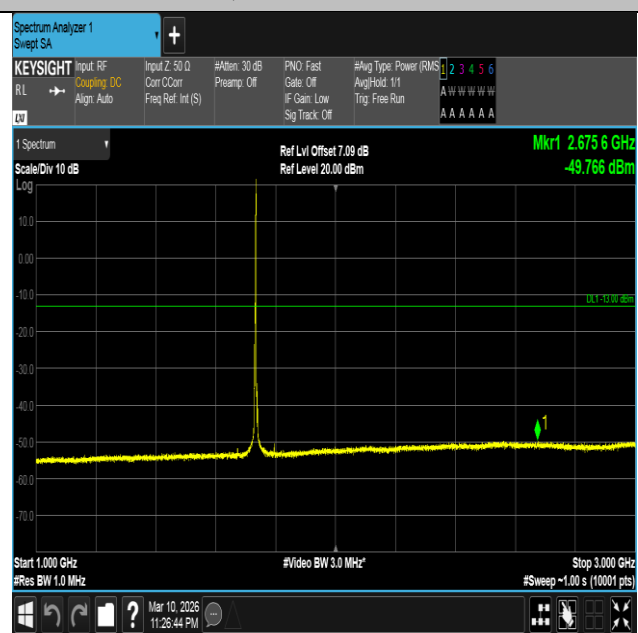
Band4-3MHz-16QAM-20175-1RB#14-1000~3000-PASS
