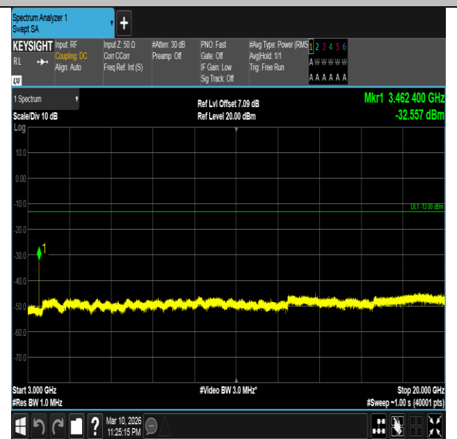
Band4-3MHz-16QAM-20175-1RB#0-3000~20000-PASS
