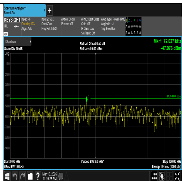
Band4-3MHz-16QAM-19965-1RB#0-0.009~0.15-PASS
