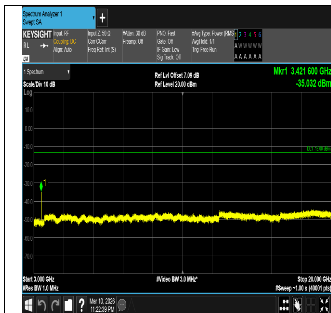
Band4-3MHz-QPSK-19965-15RB#0-3000~20000-PASS
