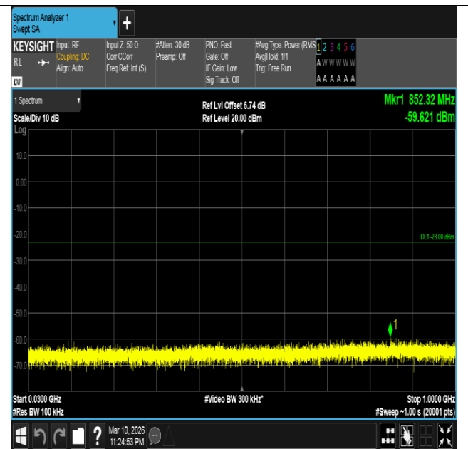
Band4-3MHz-16QAM-20175-1RB#0-30~1000-PASS
