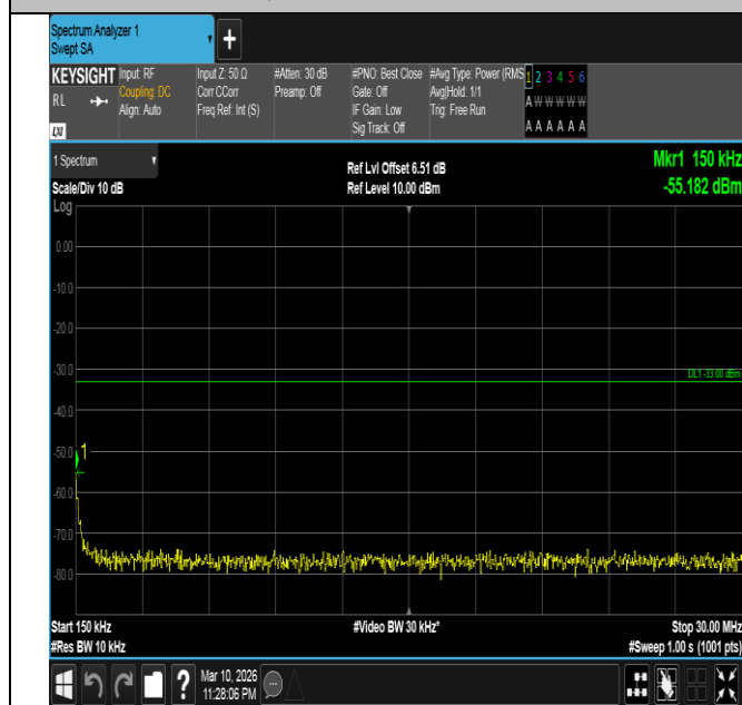
Band4-3MHz-16QAM-20175-15RB#0-0.15~30-PASS
