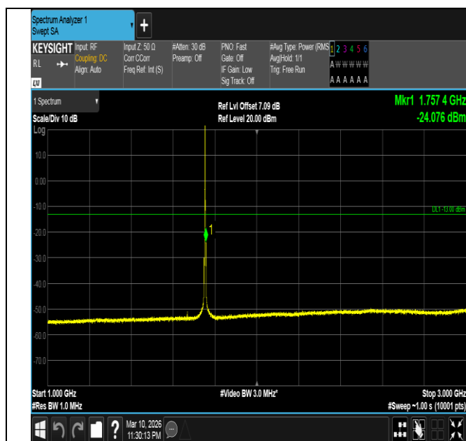
Band4-3MHz-16QAM-20385-1RB#0-1000~3000-PASS
