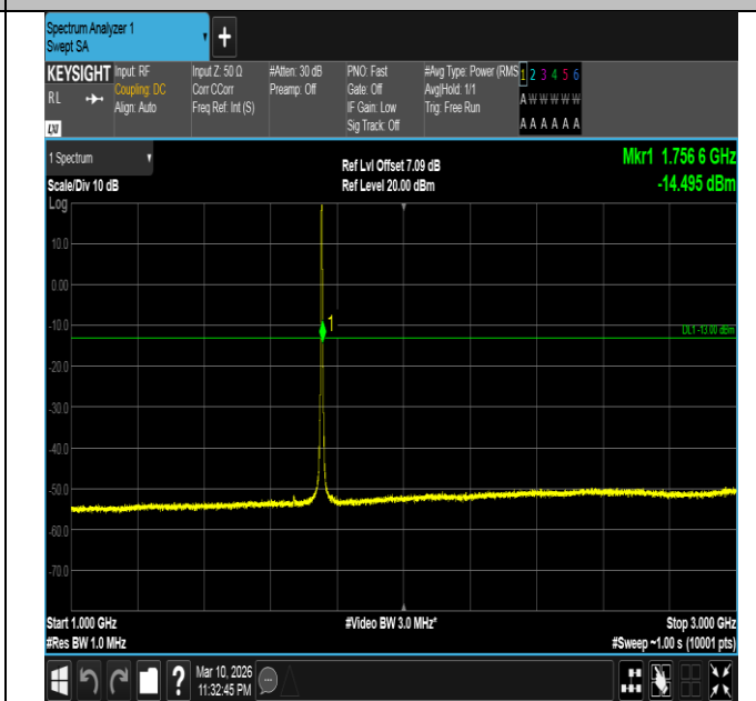
Band4-3MHz-QPSK-20385-15RB#0-1000~3000-PASS
