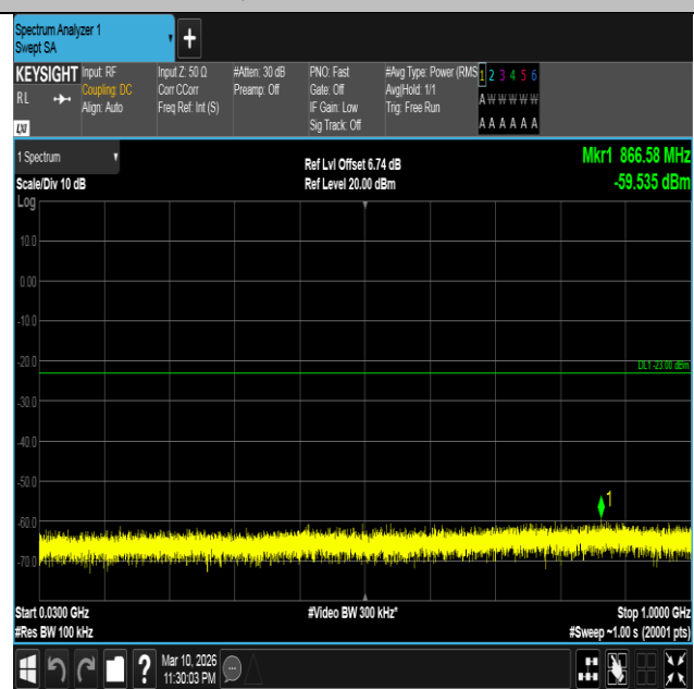
Band4-3MHz-16QAM-20385-1RB#0-30~1000-PASS
