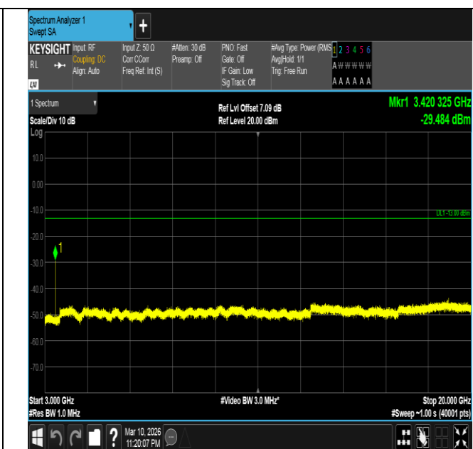
Band4-3MHz-16QAM-19965-1RB#0-3000~20000-PASS
