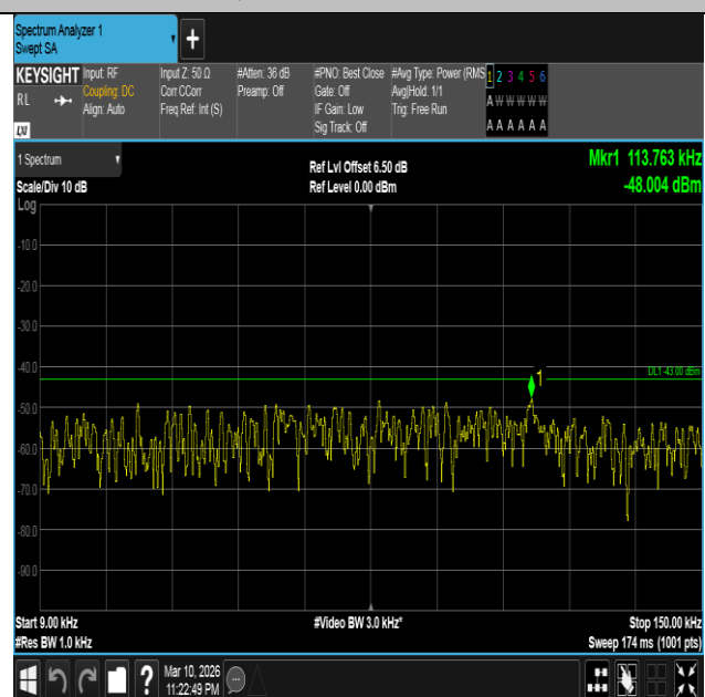
Band4-3MHz-16QAM-19965-15RB#0-0.009~0.15-PASS
