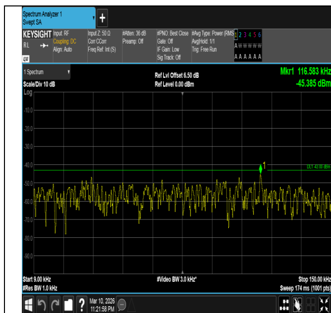
Band4-3MHz-QPSK-19965-15RB#0-0.009~0.15-PASS
