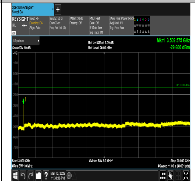
Band4-3MHz-QPSK-20385-1RB#14-3000~20000-PASS
