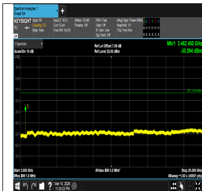
Band4-3MHz-QPSK-20175-1RB#0-3000~20000-PASS
