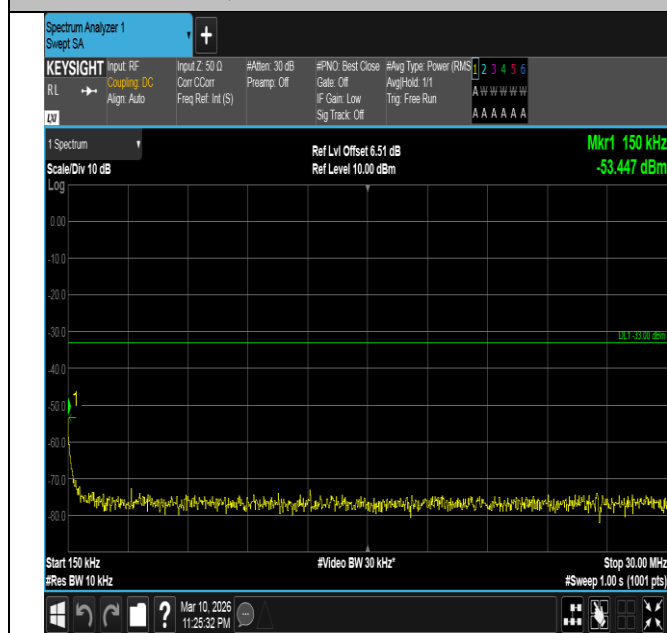
Band4-3MHz-QPSK-20175-1RB#14-0.15~30-PASS
