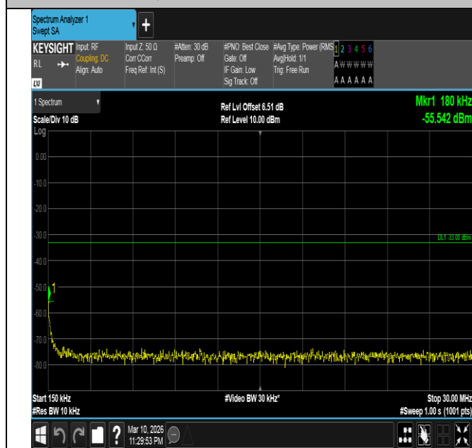
Band4-3MHz-16QAM-20385-1RB#0-0.15~30-PASS
