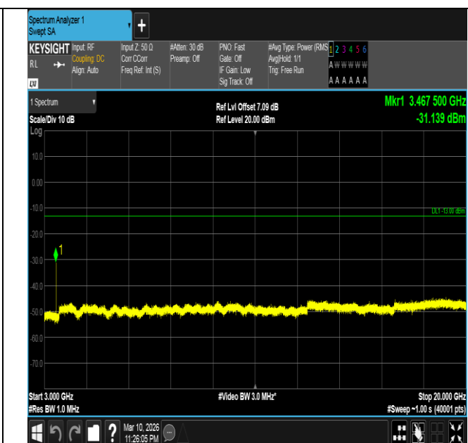
Band4-3MHz-QPSK-20175-1RB#14-3000~20000-PASS
