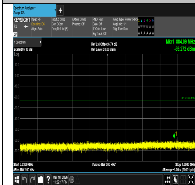
Band4-3MHz-QPSK-19965-15RB#0-30~1000-PASS
