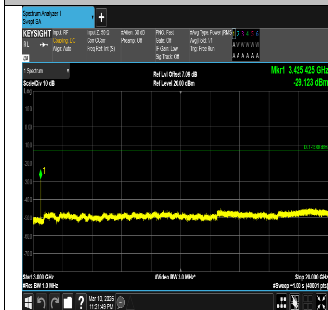
Band4-3MHz-16QAM-19965-1RB#14-3000~20000-PASS
