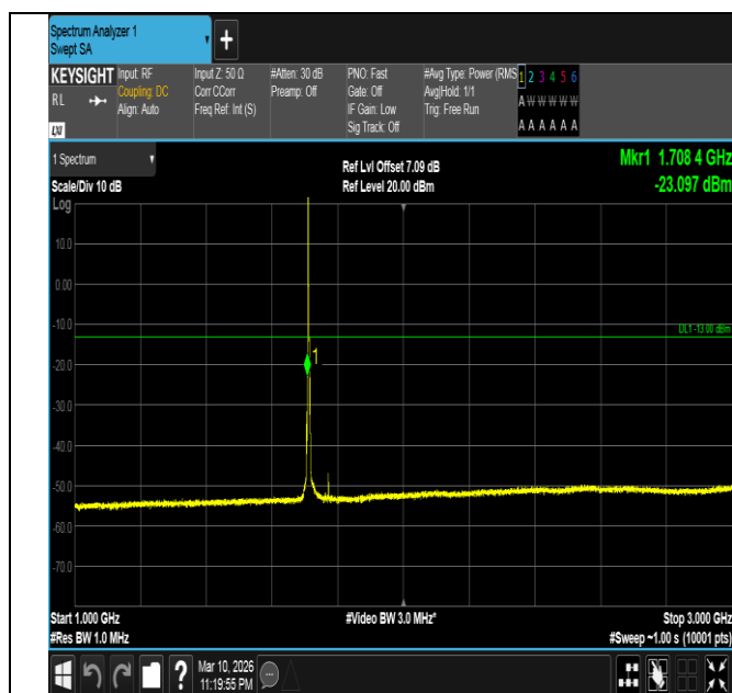
Band4-3MHz-16QAM-19965-1RB#0-1000~3000-PASS
