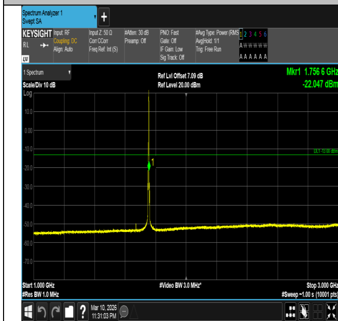
Band4-3MHz-QPSK-20385-1RB#14-1000~3000-PASS
