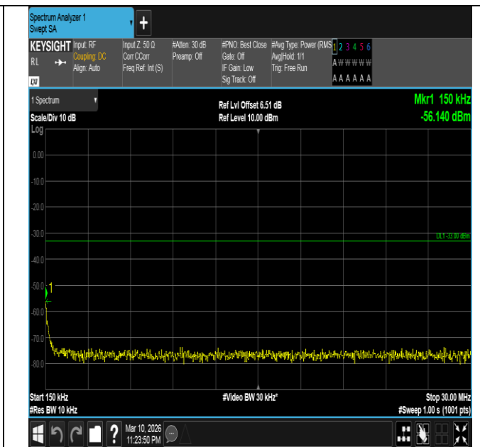
Band4-3MHz-QPSK-20175-1RB#0-0.15~30-PASS
