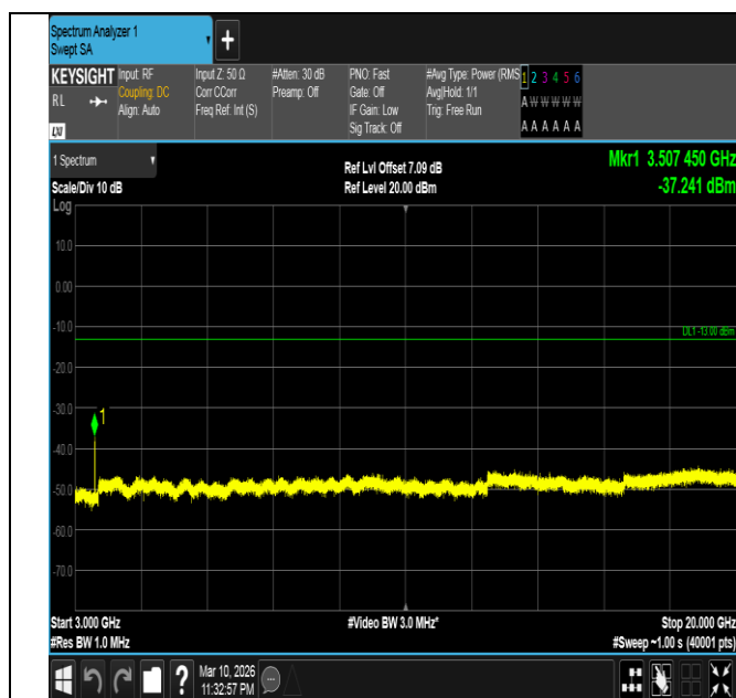
Band4-3MHz-QPSK-20385-15RB#0-3000~20000-PASS
