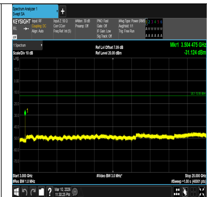
Band4-3MHz-16QAM-20385-1RB#0-3000~20000-PASS
