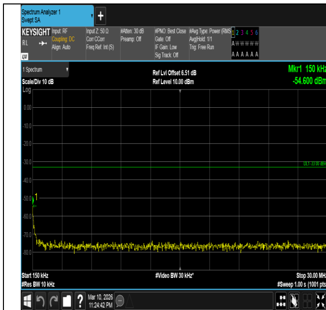
Band4-3MHz-16QAM-20175-1RB#0-0.15~30-PASS
