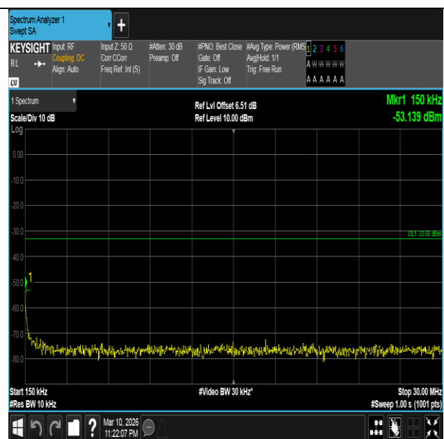
Band4-3MHz-QPSK-19965-15RB#0-0.15~30-PASS
