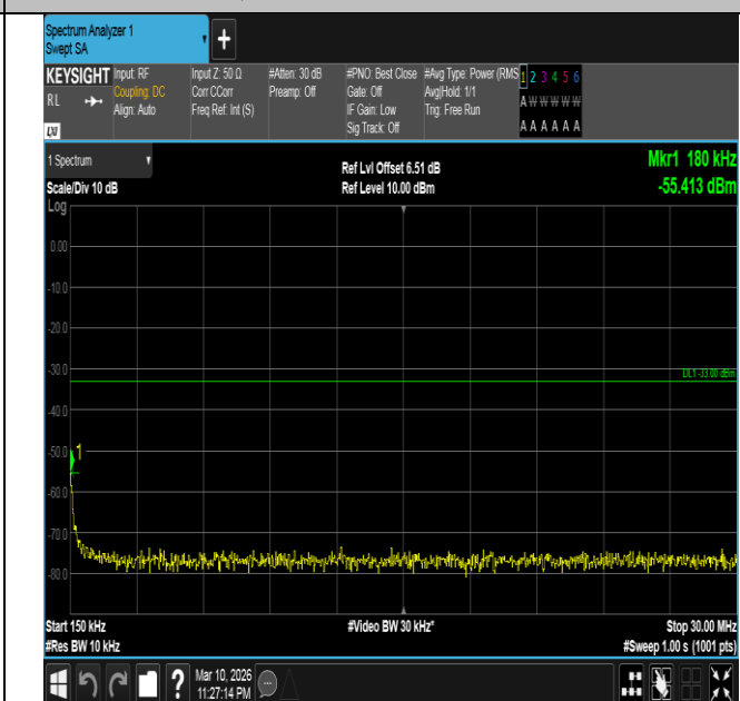
Band4-3MHz-QPSK-20175-15RB#0-0.15~30-PASS
