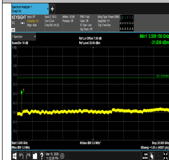
Band4-3MHz-16QAM-20385-1RB#14-3000~20000-PASS
