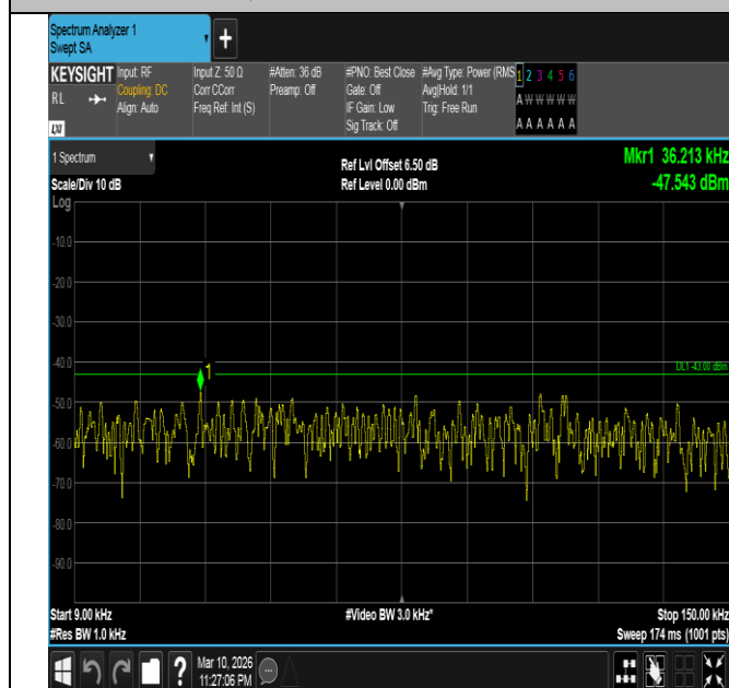
Band4-3MHz-QPSK-20175-15RB#0-0.009~0.15-PASS
