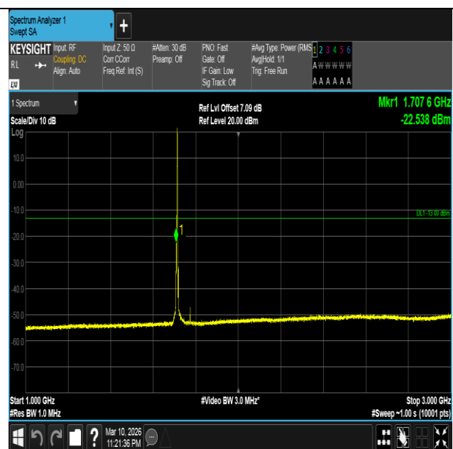
Band4-3MHz-16QAM-19965-1RB#14-1000~3000-PASS
