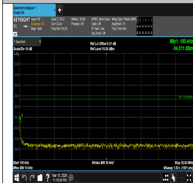
Band4-3MHz-16QAM-19965-1RB#0-0.15~30-PASS
