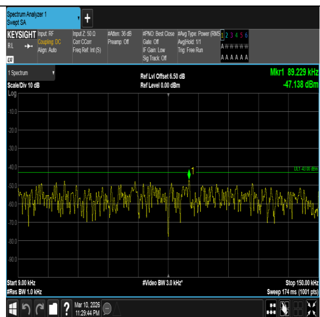
Band4-3MHz-16QAM-20385-1RB#0-0.009~0.15-PASS
