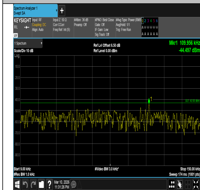
Band4-3MHz-16QAM-20385-1RB#14-0.009~0.15-PASS
