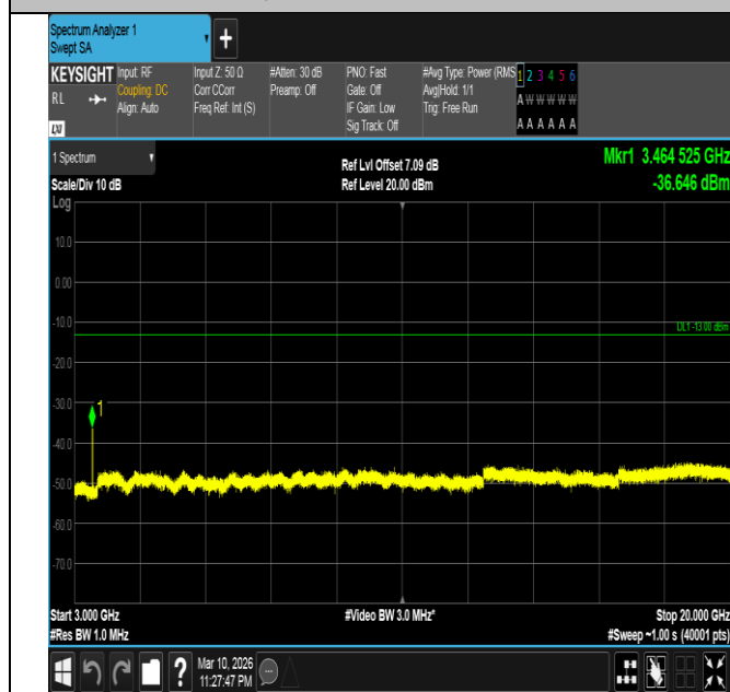
Band4-3MHz-QPSK-20175-15RB#0-3000~20000-PASS
