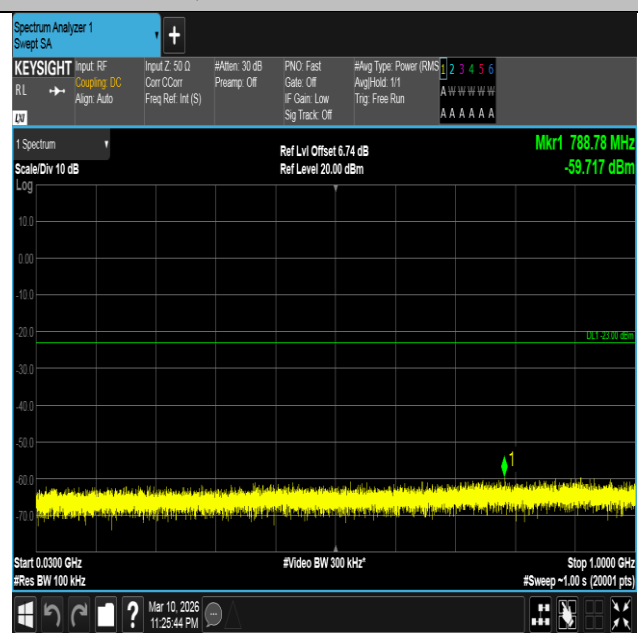
Band4-3MHz-QPSK-20175-1RB#14-30~1000-PASS
