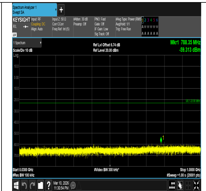
Band4-3MHz-QPSK-20385-1RB#14-30~1000-PASS
