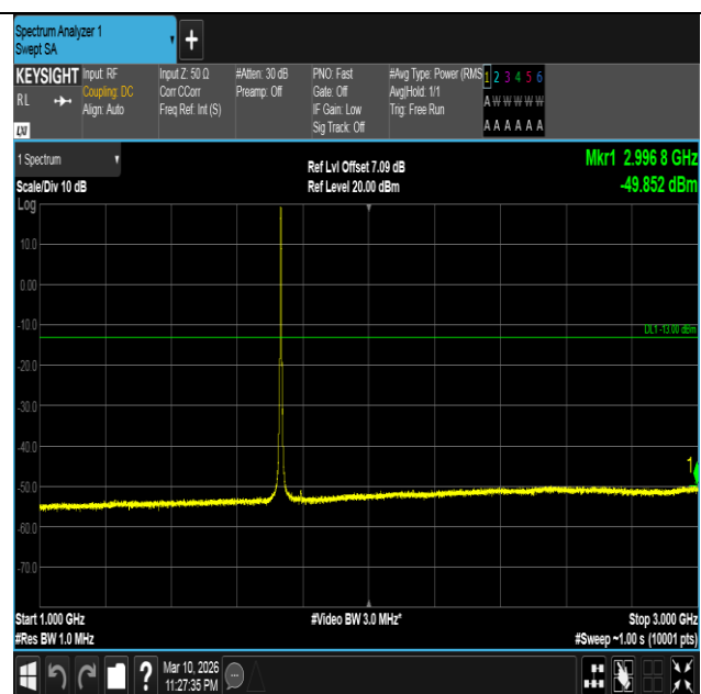
Band4-3MHz-QPSK-20175-15RB#0-1000~3000-PASS
