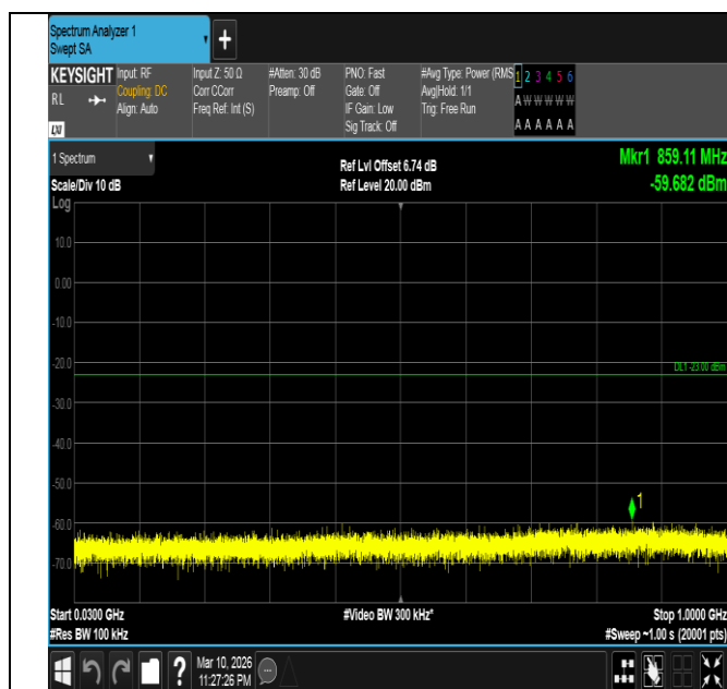
Band4-3MHz-QPSK-20175-15RB#0-30~1000-PASS
