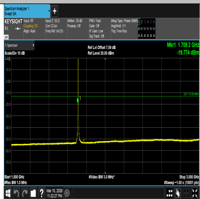
Band4-3MHz-QPSK-19965-15RB#0-1000~3000-PASS
