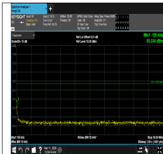
Band4-5MHz-16QAM-19975-1RB#0-0.15~30-PASS
