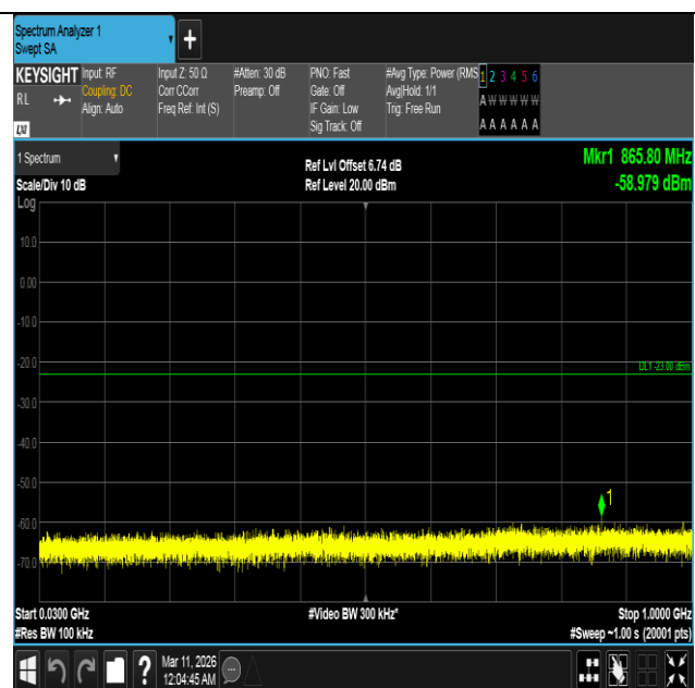
Band4-5MHz-16QAM-19975-1RB#0-30~1000-PASS
