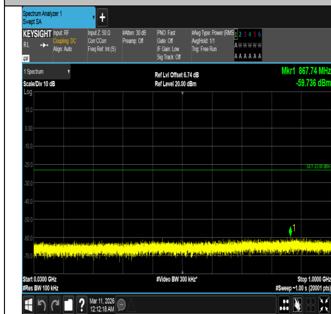
Band4-5MHz-QPSK-20175-25RB#0-30~1000-PASS
