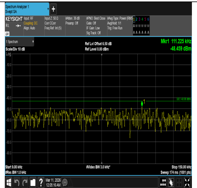
Band4-5MHz-QPSK-19975-1RB#24-0.009~0.15-PASS
