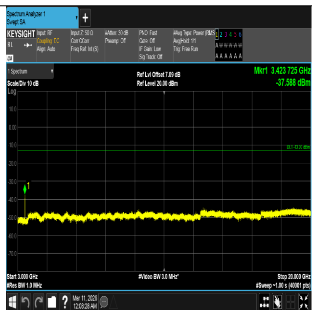
Band4-5MHz-16QAM-19975-25RB#0-3000~20000-PASS
