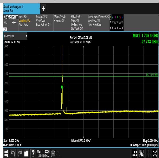
Band4-5MHz-QPSK-19975-1RB#0-1000~3000-PASS
