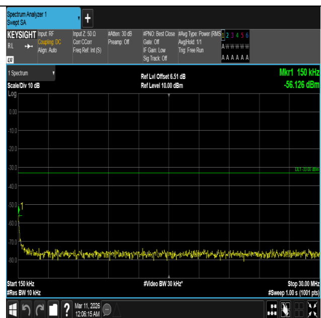
Band4-5MHz-16QAM-19975-1RB#24-0.15~30-PASS
