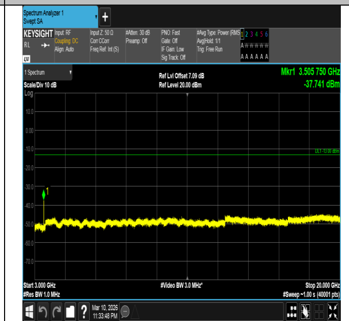
Band4-3MHz-16QAM-20385-15RB#0-3000~20000-PASS
