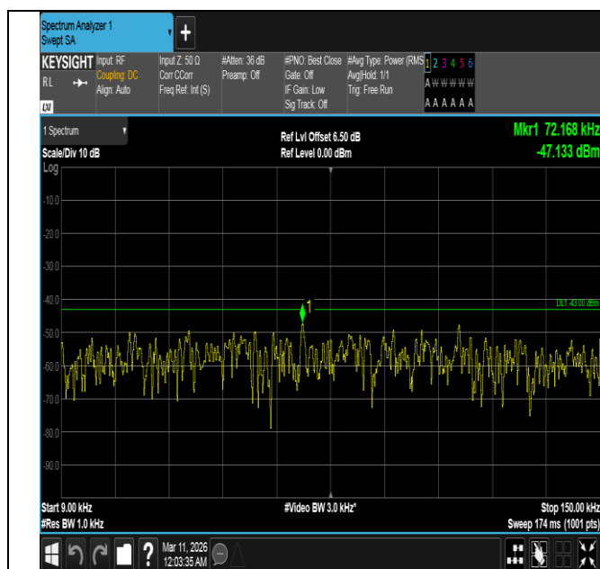
Band4-5MHz-QPSK-19975-1RB#0-0.009~0.15-PASS
