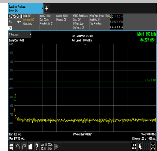
Band4-5MHz-16QAM-20175-1RB#24-0.15~30-PASS
