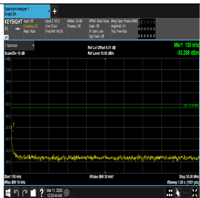
Band4-5MHz-QPSK-19975-1RB#0-0.15~30-PASS
