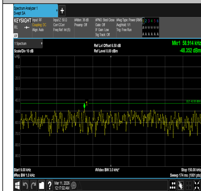
Band4-5MHz-QPSK-20375-25RB#0-0.009~0.15-PASS
