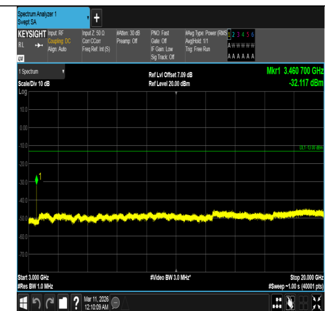
Band4-5MHz-16QAM-20175-1RB#0-3000~20000-PASS
