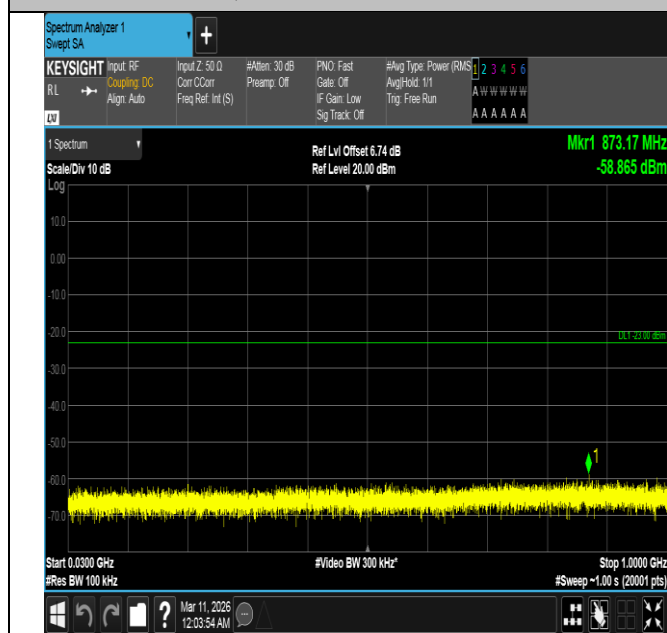
Band4-5MHz-QPSK-19975-1RB#0-30~1000-PASS
