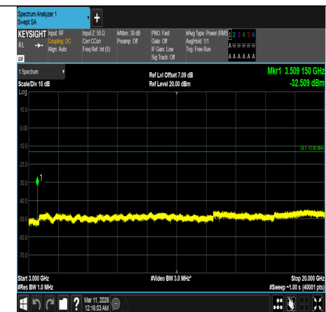
Band4-5MHz-QPSK-20375-1RB#24-3000~20000-PASS
