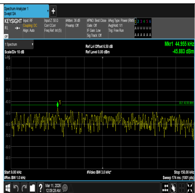
Band4-5MHz-16QAM-20175-1RB#0-0.009~0.15-PASS
