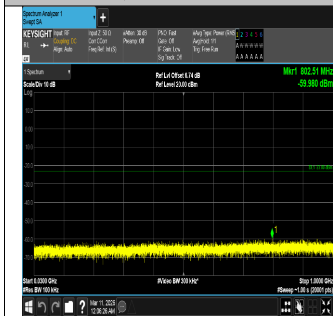
Band4-5MHz-16QAM-19975-1RB#24-30~1000-PASS
