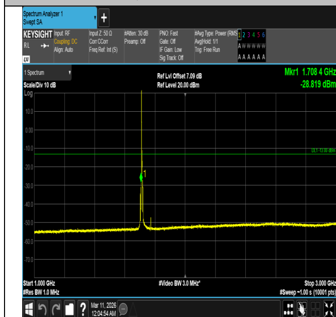
Band4-5MHz-16QAM-19975-1RB#0-1000~3000-PASS
