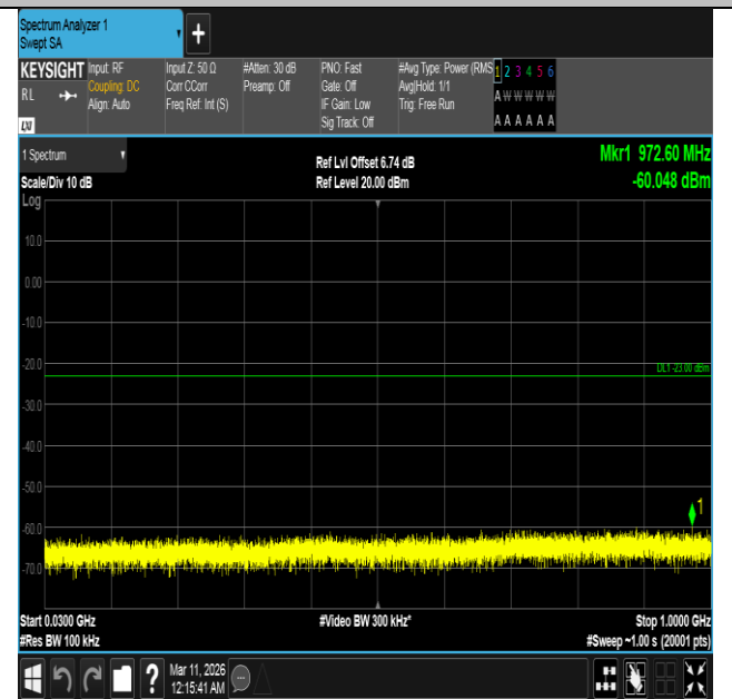
Band4-5MHz-QPSK-20375-1RB#24-30~1000-PASS
