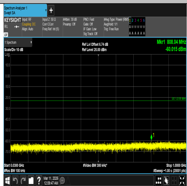
Band4-5MHz-16QAM-20175-1RB#0-30~1000-PASS
