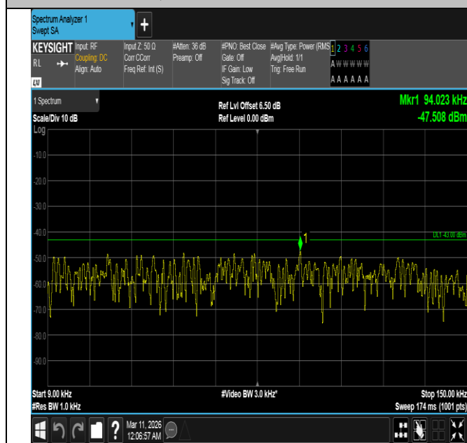
Band4-5MHz-QPSK-19975-25RB#0-0.009~0.15-PASS
