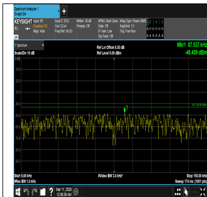
Band4-5MHz-16QAM-19975-1RB#24-0.009~0.15-PASS
