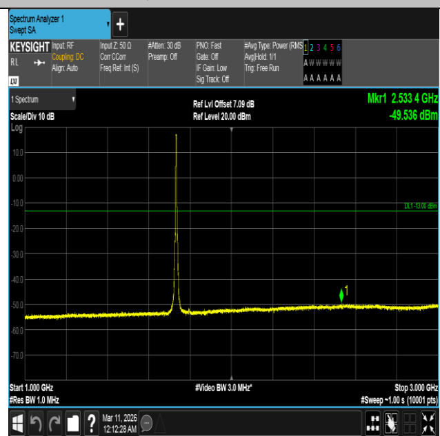
Band4-5MHz-QPSK-20175-25RB#0-1000~3000-PASS
