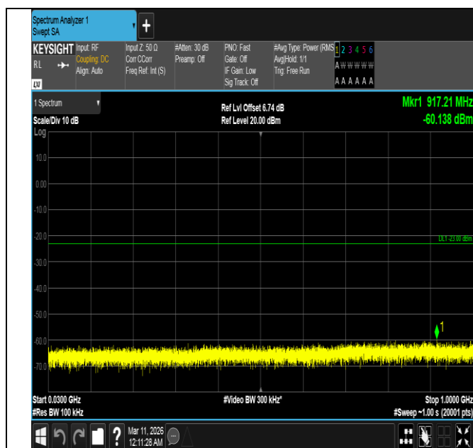
Band4-5MHz-16QAM-20175-1RB#24-30~1000-PASS
