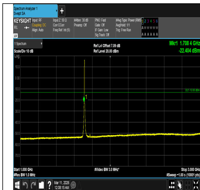
Band4-5MHz-16QAM-19975-25RB#0-1000~3000-PASS
