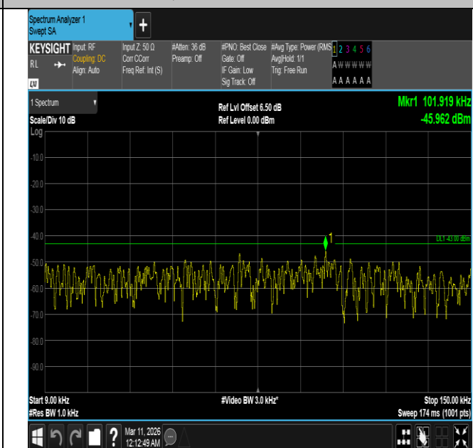
Band4-5MHz-16QAM-20175-25RB#0-0.009~0.15-PASS
