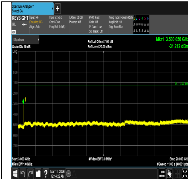
Band4-5MHz-QPSK-20375-1RB#0-3000~20000-PASS
