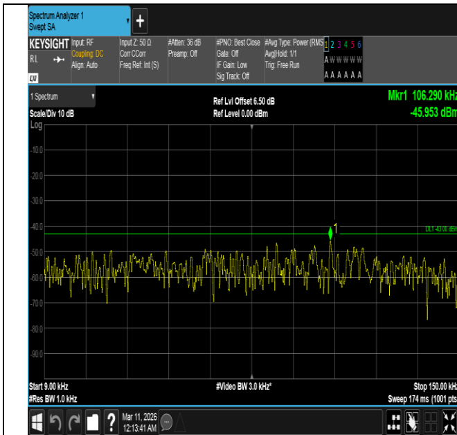
Band4-5MHz-QPSK-20375-1RB#0-0.009~0.15-PASS
