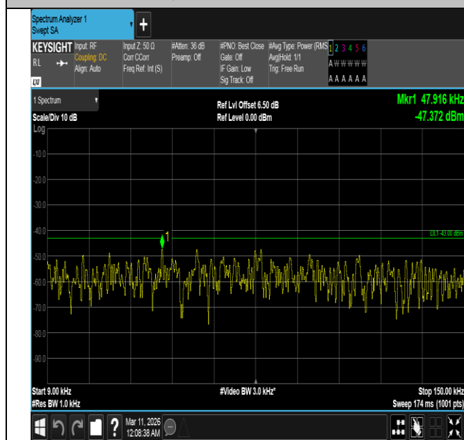
Band4-5MHz-QPSK-20175-1RB#0-0.009~0.15-PASS
