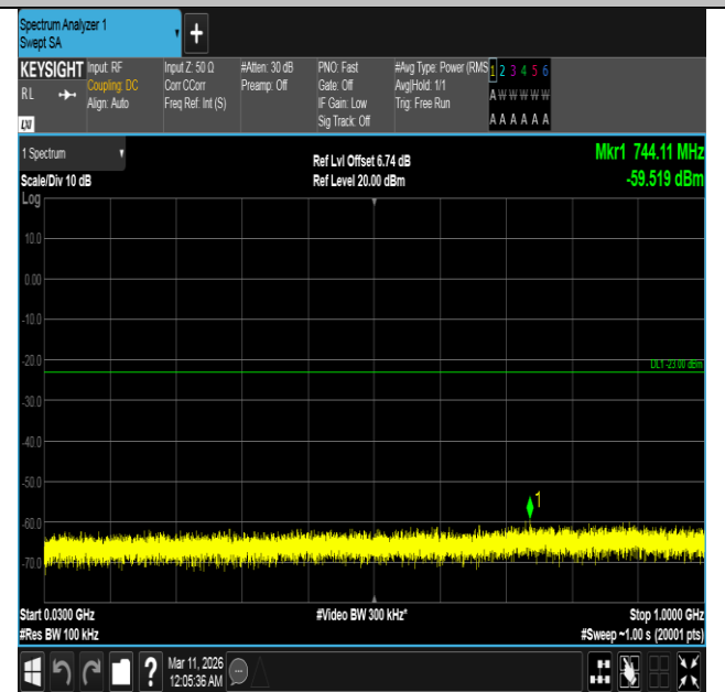
Band4-5MHz-QPSK-19975-1RB#24-30~1000-PASS
