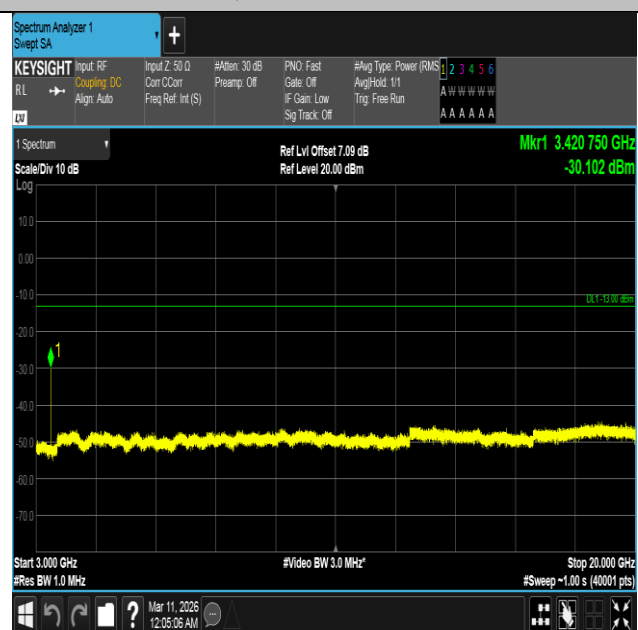
Band4-5MHz-16QAM-19975-1RB#0-3000~20000-PASS
