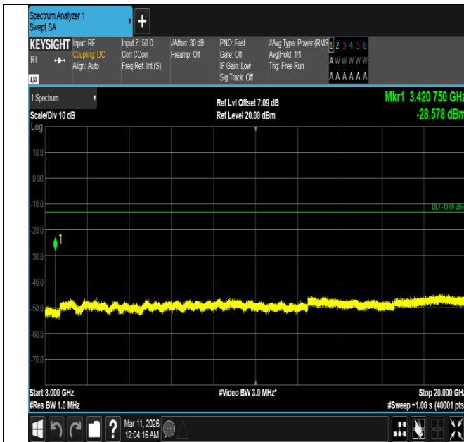
Band4-5MHz-QPSK-19975-1RB#0-3000~20000-PASS
