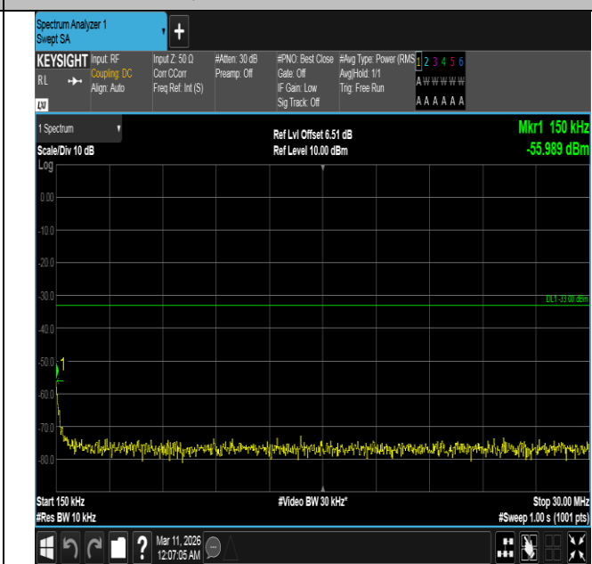
Band4-5MHz-QPSK-19975-25RB#0-0.15~30-PASS
