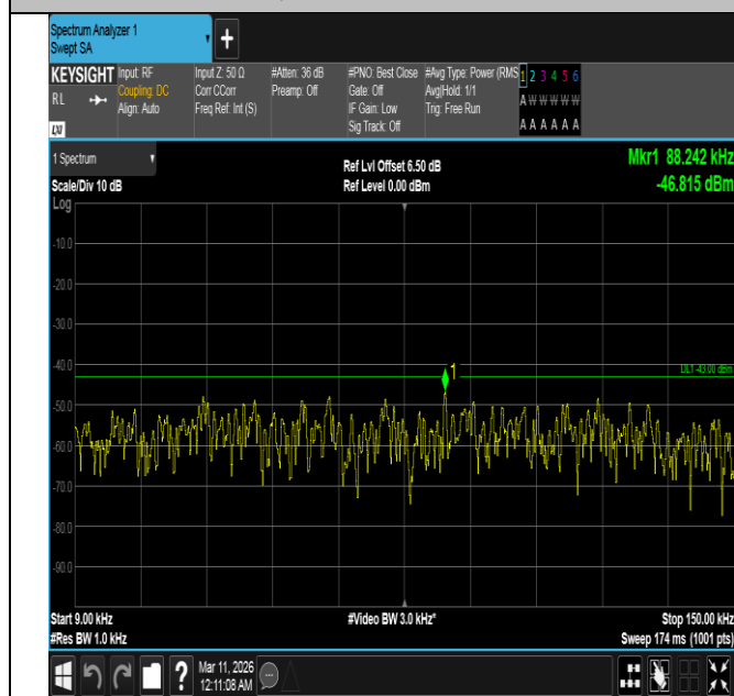
Band4-5MHz-16QAM-20175-1RB#24-0.009~0.15-PASS
