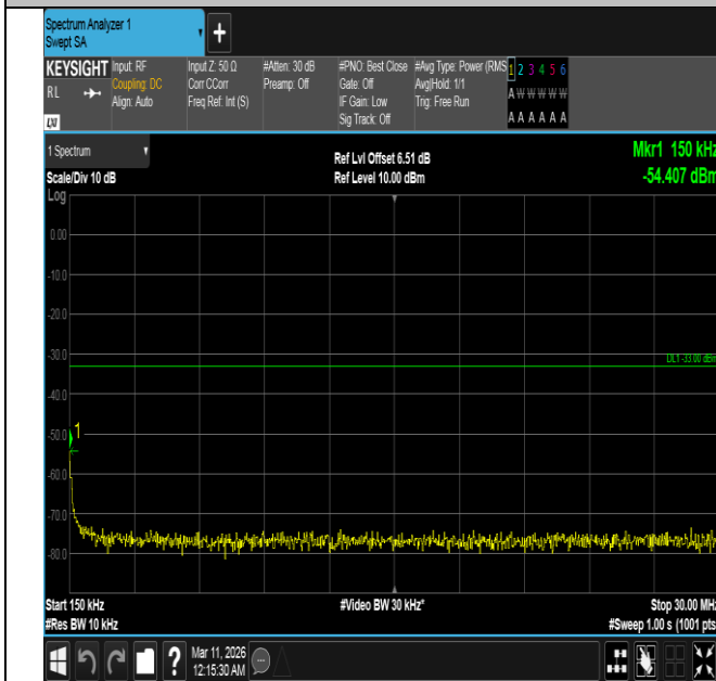
Band4-5MHz-QPSK-20375-1RB#24-0.15~30-PASS
