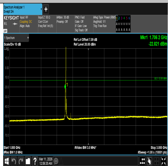
Band4-5MHz-16QAM-19975-1RB#24-1000~3000-PASS
