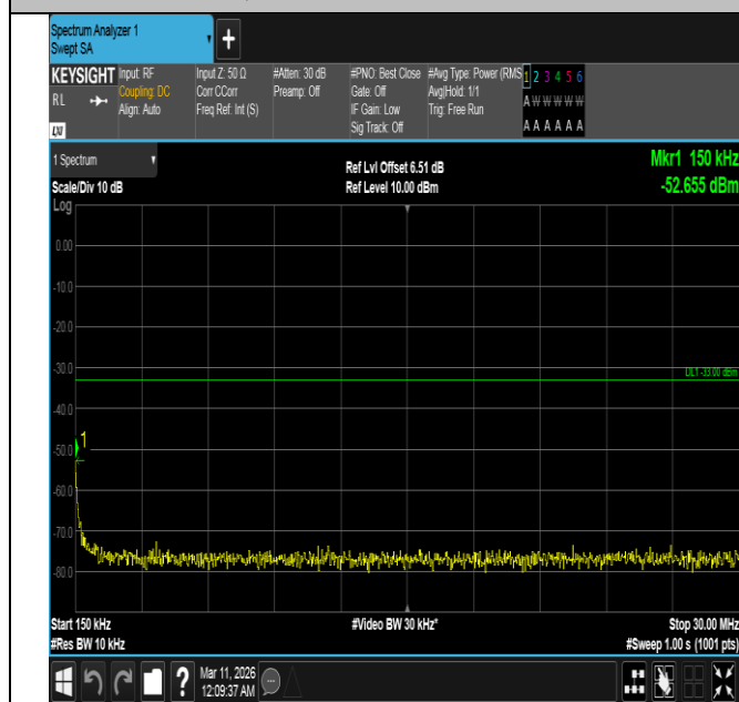
Band4-5MHz-16QAM-20175-1RB#0-0.15~30-PASS
