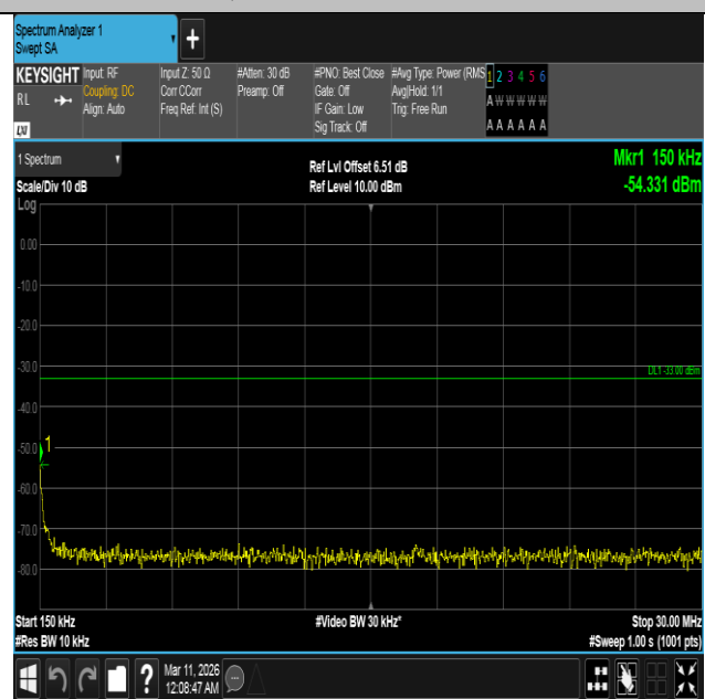
Band4-5MHz-QPSK-20175-1RB#0-0.15~30-PASS
