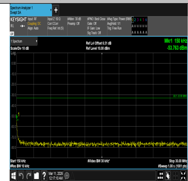
Band4-5MHz-QPSK-20375-25RB#0-0.15~30-PASS
