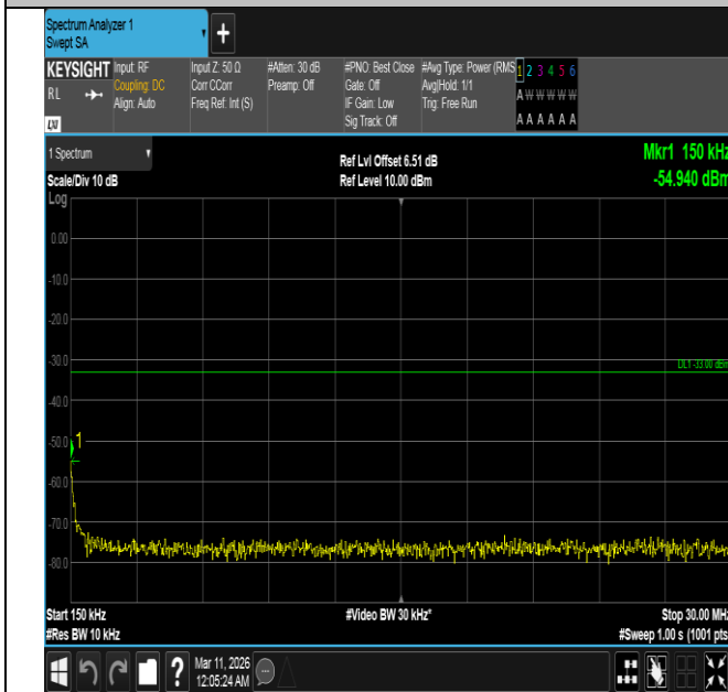
Band4-5MHz-QPSK-19975-1RB#24-0.15~30-PASS
