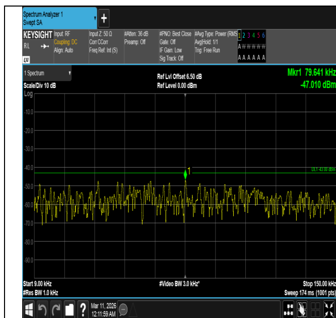
Band4-5MHz-QPSK-20175-25RB#0-0.009~0.15-PASS
