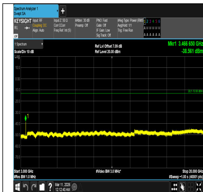
Band4-5MHz-QPSK-20175-25RB#0-3000~20000-PASS
