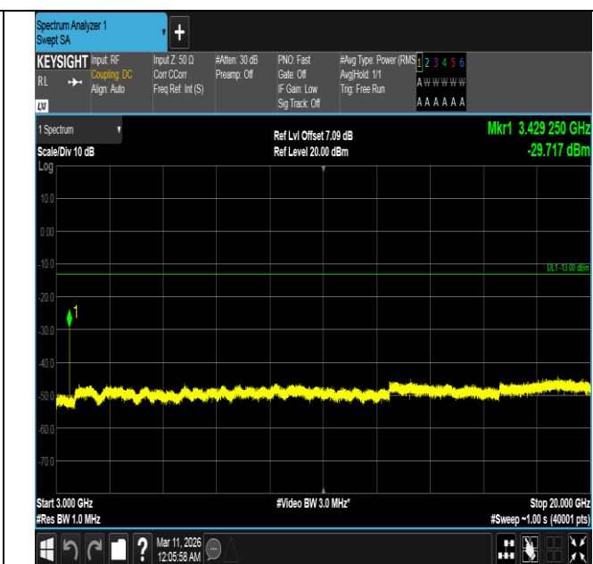
Band4-5MHz-QPSK-19975-1RB#24-3000~20000-PASS
