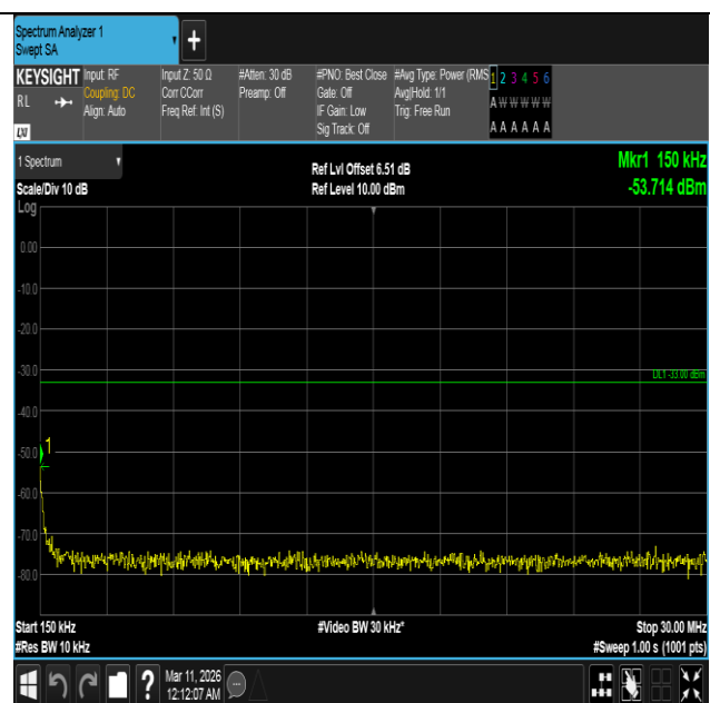
Band4-5MHz-QPSK-20175-25RB#0-0.15~30-PASS
