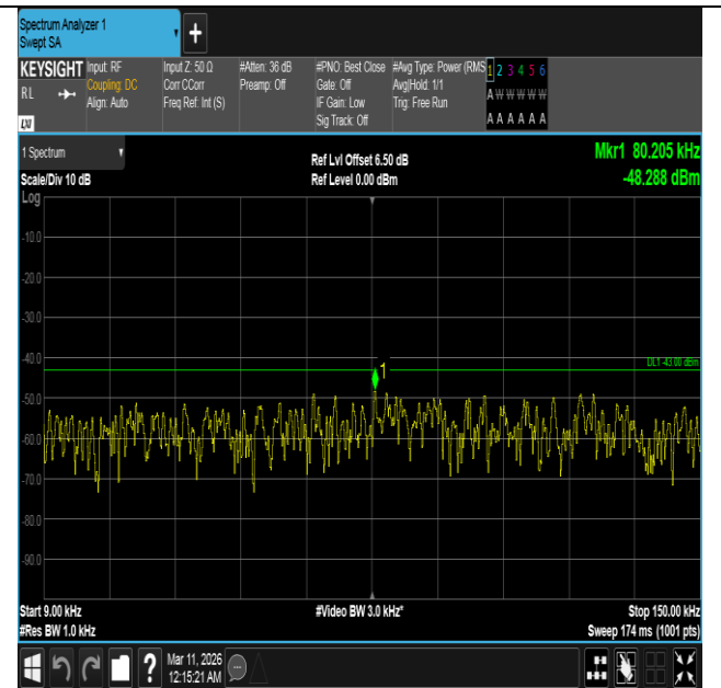
Band4-5MHz-QPSK-20375-1RB#24-0.009~0.15-PASS
