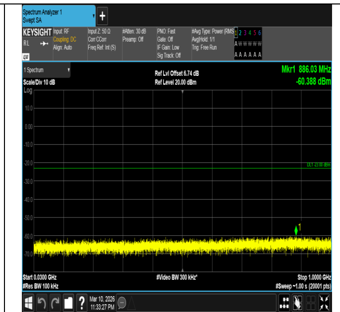
Band4-3MHz-16QAM-20385-15RB#0-30~1000-PASS
