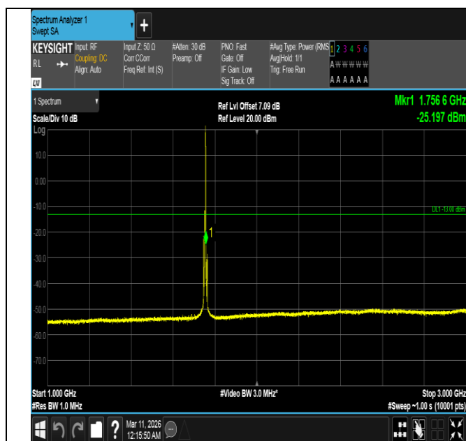
Band4-5MHz-QPSK-20375-1RB#24-1000~3000-PASS
