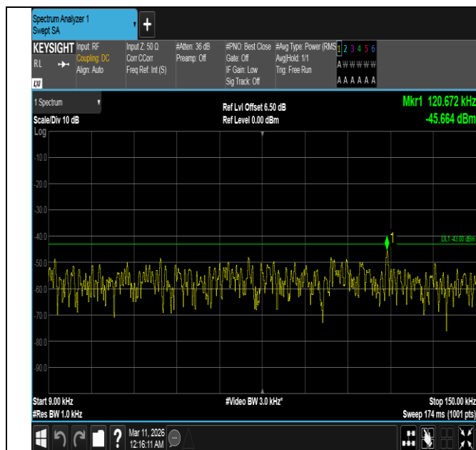
Band4-5MHz-16QAM-20375-1RB#24-0.009~0.15-PASS
