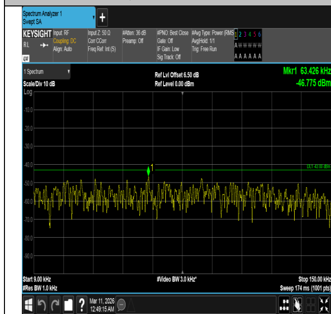
Band4-10MHz-16QAM-20000-1RB#49-0.009~0.15-PASS
