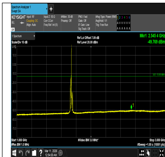
Band4-10MHz-QPSK-20175-1RB#49-1000~3000-PASS
