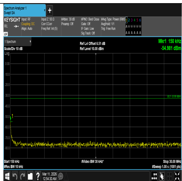
Band4-10MHz-16QAM-20175-1RB#49-0.15~30-PASS
