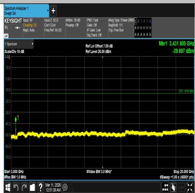
Band4-10MHz-16QAM-20000-50RB#0-3000~20000-PASS
