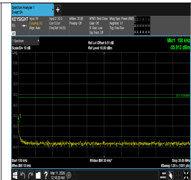
Band4-5MHz-16QAM-20375-1RB#24-0.15~30-PASS
