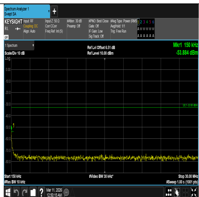
Band4-10MHz-QPSK-20000-50RB#0-0.15~30-PASS
