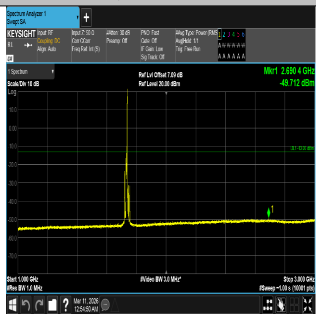
Band4-10MHz-16QAM-20175-1RB#49-1000~3000-PASS
