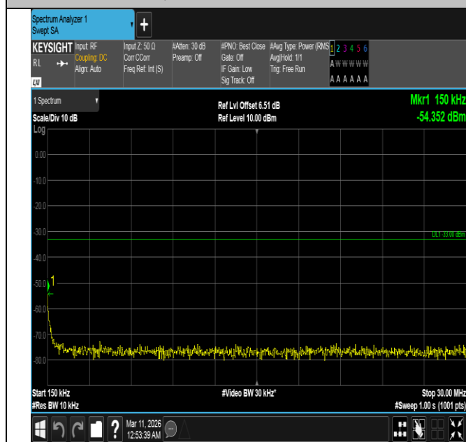
Band4-10MHz-QPSK-20175-1RB#49-0.15~30-PASS
