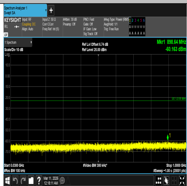
Band4-5MHz-16QAM-20375-25RB#0-30~1000-PASS
