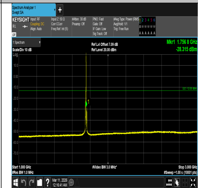
Band4-5MHz-16QAM-20375-1RB#24-1000~3000-PASS
