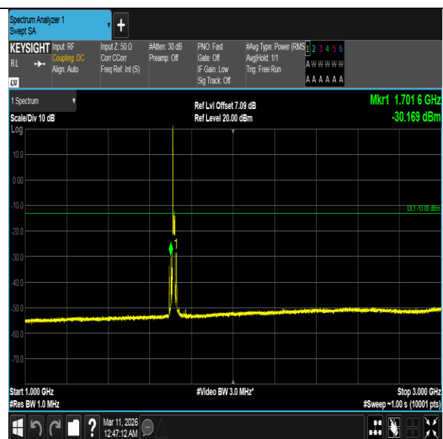
Band4-10MHz-QPSK-20000-1RB#0-1000~3000-PASS
