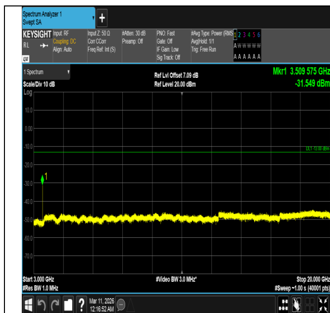
Band4-5MHz-16QAM-20375-1RB#24-3000~20000-PASS
