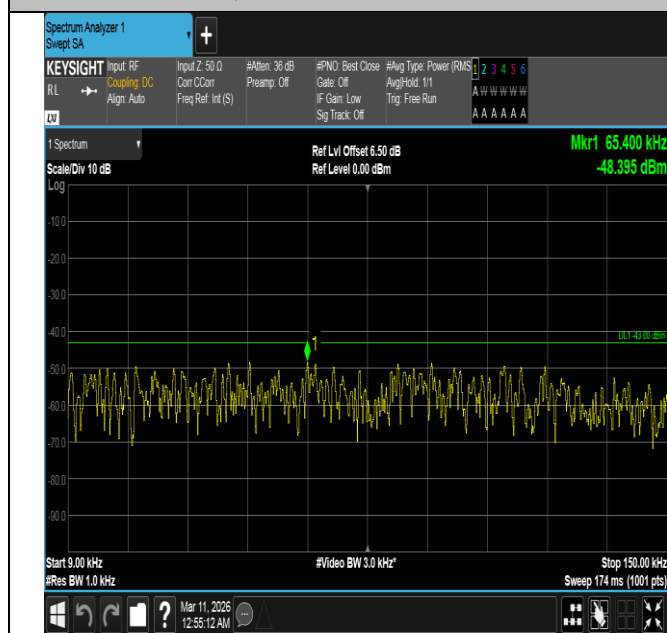
Band4-10MHz-QPSK-20175-50RB#0-0.009~0.15-PASS
