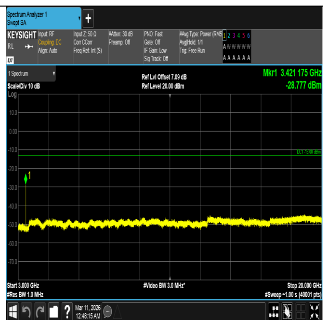
Band4-10MHz-16QAM-20000-1RB#0-3000~20000-PASS
