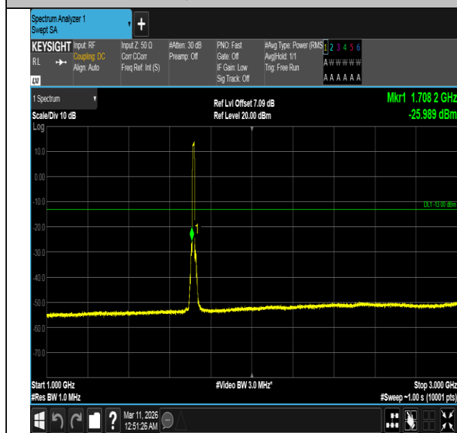
Band4-10MHz-16QAM-20000-50RB#0-1000~3000-PASS
