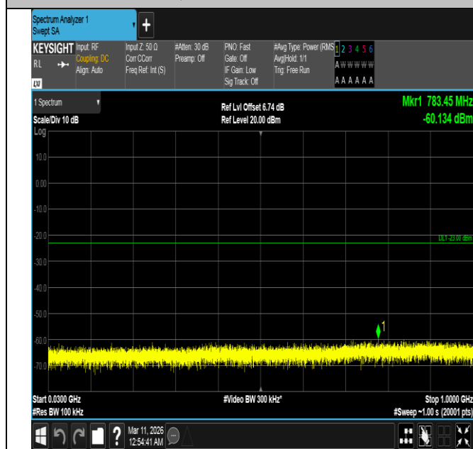
Band4-10MHz-16QAM-20175-1RB#49-30~1000-PASS
