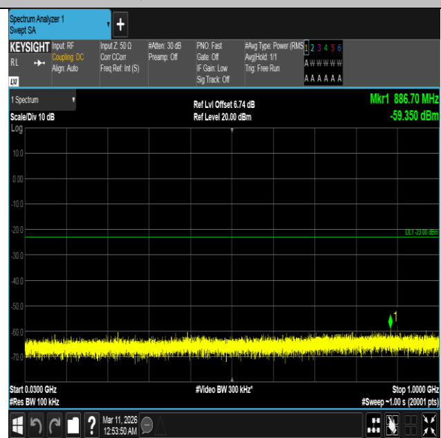
Band4-10MHz-QPSK-20175-1RB#49-30~1000-PASS
