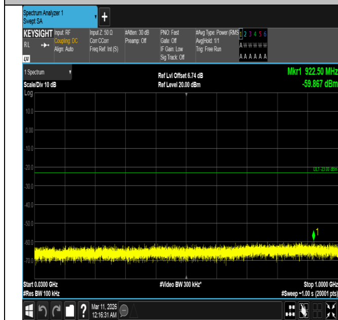
Band4-5MHz-16QAM-20375-1RB#24-30~1000-PASS
