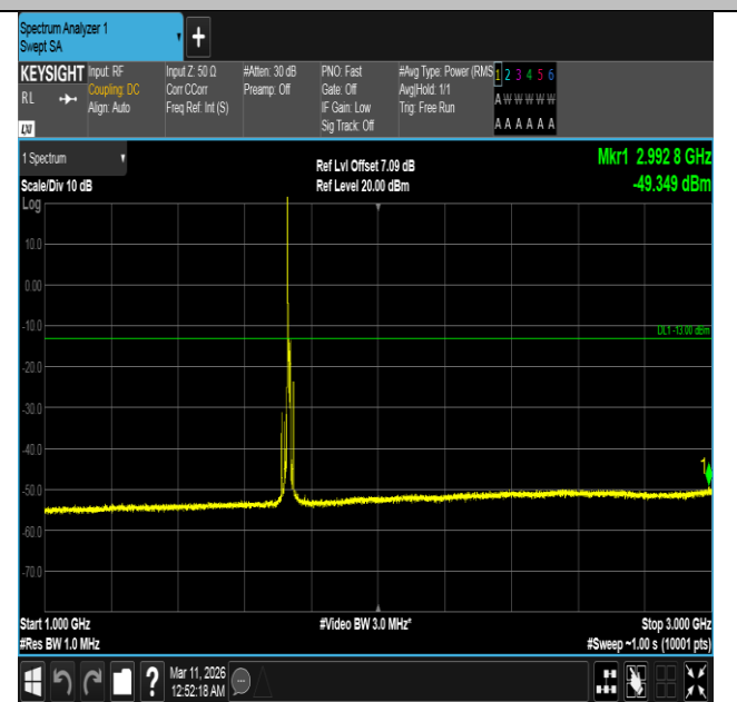
Band4-10MHz-QPSK-20175-1RB#0-1000~3000-PASS
