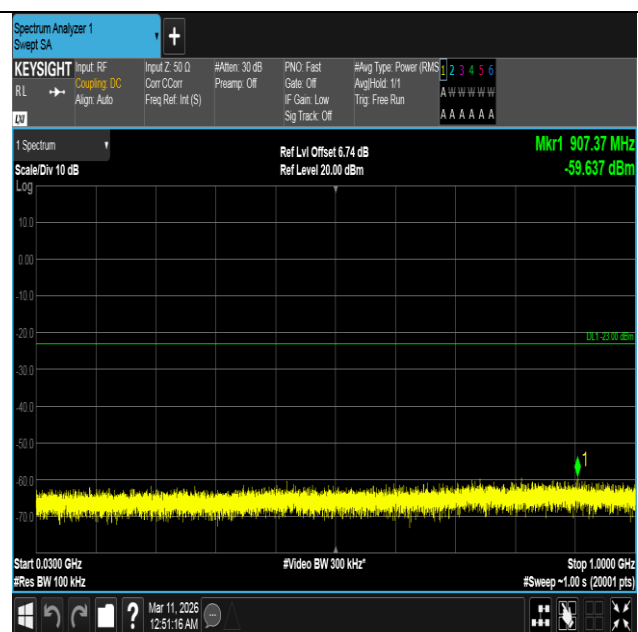
Band4-10MHz-16QAM-20000-50RB#0-30~1000-PASS
