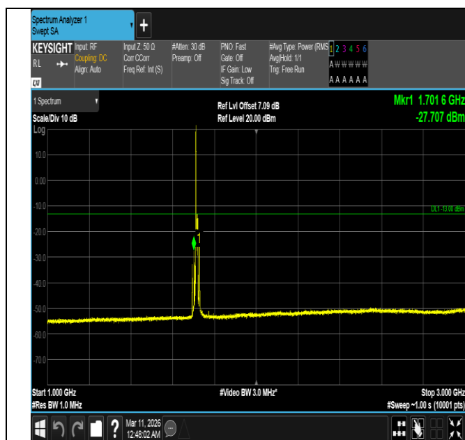
Band4-10MHz-16QAM-20000-1RB#0-1000~3000-PASS
