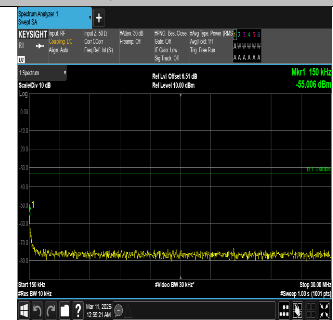
Band4-10MHz-QPSK-20175-50RB#0-0.15~30-PASS
