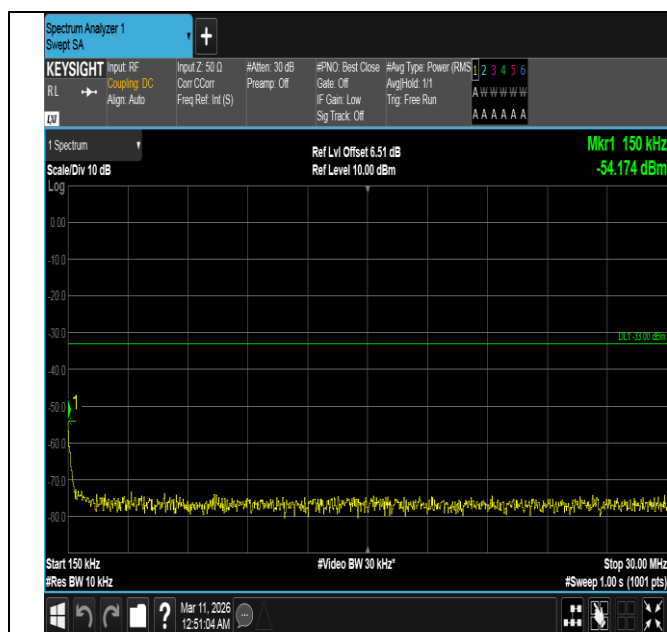
Band4-10MHz-16QAM-20000-50RB#0-0.15~30-PASS
