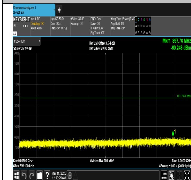
Band4-10MHz-QPSK-20000-50RB#0-30~1000-PASS
