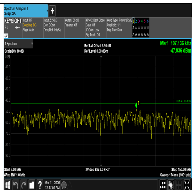
Band4-5MHz-16QAM-20375-25RB#0-0.009~0.15-PASS
