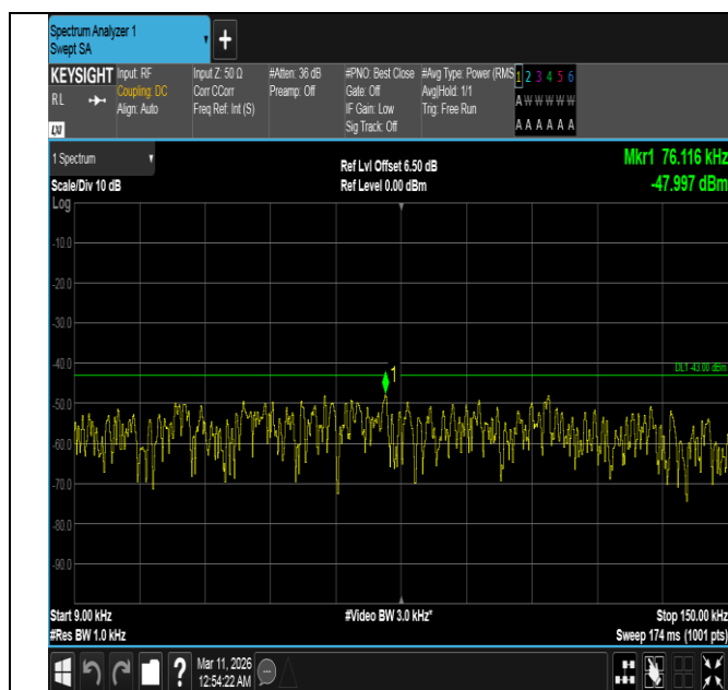
Band4-10MHz-16QAM-20175-1RB#49-0.009~0.15-PASS
