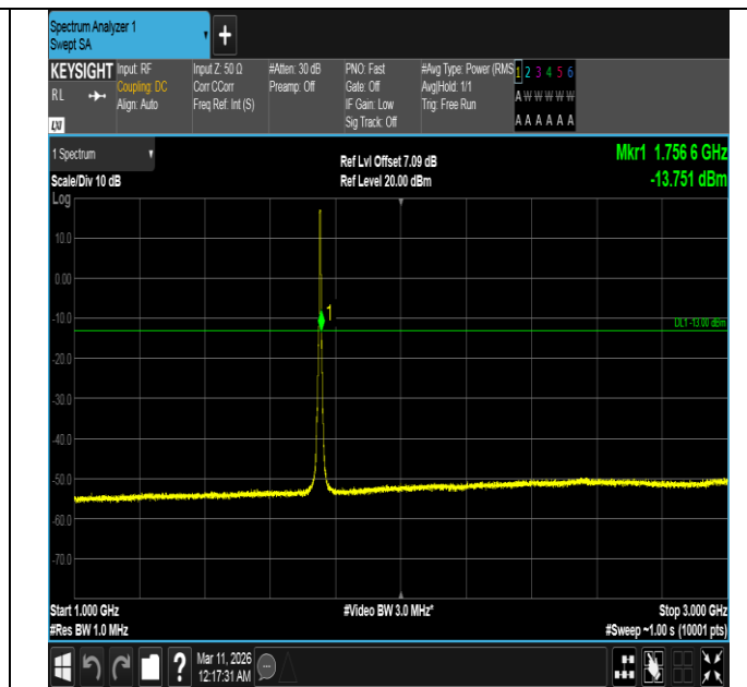
Band4-5MHz-QPSK-20375-25RB#0-1000~3000-PASS
