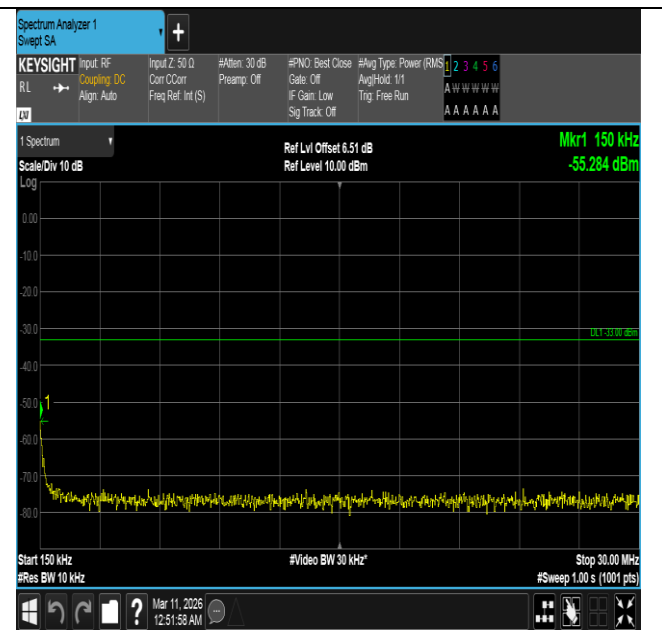
Band4-10MHz-QPSK-20175-1RB#0-0.15~30-PASS
