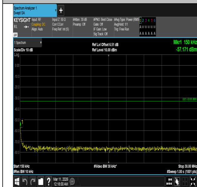
Band4-5MHz-16QAM-20375-25RB#0-0.15~30-PASS
