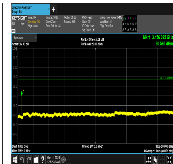
Band4-10MHz-QPSK-20175-1RB#0-3000~20000-PASS
