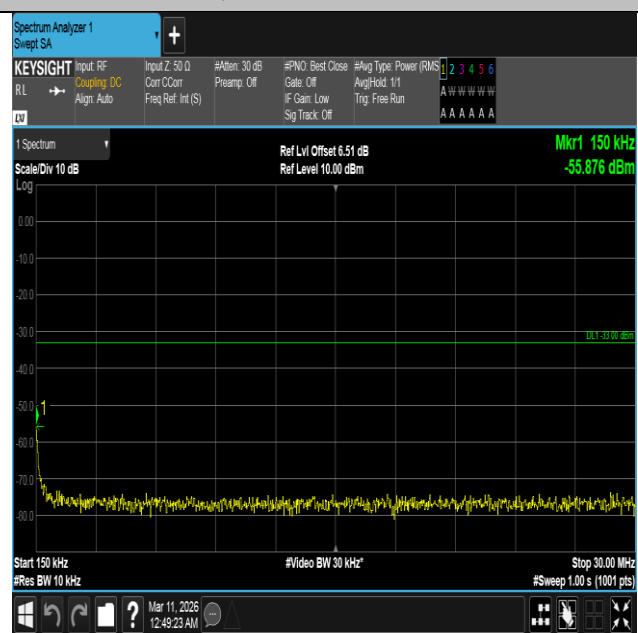
Band4-10MHz-16QAM-20000-1RB#49-0.15~30-PASS
