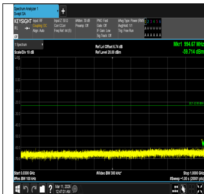
Band4-10MHz-QPSK-20000-1RB#0-30~1000-PASS
