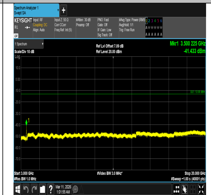
Band4-10MHz-16QAM-20350-50RB#0-3000~20000-PASS
