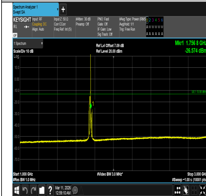
Band4-10MHz-QPSK-20350-1RB#49-1000~3000-PASS
