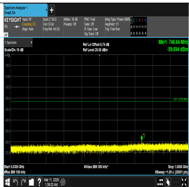
Band4-15MHz-QPSK-20175-1RB#74-30~1000-PASS
