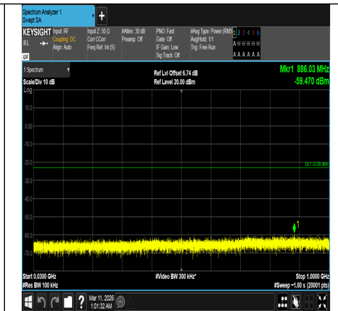
Band4-10MHz-16QAM-20350-50RB#0-30~1000-PASS
