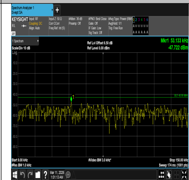
Band4-10MHz-16QAM-20350-50RB#0-0.009~0.15-PASS
