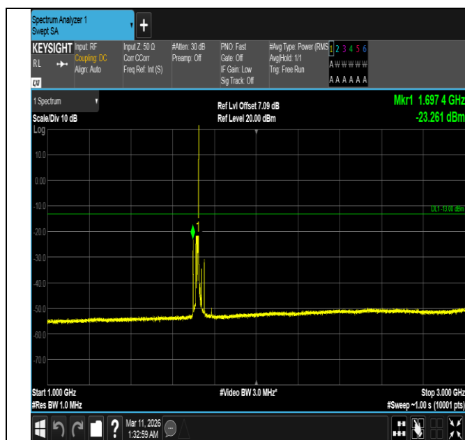
Band4-15MHz-QPSK-20025-1RB#74-1000~3000-PASS
