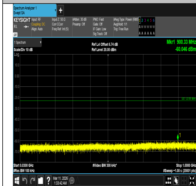
Band4-15MHz-16QAM-20025-1RB#74-30~1000-PASS
