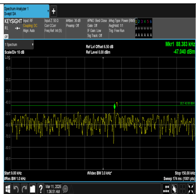
Band4-15MHz-16QAM-20175-1RB#0-0.009~0.15-PASS
