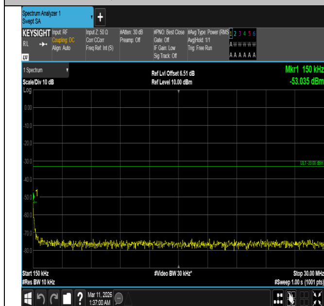
Band4-15MHz-16QAM-20175-1RB#0-0.15~30-PASS
