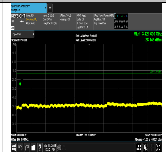
Band4-15MHz-16QAM-20025-1RB#0-3000~20000-PASS
