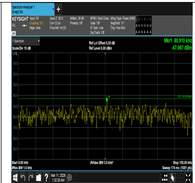
Band4-15MHz-QPSK-20025-1RB#74-0.009~0.15-PASS
