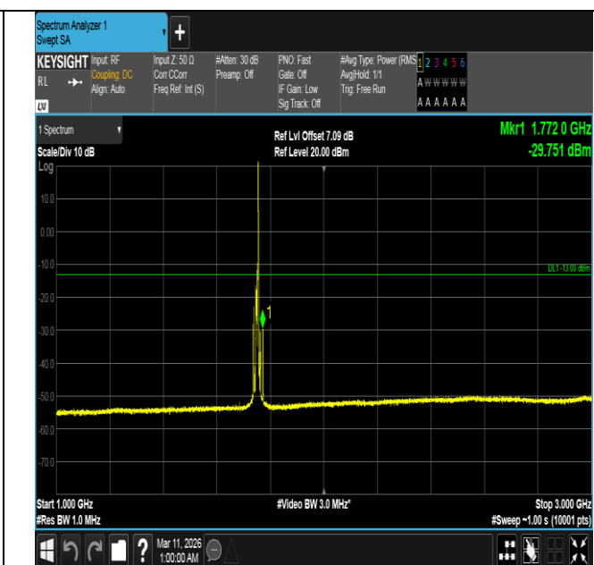
Band4-10MHz-16QAM-20350-1RB#49-1000~3000-PASS
