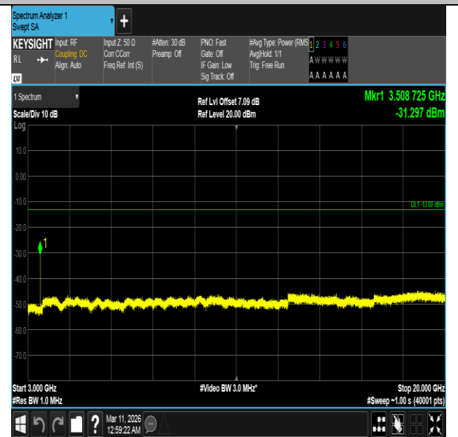
Band4-10MHz-QPSK-20350-1RB#49-3000~20000-PASS
