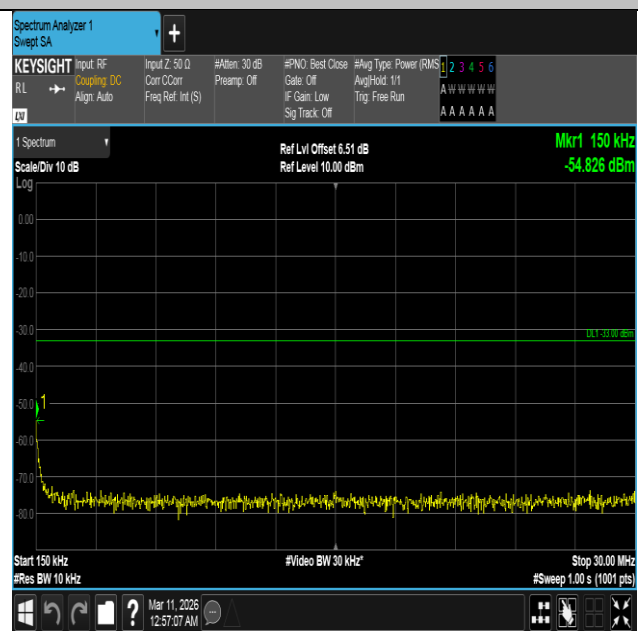
Band4-10MHz-QPSK-20350-1RB#0-0.15~30-PASS
