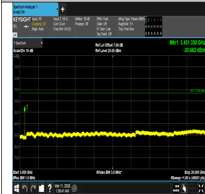
Band4-15MHz-QPSK-20175-1RB#0-3000~20000-PASS
