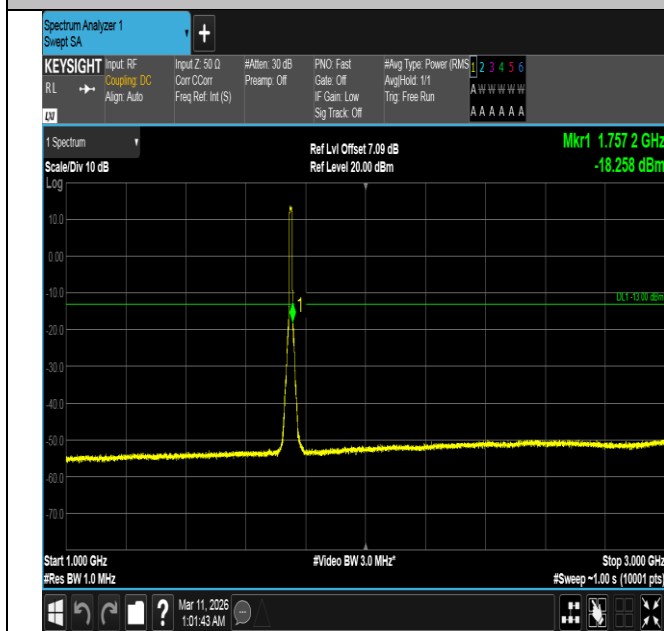
Band4-10MHz-16QAM-20350-50RB#0-1000~3000-PASS
