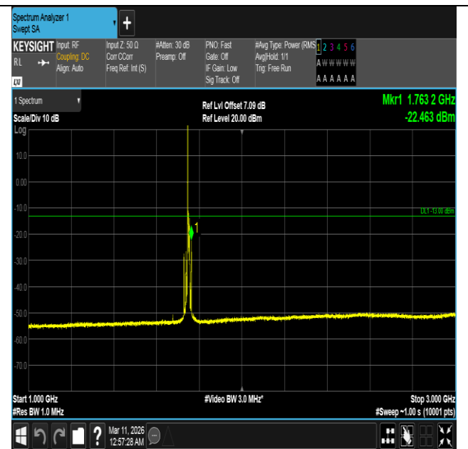
Band4-10MHz-QPSK-20350-1RB#0-1000~3000-PASS
