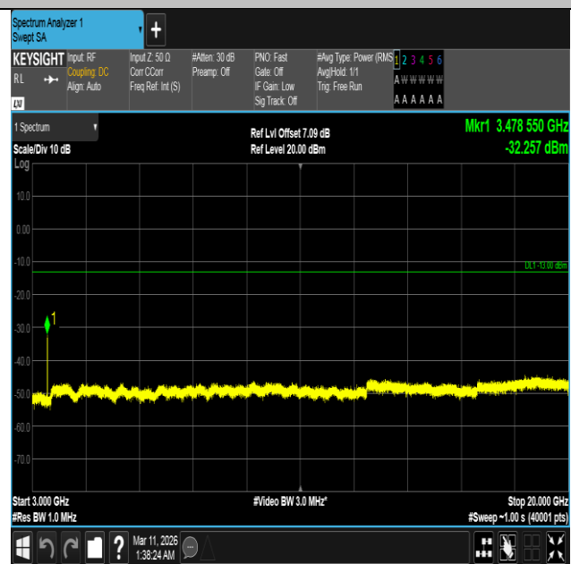
Band4-15MHz-QPSK-20175-1RB#74-3000~20000-PASS
