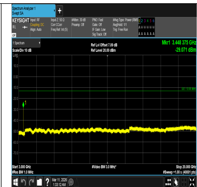
Band4-15MHz-QPSK-20025-1RB#74-3000~20000-PASS
