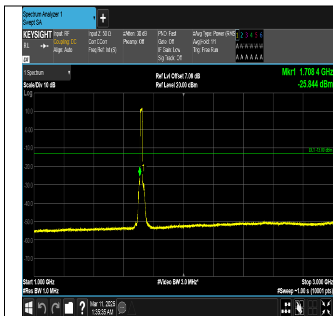
Band4-15MHz-16QAM-20025-75RB#0-1000~3000-PASS
