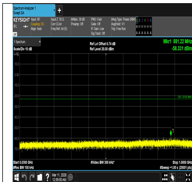
Band4-10MHz-16QAM-20350-1RB#49-30~1000-PASS
