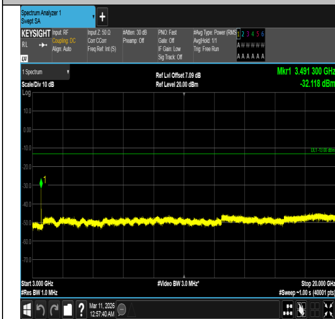
Band4-10MHz-QPSK-20350-1RB#0-3000~20000-PASS
