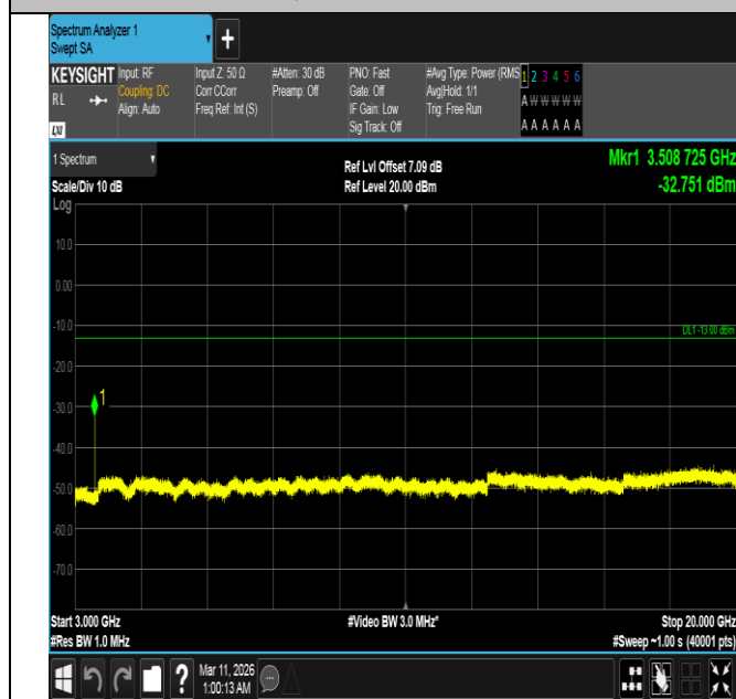
Band4-10MHz-16QAM-20350-1RB#49-3000~20000-PASS
