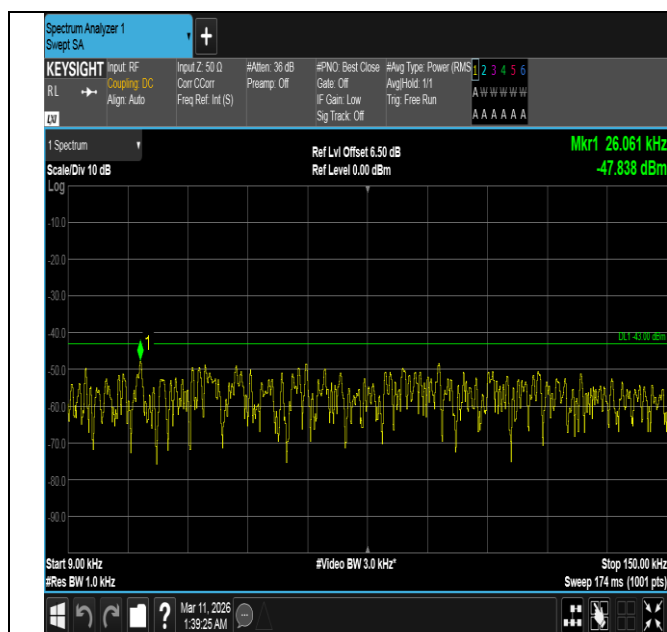
Band4-15MHz-QPSK-20175-75RB#0-0.009~0.15-PASS
