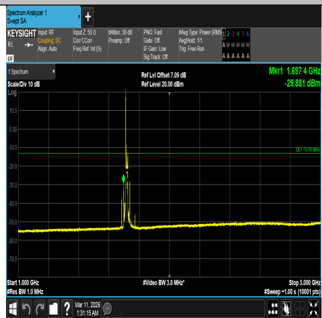
Band4-15MHz-QPSK-20025-1RB#0-1000~3000-PASS
