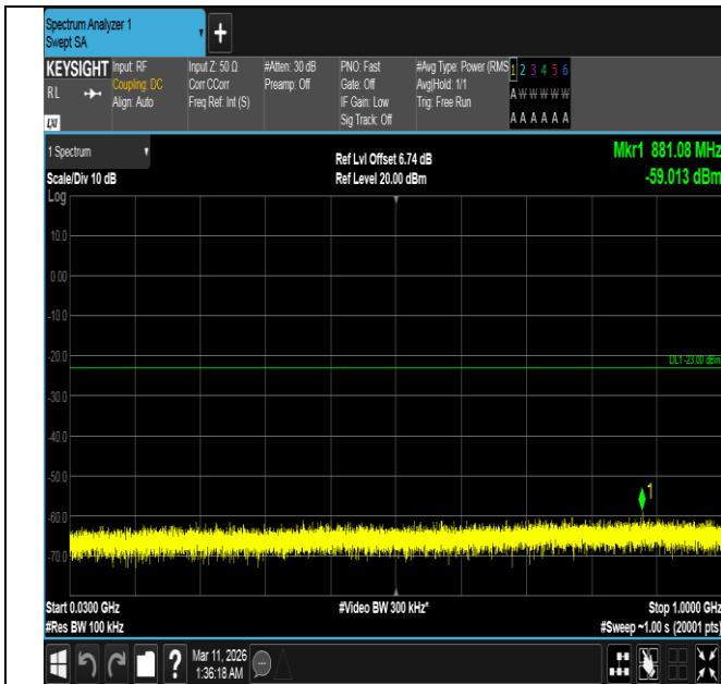
Band4-15MHz-QPSK-20175-1RB#0-30~1000-PASS
