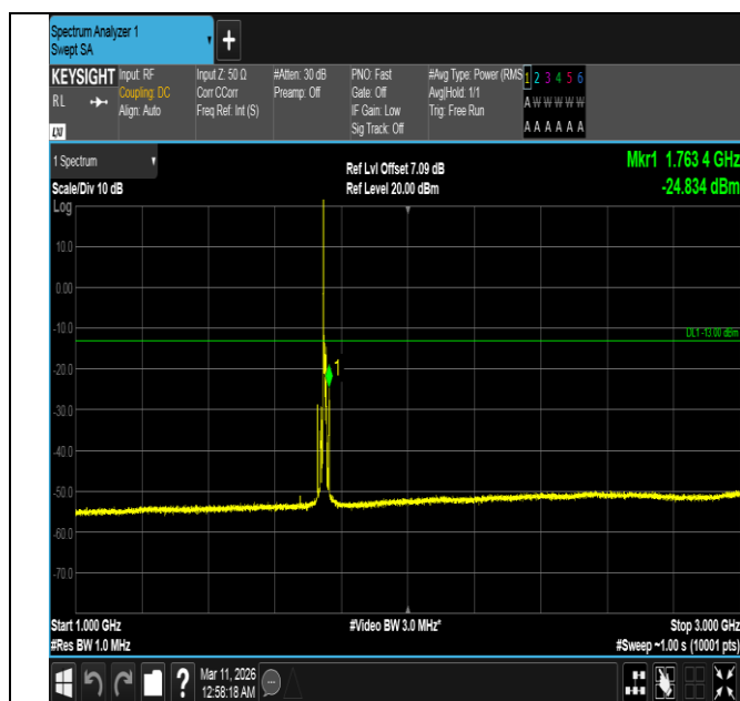
Band4-10MHz-16QAM-20350-1RB#0-1000~3000-PASS
