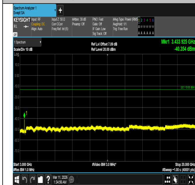
Band4-15MHz-QPSK-20025-75RB#0-3000~20000-PASS
