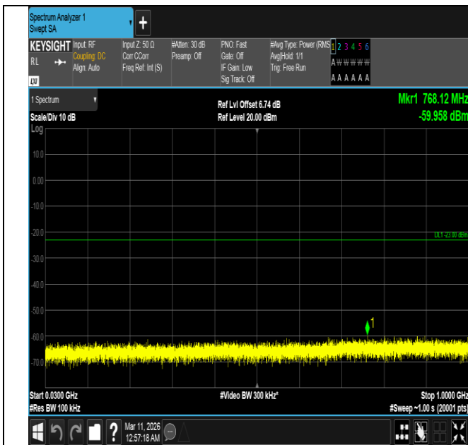
Band4-10MHz-QPSK-20350-1RB#0-30~1000-PASS
