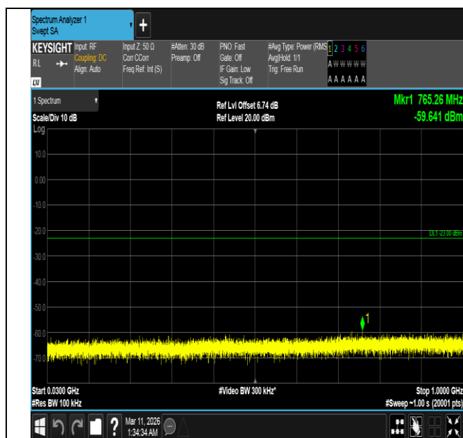
Band4-15MHz-QPSK-20025-75RB#0-30~1000-PASS
