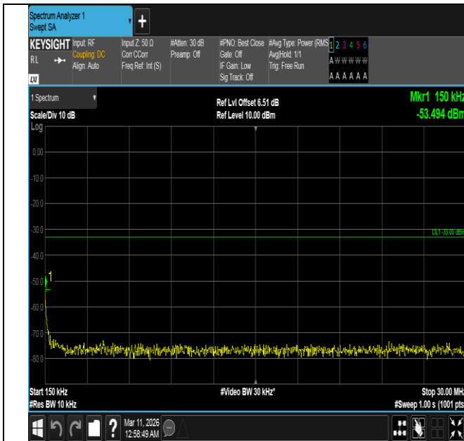
Band4-10MHz-QPSK-20350-1RB#49-0.15~30-PASS
