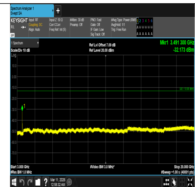
Band4-10MHz-16QAM-20350-1RB#0-3000~20000-PASS
