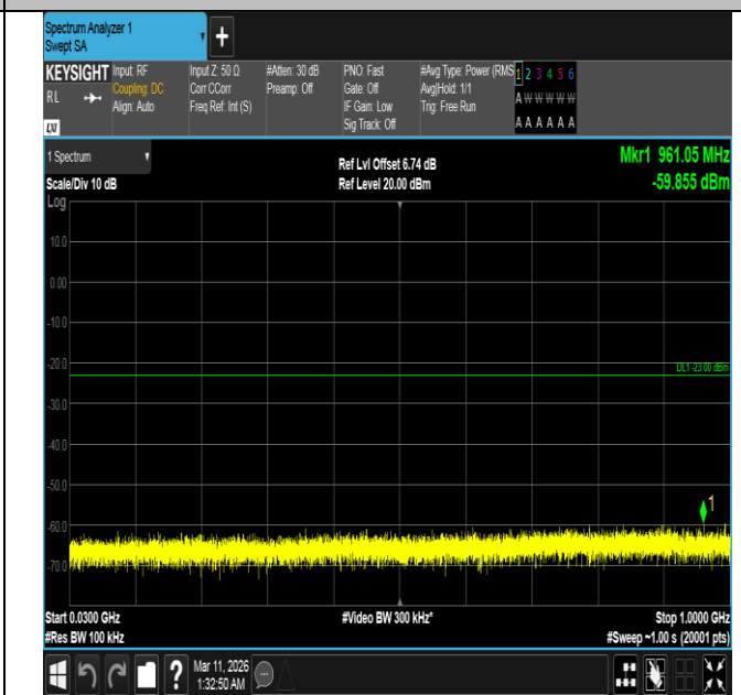
Band4-15MHz-QPSK-20025-1RB#74-30~1000-PASS
