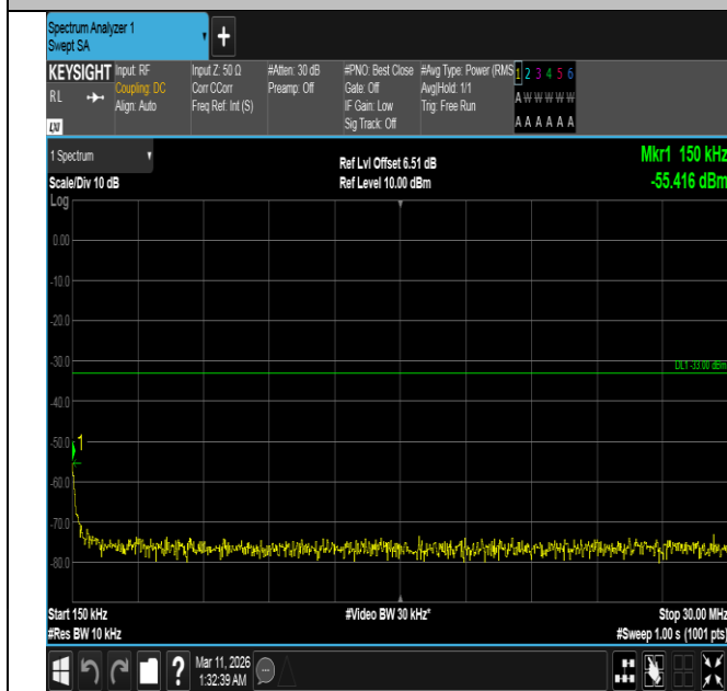
Band4-15MHz-QPSK-20025-1RB#74-0.15~30-PASS
