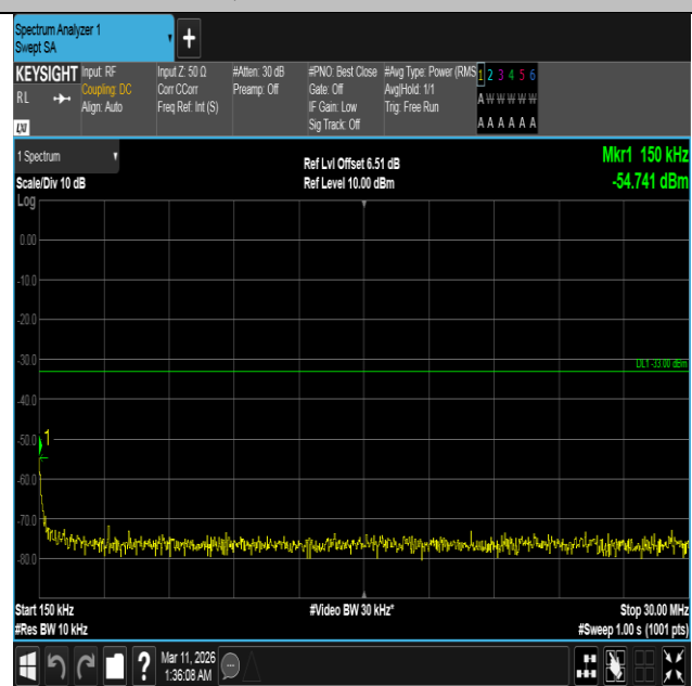
Band4-15MHz-QPSK-20175-1RB#0-0.15~30-PASS
