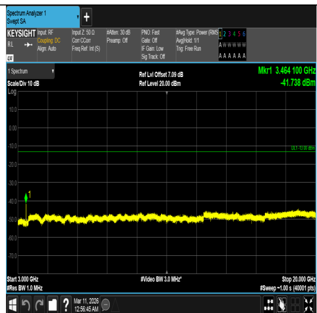
Band4-10MHz-16QAM-20175-50RB#0-3000~20000-PASS
