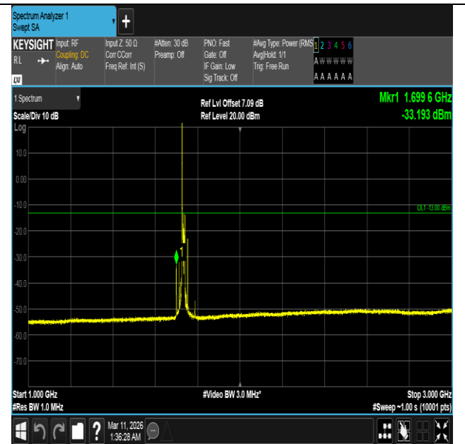
Band4-15MHz-QPSK-20175-1RB#0-1000~3000-PASS
