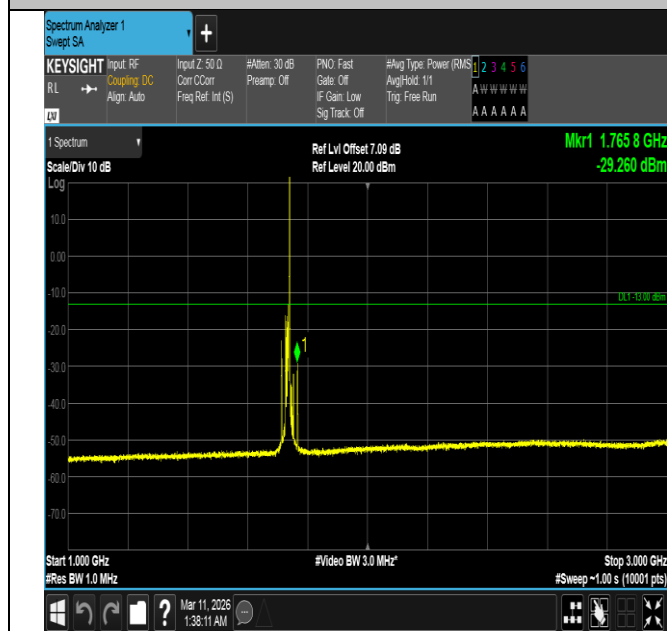
Band4-15MHz-QPSK-20175-1RB#74-1000~3000-PASS
