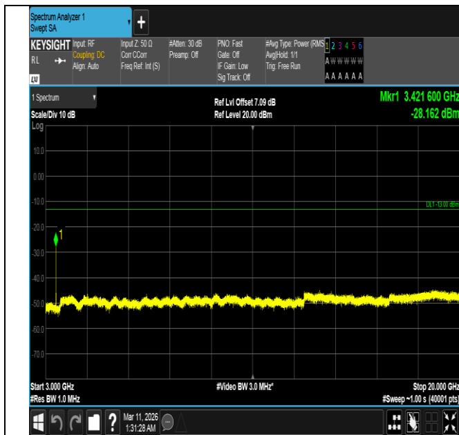
Band4-15MHz-QPSK-20025-1RB#0-3000~20000-PASS
