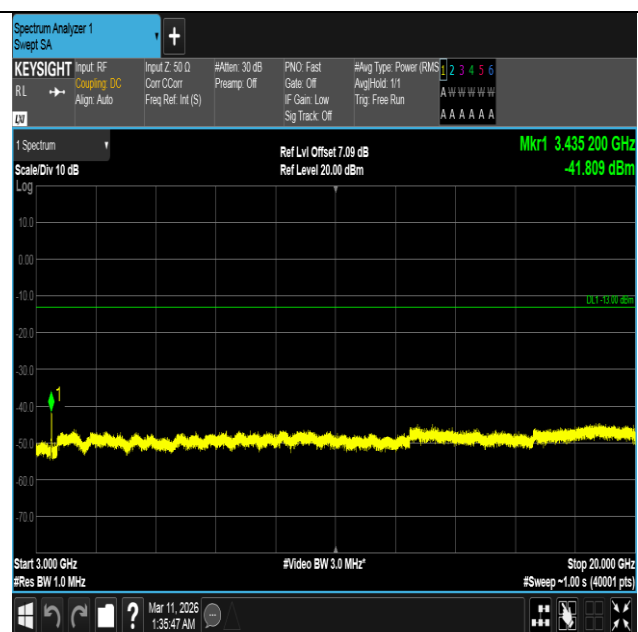
Band4-15MHz-16QAM-20025-75RB#0-3000~20000-PASS
