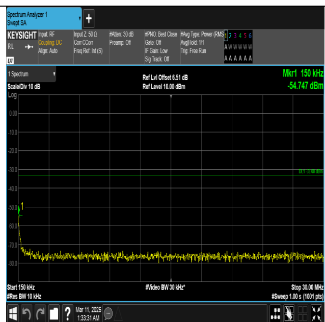
Band4-15MHz-16QAM-20025-1RB#74-0.15~30-PASS
