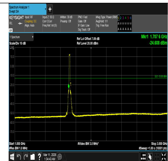
Band4-15MHz-QPSK-20025-75RB#0-1000~3000-PASS
