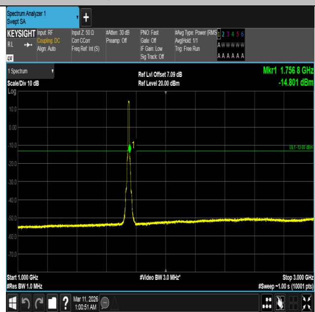
Band4-10MHz-QPSK-20350-50RB#0-1000~3000-PASS
