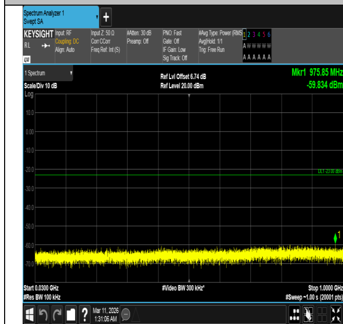
Band4-15MHz-QPSK-20025-1RB#0-30~1000-PASS
