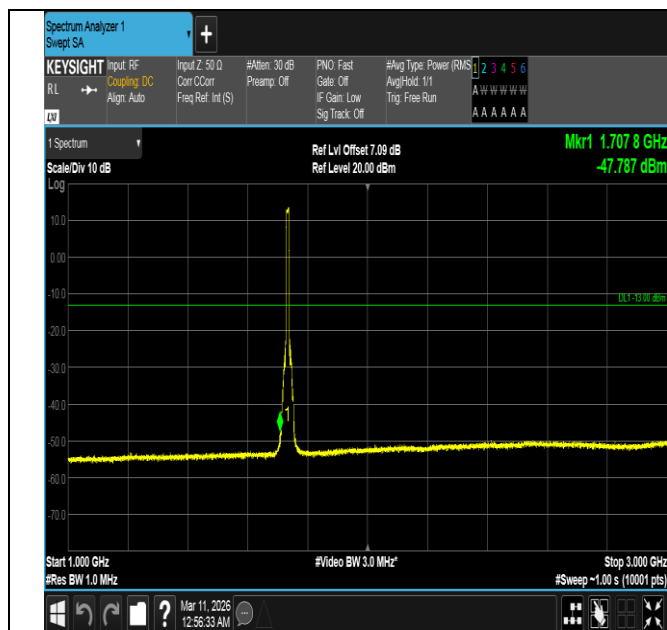
Band4-10MHz-16QAM-20175-50RB#0-1000~3000-PASS
