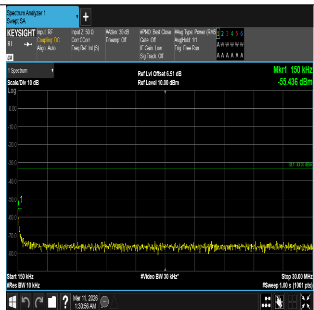
Band4-15MHz-QPSK-20025-1RB#0-0.15~30-PASS
