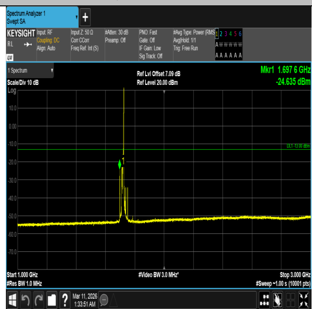
Band4-15MHz-16QAM-20025-1RB#74-1000~3000-PASS
