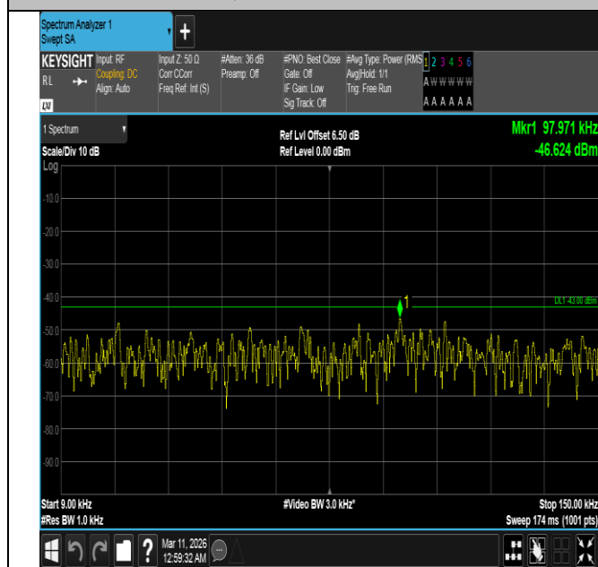
Band4-10MHz-16QAM-20350-1RB#49-0.009~0.15-PASS
