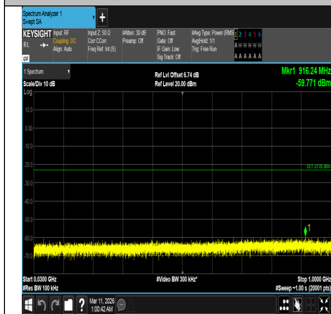
Band4-10MHz-QPSK-20350-50RB#0-30~1000-PASS
