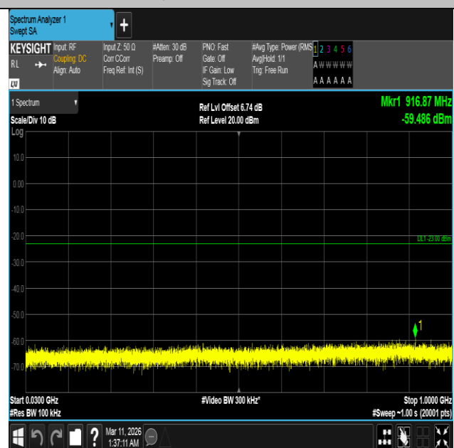
Band4-15MHz-16QAM-20175-1RB#0-30~1000-PASS
