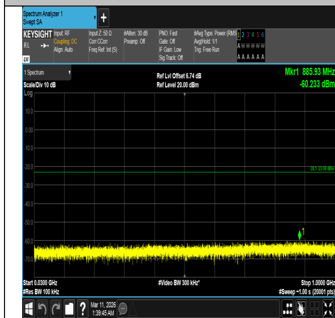
Band4-15MHz-QPSK-20175-75RB#0-30~1000-PASS
