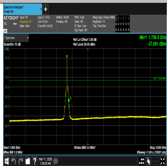
Band4-15MHz-QPSK-20175-75RB#0-1000~3000-PASS
