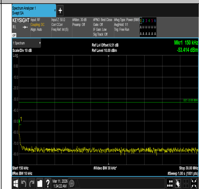
Band4-15MHz-QPSK-20025-75RB#0-0.15~30-PASS
