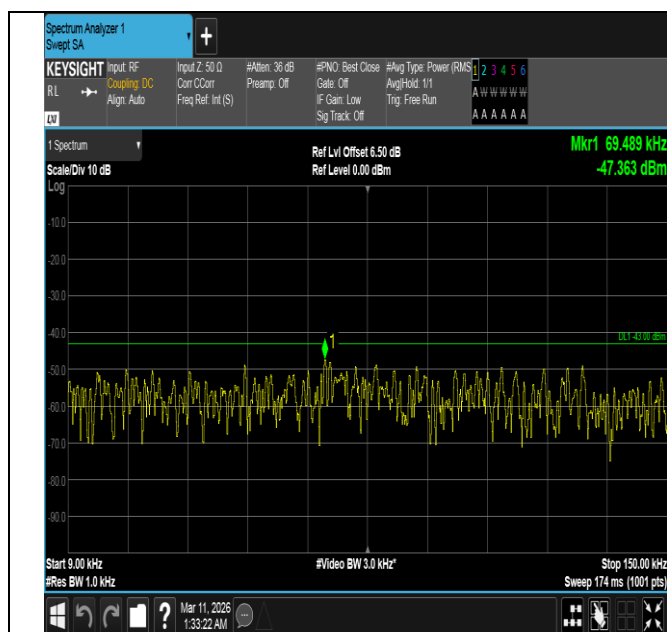
Band4-15MHz-16QAM-20025-1RB#74-0.009~0.15-PASS
