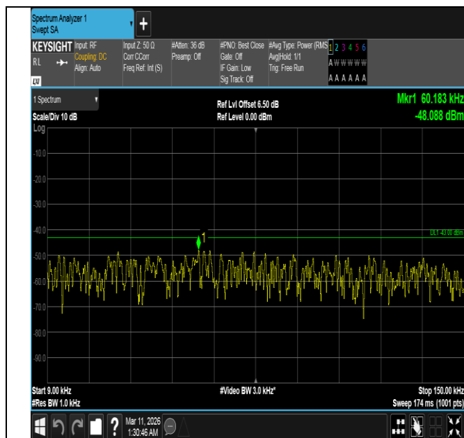
Band4-15MHz-QPSK-20025-1RB#0-0.009~0.15-PASS
