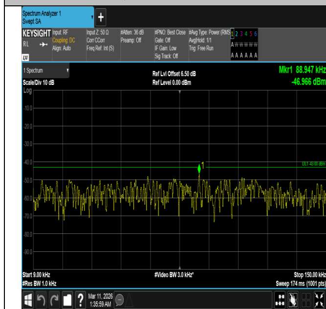
Band4-15MHz-QPSK-20175-1RB#0-0.009~0.15-PASS
