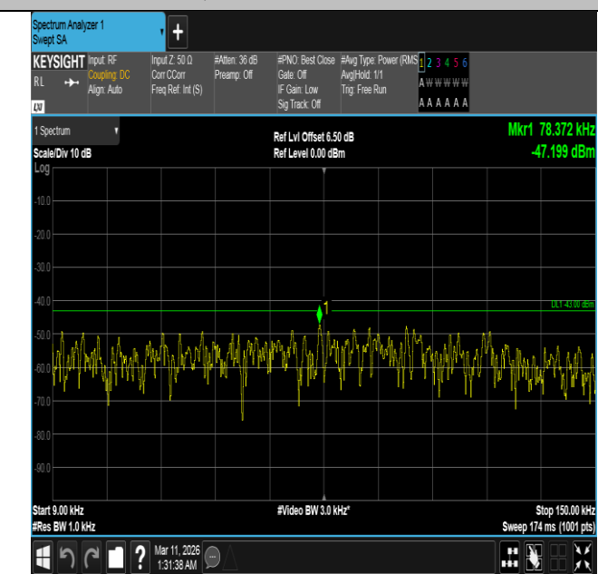
Band4-15MHz-16QAM-20025-1RB#0-0.009~0.15-PASS
