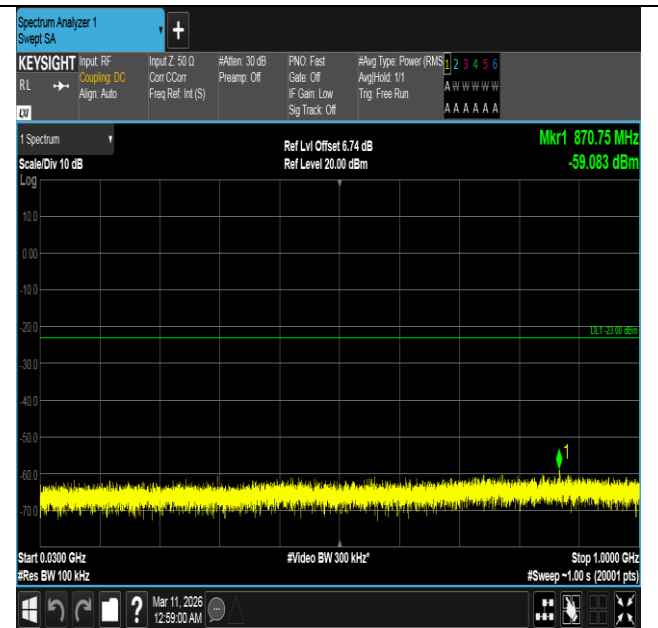
Band4-10MHz-QPSK-20350-1RB#49-30~1000-PASS
