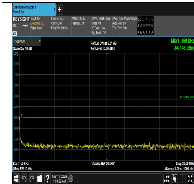
Band4-10MHz-16QAM-20350-50RB#0-0.15~30-PASS
