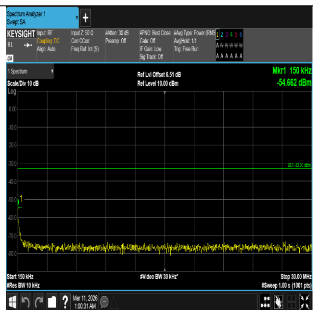
Band4-10MHz-QPSK-20350-50RB#0-0.15~30-PASS
