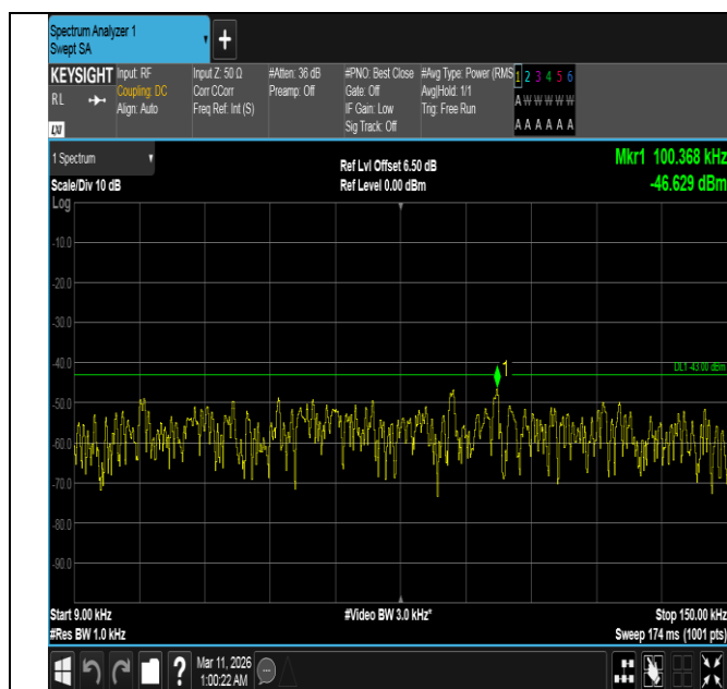
Band4-10MHz-QPSK-20350-50RB#0-0.009~0.15-PASS
