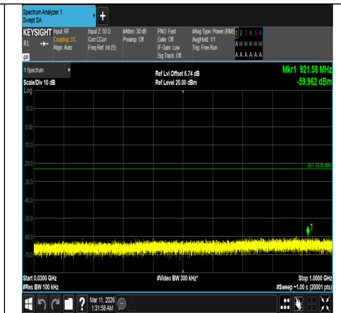
Band4-15MHz-16QAM-20025-1RB#0-30~1000-PASS
