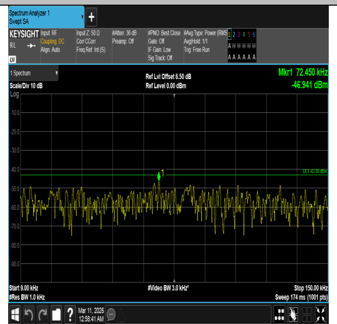
Band4-10MHz-QPSK-20350-1RB#49-0.009~0.15-PASS
