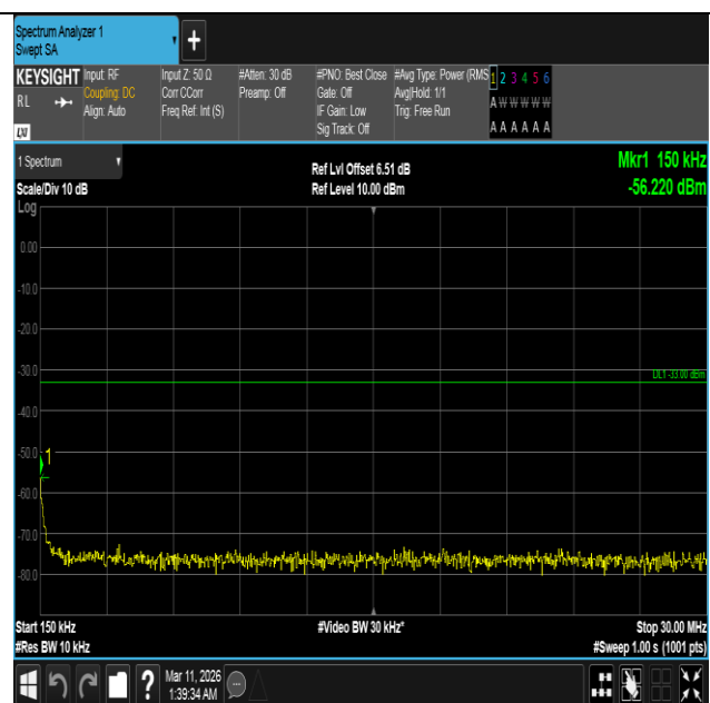
Band4-15MHz-QPSK-20175-75RB#0-0.15~30-PASS
