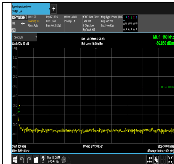
Band4-15MHz-QPSK-20175-1RB#74-0.15~30-PASS
