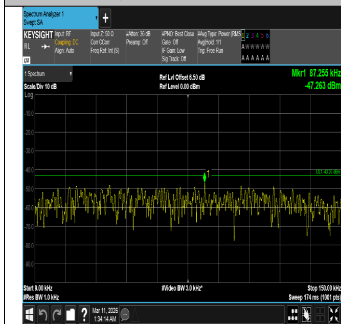
Band4-15MHz-QPSK-20025-75RB#0-0.009~0.15-PASS
