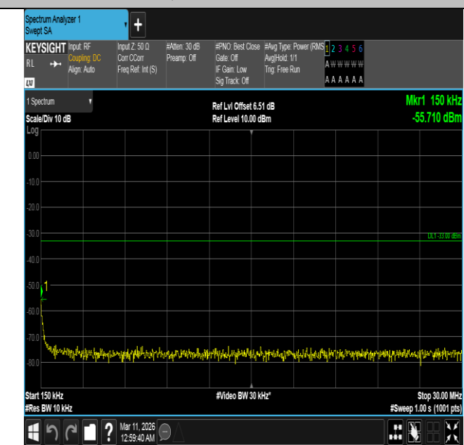
Band4-10MHz-16QAM-20350-1RB#49-0.15~30-PASS
