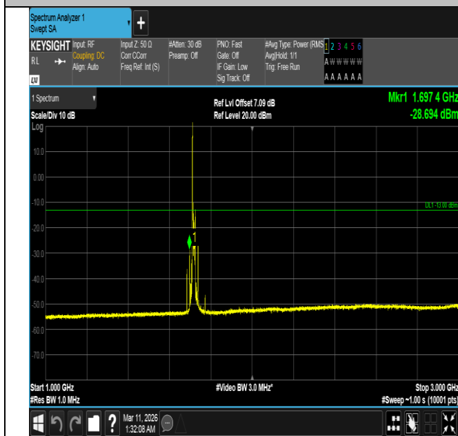
Band4-15MHz-16QAM-20025-1RB#0-1000~3000-PASS
