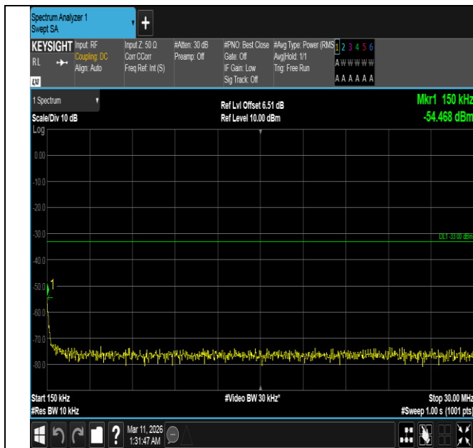
Band4-15MHz-16QAM-20025-1RB#0-0.15~30-PASS
