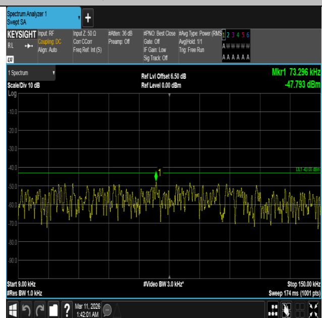
Band4-15MHz-16QAM-20325-1RB#0-0.009~0.15-PASS
