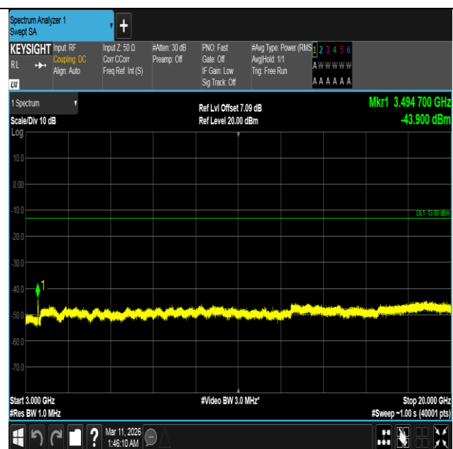
Band4-15MHz-16QAM-20325-75RB#0-3000~20000-PASS
