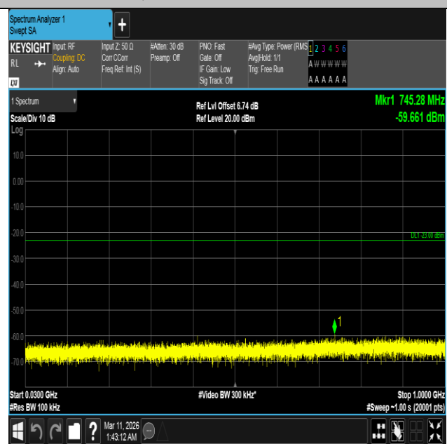
Band4-15MHz-QPSK-20325-1RB#74-30~1000-PASS
