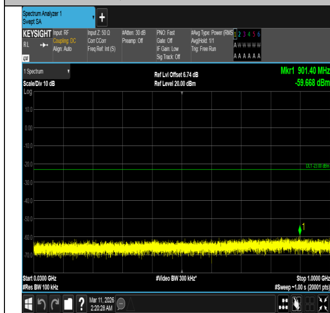
Band4-20MHz-QPSK-20175-1RB#0-30~1000-PASS
