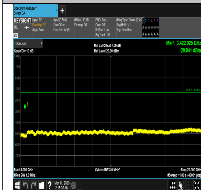
Band4-20MHz-QPSK-20050-1RB#0-3000~20000-PASS
