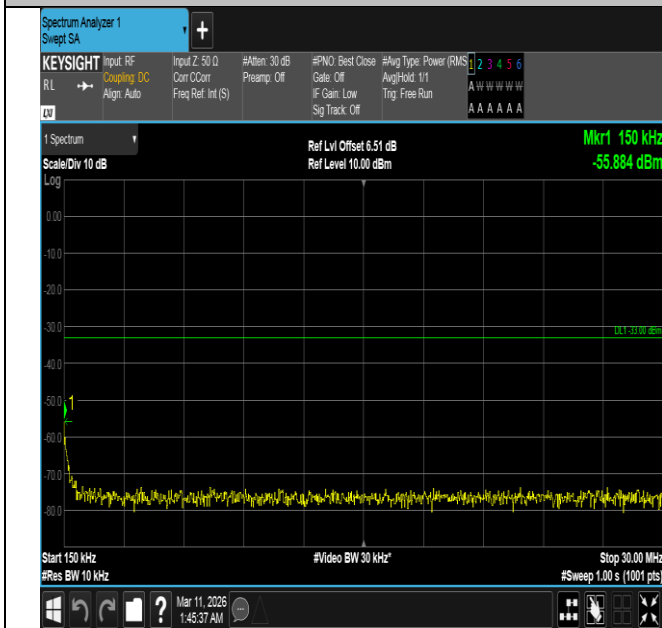
Band4-15MHz-16QAM-20325-75RB#0-0.15~30-PASS
