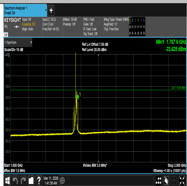
Band4-15MHz-QPSK-20325-1RB#0-1000~3000-PASS
