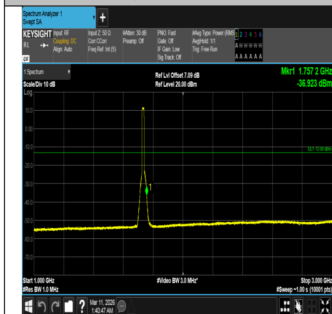
Band4-15MHz-16QAM-20175-75RB#0-1000~3000-PASS
