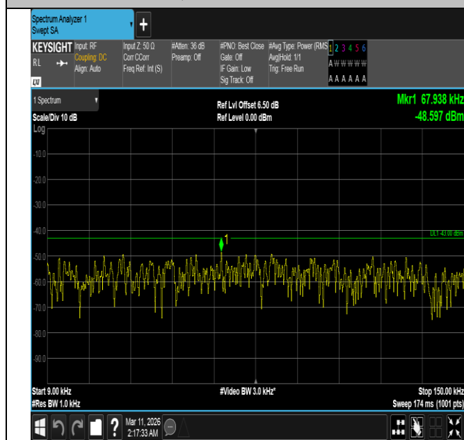
Band4-20MHz-16QAM-20050-1RB#99-0.009~0.15-PASS
