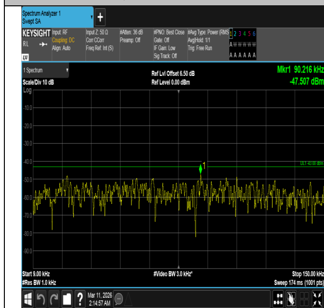
Band4-20MHz-QPSK-20050-1RB#0-0.009~0.15-PASS
