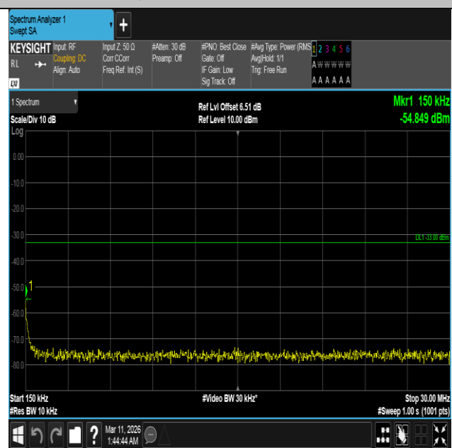
Band4-15MHz-QPSK-20325-75RB#0-0.15~30-PASS
