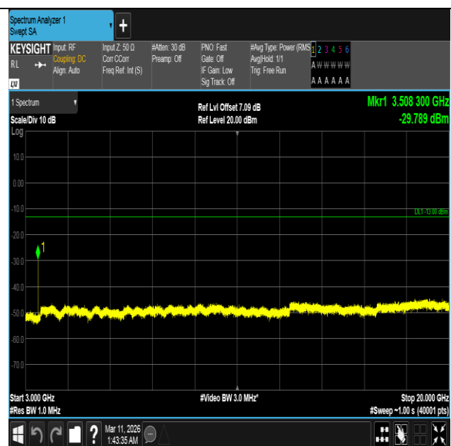
Band4-15MHz-QPSK-20325-1RB#74-3000~20000-PASS
