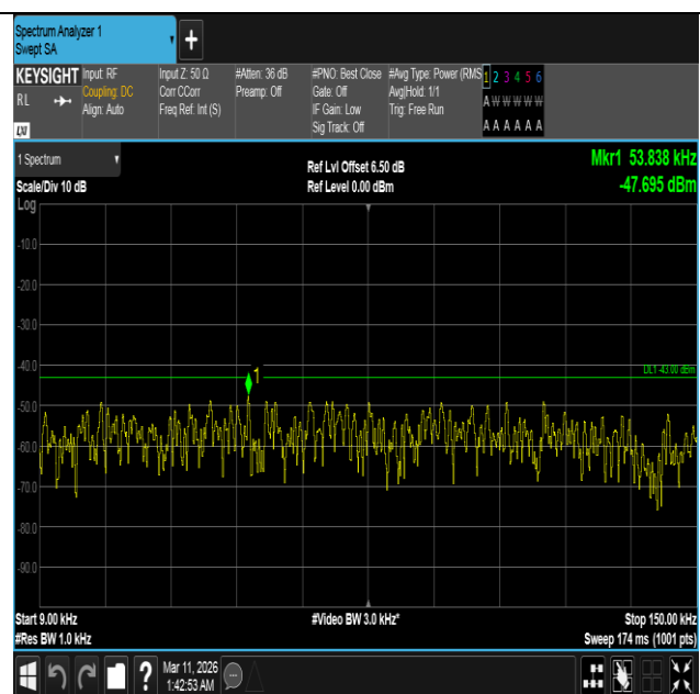
Band4-15MHz-QPSK-20325-1RB#74-0.009~0.15-PASS
