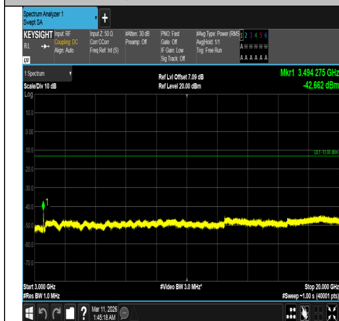
Band4-15MHz-QPSK-20325-75RB#0-3000~20000-PASS
