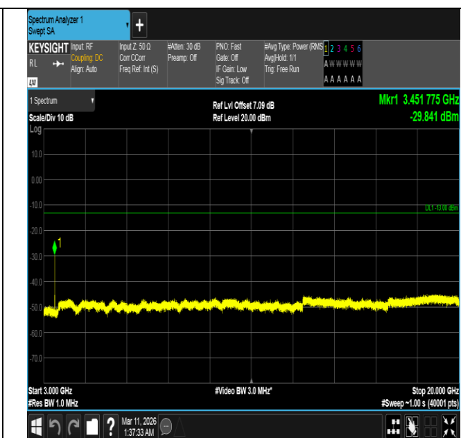
Band4-15MHz-16QAM-20175-1RB#0-3000~20000-PASS
