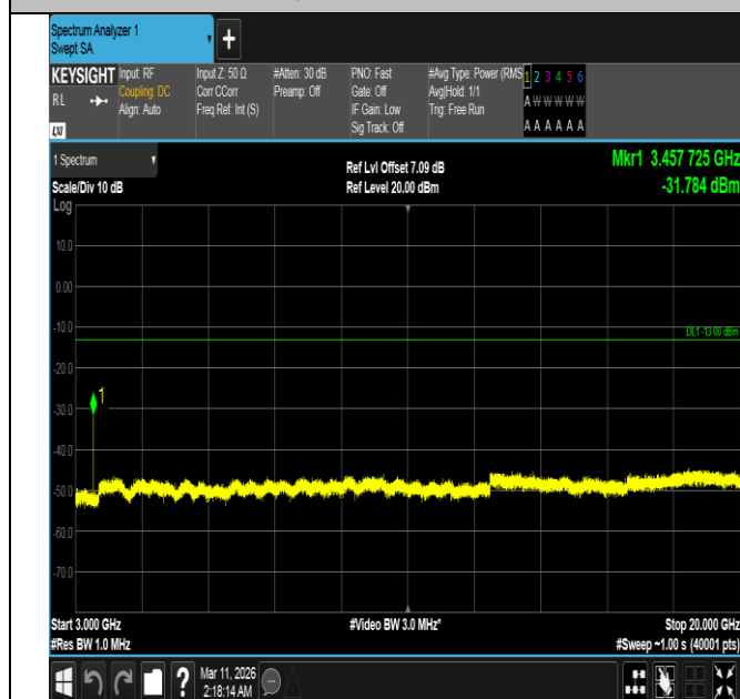
Band4-20MHz-16QAM-20050-1RB#99-3000~20000-PASS
