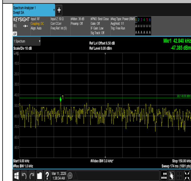
Band4-15MHz-16QAM-20175-1RB#74-0.009~0.15-PASS
