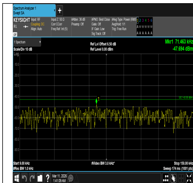
Band4-15MHz-QPSK-20325-1RB#0-0.009~0.15-PASS
