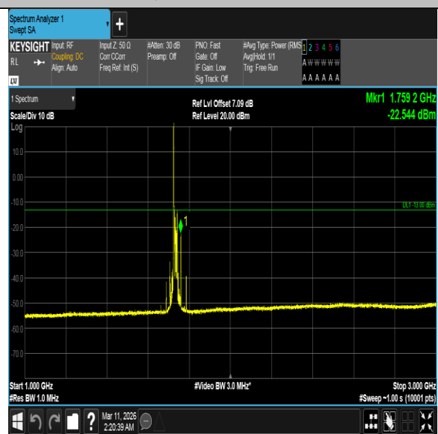
Band4-20MHz-QPSK-20175-1RB#0-1000~3000-PASS
