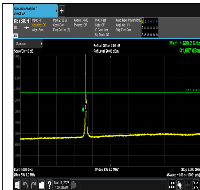
Band4-15MHz-16QAM-20175-1RB#0-1000~3000-PASS
