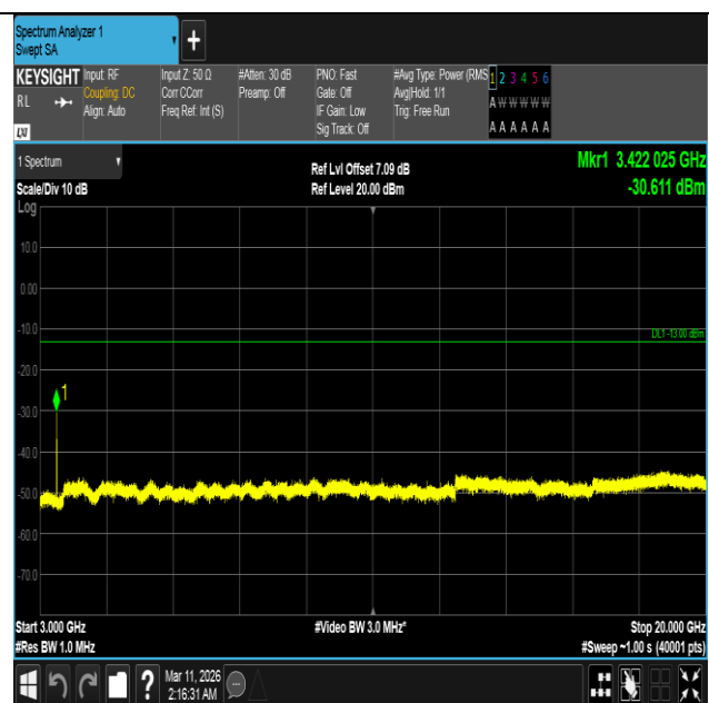
Band4-20MHz-16QAM-20050-1RB#0-3000~20000-PASS
