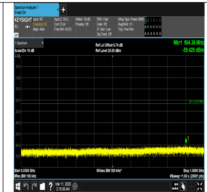
Band4-20MHz-16QAM-20050-100RB#0-30~1000-PASS
