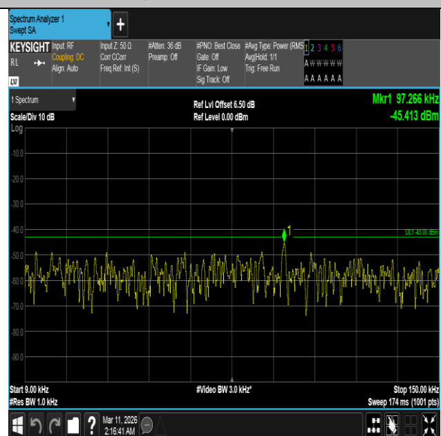
Band4-20MHz-QPSK-20050-1RB#99-0.009~0.15-PASS
