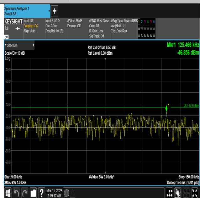
Band4-20MHz-16QAM-20050-100RB#0-0.009~0.15-PASS
