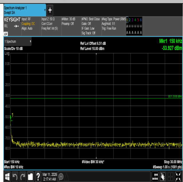
Band4-20MHz-16QAM-20050-1RB#99-0.15~30-PASS
