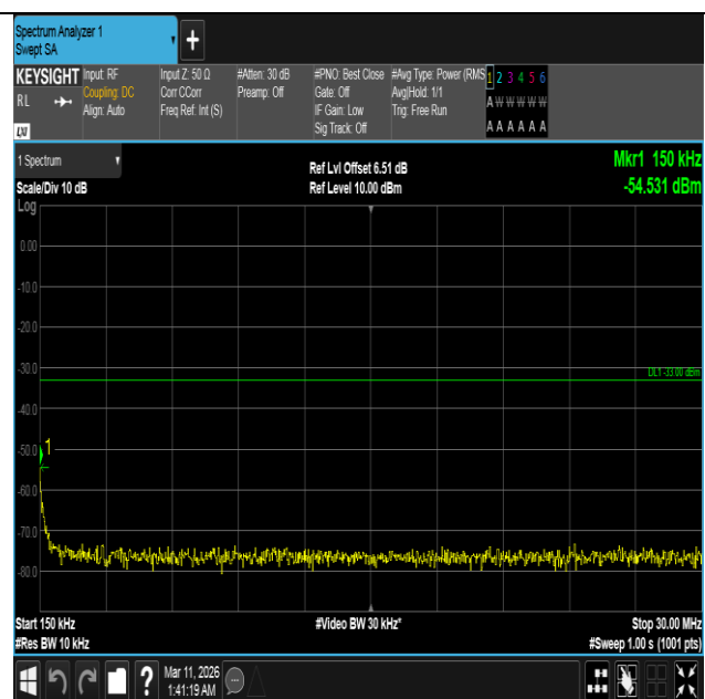
Band4-15MHz-QPSK-20325-1RB#0-0.15~30-PASS
