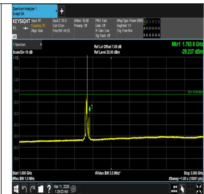
Band4-15MHz-16QAM-20175-1RB#74-1000~3000-PASS
