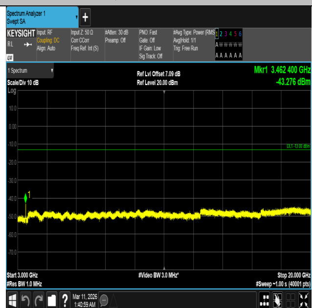
Band4-15MHz-16QAM-20175-75RB#0-3000~20000-PASS
