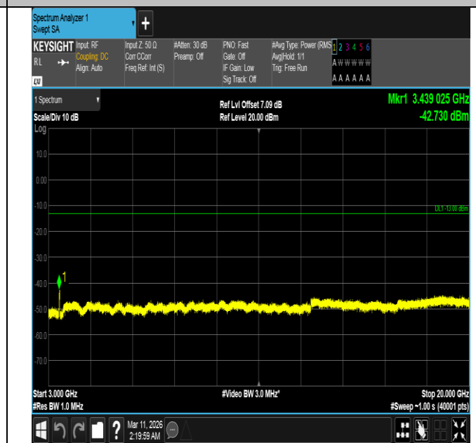
Band4-20MHz-16QAM-20050-100RB#0-3000~20000-PASS
