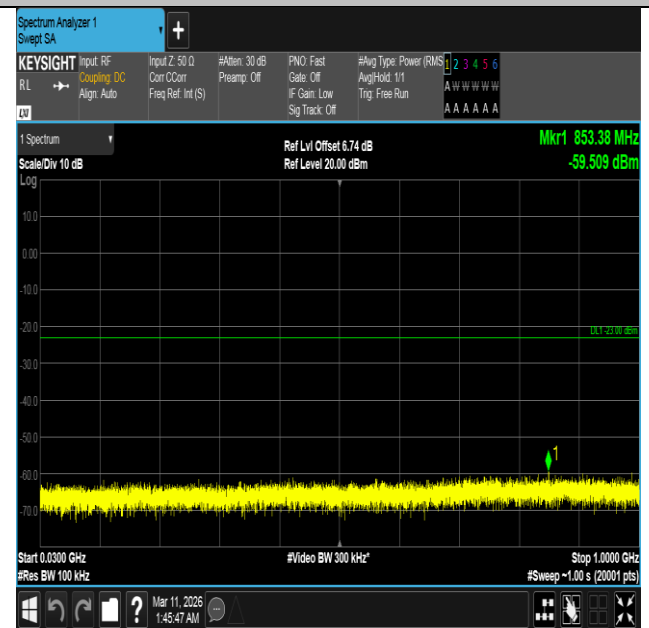
Band4-15MHz-16QAM-20325-75RB#0-30~1000-PASS
