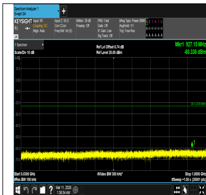
Band4-15MHz-16QAM-20175-1RB#74-30~1000-PASS
