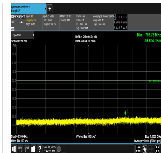
Band4-15MHz-QPSK-20325-75RB#0-30~1000-PASS
