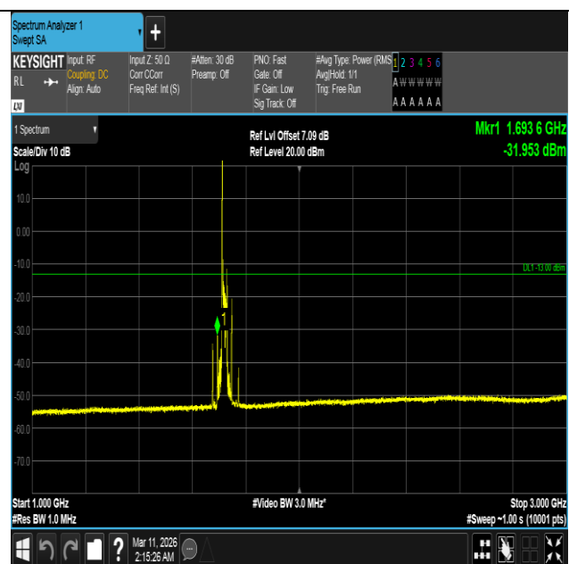
Band4-20MHz-QPSK-20050-1RB#0-1000~3000-PASS
