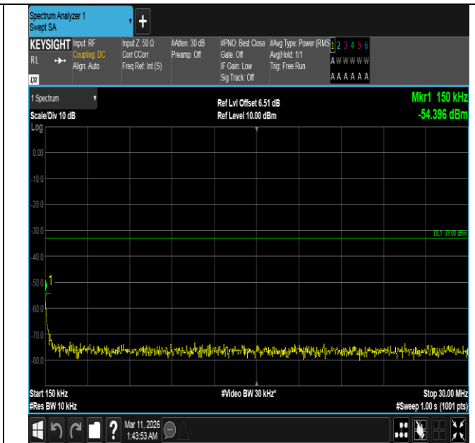
Band4-15MHz-16QAM-20325-1RB#74-0.15~30-PASS
