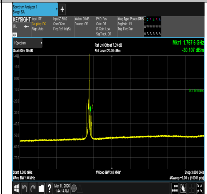
Band4-15MHz-16QAM-20325-1RB#74-1000~3000-PASS
