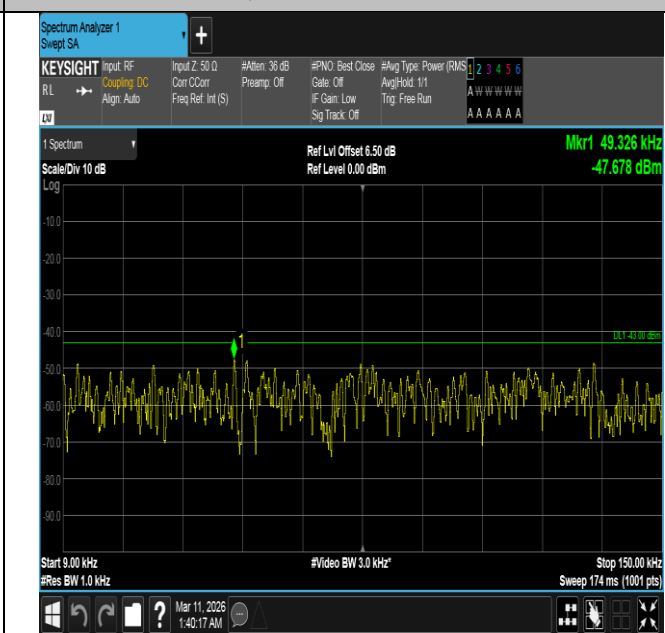
Band4-15MHz-16QAM-20175-75RB#0-0.009~0.15-PASS
