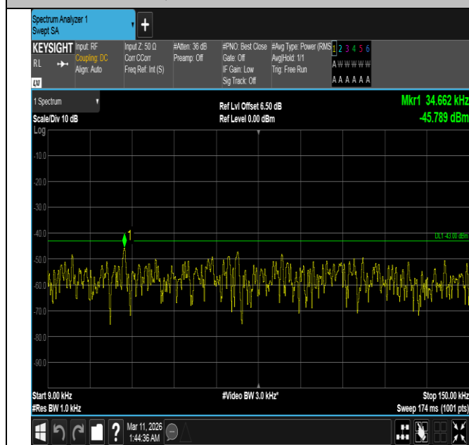
Band4-15MHz-QPSK-20325-75RB#0-0.009~0.15-PASS
