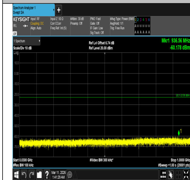
Band4-15MHz-QPSK-20325-1RB#0-30~1000-PASS
