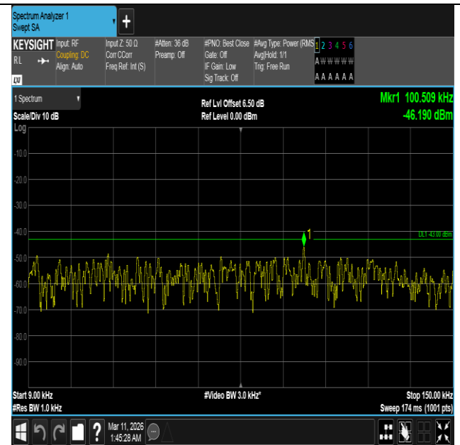
Band4-15MHz-16QAM-20325-75RB#0-0.009~0.15-PASS
