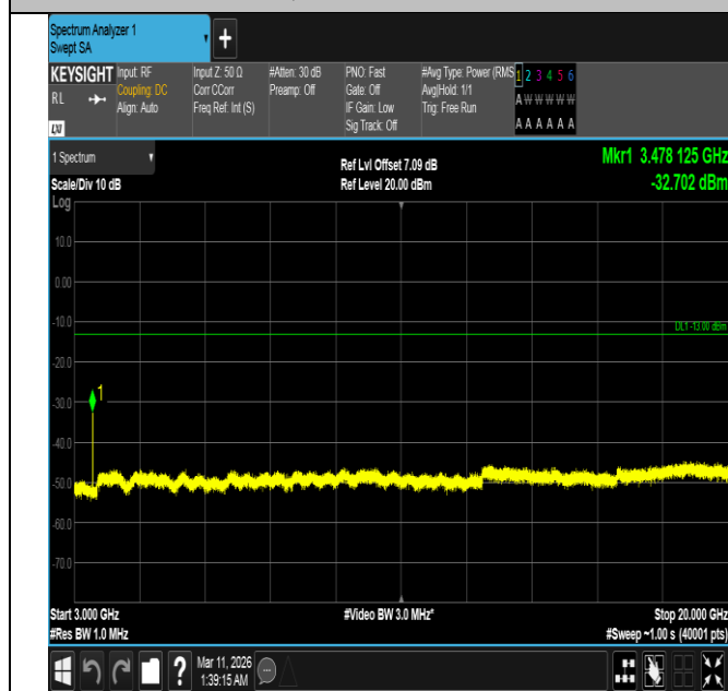
Band4-15MHz-16QAM-20175-1RB#74-3000~20000-PASS
