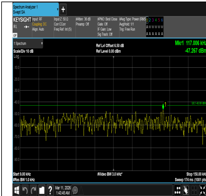
Band4-15MHz-16QAM-20325-1RB#74-0.009~0.15-PASS
