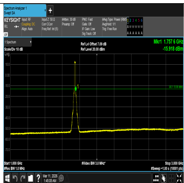
Band4-15MHz-QPSK-20325-75RB#0-1000~3000-PASS
