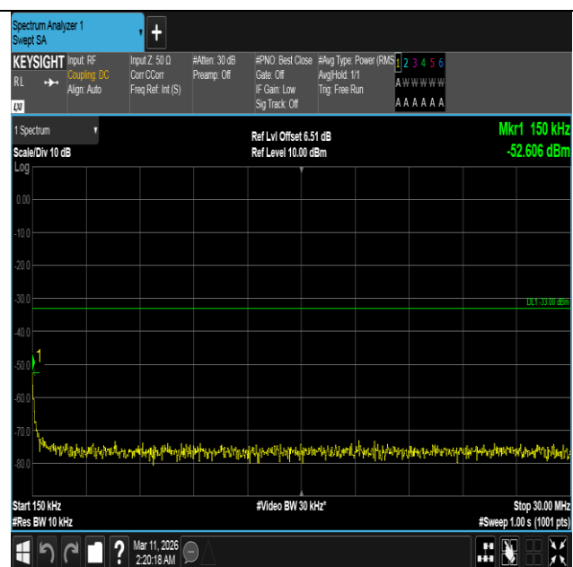
Band4-20MHz-QPSK-20175-1RB#0-0.15~30-PASS
