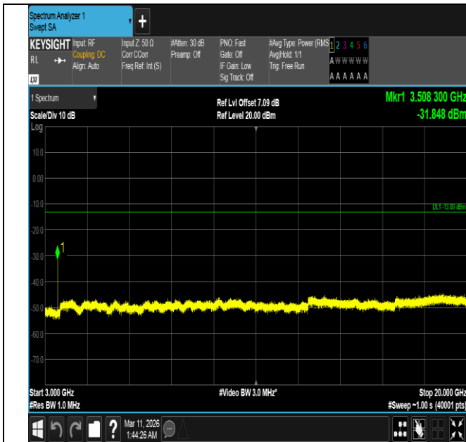
Band4-15MHz-16QAM-20325-1RB#74-3000~20000-PASS
