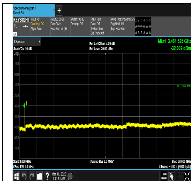
Band4-15MHz-QPSK-20325-1RB#0-3000~20000-PASS
