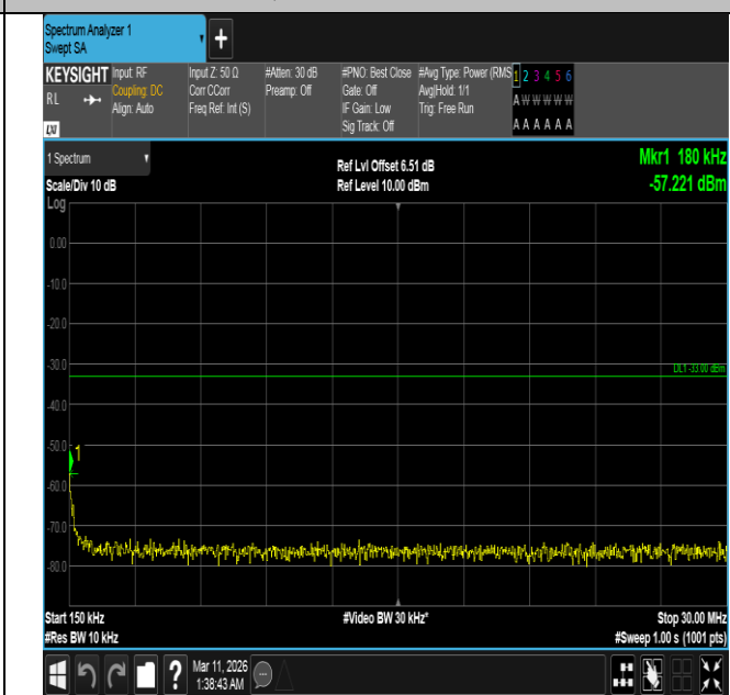
Band4-15MHz-16QAM-20175-1RB#74-0.15~30-PASS
