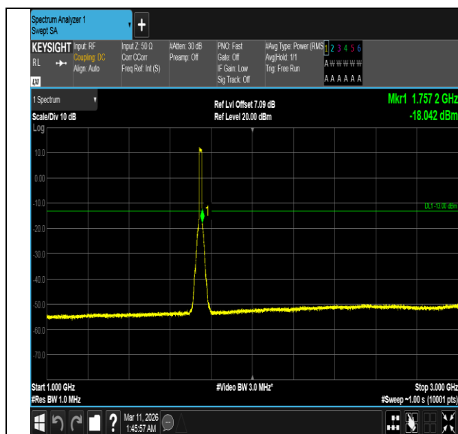
Band4-15MHz-16QAM-20325-75RB#0-1000~3000-PASS
