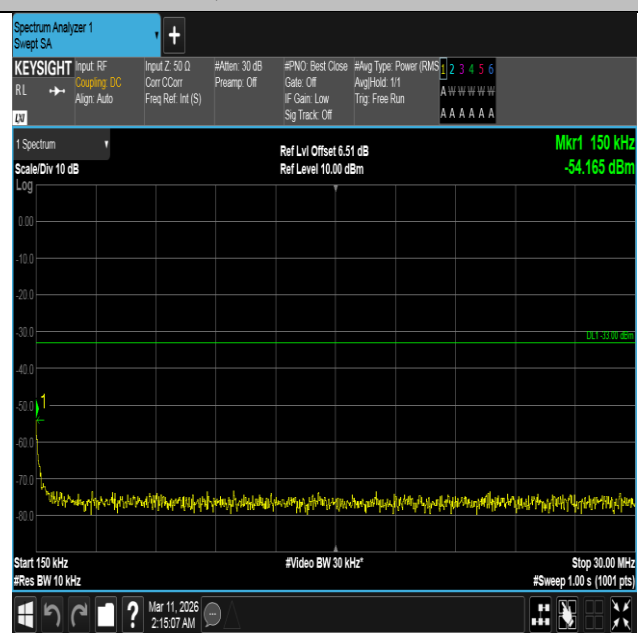
Band4-20MHz-QPSK-20050-1RB#0-0.15~30-PASS
