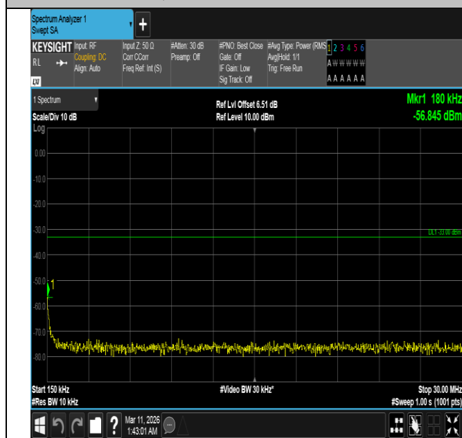
Band4-15MHz-QPSK-20325-1RB#74-0.15~30-PASS
