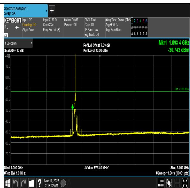
Band4-20MHz-16QAM-20050-1RB#99-1000~3000-PASS
