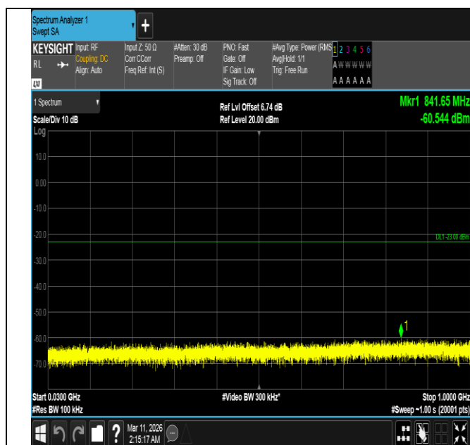
Band4-20MHz-QPSK-20050-1RB#0-30~1000-PASS
