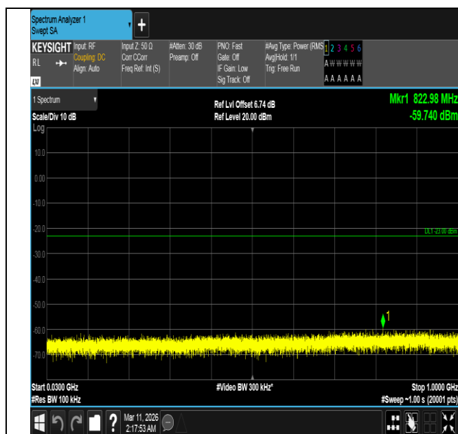
Band4-20MHz-16QAM-20050-1RB#99-30~1000-PASS
