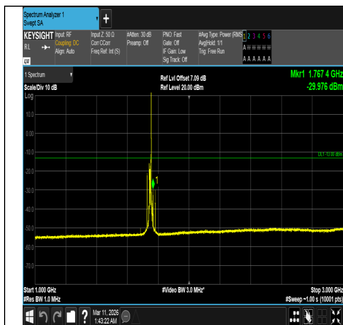
Band4-15MHz-QPSK-20325-1RB#74-1000~3000-PASS
