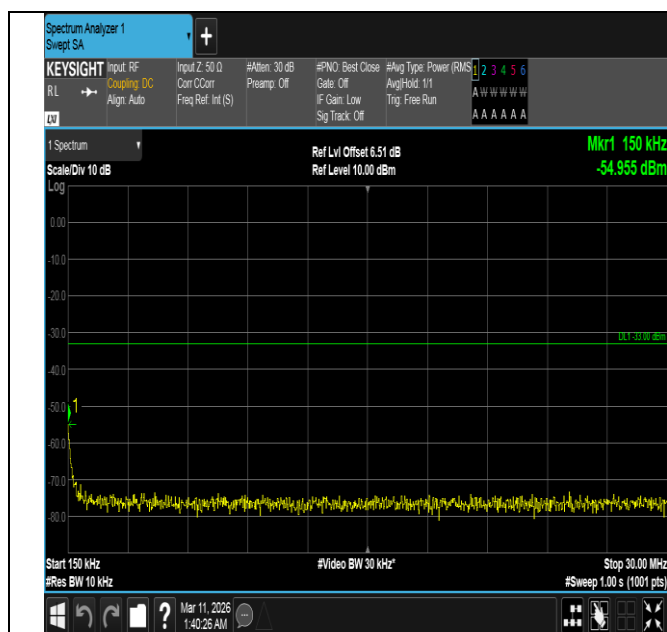
Band4-15MHz-16QAM-20175-75RB#0-0.15~30-PASS
