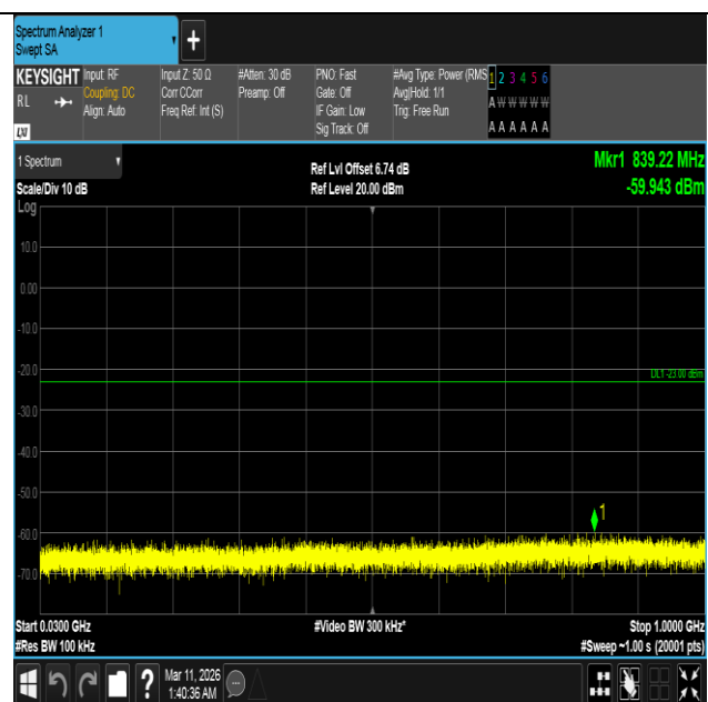
Band4-15MHz-16QAM-20175-75RB#0-30~1000-PASS
