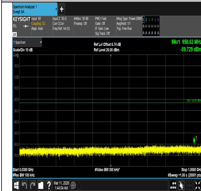
Band4-15MHz-16QAM-20325-1RB#74-30~1000-PASS
