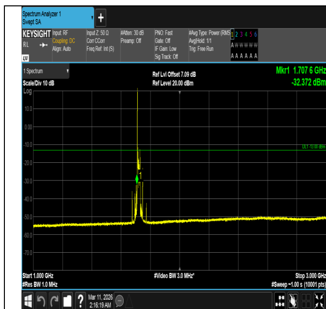
Band4-20MHz-16QAM-20050-1RB#0-1000~3000-PASS
