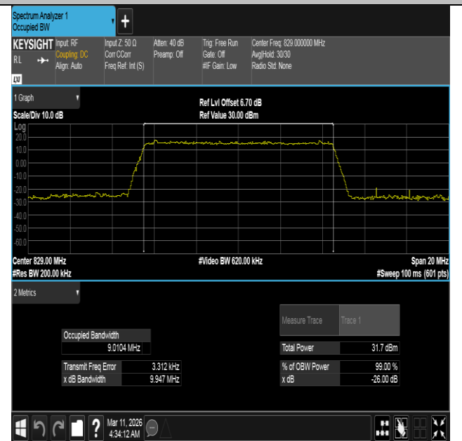
Band5-10MHz-16QAM-20450-50RB#0-PASS
