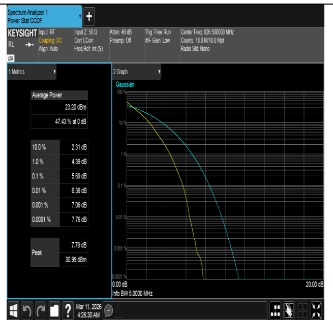
Band5-5MHz-QPSK-20425-25RB#0-PASS
