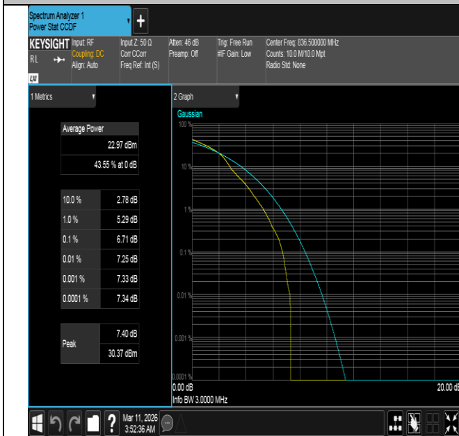
Band5-3MHz-16QAM-20525-1RB#0-PASS
