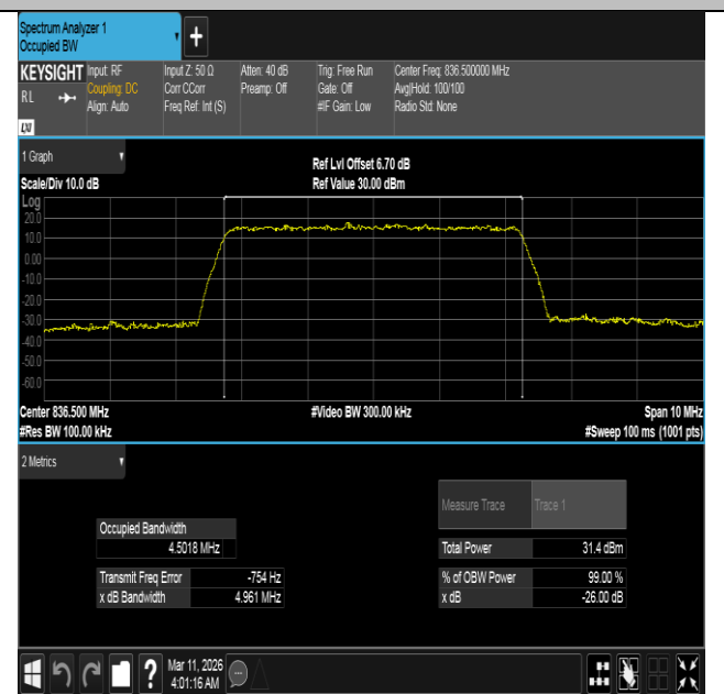
Band5-5MHz-16QAM-20525-25RB#0-PASS
