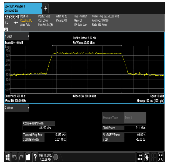
Band5-5MHz-16QAM-20425-25RB#0-PASS
