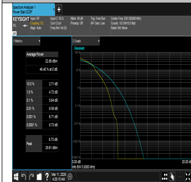
Band5-5MHz-16QAM-20425-1RB#0-PASS
