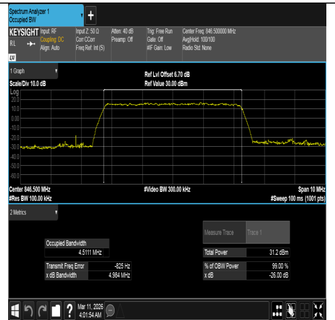
Band5-5MHz-16QAM-20625-25RB#0-PASS
