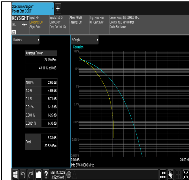
Band5-3MHz-QPSK-20525-1RB#0-PASS
