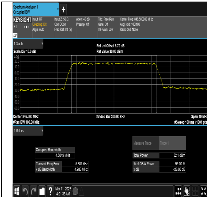
Band5-5MHz-QPSK-20625-25RB#0-PASS
