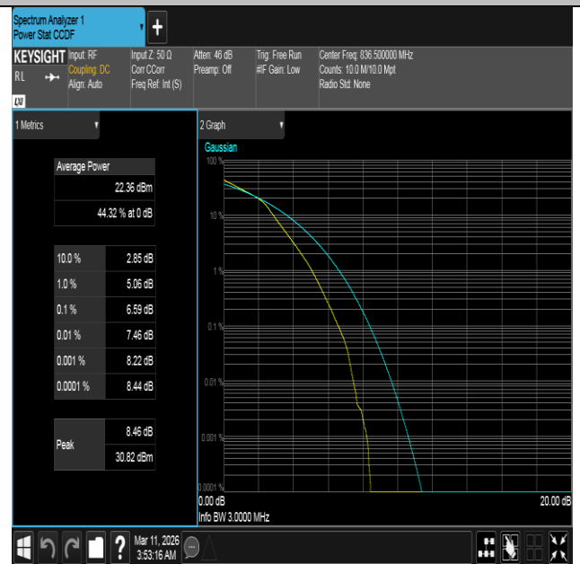
Band5-3MHz-16QAM-20525-15RB#0-PASS
