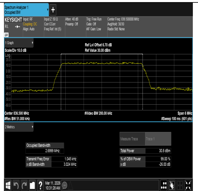
Band5-3MHz-16QAM-20525-15RB#0-PASS
