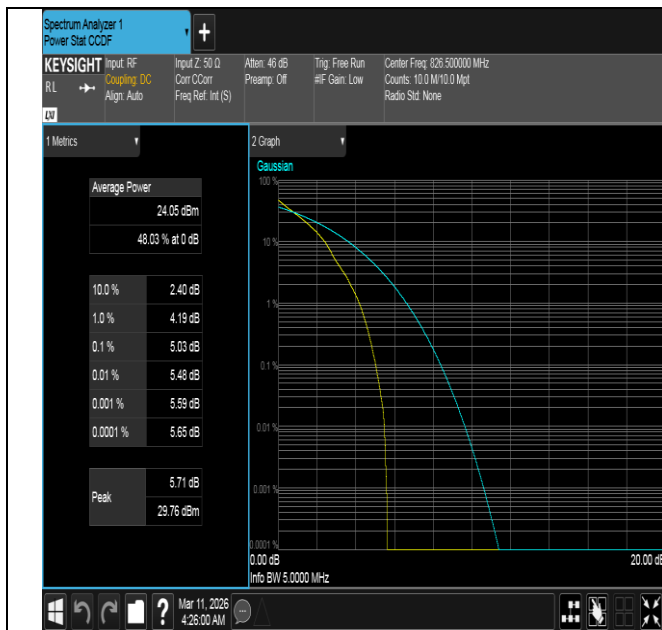
Band5-5MHz-QPSK-20425-1RB#0-PASS
