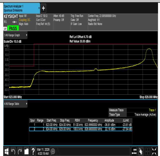
Band5-5MHz-QPSK-20425-1RB#24-PASS
