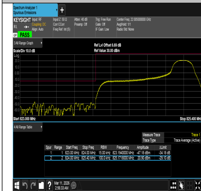
Band5-1.4MHz-16QAM-20407-1RB#5-PASS
