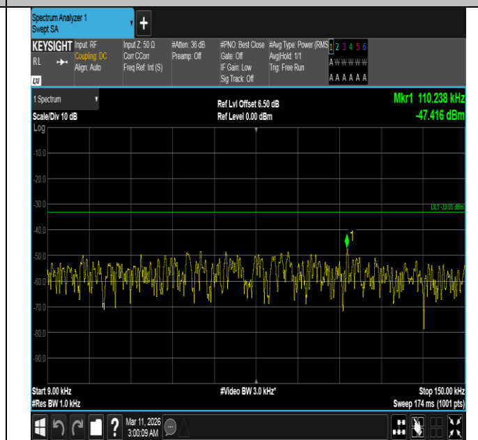
Band5-1.4MHz-QPSK-20407-1RB#5-0.009~0.15-PASS
