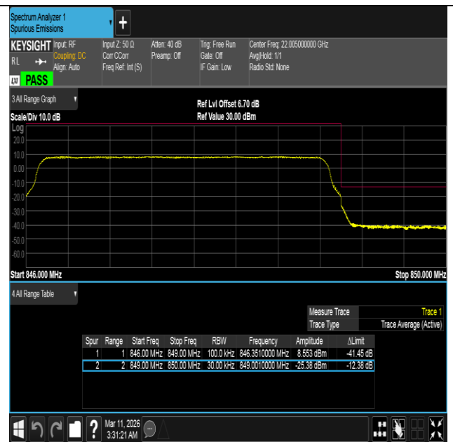
Band5-3MHz-16QAM-20635-15RB#0-PASS
