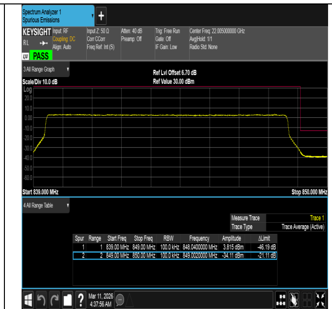
Band5-10MHz-16QAM-20600-50RB#0-PASS
