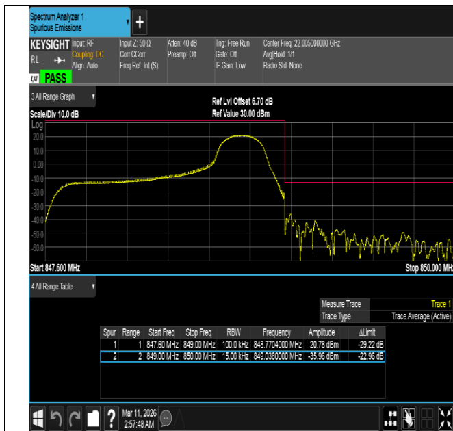
Band5-1.4MHz-16QAM-20643-1RB#5-PASS
