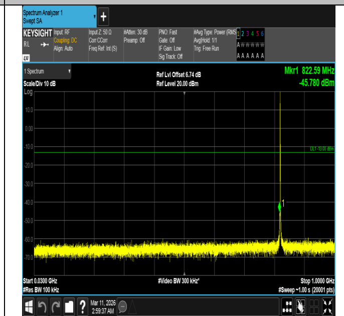
Band5-1.4MHz-16QAM-20407-1RB#0-30~1000-PASS
