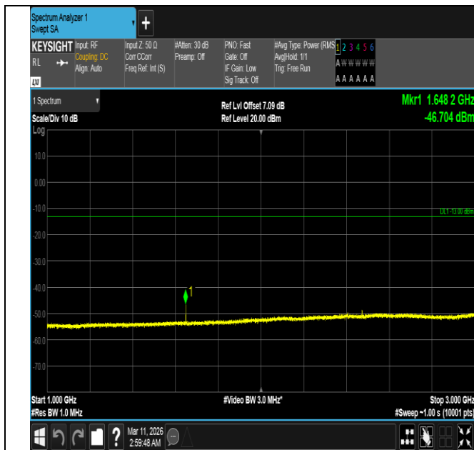
Band5-1.4MHz-16QAM-20407-1RB#0-1000~3000-PASS
