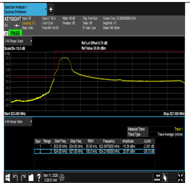
Band5-3MHz-16QAM-20415-1RB#0-PASS
