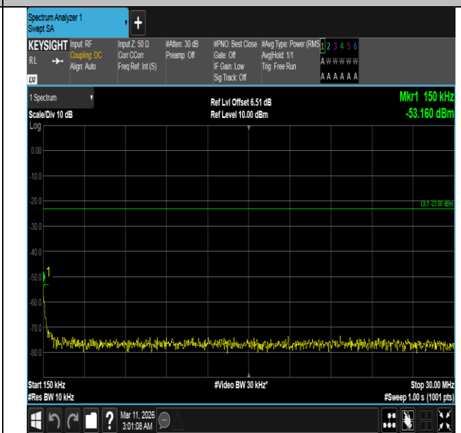
Band5-1.4MHz-16QAM-20407-1RB#5-0.15~30-PASS
