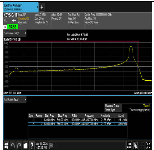
Band5-10MHz-QPSK-20600-1RB#49-PASS
