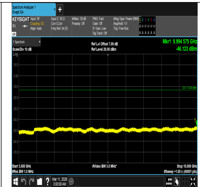
Band5-1.4MHz-16QAM-20407-1RB#0-3000~10000-PASS
