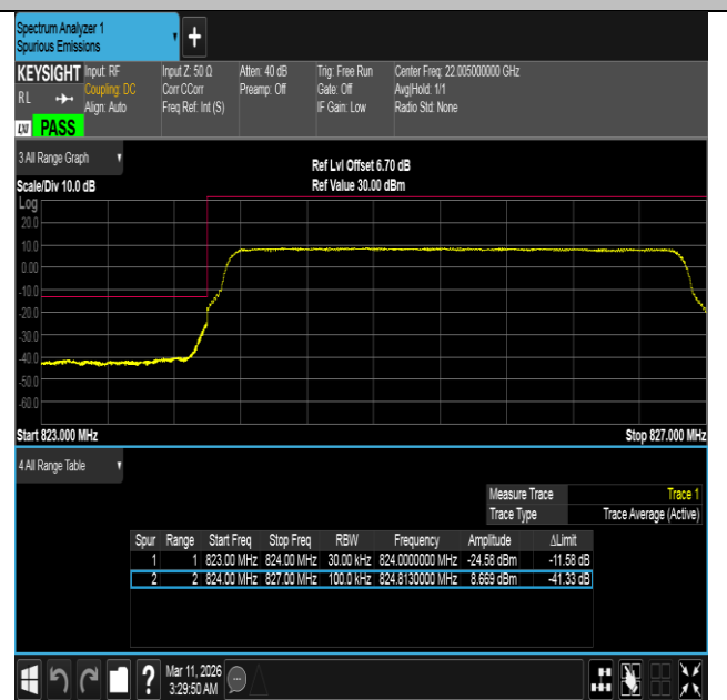
Band5-3MHz-16QAM-20415-15RB#0-PASS
