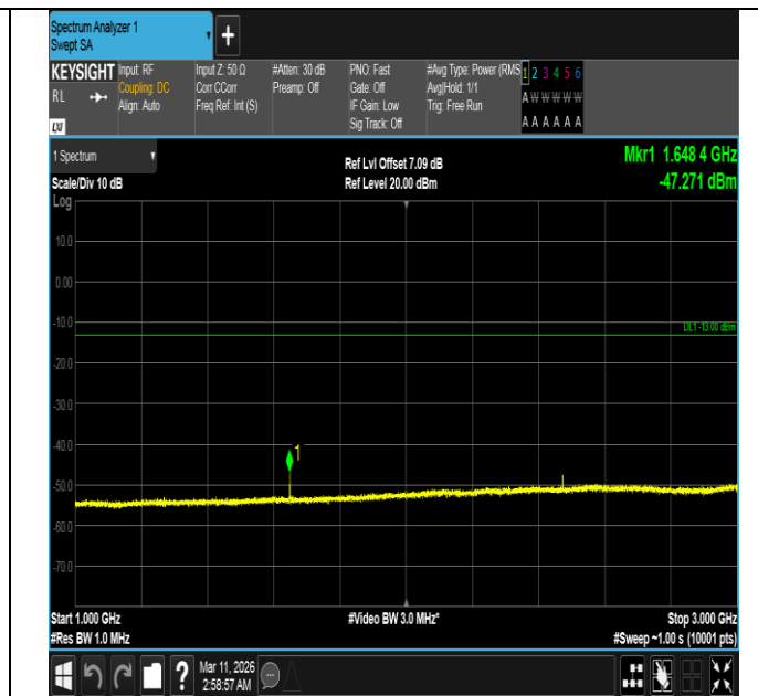
Band5-1.4MHz-QPSK-20407-1RB#0-1000~3000-PASS
