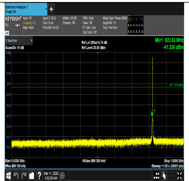
Band5-1.4MHz-16QAM-20407-6RB#0-30~1000-PASS
