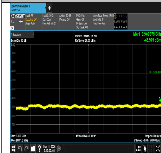
Band5-1.4MHz-16QAM-20643-1RB#5-3000~10000-PASS
