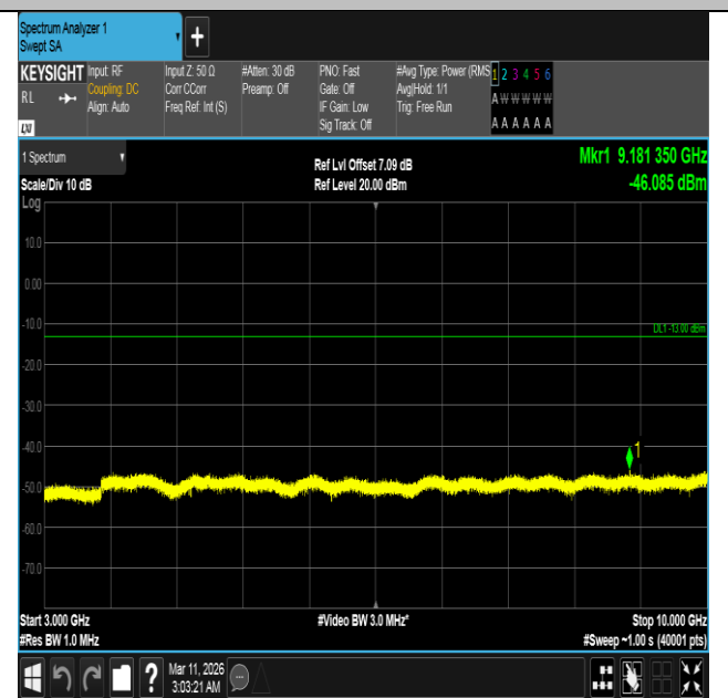
Band5-1.4MHz-16QAM-20407-6RB#0-3000~10000-PASS
