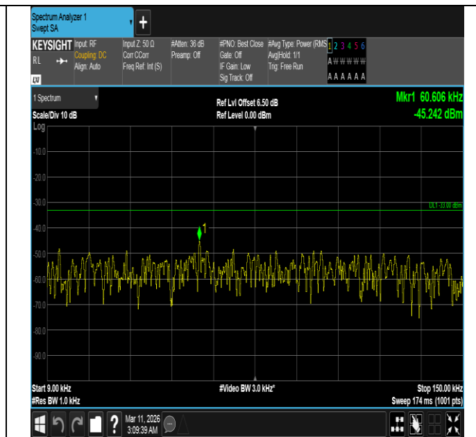
Band5-1.4MHz-16QAM-20643-1RB#0-0.009~0.15-PASS
