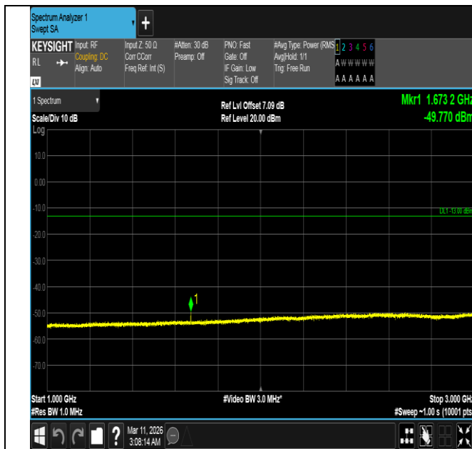
Band5-1.4MHz-16QAM-20525-6RB#0-1000~3000-PASS
