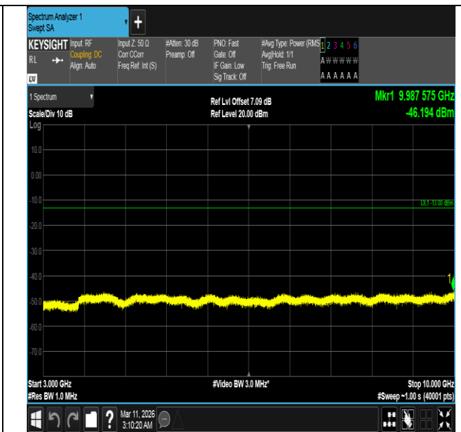
Band5-1.4MHz-16QAM-20643-1RB#0-3000~10000-PASS
