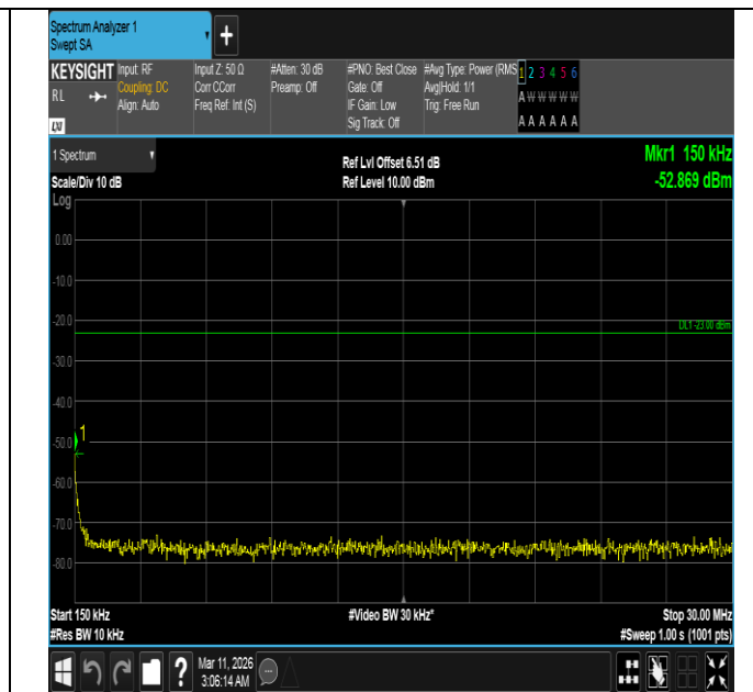
Band5-1.4MHz-16QAM-20525-1RB#5-0.15~30-PASS
