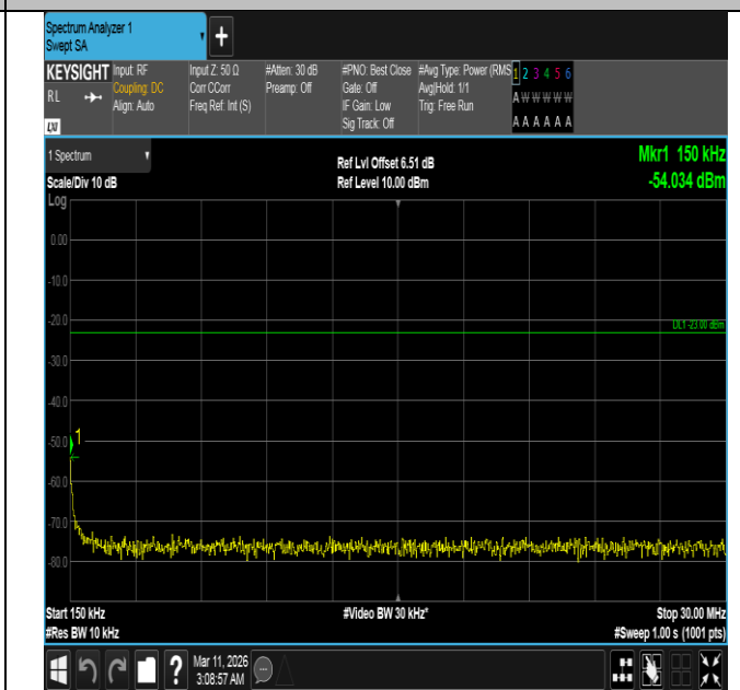
Band5-1.4MHz-QPSK-20643-1RB#0-0.15~30-PASS
