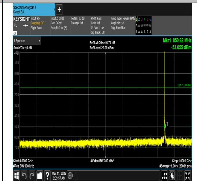
Band5-1.4MHz-16QAM-20643-1RB#0-30~1000-PASS
