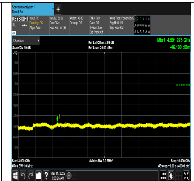
Band5-1.4MHz-16QAM-20525-6RB#0-3000~10000-PASS
