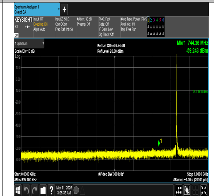
Band5-1.4MHz-QPSK-20525-1RB#5-30~1000-PASS
