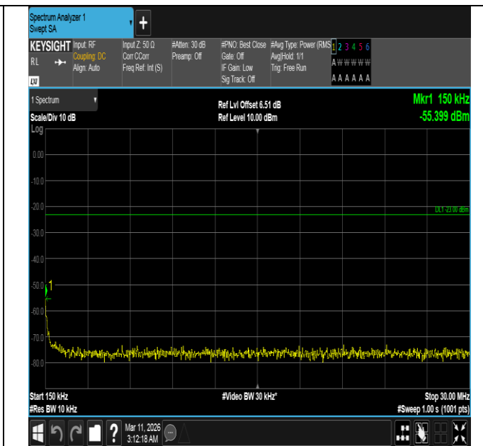
Band5-1.4MHz-QPSK-20643-6RB#0-0.15~30-PASS
