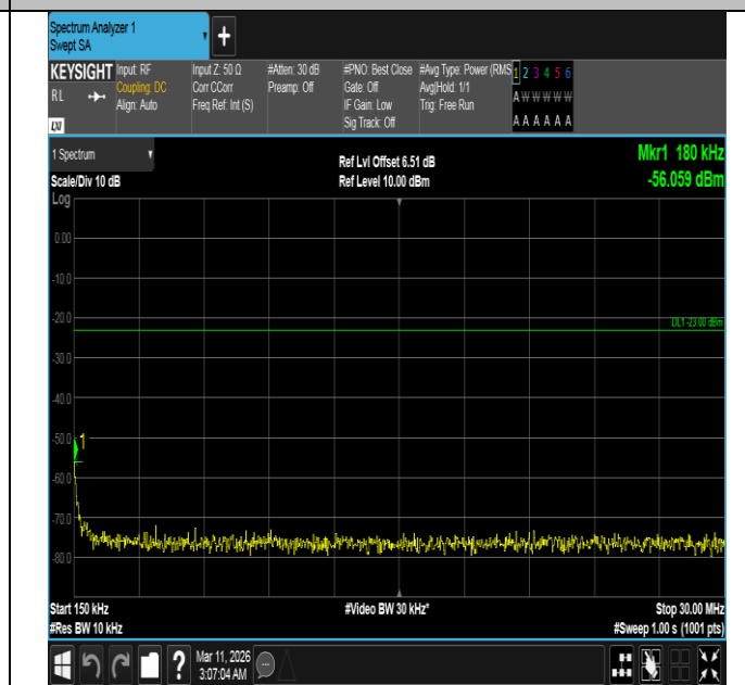
Band5-1.4MHz-QPSK-20525-6RB#0-0.15~30-PASS
