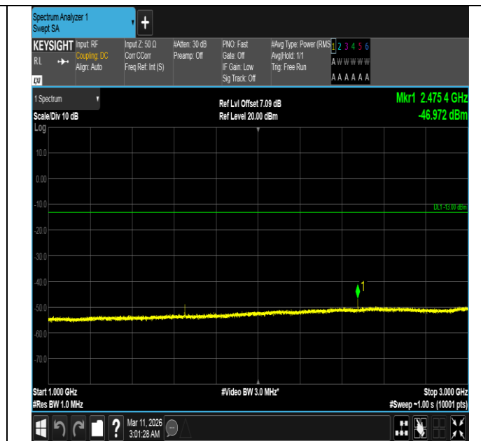
Band5-1.4MHz-16QAM-20407-1RB#5-1000~3000-PASS
