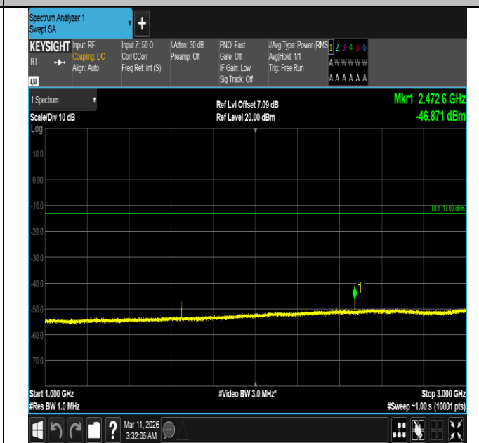
Band5-3MHz-QPSK-20415-1RB#0-1000~3000-PASS
