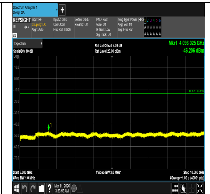
Band5-3MHz-QPSK-20415-1RB#14-3000~10000-PASS
