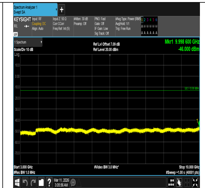
Band5-1.4MHz-QPSK-20525-1RB#5-3000~10000-PASS
