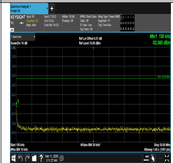
Band5-1.4MHz-16QAM-20643-1RB#5-0.15~30-PASS
