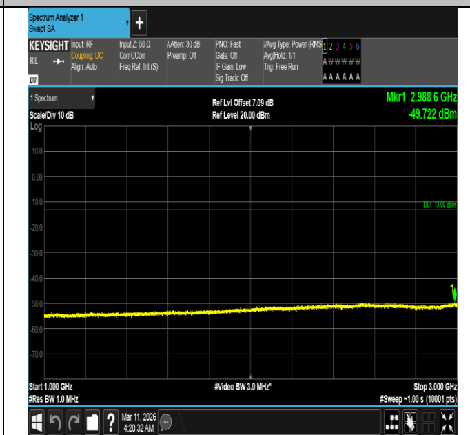
Band5-5MHz-QPSK-20625-25RB#0-1000~3000-PASS
