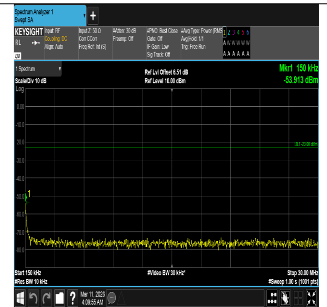
Band5-5MHz-QPSK-20425-25RB#0-0.15~30-PASS
