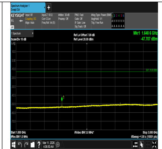
Band5-5MHz-QPSK-20425-1RB#0-1000~3000-PASS
