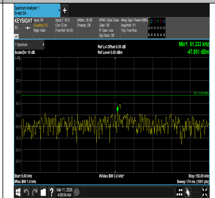
Band5-5MHz-QPSK-20425-1RB#24-0.009~0.15-PASS
