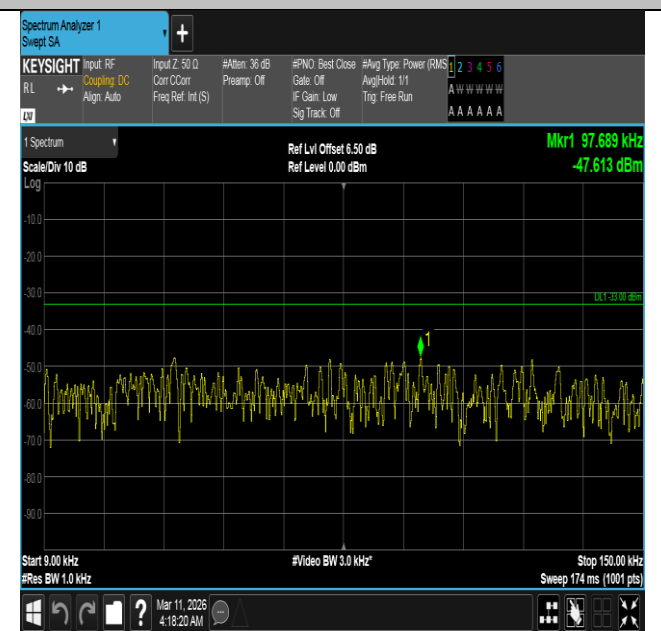
Band5-5MHz-QPSK-20625-1RB#24-0.009~0.15-PASS
