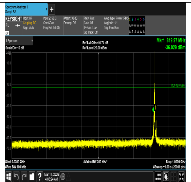
Band5-5MHz-QPSK-20425-1RB#24-30~1000-PASS
