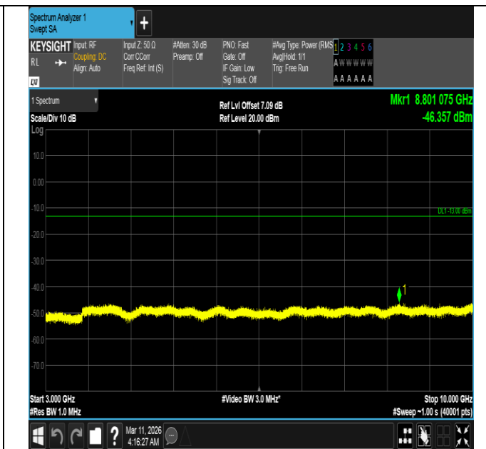
Band5-5MHz-16QAM-20525-25RB#0-3000~10000-PASS
