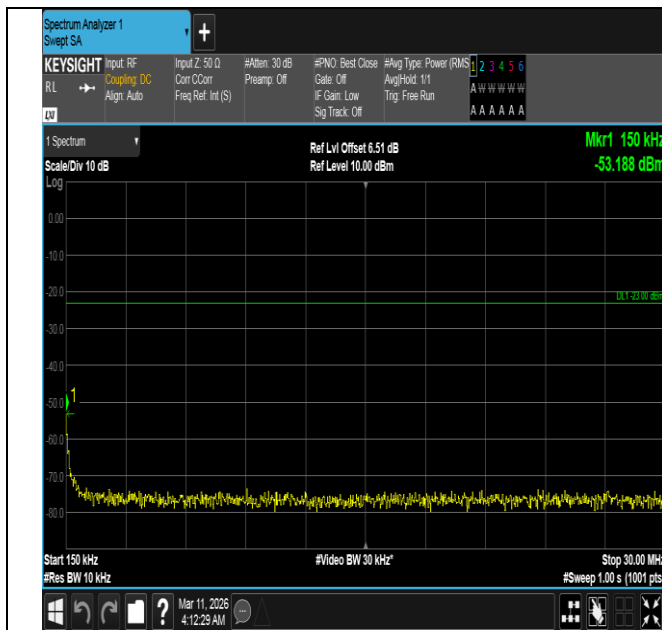
Band5-5MHz-16QAM-20525-1RB#0-0.15~30-PASS
