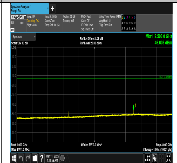
Band5-5MHz-QPSK-20525-1RB#0-1000~3000-PASS
