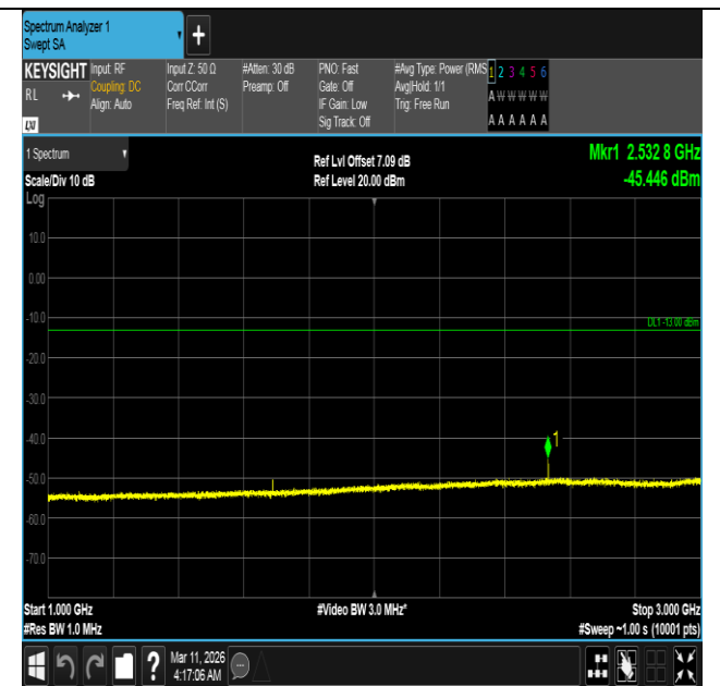
Band5-5MHz-QPSK-20625-1RB#0-1000~3000-PASS
