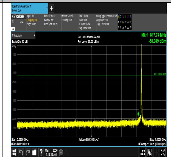
Band5-5MHz-QPSK-20525-1RB#24-30~1000-PASS
