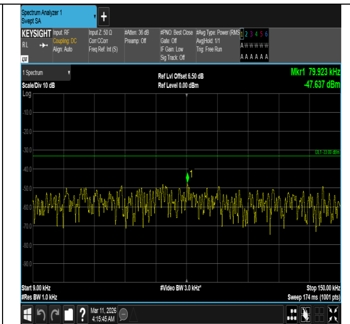
Band5-5MHz-16QAM-20525-25RB#0-0.009~0.15-PASS
