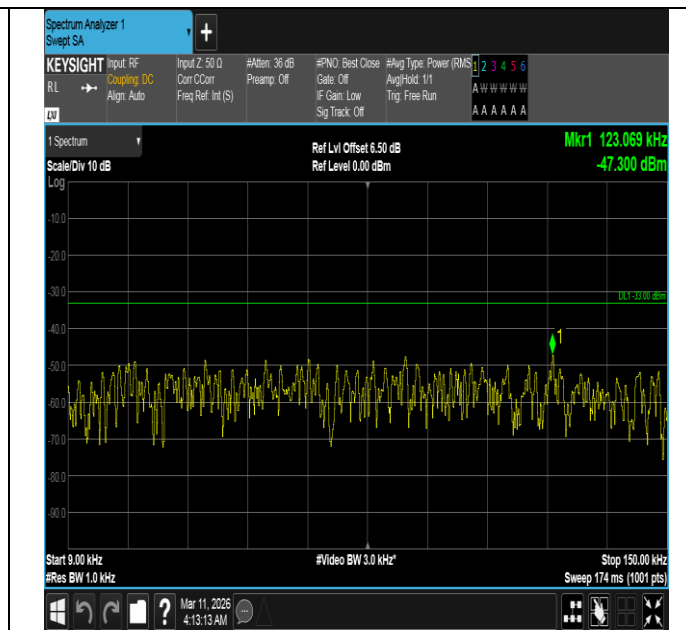
Band5-5MHz-QPSK-20525-1RB#24-0.009~0.15-PASS
