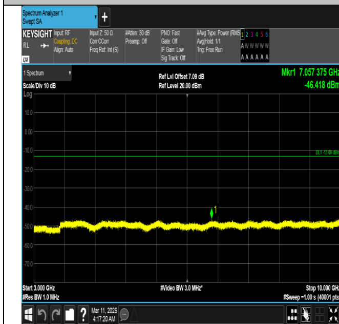
Band5-5MHz-QPSK-20625-1RB#0-3000~10000-PASS
