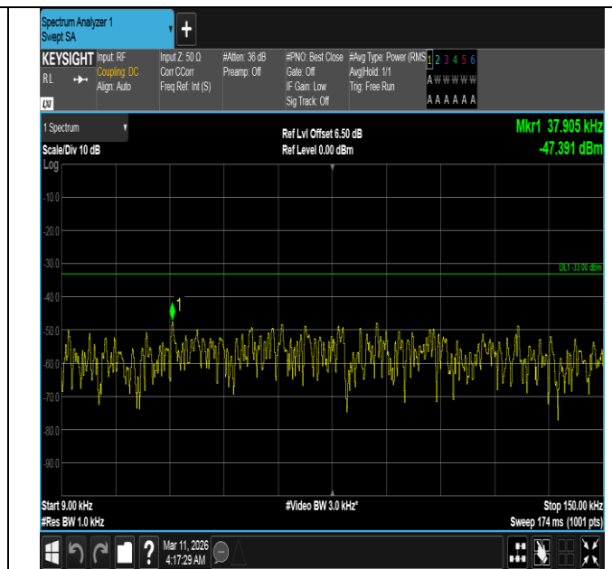
Band5-5MHz-16QAM-20625-1RB#0-0.009~0.15-PASS
