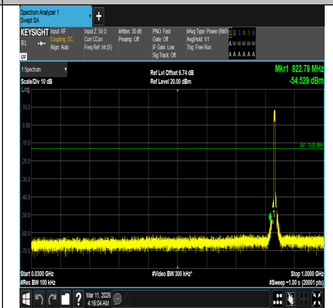
Band5-5MHz-16QAM-20525-25RB#0-30~1000-PASS
