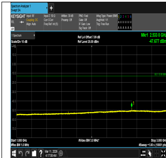
Band5-5MHz-16QAM-20625-1RB#0-1000~3000-PASS
