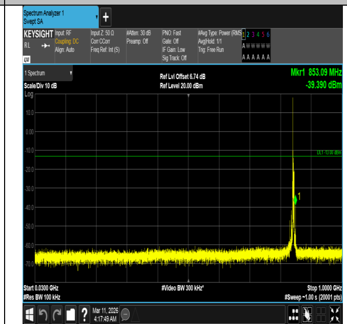
Band5-5MHz-16QAM-20625-1RB#0-30~1000-PASS
