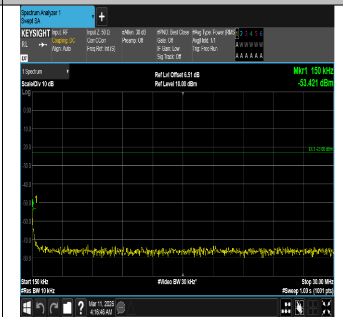
Band5-5MHz-QPSK-20625-1RB#0-0.15~30-PASS
