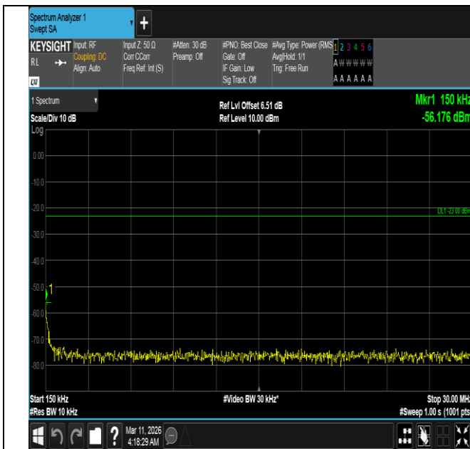
Band5-5MHz-QPSK-20625-1RB#24-0.15~30-PASS
