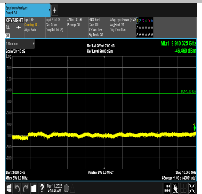
Band5-5MHz-QPSK-20425-1RB#24-3000~10000-PASS
