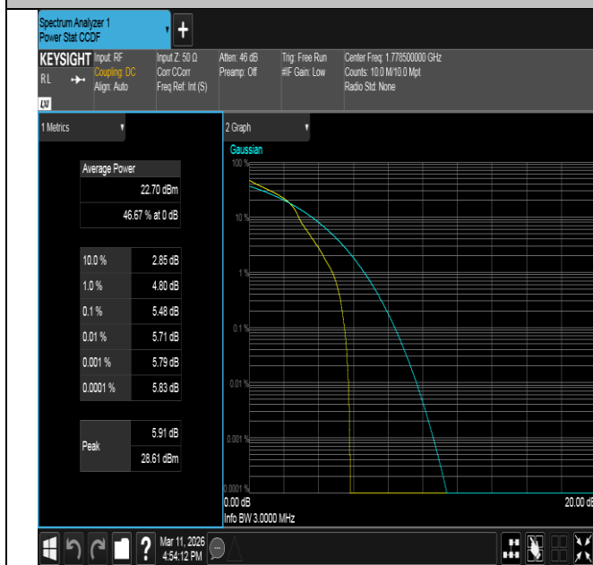
Band66-3MHz-16QAM-132657-1RB#0-PASS
