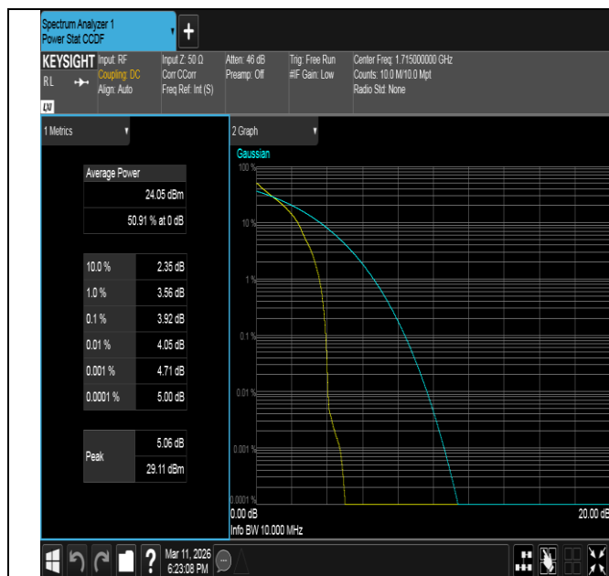
Band66-10MHz-QPSK-132022-1RB#0-PASS
