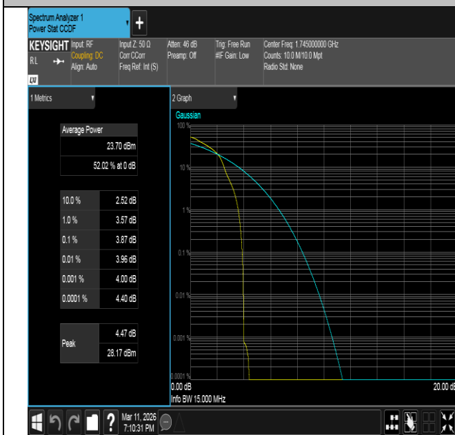
Band66-15MHz-16QAM-132322-1RB#0-PASS
