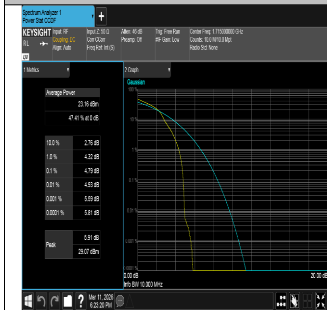
Band66-10MHz-16QAM-132022-1RB#0-PASS
