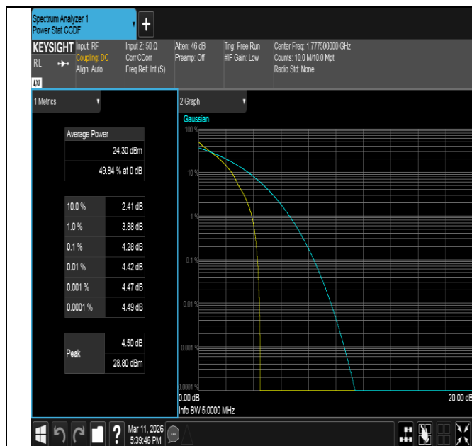
Band66-5MHz-QPSK-132647-1RB#0-PASS
