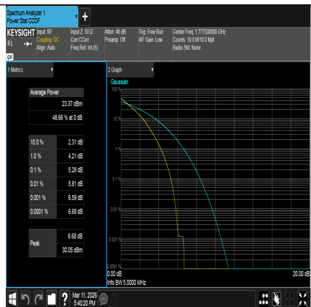
Band66-5MHz-QPSK-132647-25RB#0-PASS
