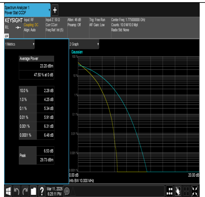
Band66-10MHz-QPSK-132622-50RB#0-PASS
