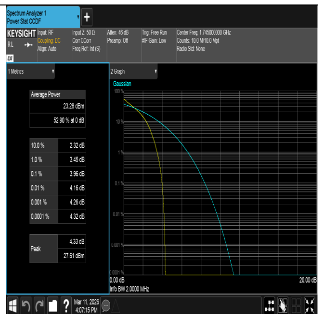
Band66-1.4MHz-QPSK-132322-6RB#0-PASS
