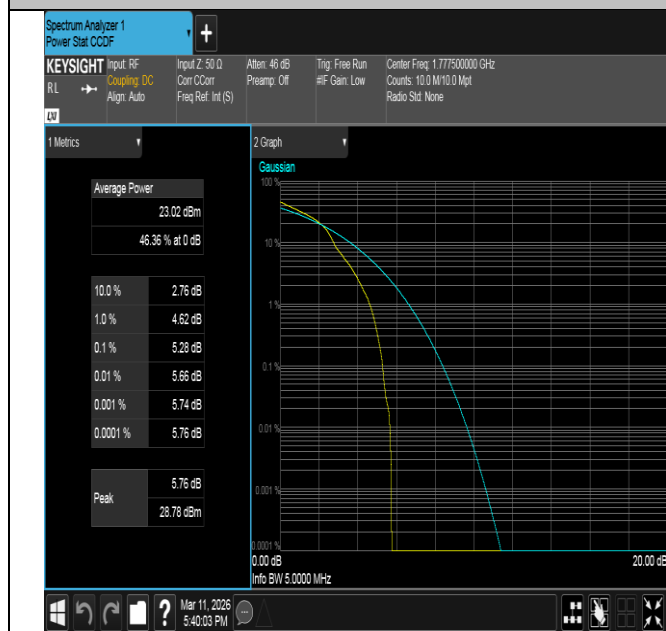
Band66-5MHz-16QAM-132647-1RB#0-PASS
