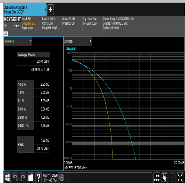
Band66-15MHz-16QAM-132597-75RB#0-PASS
