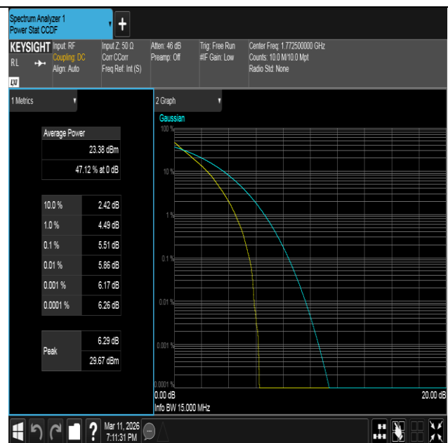
Band66-15MHz-QPSK-132597-75RB#0-PASS
