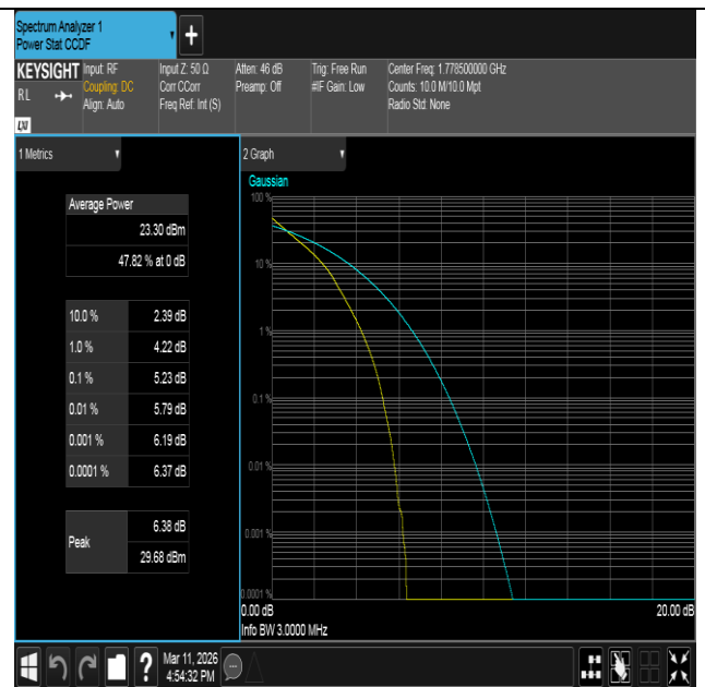
Band66-3MHz-QPSK-132657-15RB#0-PASS
