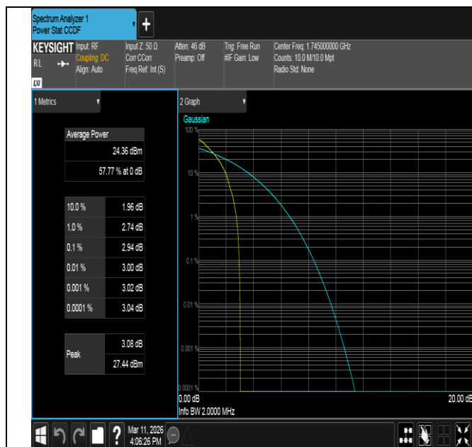
Band66-1.4MHz-QPSK-132322-1RB#0-PASS
