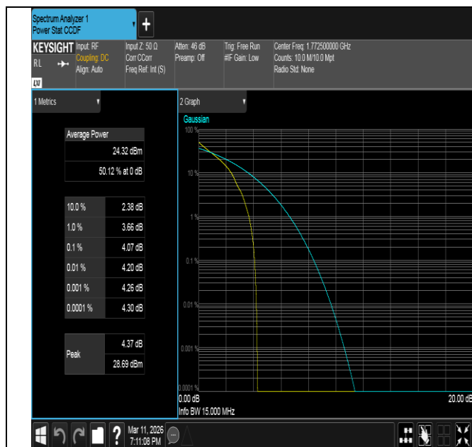
Band66-15MHz-QPSK-132597-1RB#0-PASS
