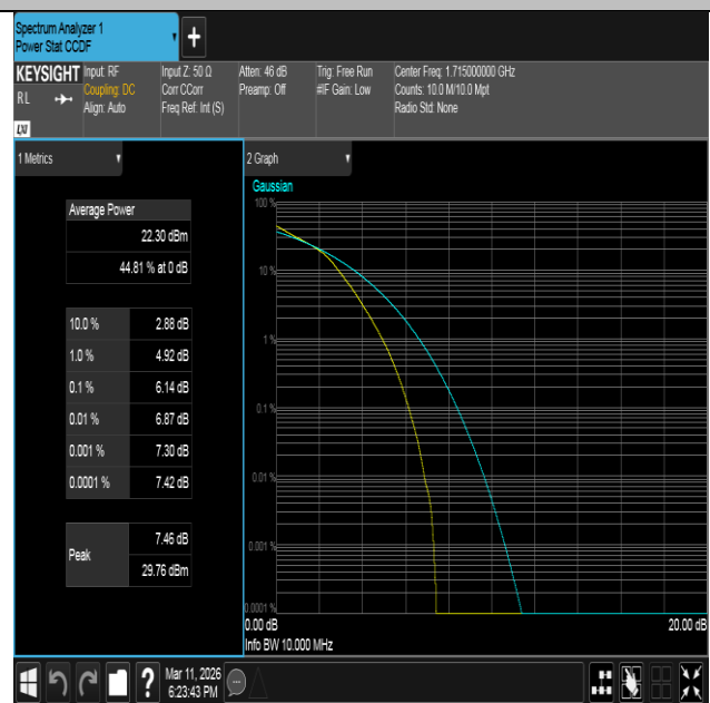
Band66-10MHz-16QAM-132022-50RB#0-PASS
