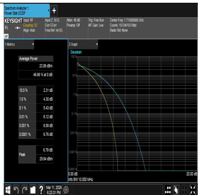
Band66-10MHz-QPSK-132022-50RB#0-PASS
