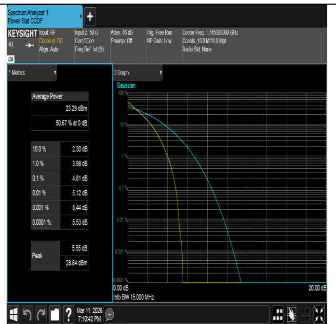
Band66-15MHz-QPSK-132322-75RB#0-PASS
