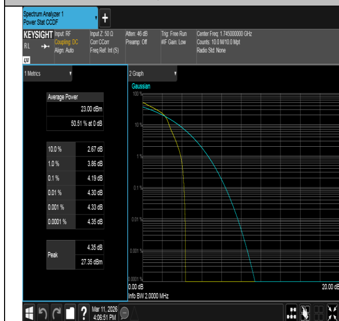
Band66-1.4MHz-16QAM-132322-1RB#0-PASS
