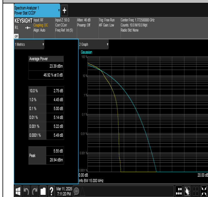
Band66-15MHz-16QAM-132597-1RB#0-PASS
