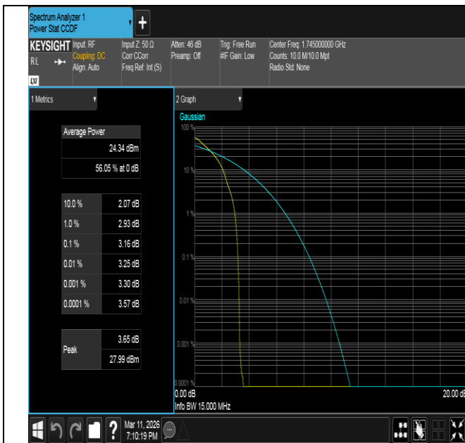
Band66-15MHz-QPSK-132322-1RB#0-PASS
