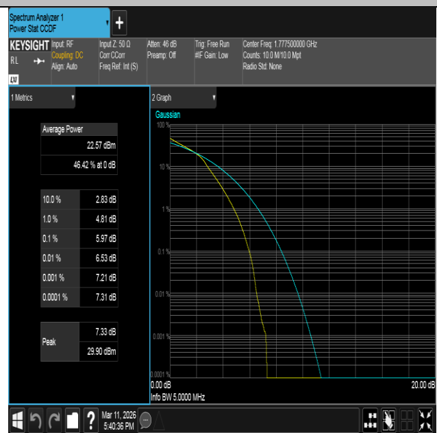
Band66-5MHz-16QAM-132647-25RB#0-PASS
