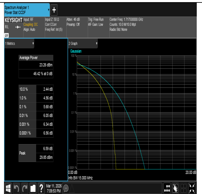
Band66-15MHz-QPSK-132047-75RB#0-PASS
