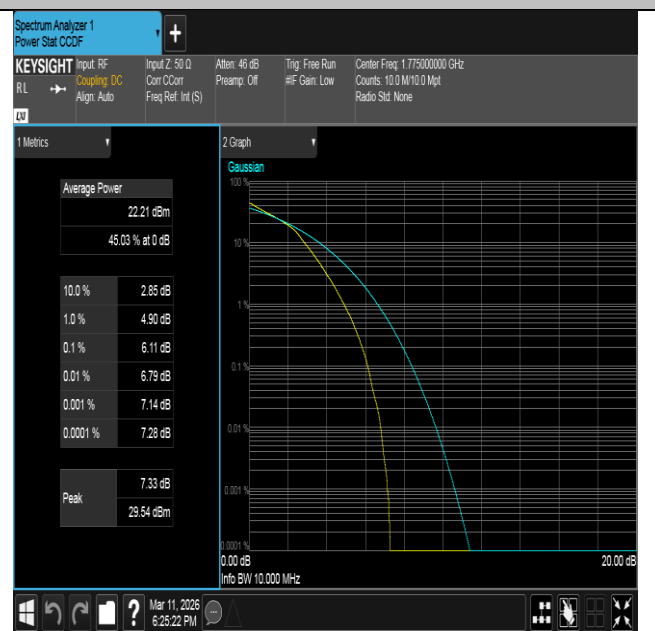
Band66-10MHz-16QAM-132622-50RB#0-PASS
