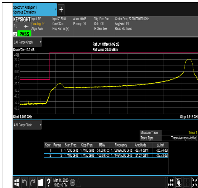
Band66-5MHz-16QAM-131997-1RB#24-PASS
