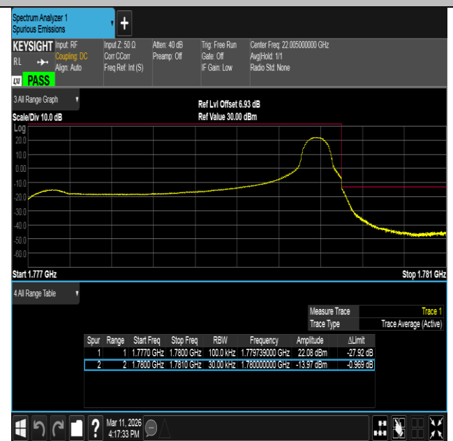
Band66-3MHz-QPSK-132657-1RB#14-PASS
