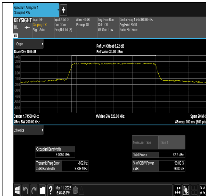
Band66-10MHz-QPSK-132322-50RB#0-PASS
