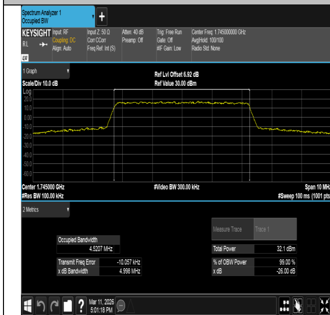
Band66-5MHz-QPSK-132322-25RB#0-PASS
