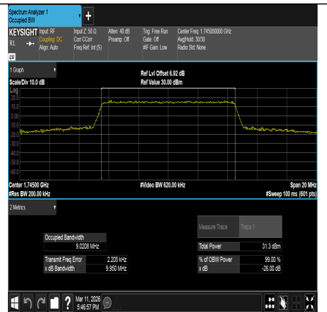
Band66-10MHz-16QAM-132322-50RB#0-PASS
