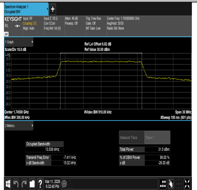
Band66-15MHz-16QAM-132322-75RB#0-PASS
