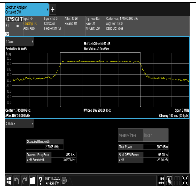
Band66-3MHz-16QAM-132322-15RB#0-PASS
