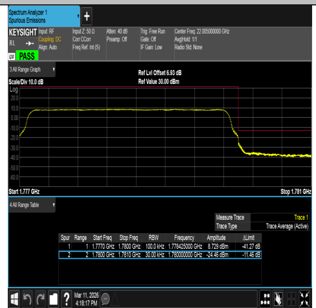
Band66-3MHz-16QAM-132657-15RB#0-PASS
