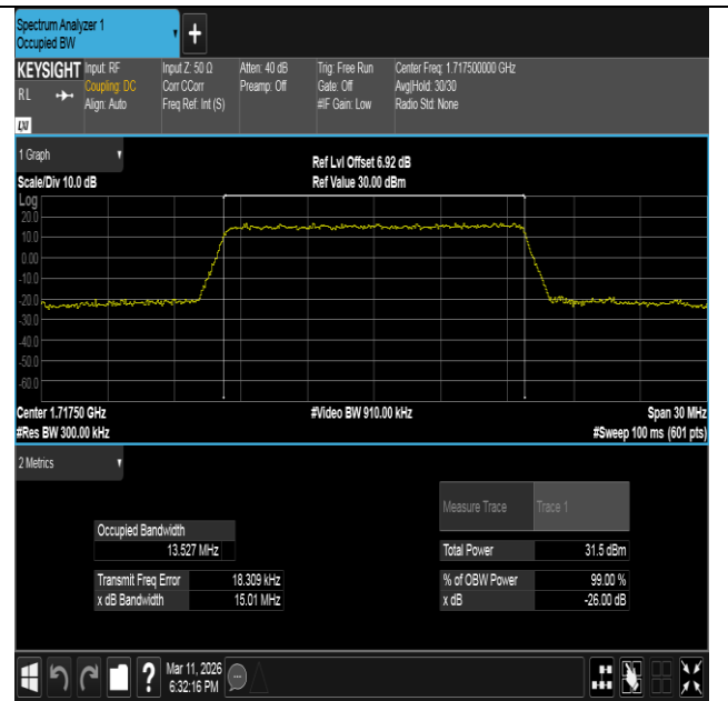
Band66-15MHz-16QAM-132047-75RB#0-PASS
