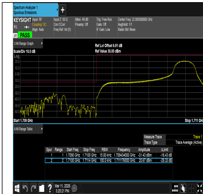
Band66-1.4MHz-16QAM-131979-1RB#5-PASS
