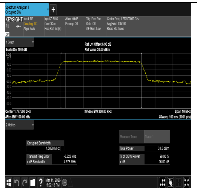
Band66-5MHz-16QAM-132647-25RB#0-PASS
