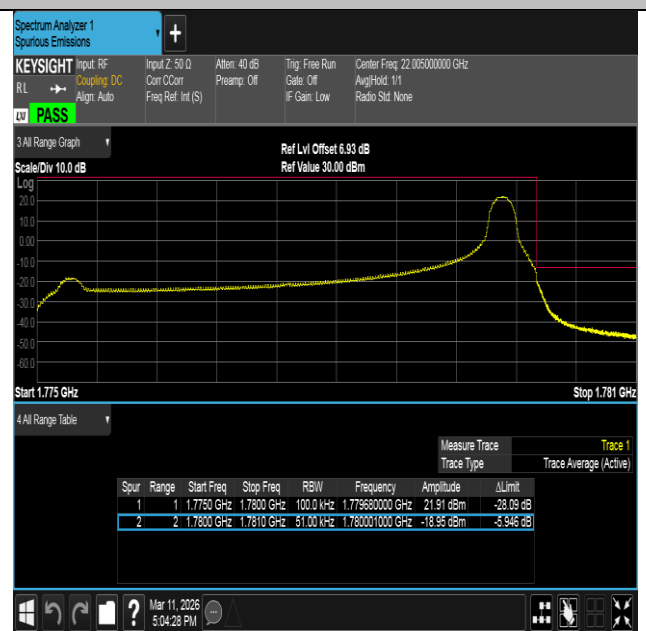
Band66-5MHz-QPSK-132647-1RB#24-PASS
