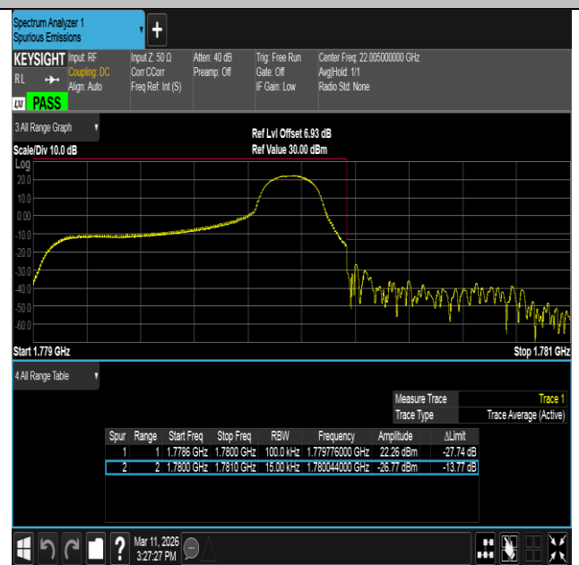
Band66-1.4MHz-QPSK-132665-1RB#5-PASS
