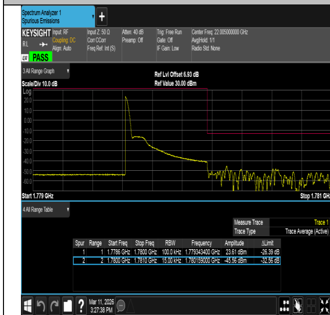
Band66-1.4MHz-16QAM-132665-1RB#5-PASS
