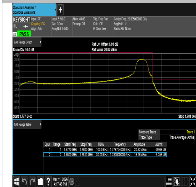
Band66-3MHz-16QAM-132657-1RB#14-PASS
