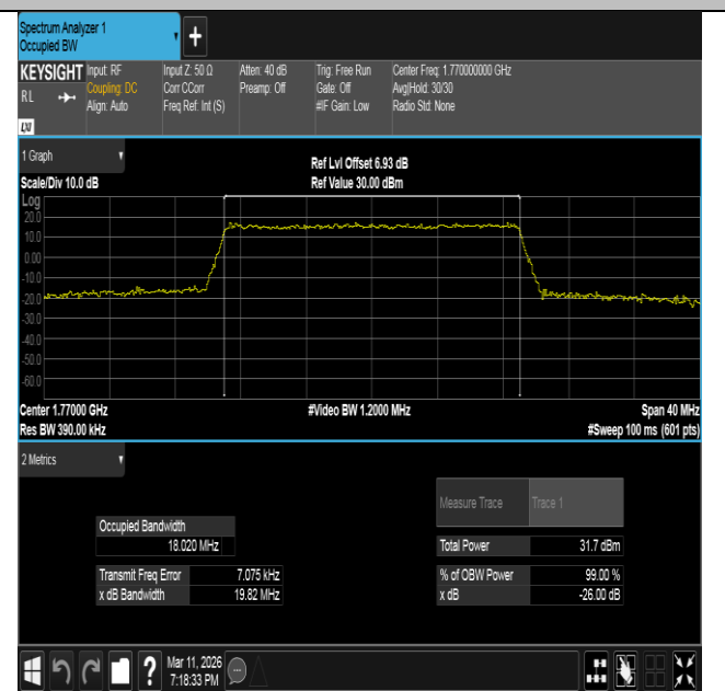
Band66-20MHz-16QAM-132572-100RB#0-PASS
