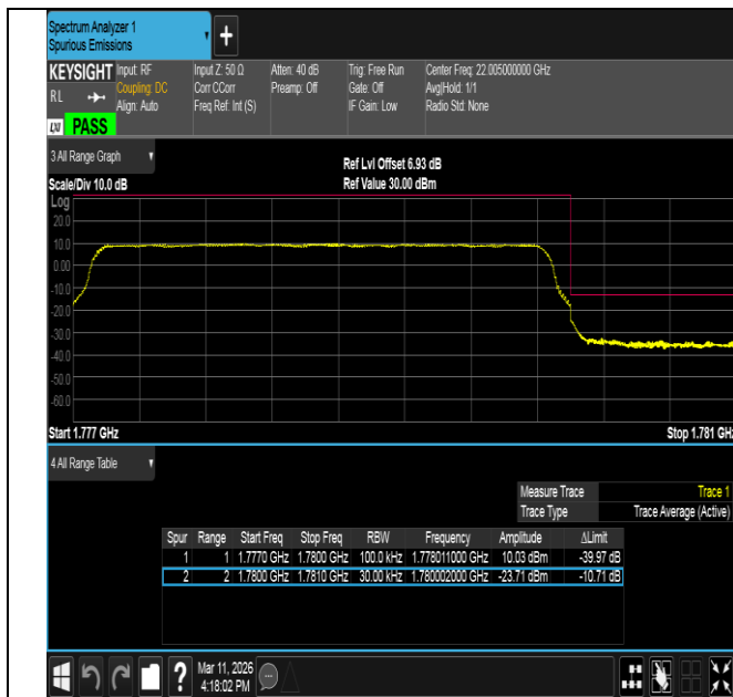
Band66-3MHz-QPSK-132657-15RB#0-PASS
