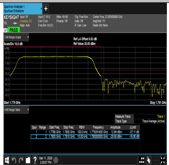
Band66-1.4MHz-16QAM-132665-6RB#0-PASS
