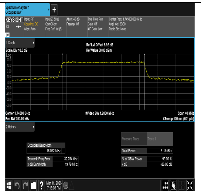
Band66-20MHz-16QAM-132322-100RB#0-PASS
