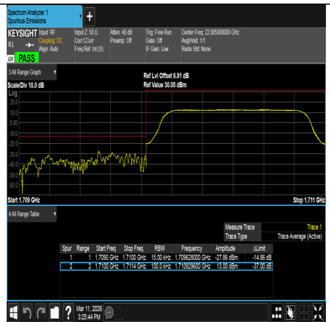
Band66-1.4MHz-16QAM-131979-6RB#0-PASS
