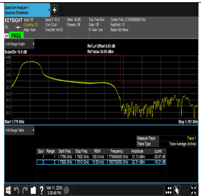
Band66-1.4MHz-16QAM-132665-1RB#0-PASS
