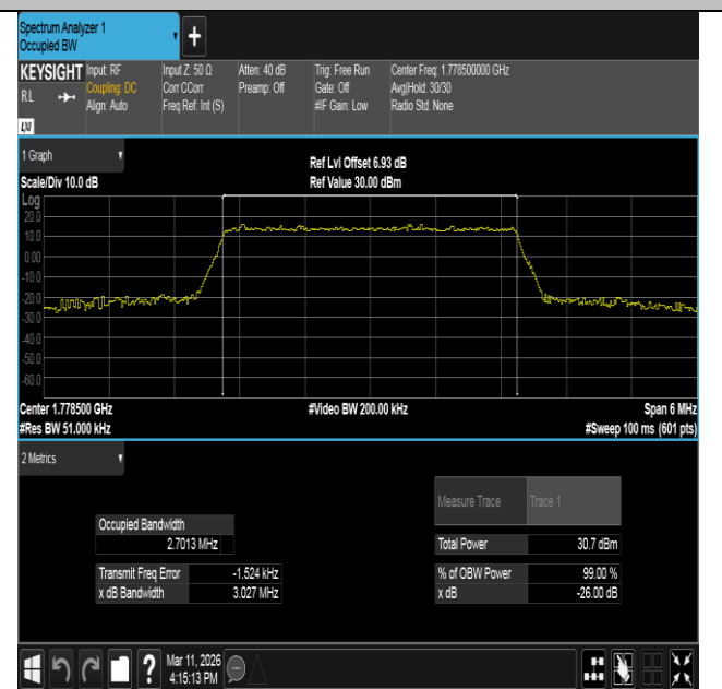
Band66-3MHz-16QAM-132657-15RB#0-PASS
