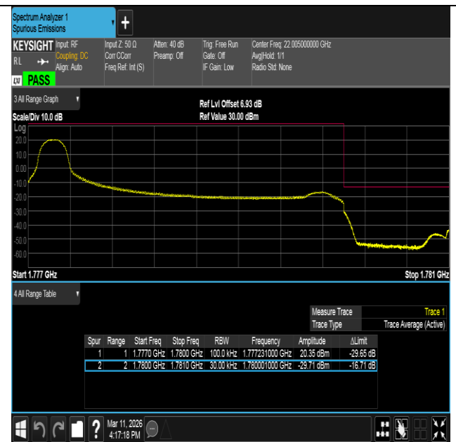
Band66-3MHz-16QAM-132657-1RB#0-PASS
