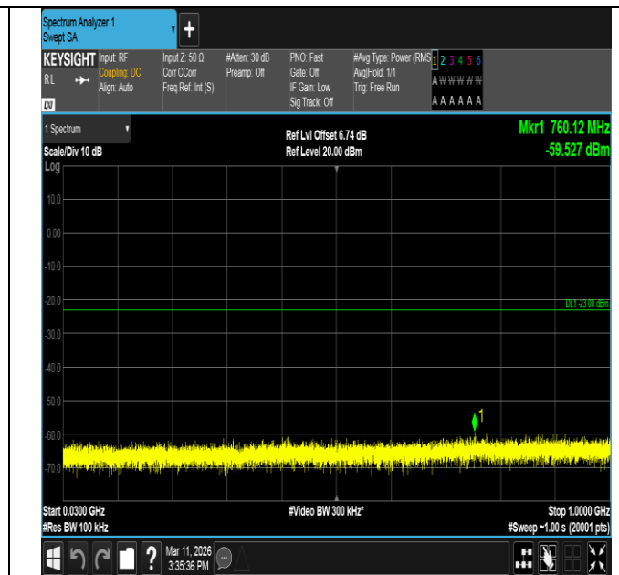
Band66-1.4MHz-QPSK-132322-1RB#5-30~1000-PASS
