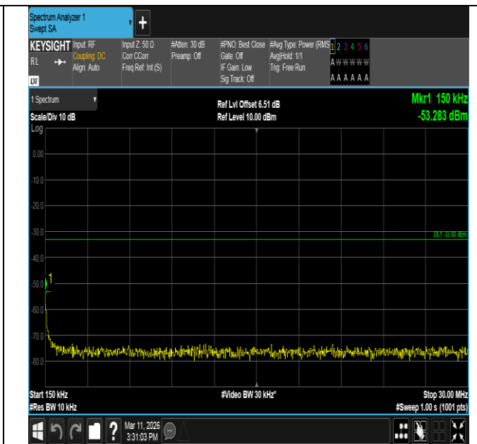
Band66-1.4MHz-16QAM-131979-1RB#5-0.15~30-PASS
