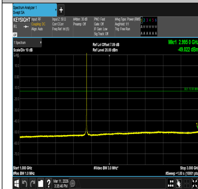
Band66-1.4MHz-QPSK-132322-1RB#5-1000~3000-PASS
