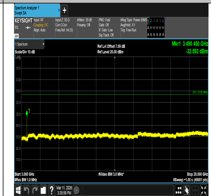
Band66-1.4MHz-QPSK-132322-1RB#5-3000~20000-PASS
