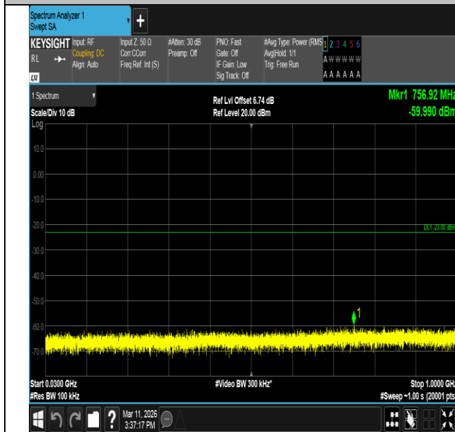
Band66-1.4MHz-QPSK-132322-6RB#0-30~1000-PASS
