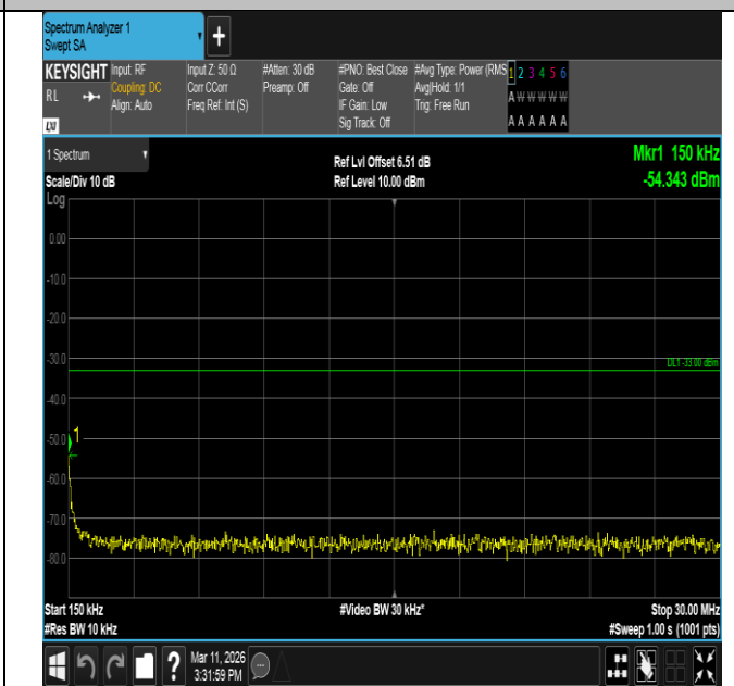
Band66-1.4MHz-QPSK-131979-6RB#0-0.15~30-PASS
