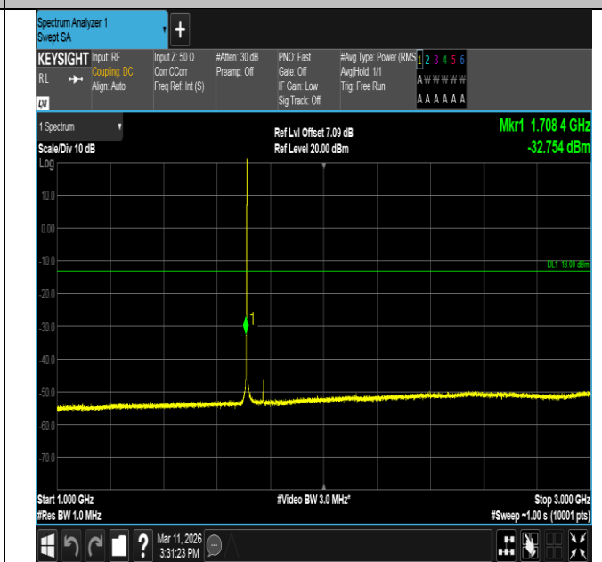
Band66-1.4MHz-16QAM-131979-1RB#5-1000~3000-PASS
