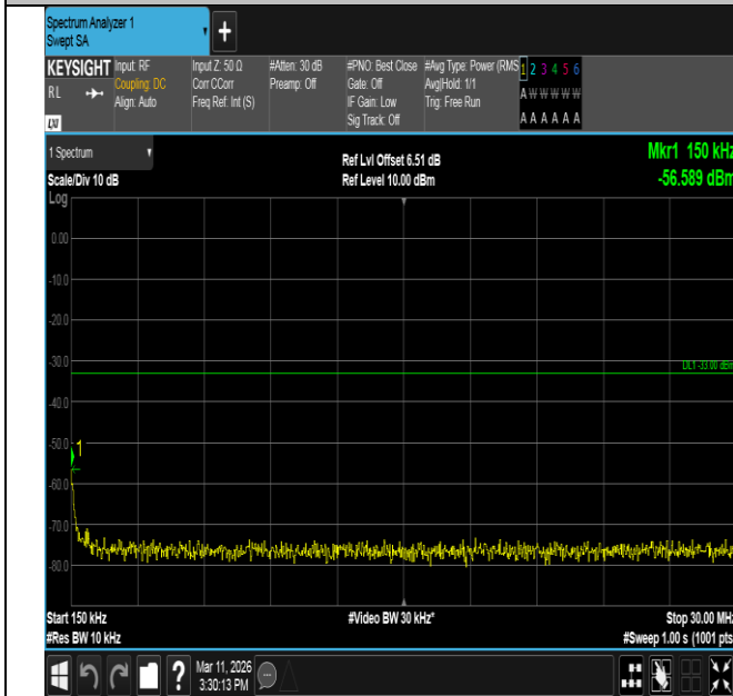
Band66-1.4MHz-QPSK-131979-1RB#5-0.15~30-PASS
