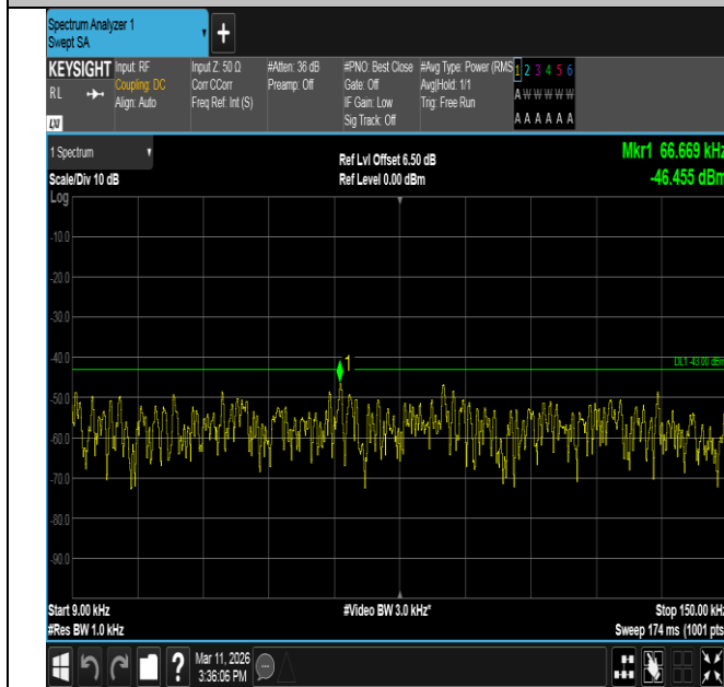
Band66-1.4MHz-16QAM-132322-1RB#5-0.009~0.15-PASS
