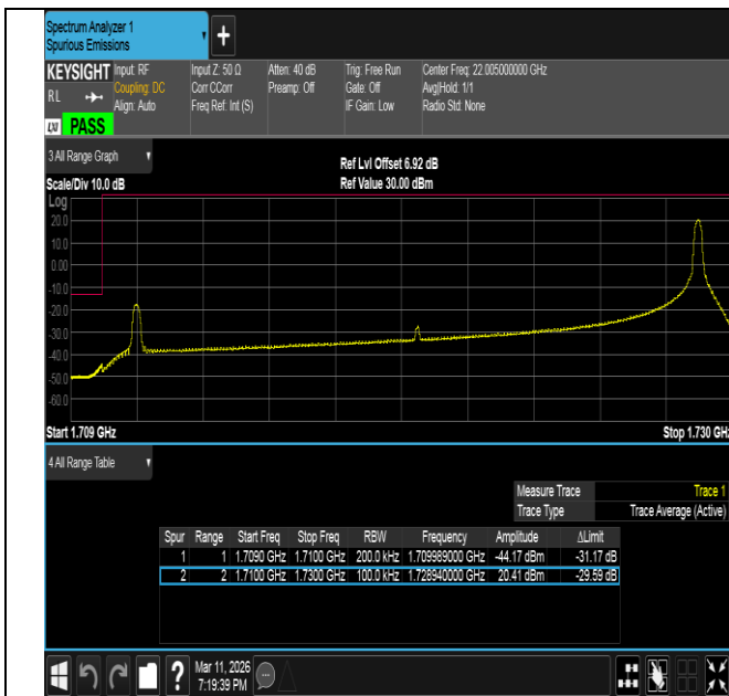
Band66-20MHz-16QAM-132072-1RB#99-PASS
