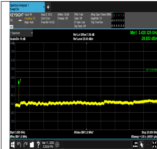
Band66-1.4MHz-QPSK-131979-1RB#0-3000~20000-PASS
