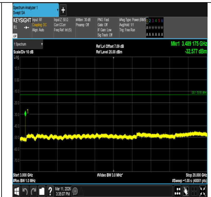
Band66-1.4MHz-16QAM-132322-1RB#0-3000~20000-PASS
