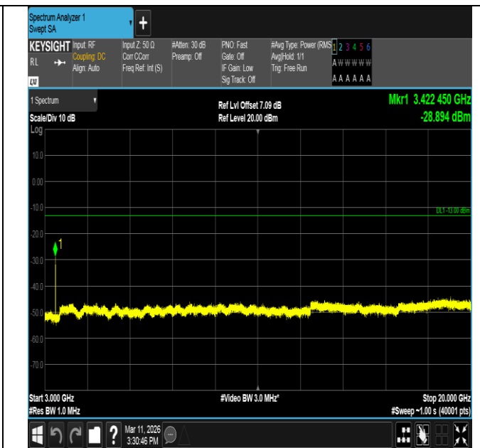
Band66-1.4MHz-QPSK-131979-1RB#5-3000~20000-PASS
