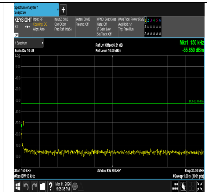
Band66-5MHz-QPSK-131997-1RB#0-0.15~30-PASS
