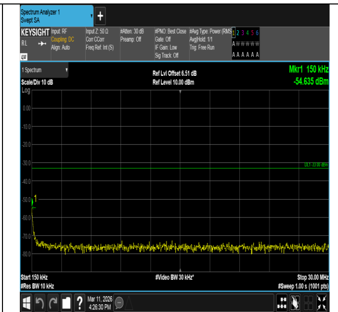
Band66-3MHz-16QAM-132322-1RB#14-0.15~30-PASS
