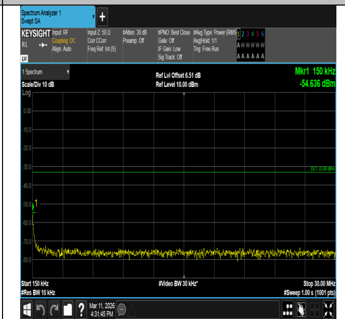
Band66-3MHz-16QAM-132657-1RB#14-0.15~30-PASS
