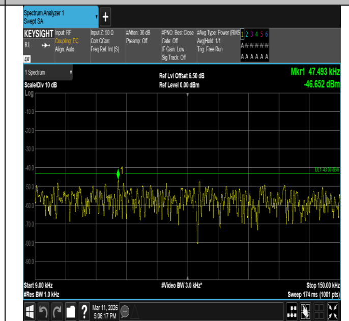
Band66-5MHz-16QAM-131997-1RB#0-0.009~0.15-PASS
