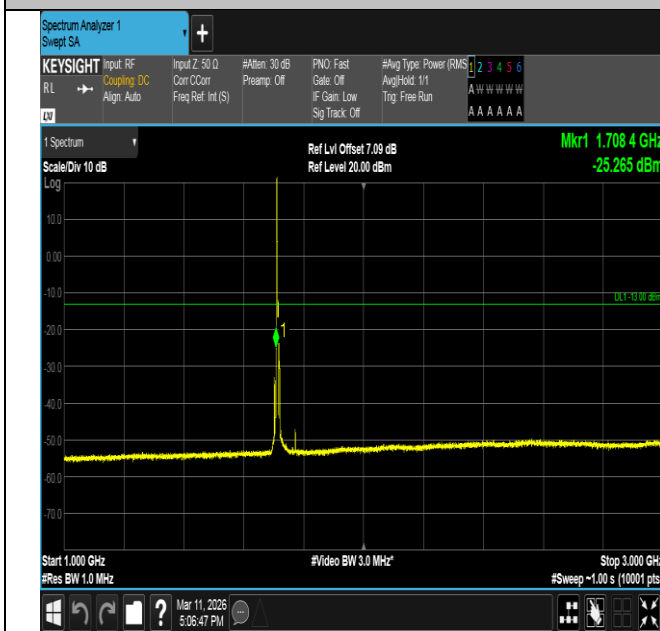
Band66-5MHz-16QAM-131997-1RB#0-1000~3000-PASS
