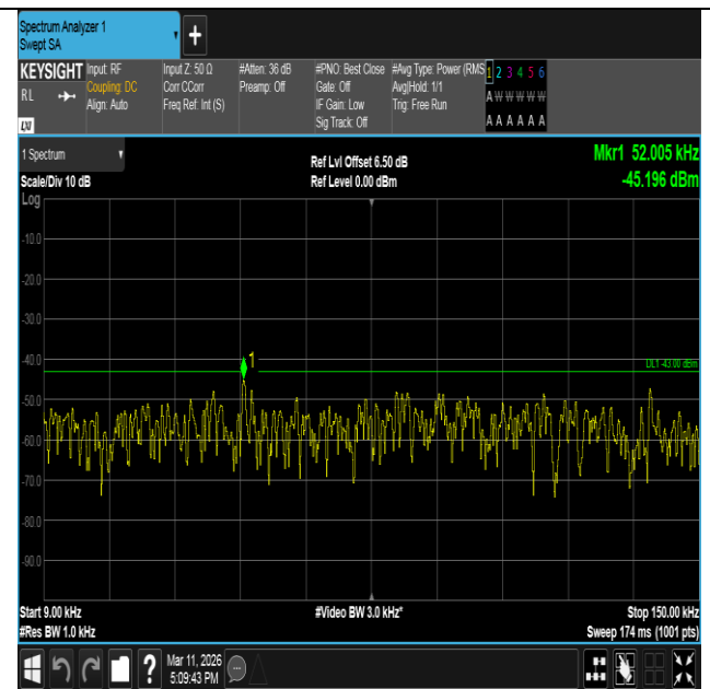
Band66-5MHz-16QAM-131997-25RB#0-0.009~0.15-PASS
