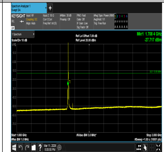
Band66-5MHz-QPSK-131997-1RB#0-1000~3000-PASS
