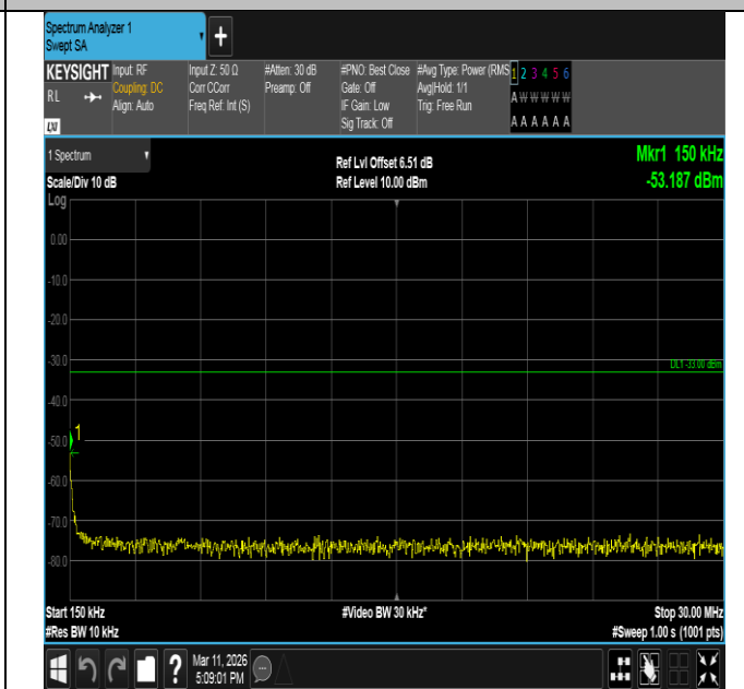
Band66-5MHz-QPSK-131997-25RB#0-0.15~30-PASS
