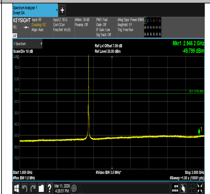
Band66-3MHz-16QAM-132322-1RB#14-1000~3000-PASS
