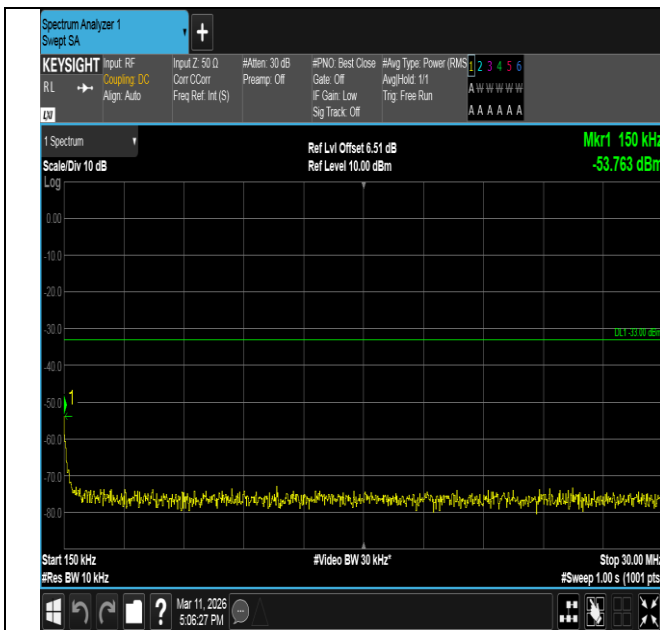
Band66-5MHz-16QAM-131997-1RB#0-0.15~30-PASS
