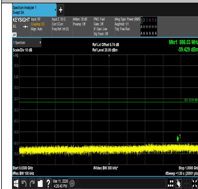
Band66-3MHz-16QAM-132322-1RB#14-30~1000-PASS
