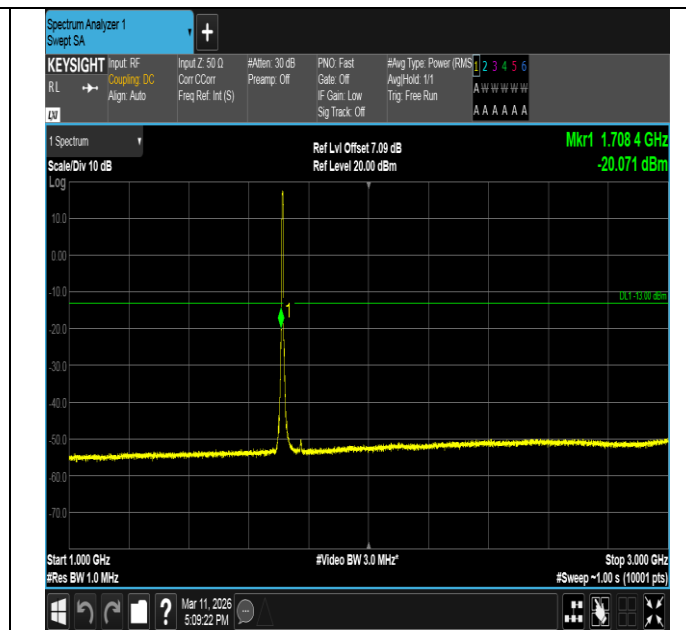
Band66-5MHz-QPSK-131997-25RB#0-1000~3000-PASS
