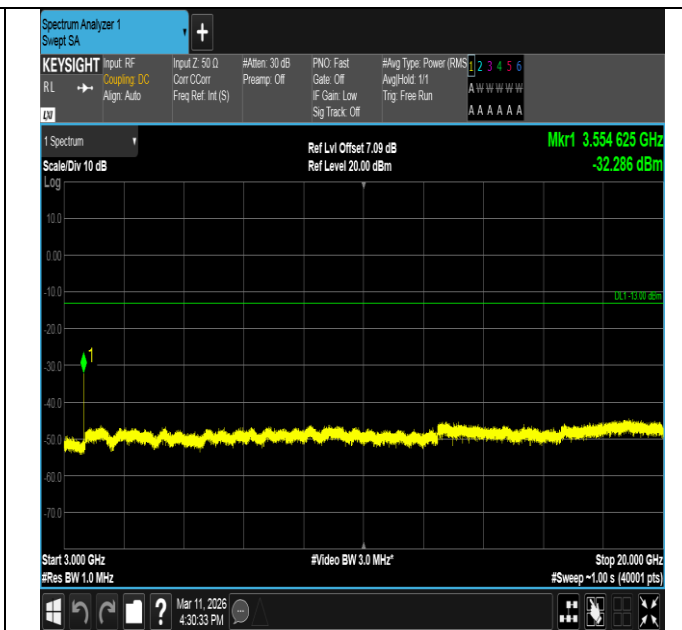
Band66-3MHz-16QAM-132657-1RB#0-3000~20000-PASS
