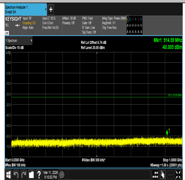
Band66-5MHz-16QAM-131997-25RB#0-30~1000-PASS
