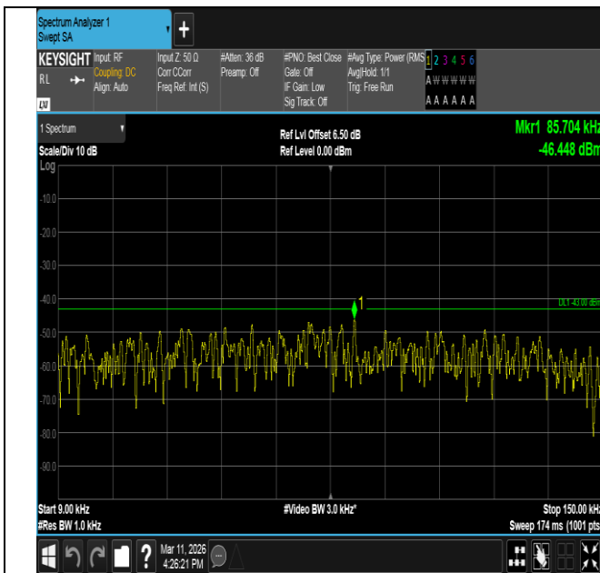
Band66-3MHz-16QAM-132322-1RB#14-0.009~0.15-PASS
