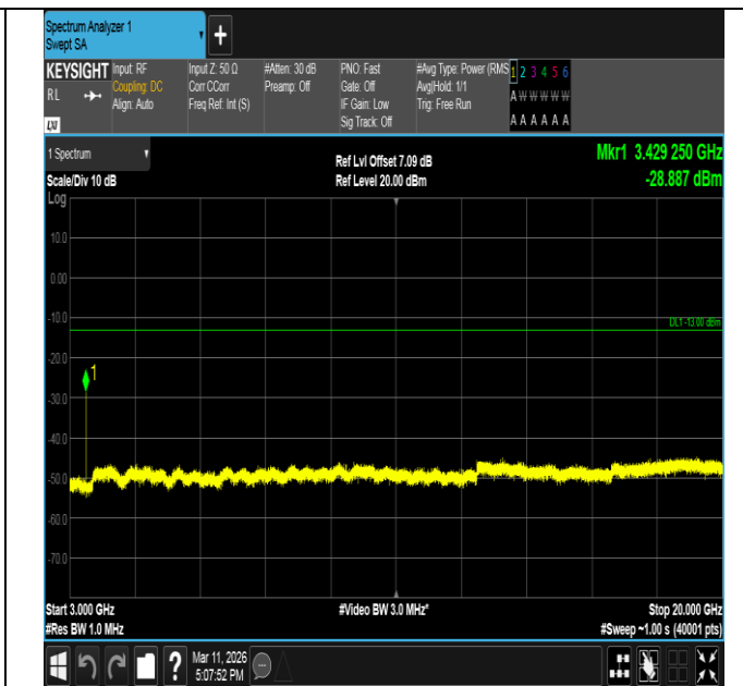
Band66-5MHz-QPSK-131997-1RB#24-3000~20000-PASS
