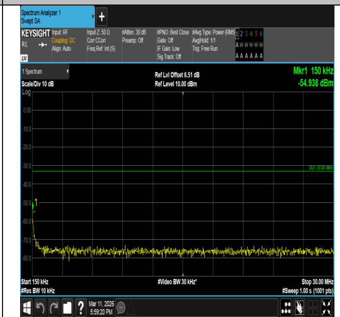
Band66-10MHz-QPSK-132322-50RB#0-0.15~30-PASS
