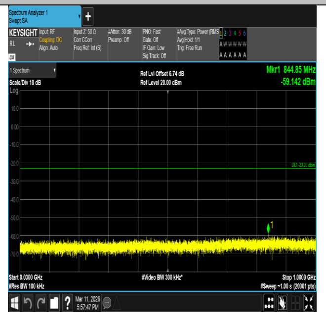
Band66-10MHz-QPSK-132322-1RB#49-30~1000-PASS
