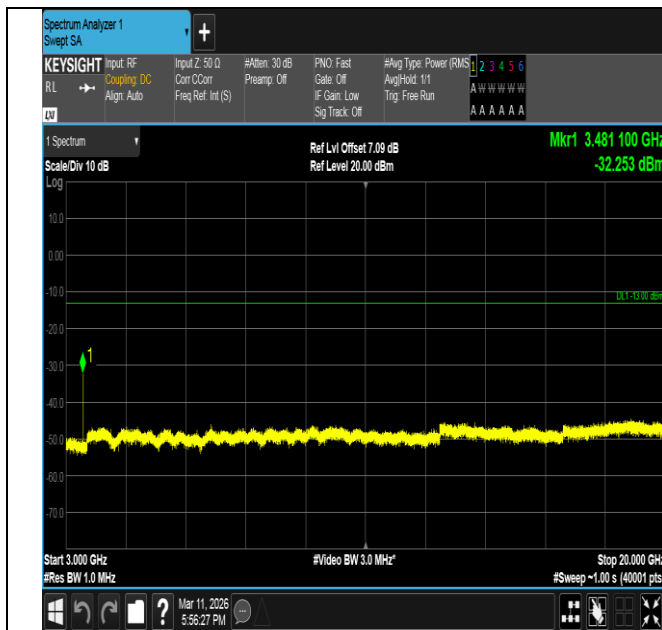
Band66-10MHz-QPSK-132322-1RB#0-3000~20000-PASS
