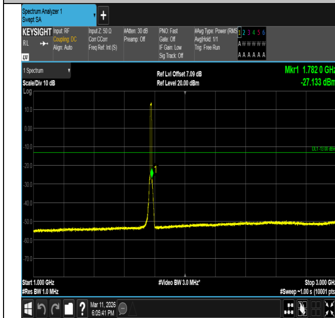
Band66-10MHz-16QAM-132622-50RB#0-1000~3000-PASS
