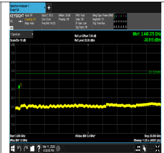
Band66-15MHz-QPSK-132047-1RB#74-3000~20000-PASS
