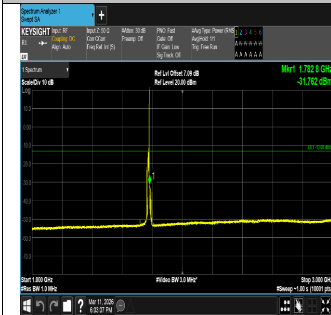
Band66-10MHz-QPSK-132622-1RB#49-1000~3000-PASS
