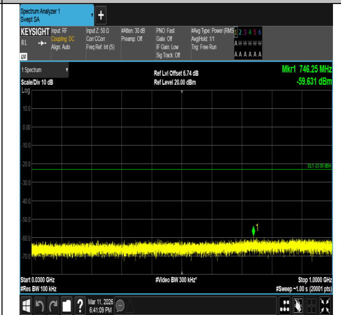
Band66-15MHz-16QAM-132047-75RB#0-30~1000-PASS
