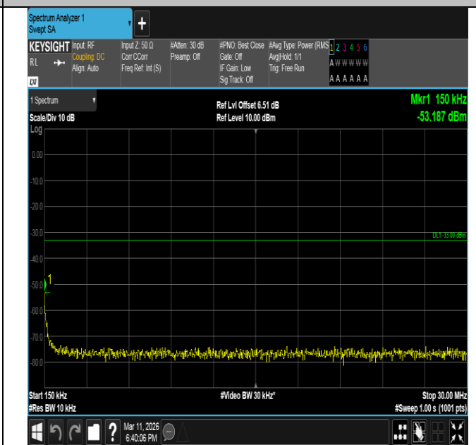
Band66-15MHz-QPSK-132047-75RB#0-0.15~30-PASS
