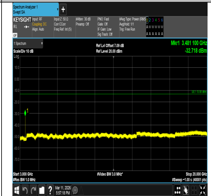
Band66-10MHz-16QAM-132322-1RB#0-3000~20000-PASS
