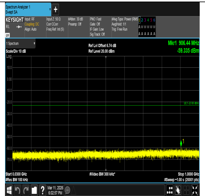
Band66-10MHz-QPSK-132622-1RB#49-30~1000-PASS
