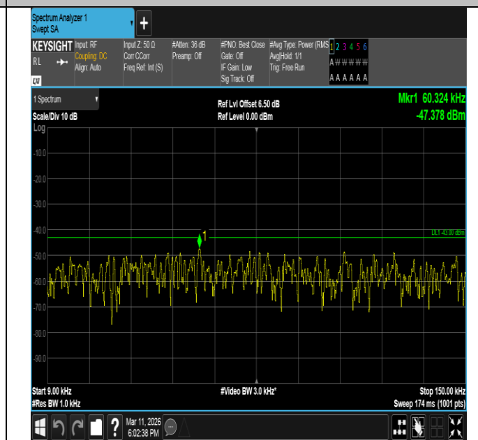
Band66-10MHz-QPSK-132622-1RB#49-0.009~0.15-PASS
