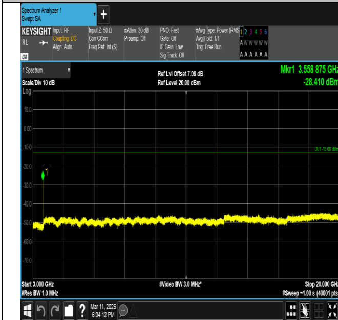
Band66-10MHz-16QAM-132622-1RB#49-3000~20000-PASS
