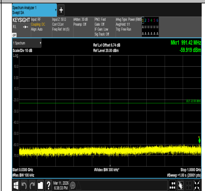
Band66-15MHz-QPSK-132047-1RB#74-30~1000-PASS
