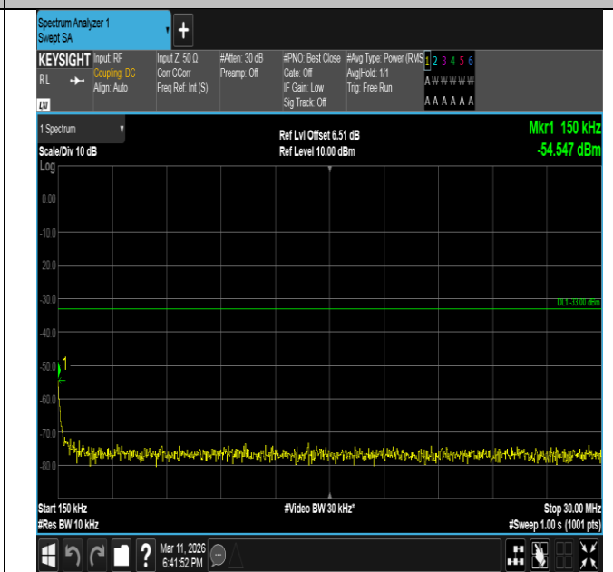
Band66-15MHz-QPSK-132322-1RB#0-0.15~30-PASS
