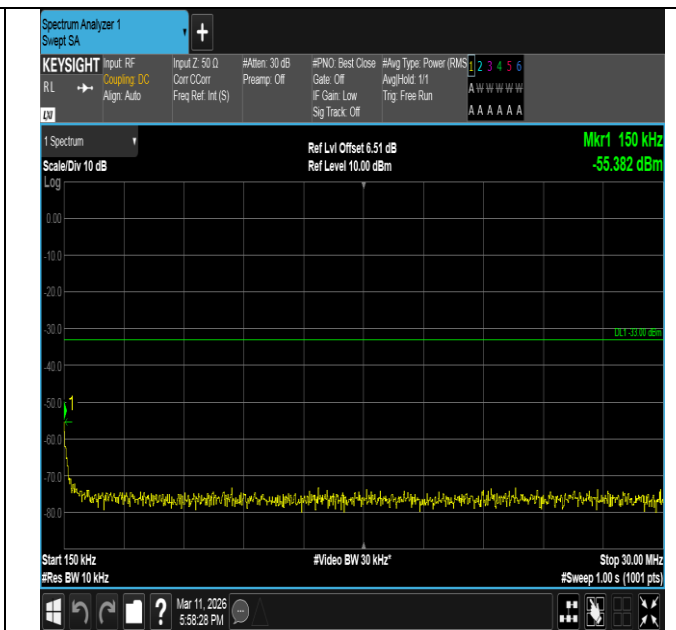
Band66-10MHz-16QAM-132322-1RB#49-0.15~30-PASS
