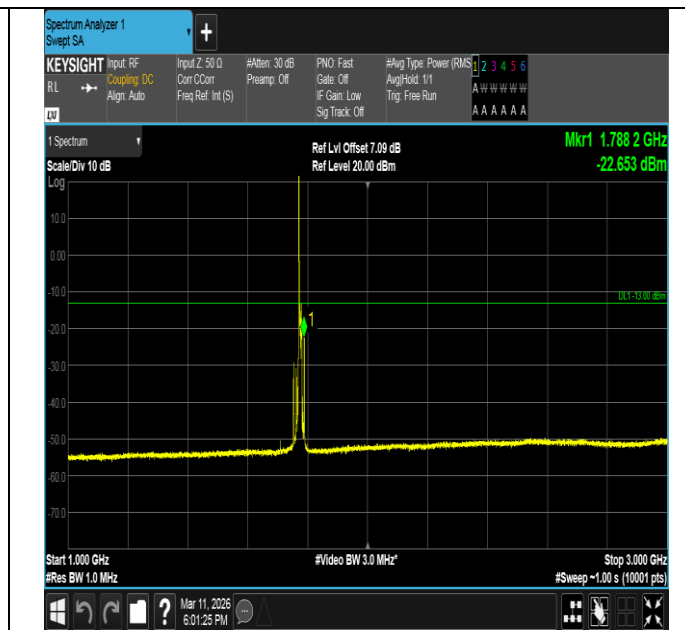
Band66-10MHz-QPSK-132622-1RB#0-1000~3000-PASS
