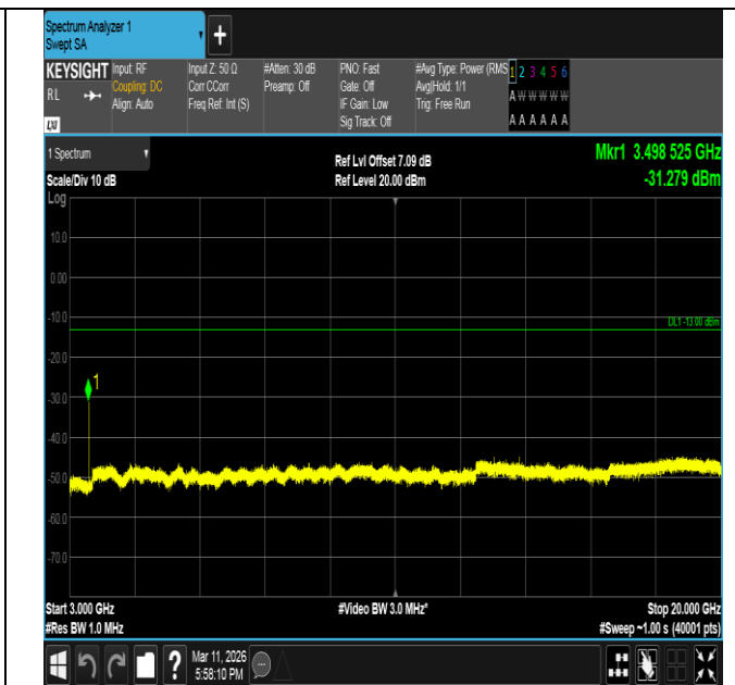
Band66-10MHz-QPSK-132322-1RB#49-3000~20000-PASS
