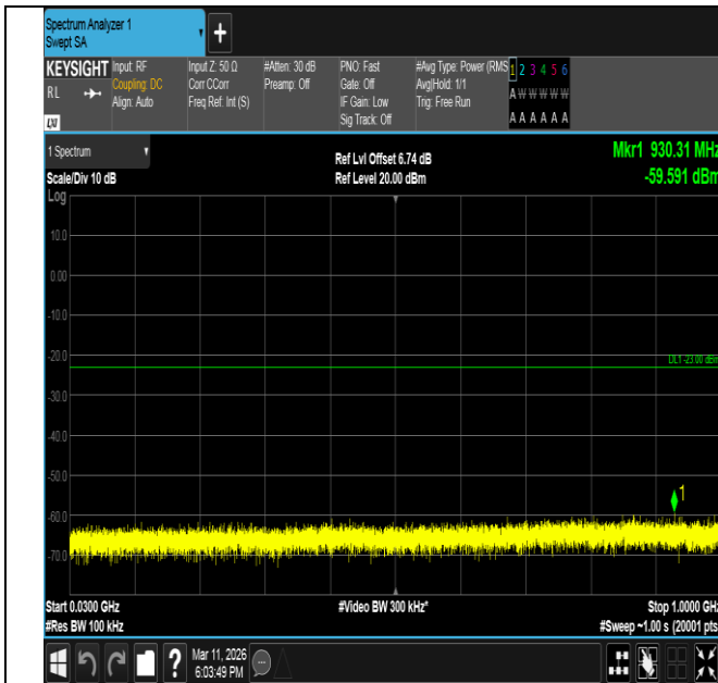
Band66-10MHz-16QAM-132622-1RB#49-30~1000-PASS
