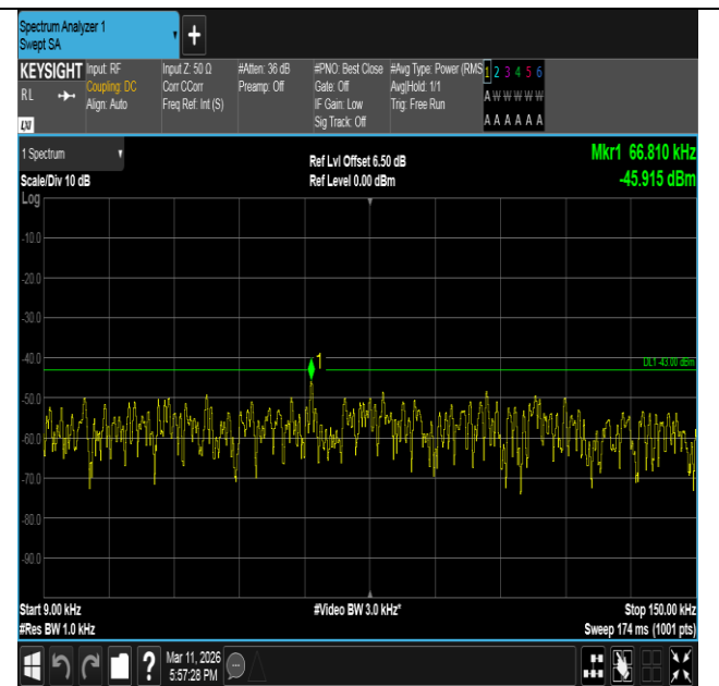
Band66-10MHz-QPSK-132322-1RB#49-0.009~0.15-PASS
