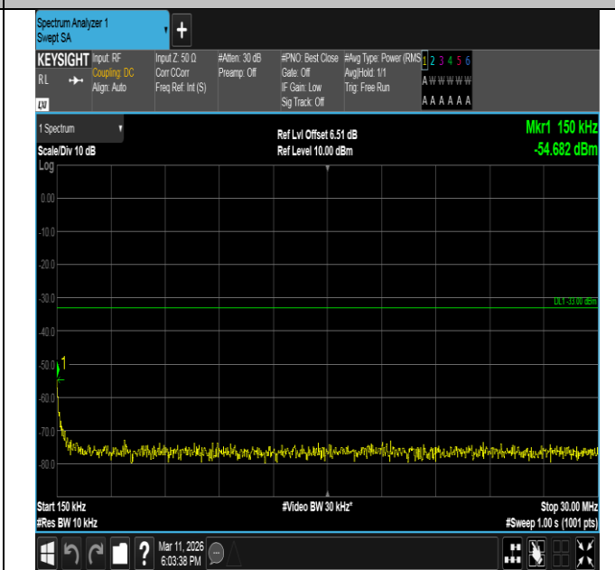
Band66-10MHz-16QAM-132622-1RB#49-0.15~30-PASS
