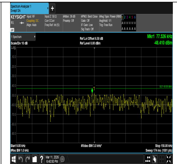
Band66-15MHz-16QAM-132047-75RB#0-0.009~0.15-PASS
