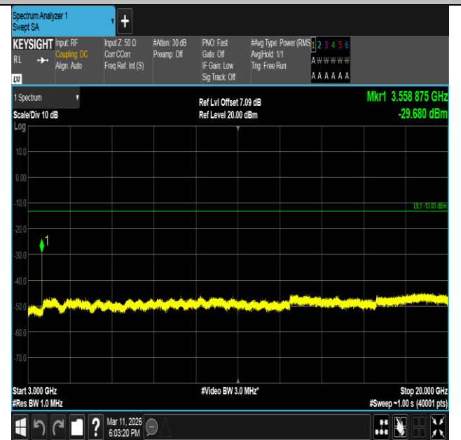
Band66-10MHz-QPSK-132622-1RB#49-3000~20000-PASS
