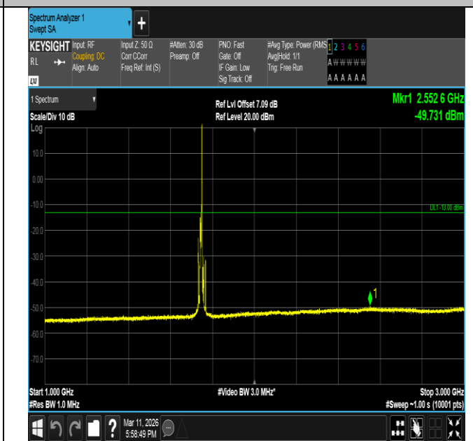
Band66-10MHz-16QAM-132322-1RB#49-1000~3000-PASS
