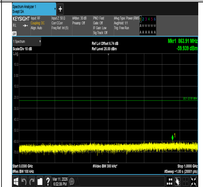
Band66-10MHz-16QAM-132622-1RB#0-30~1000-PASS
