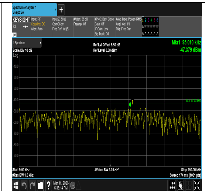
Band66-15MHz-QPSK-132047-1RB#74-0.009~0.15-PASS
