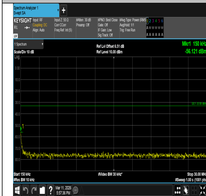
Band66-10MHz-QPSK-132322-1RB#49-0.15~30-PASS
