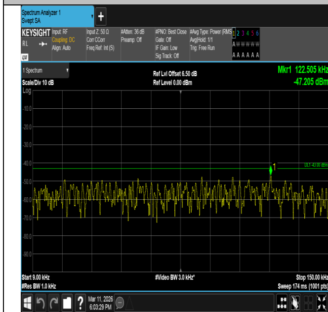
Band66-10MHz-16QAM-132622-1RB#49-0.009~0.15-PASS
