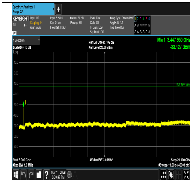
Band66-15MHz-16QAM-132047-1RB#74-3000~20000-PASS
