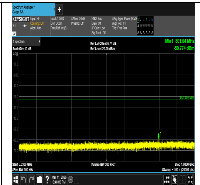
Band66-15MHz-16QAM-132597-1RB#0-30~1000-PASS
