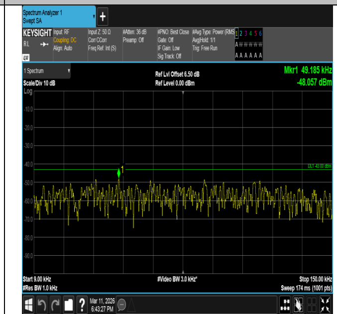
Band66-15MHz-QPSK-132322-1RB#74-0.009~0.15-PASS
