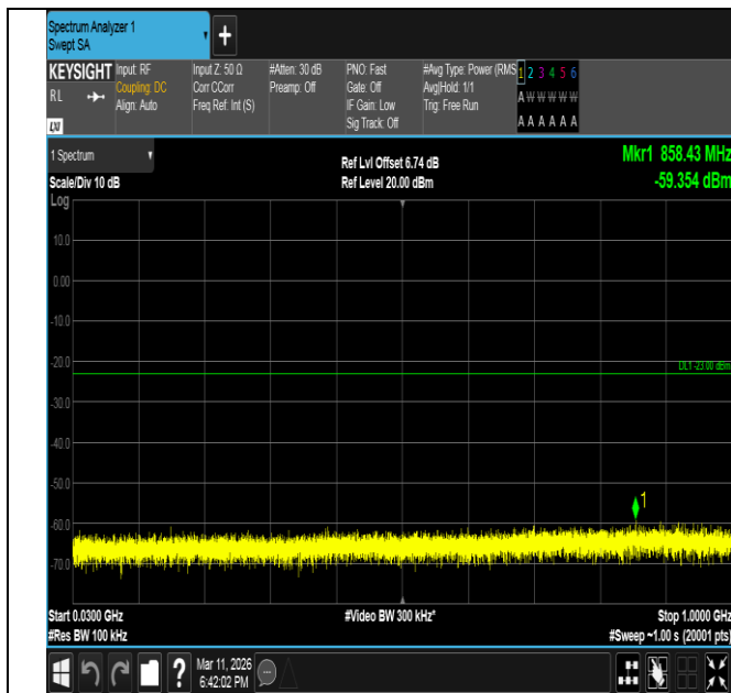
Band66-15MHz-QPSK-132322-1RB#0-30~1000-PASS
