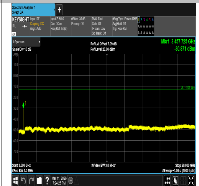
Band66-20MHz-QPSK-132072-1RB#99-3000~20000-PASS
