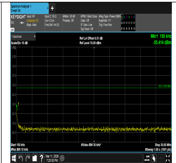
Band66-20MHz-QPSK-132072-100RB#0-0.15~30-PASS
