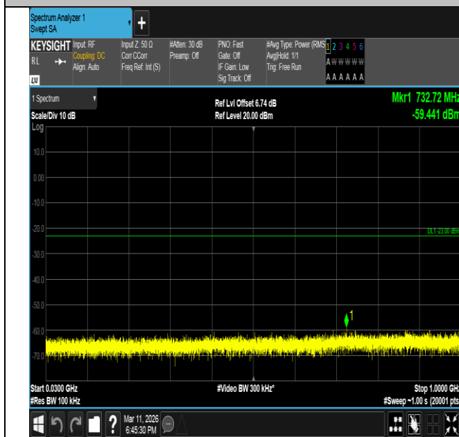
Band66-15MHz-QPSK-132322-75RB#0-30~1000-PASS
