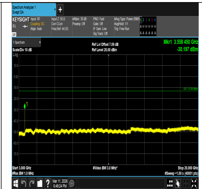
Band66-15MHz-QPSK-132597-1RB#74-3000~20000-PASS
