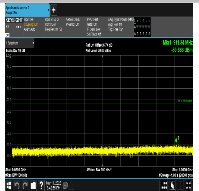
Band66-15MHz-16QAM-132322-1RB#0-30~1000-PASS
