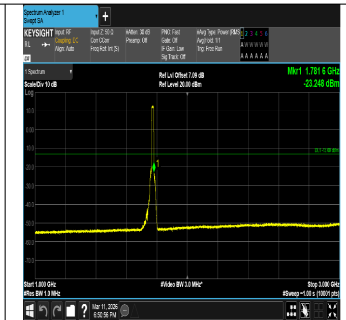
Band66-15MHz-QPSK-132597-75RB#0-1000~3000-PASS
