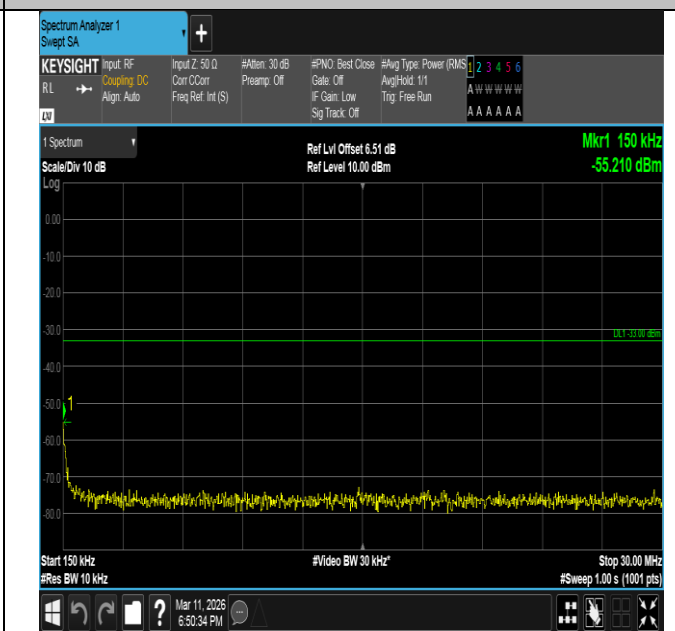
Band66-15MHz-QPSK-132597-75RB#0-0.15~30-PASS
