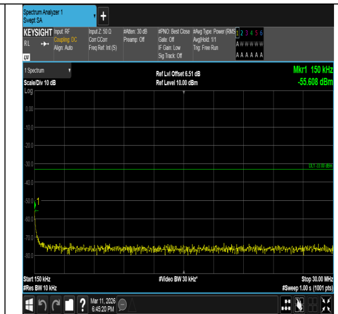
Band66-15MHz-QPSK-132322-75RB#0-0.15~30-PASS
