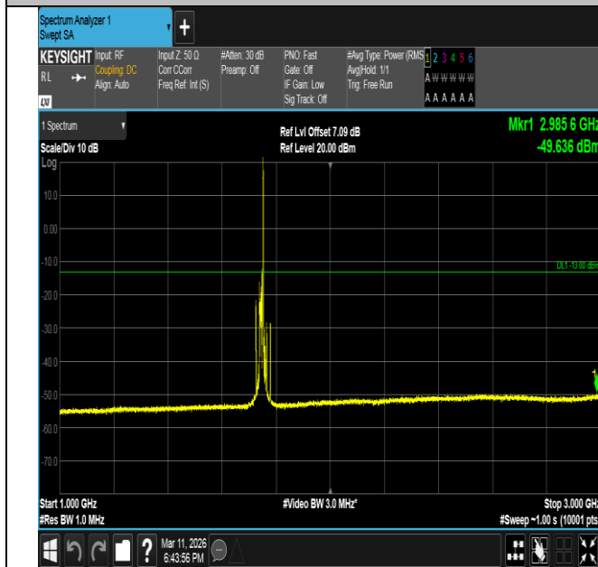
Band66-15MHz-QPSK-132322-1RB#74-1000~3000-PASS
