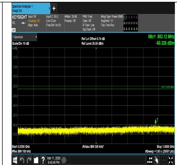
Band66-15MHz-QPSK-132322-1RB#74-30~1000-PASS
