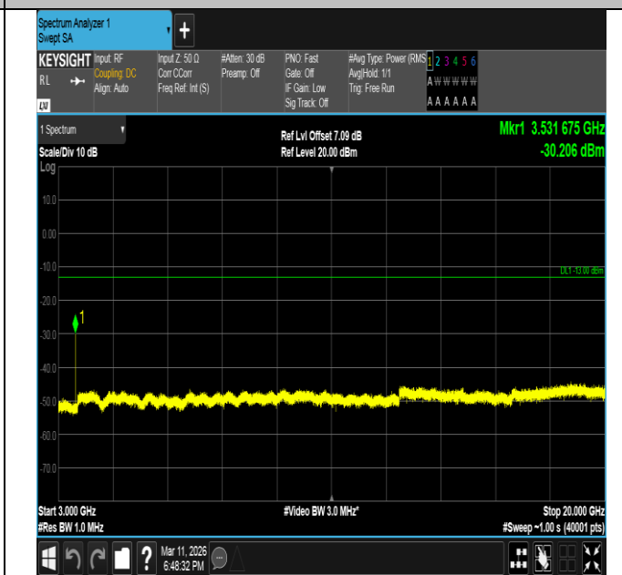
Band66-15MHz-16QAM-132597-1RB#0-3000~20000-PASS
