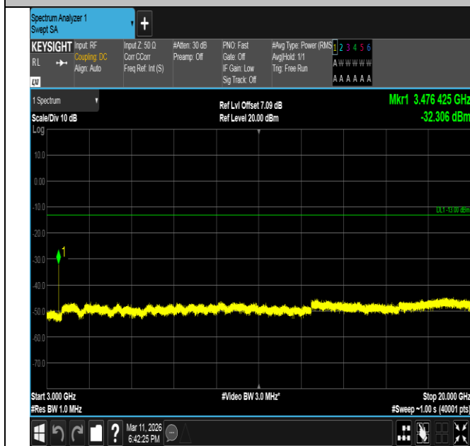
Band66-15MHz-QPSK-132322-1RB#0-3000~20000-PASS
