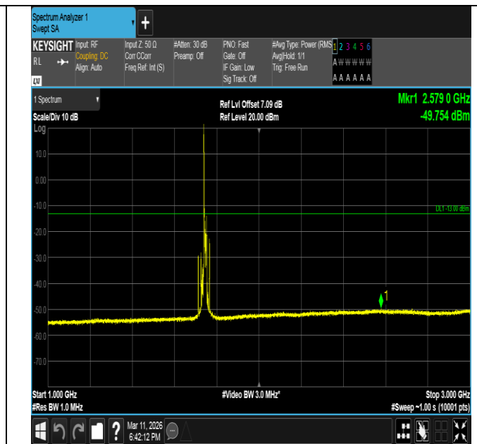
Band66-15MHz-QPSK-132322-1RB#0-1000~3000-PASS
