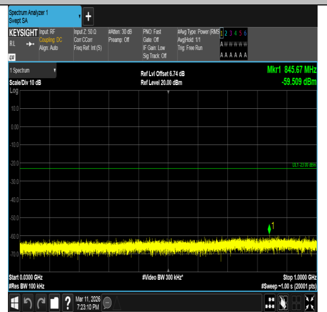
Band66-20MHz-16QAM-132072-1RB#0-30~1000-PASS
