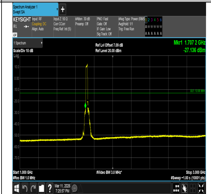
Band66-20MHz-QPSK-132072-100RB#0-1000~3000-PASS
