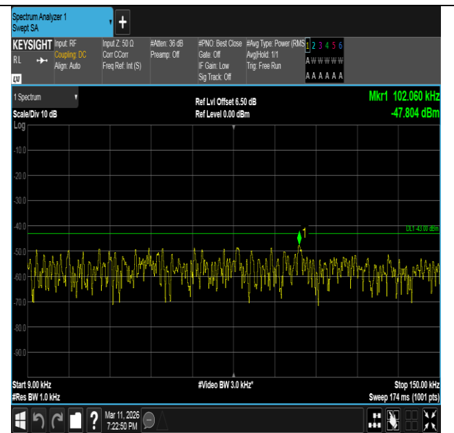
Band66-20MHz-16QAM-132072-1RB#0-0.009~0.15-PASS
