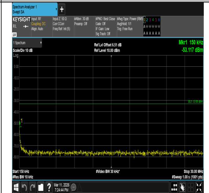
Band66-20MHz-16QAM-132072-1RB#99-0.15~30-PASS
