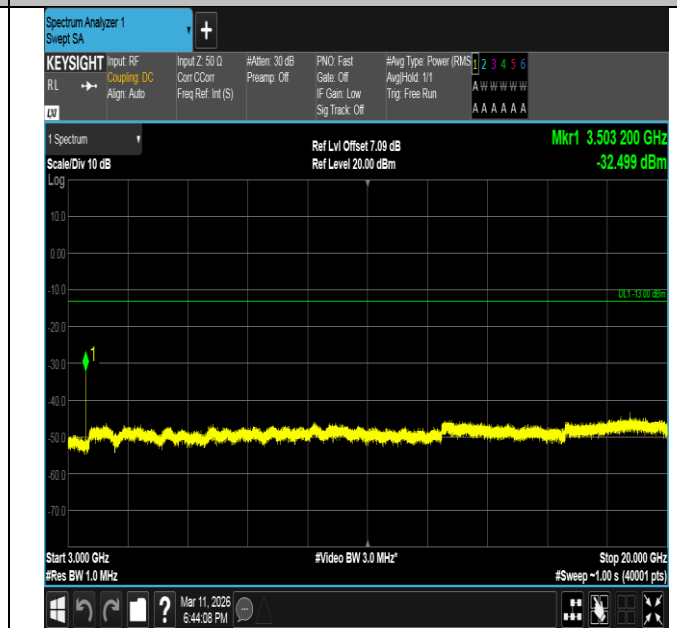
Band66-15MHz-QPSK-132322-1RB#74-3000~20000-PASS
