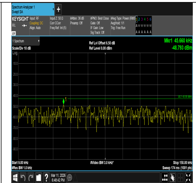
Band66-15MHz-QPSK-132597-1RB#74-0.009~0.15-PASS
