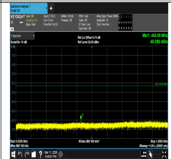
Band66-15MHz-QPSK-132597-1RB#74-30~1000-PASS
