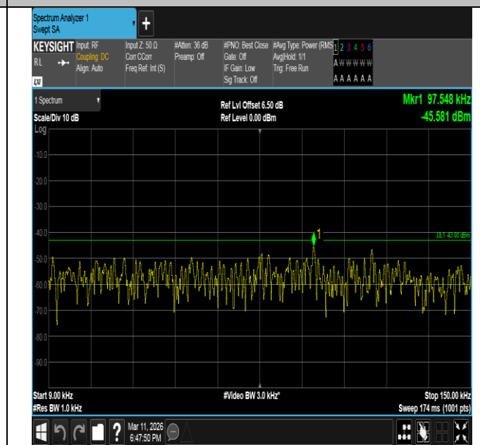
Band66-15MHz-16QAM-132597-1RB#0-0.009~0.15-PASS
