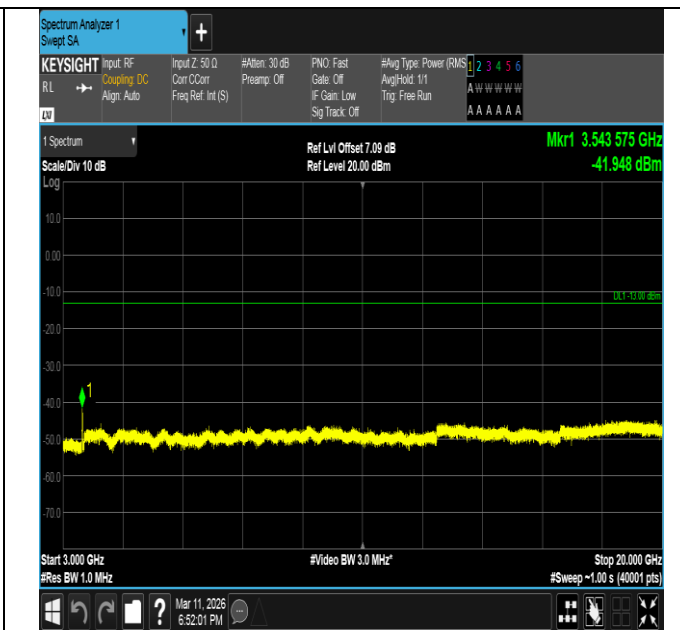
Band66-15MHz-16QAM-132597-75RB#0-3000~20000-PASS
