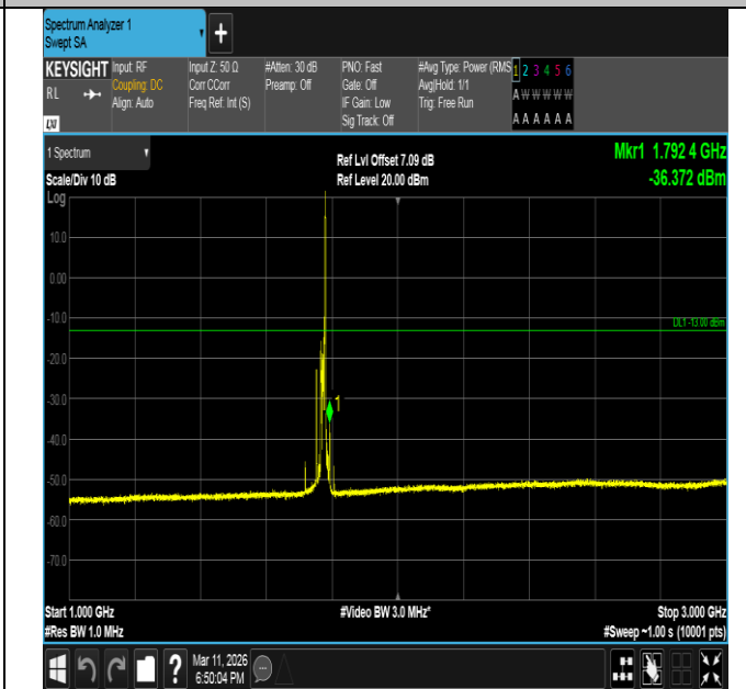
Band66-15MHz-16QAM-132597-1RB#74-1000~3000-PASS
