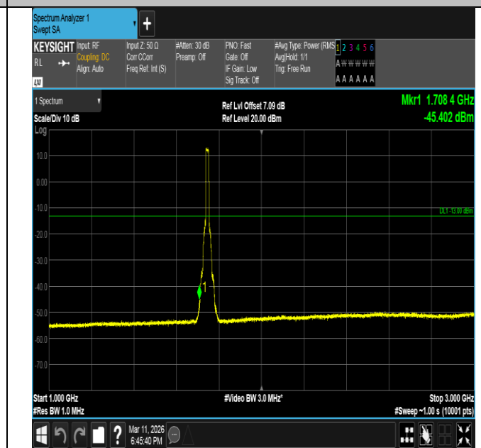
Band66-15MHz-QPSK-132322-75RB#0-1000~3000-PASS
