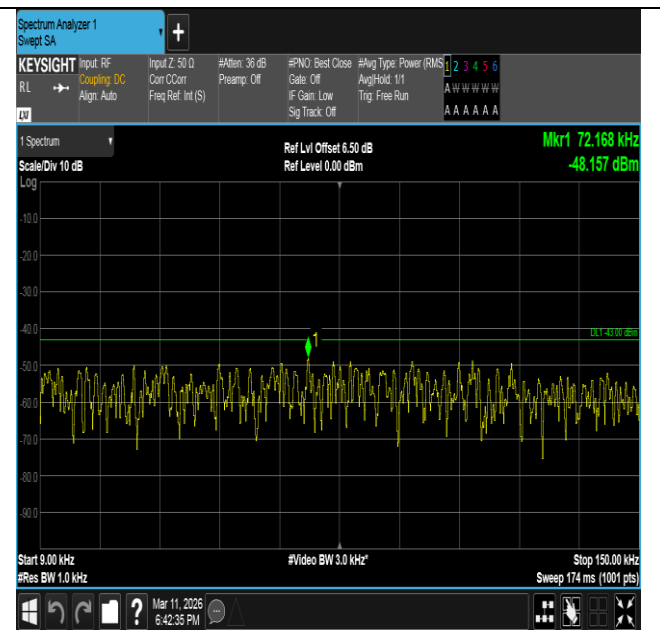
Band66-15MHz-16QAM-132322-1RB#0-0.009~0.15-PASS
