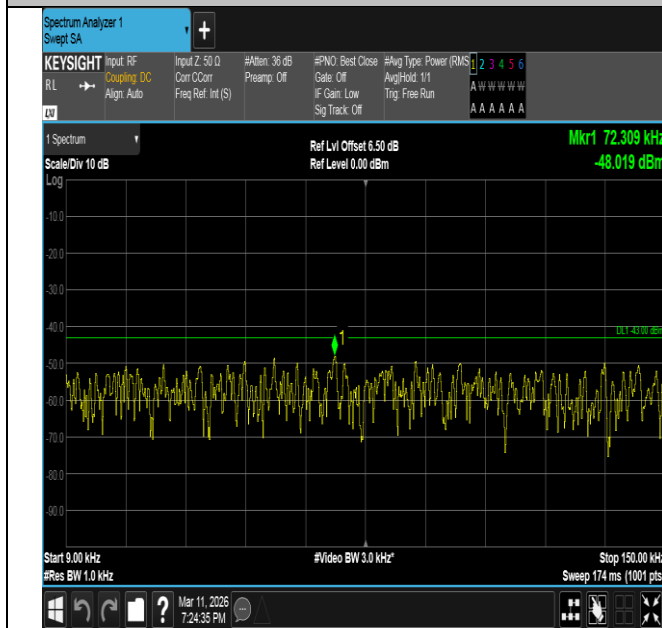
Band66-20MHz-16QAM-132072-1RB#99-0.009~0.15-PASS
