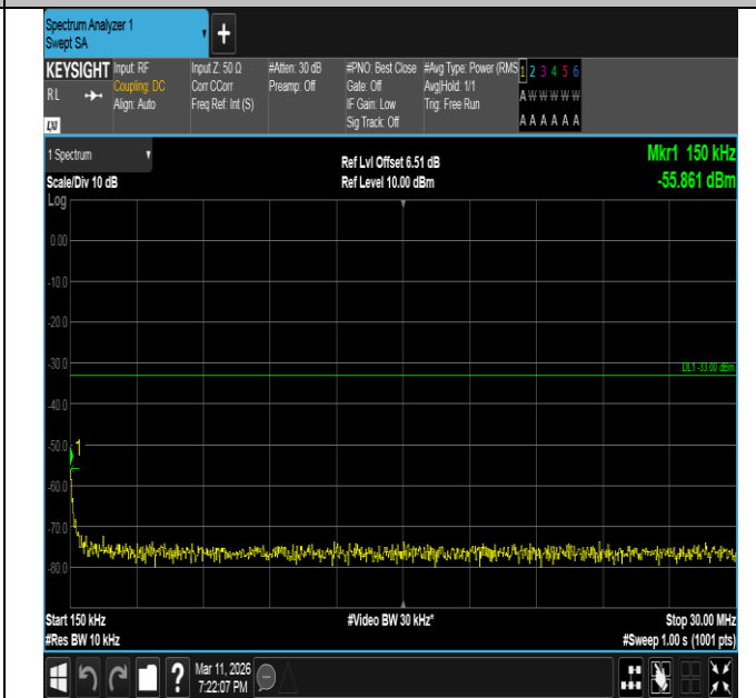
Band66-20MHz-QPSK-132072-1RB#0-0.15~30-PASS
