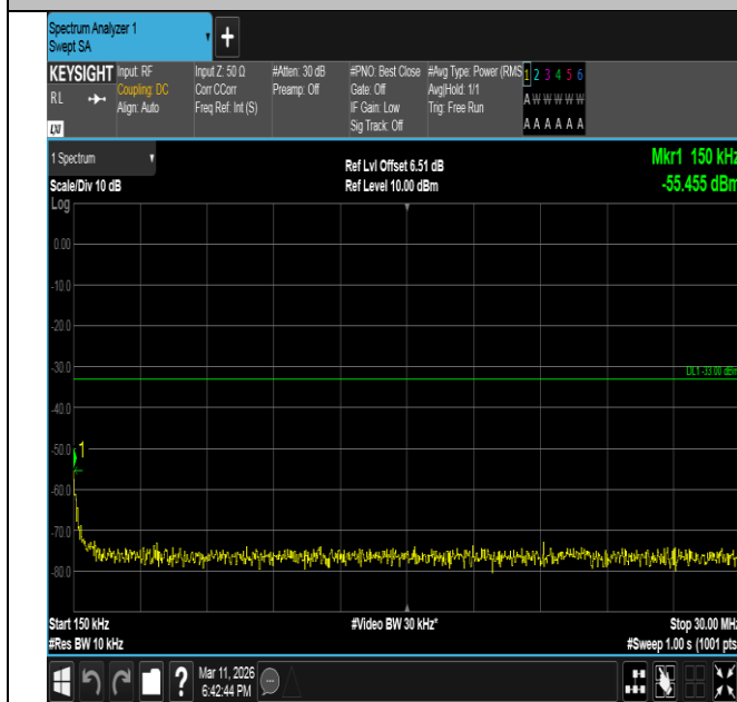
Band66-15MHz-16QAM-132322-1RB#0-0.15~30-PASS
