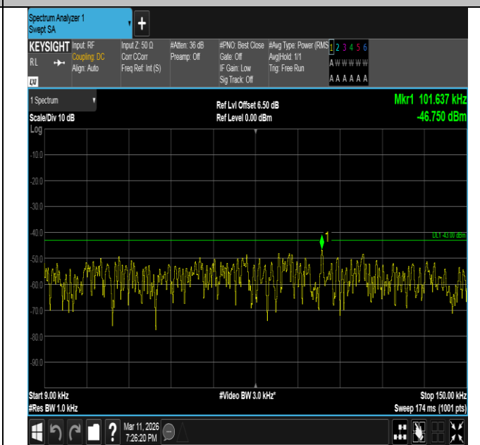
Band66-20MHz-16QAM-132072-100RB#0-0.009~0.15-PASS
