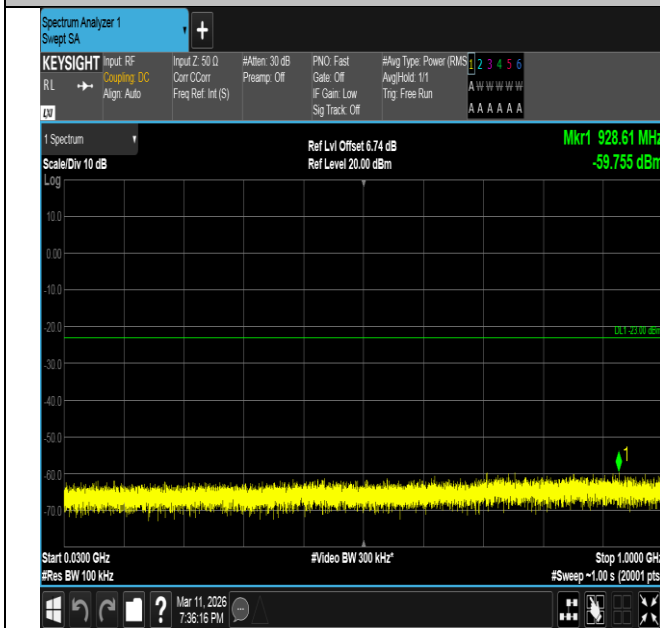
Band66-20MHz-QPSK-132572-100RB#0-30~1000-PASS
