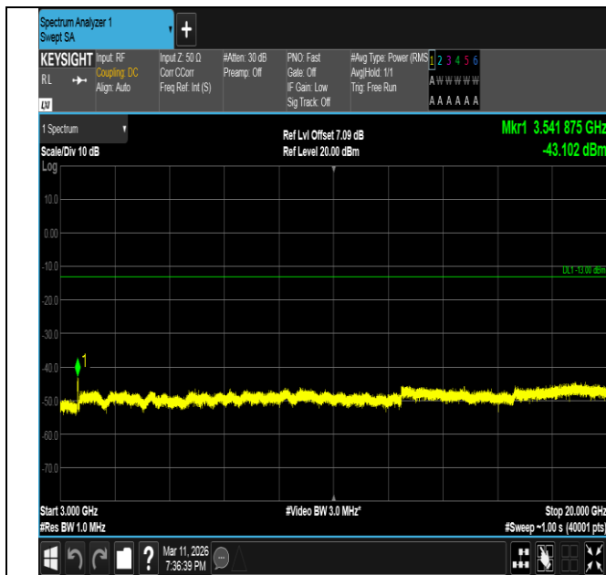
Band66-20MHz-QPSK-132572-100RB#0-3000~20000-PASS
