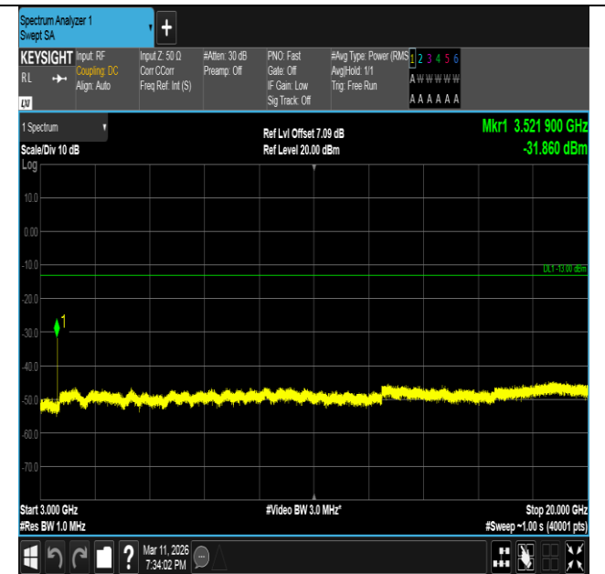
Band66-20MHz-16QAM-132572-1RB#0-3000~20000-PASS
