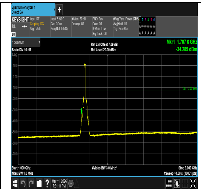
Band66-20MHz-QPSK-132322-100RB#0-1000~3000-PASS
