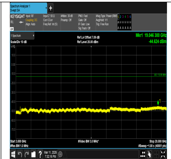
Band66-20MHz-16QAM-132322-100RB#0-3000~20000-PASS
