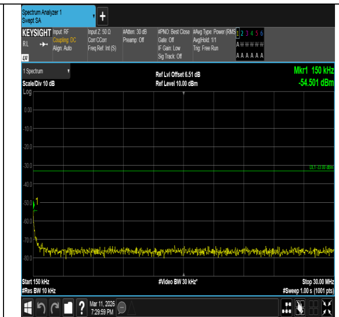
Band66-20MHz-16QAM-132322-1RB#99-0.15~30-PASS
