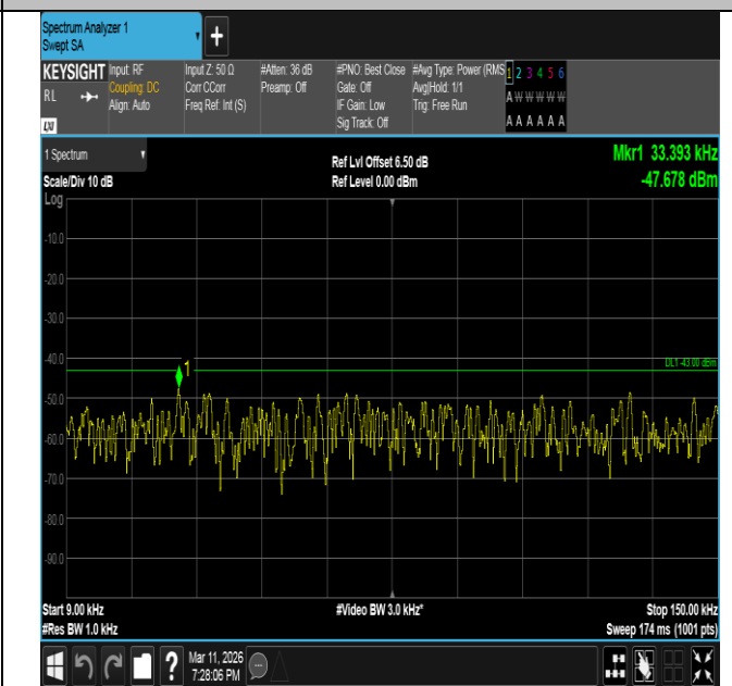
Band66-20MHz-16QAM-132322-1RB#0-0.009~0.15-PASS
