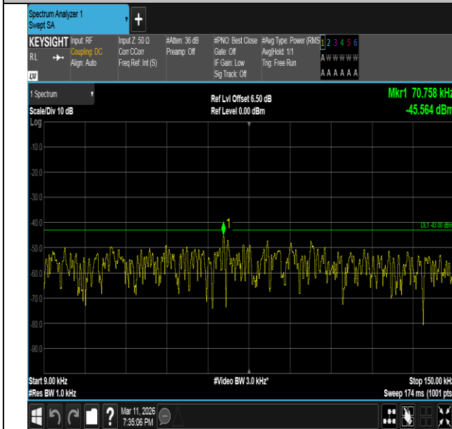
Band66-20MHz-16QAM-132572-1RB#99-0.009~0.15-PASS
