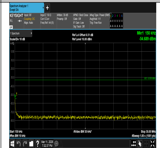
Band66-20MHz-QPSK-132572-1RB#0-0.15~30-PASS
