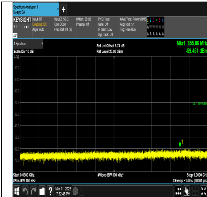
Band66-20MHz-QPSK-132572-1RB#0-30~1000-PASS
