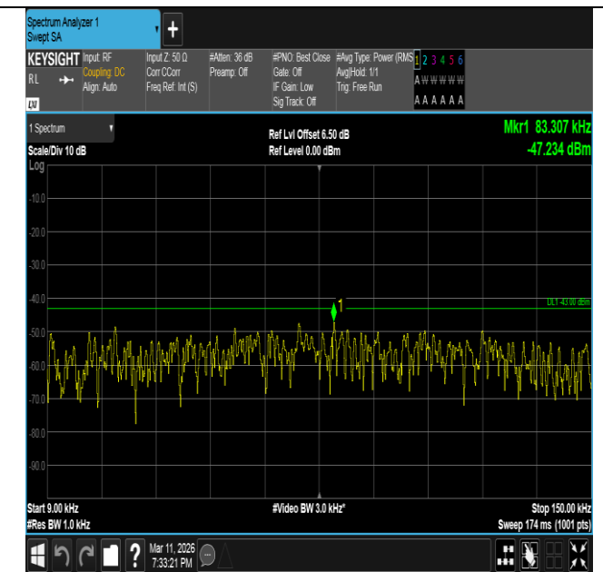
Band66-20MHz-16QAM-132572-1RB#0-0.009~0.15-PASS
