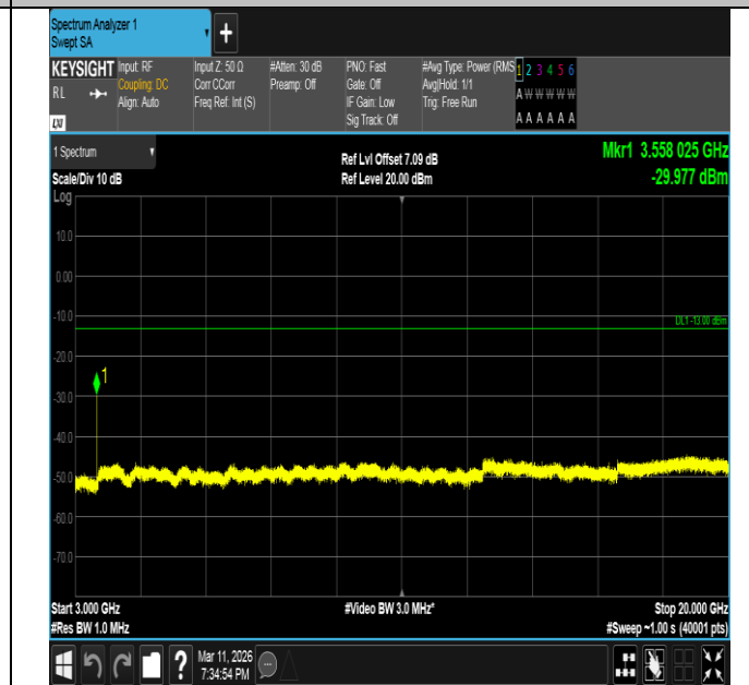
Band66-20MHz-QPSK-132572-1RB#99-3000~20000-PASS
