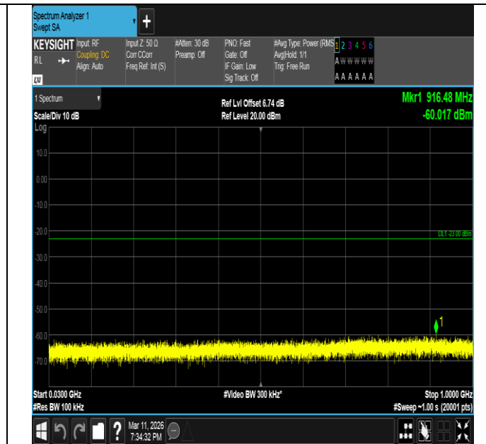
Band66-20MHz-QPSK-132572-1RB#99-30~1000-PASS
