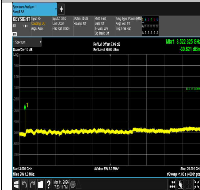
Band66-20MHz-QPSK-132572-1RB#0-3000~20000-PASS
