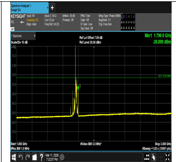
Band66-20MHz-QPSK-132572-1RB#0-1000~3000-PASS
