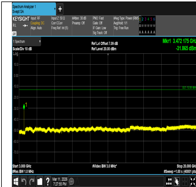
Band66-20MHz-QPSK-132322-1RB#0-3000~20000-PASS
