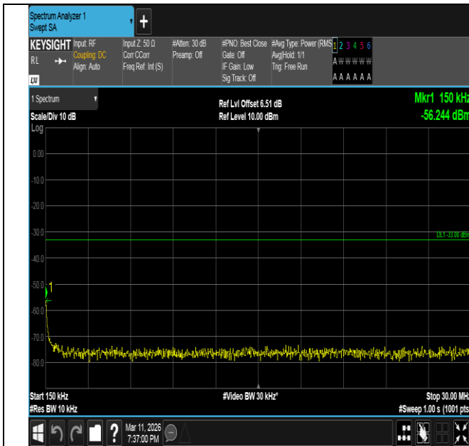
Band66-20MHz-16QAM-132572-100RB#0-0.15~30-PASS
