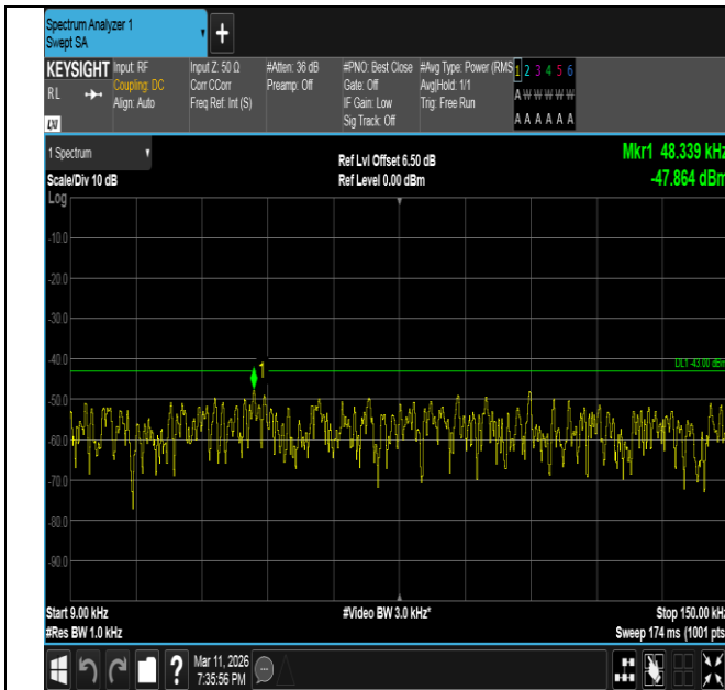
Band66-20MHz-QPSK-132572-100RB#0-0.009~0.15-PASS
