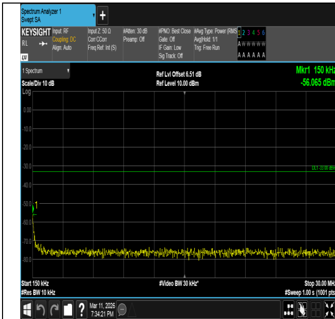
Band66-20MHz-QPSK-132572-1RB#99-0.15~30-PASS
