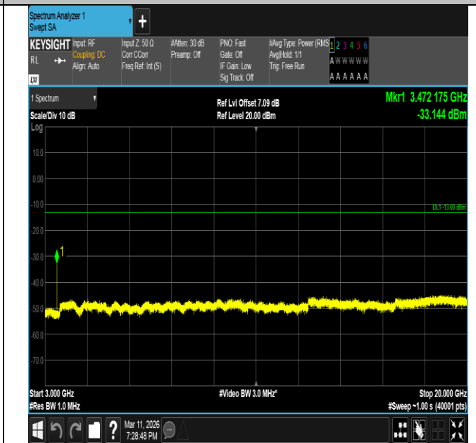
Band66-20MHz-16QAM-132322-1RB#0-3000~20000-PASS
