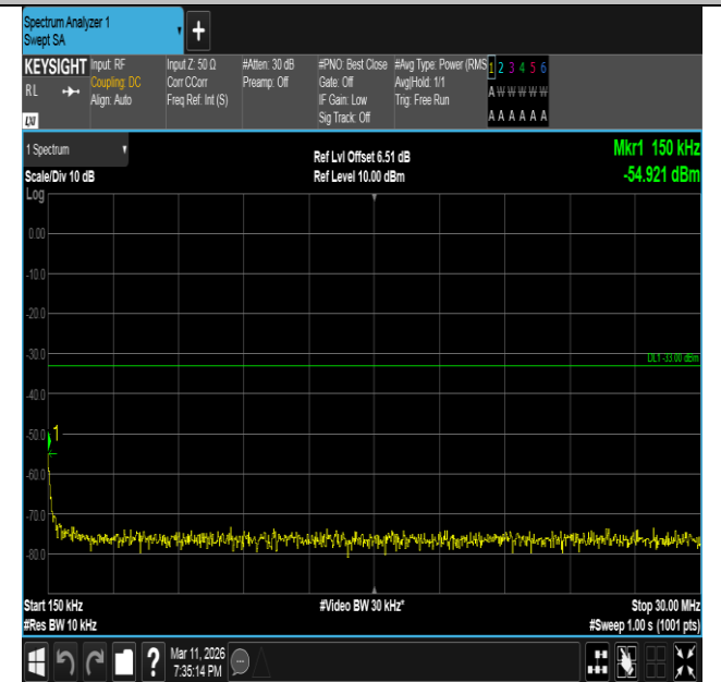
Band66-20MHz-16QAM-132572-1RB#99-0.15~30-PASS
