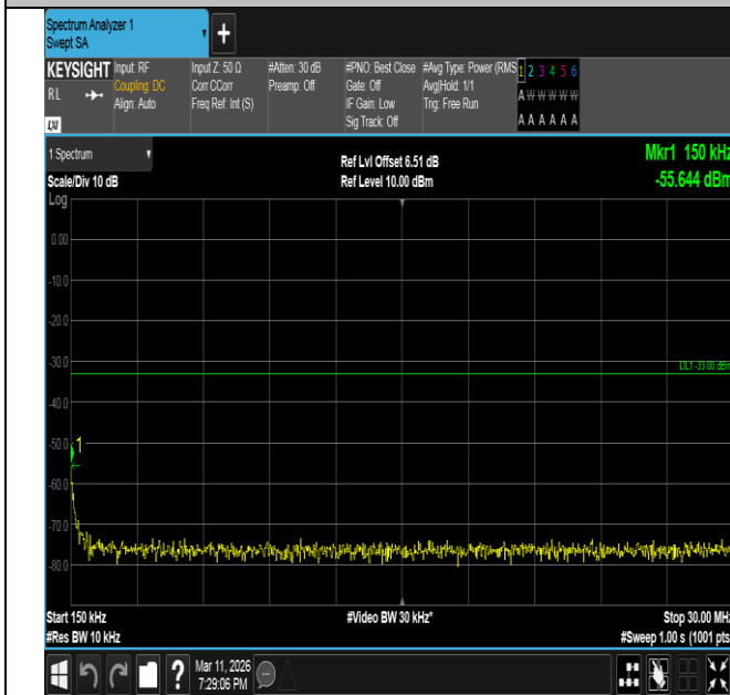
Band66-20MHz-QPSK-132322-1RB#99-0.15~30-PASS
