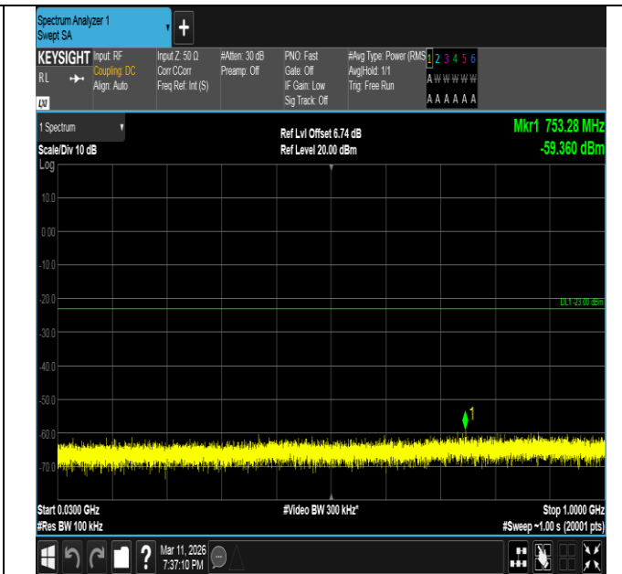
Band66-20MHz-16QAM-132572-100RB#0-30~1000-PASS
