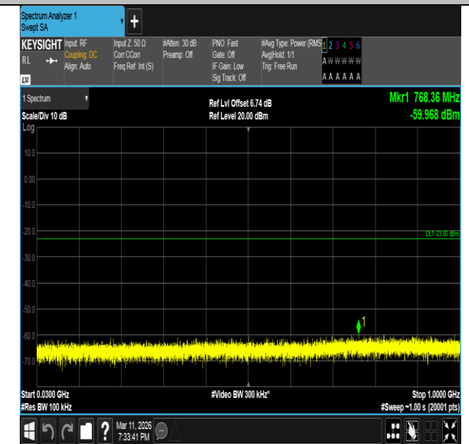
Band66-20MHz-16QAM-132572-1RB#0-30~1000-PASS
