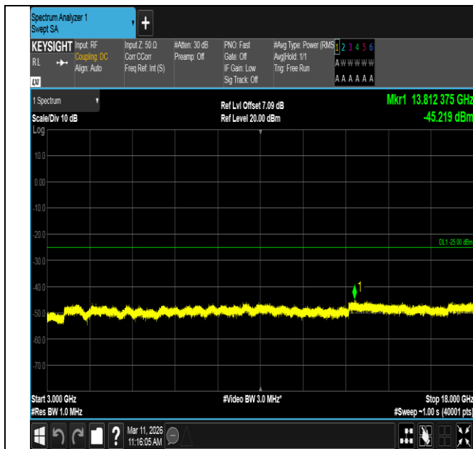
Band7-5MHz-QPSK-21425-1RB#24-3000~18000-PASS
