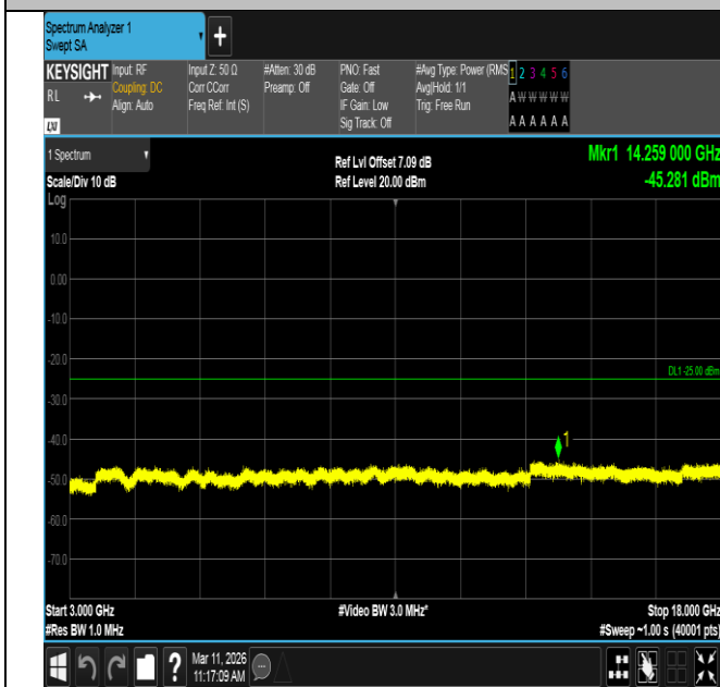
Band7-5MHz-16QAM-21425-1RB#24-3000~18000-PASS
