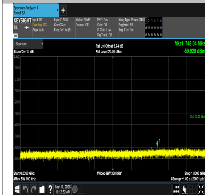
Band7-5MHz-16QAM-21100-25RB#0-30~1000-PASS
