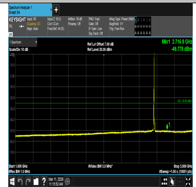
Band7-5MHz-QPSK-21425-1RB#24-1000~3000-PASS
