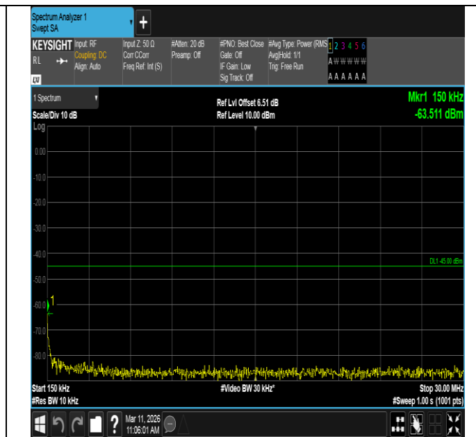
Band7-5MHz-16QAM-20775-25RB#0-0.15~30-PASS
