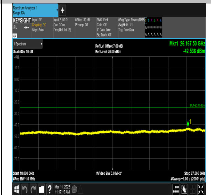
Band7-5MHz-16QAM-21425-1RB#24-18000~27000-PASS
