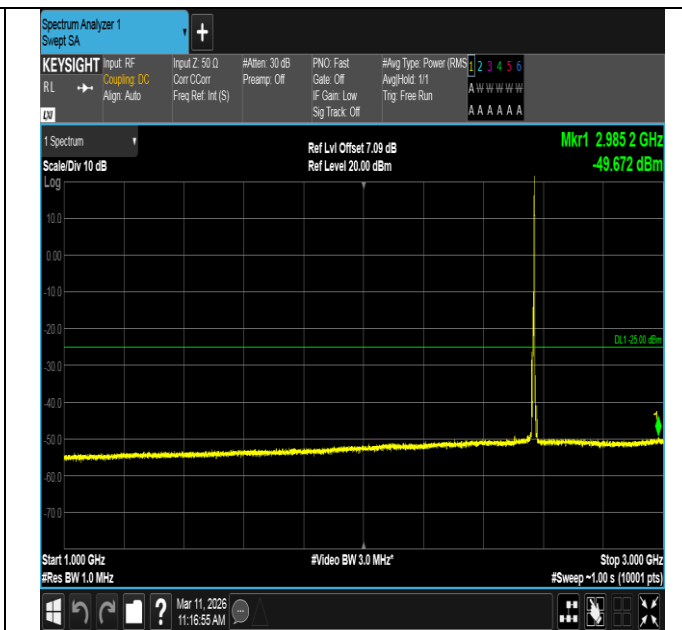
Band7-5MHz-16QAM-21425-1RB#24-1000~3000-PASS
