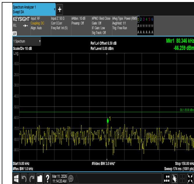
Band7-5MHz-16QAM-21425-1RB#0-0.009~0.15-PASS
