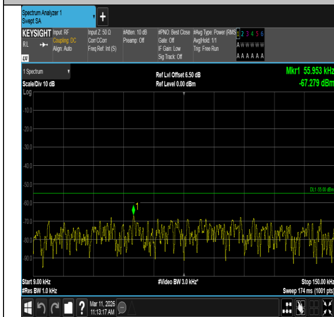
Band7-5MHz-QPSK-21425-1RB#0-0.009~0.15-PASS
