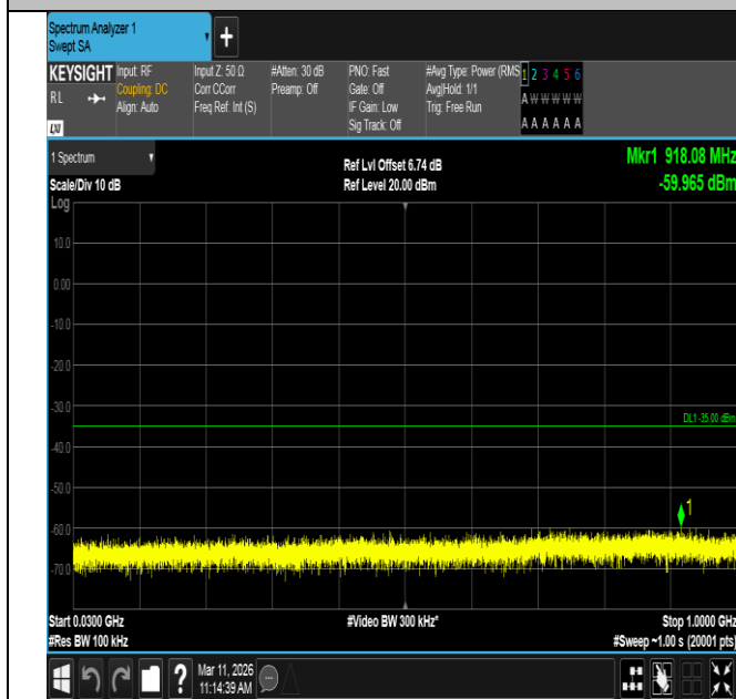
Band7-5MHz-16QAM-21425-1RB#0-30~1000-PASS
