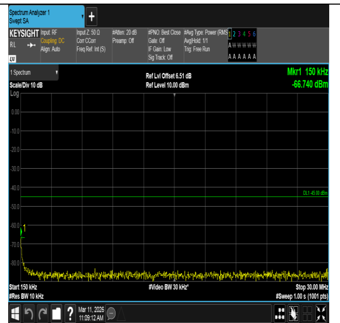
Band7-5MHz-QPSK-21100-1RB#24-0.15~30-PASS
