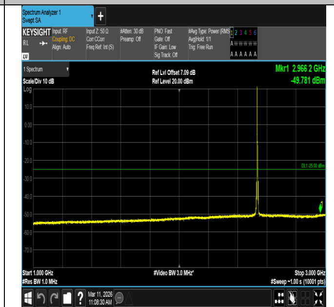
Band7-5MHz-16QAM-21100-1RB#0-1000~3000-PASS
