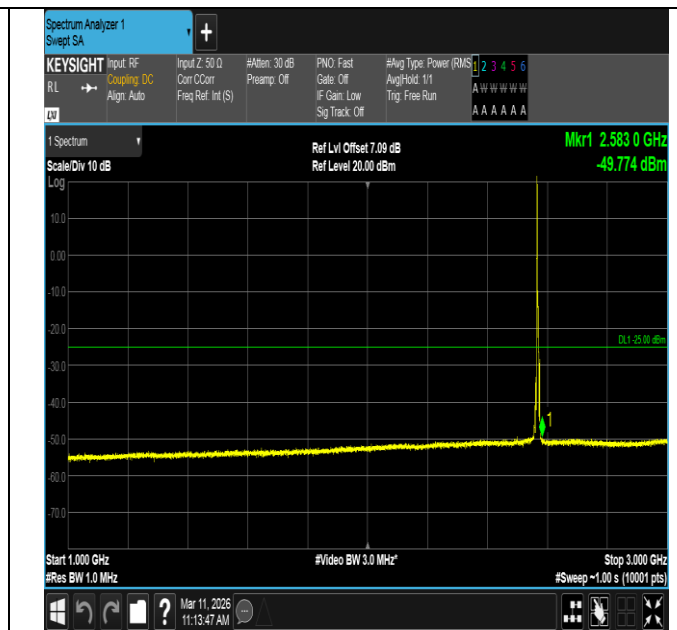
Band7-5MHz-QPSK-21425-1RB#0-1000~3000-PASS
