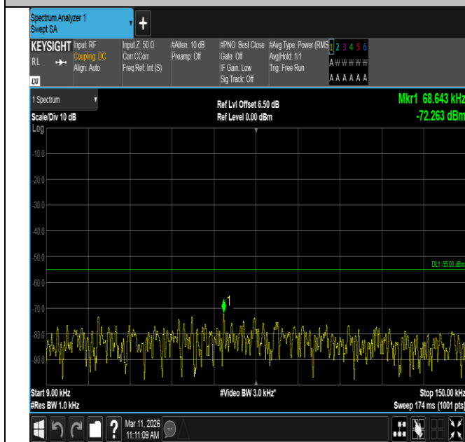
Band7-5MHz-QPSK-21100-25RB#0-0.009~0.15-PASS
