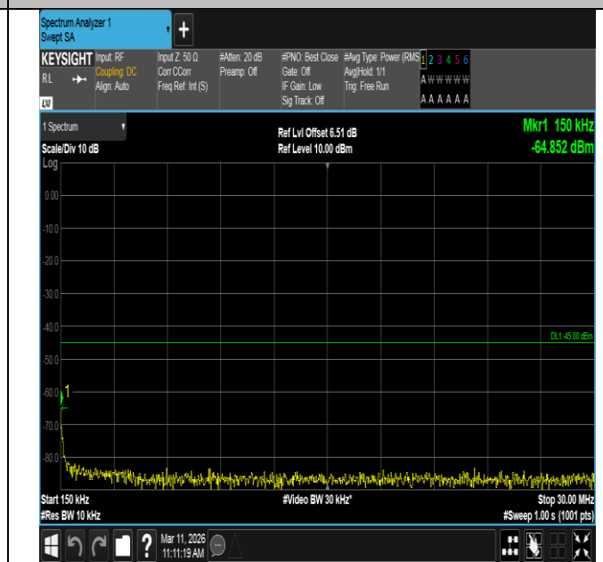
Band7-5MHz-QPSK-21100-25RB#0-0.15~30-PASS
