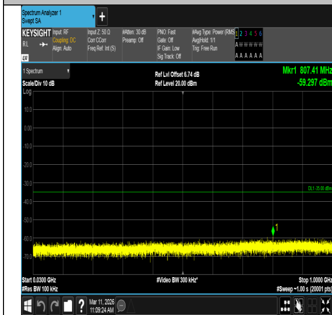
Band7-5MHz-QPSK-21100-1RB#24-30~1000-PASS
