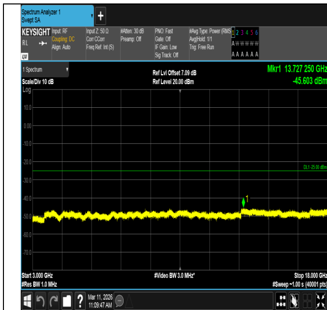
Band7-5MHz-QPSK-21100-1RB#24-3000~18000-PASS
