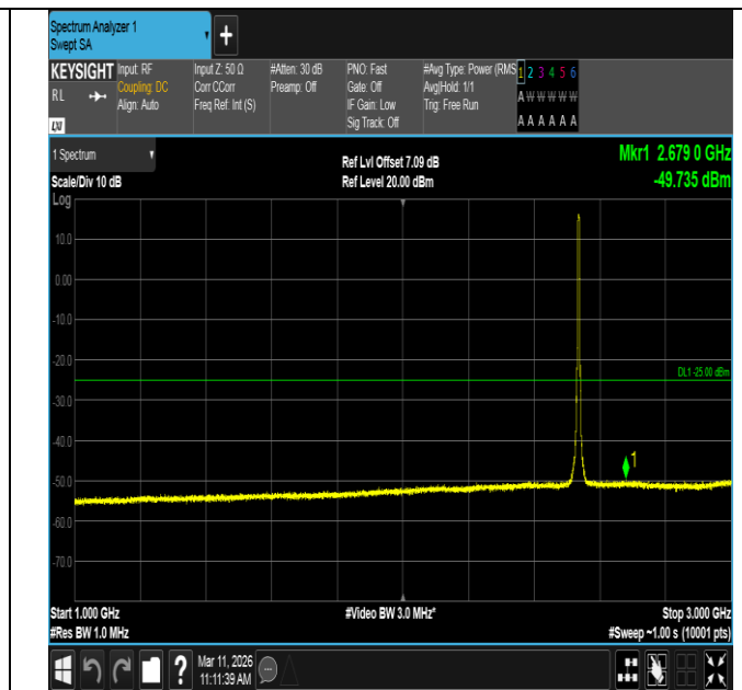
Band7-5MHz-QPSK-21100-25RB#0-1000~3000-PASS
