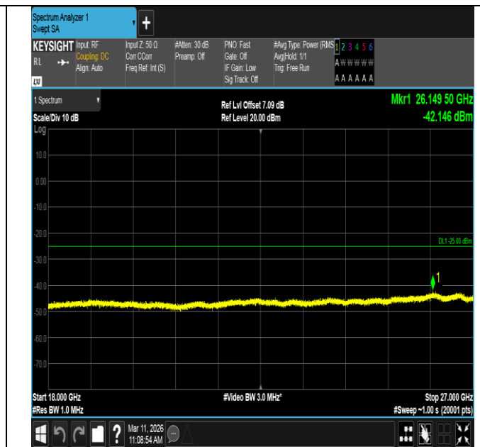
Band7-5MHz-16QAM-21100-1RB#0-18000~27000-PASS
