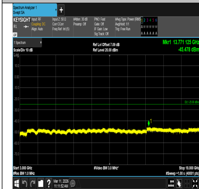
Band7-5MHz-QPSK-21100-25RB#0-3000~18000-PASS
