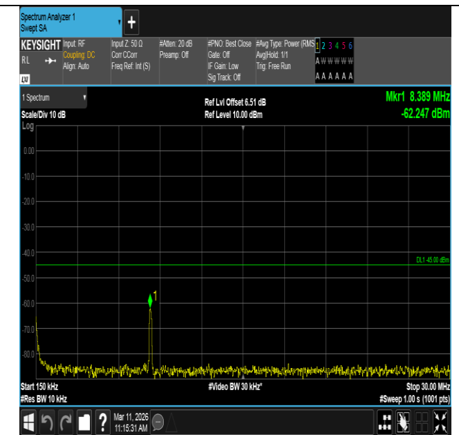
Band7-5MHz-QPSK-21425-1RB#24-0.15~30-PASS
