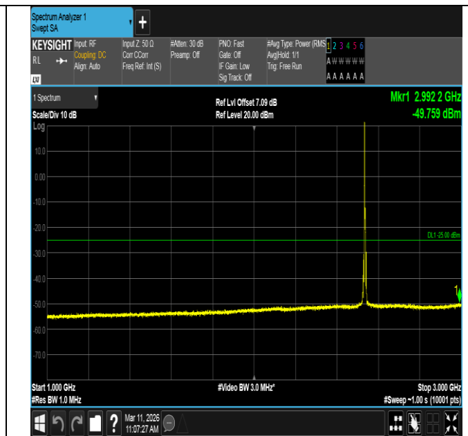
Band7-5MHz-QPSK-21100-1RB#0-1000~3000-PASS
