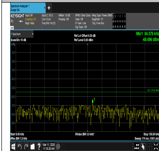
Band7-5MHz-16QAM-21425-1RB#24-0.009~0.15-PASS
