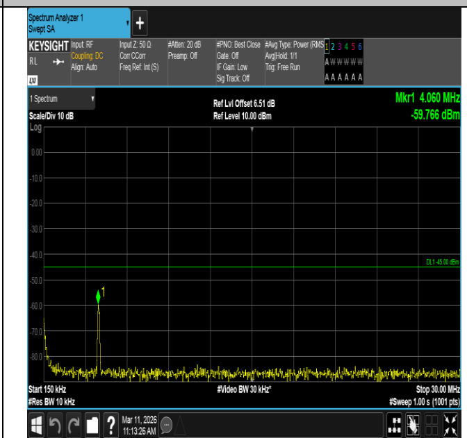
Band7-5MHz-QPSK-21425-1RB#0-0.15~30-PASS
