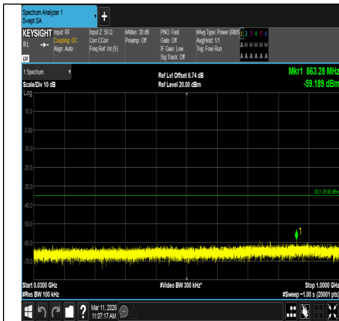
Band7-5MHz-QPSK-21100-1RB#0-30~1000-PASS
