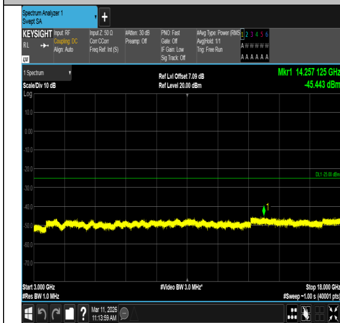
Band7-5MHz-QPSK-21425-1RB#0-3000~18000-PASS
