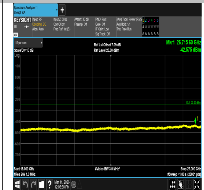
Band7-10MHz-QPSK-20800-1RB#0-18000~27000-PASS
