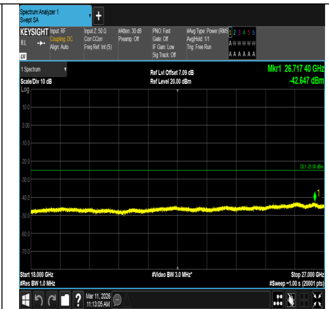
Band7-5MHz-16QAM-21100-25RB#0-18000~27000-PASS
