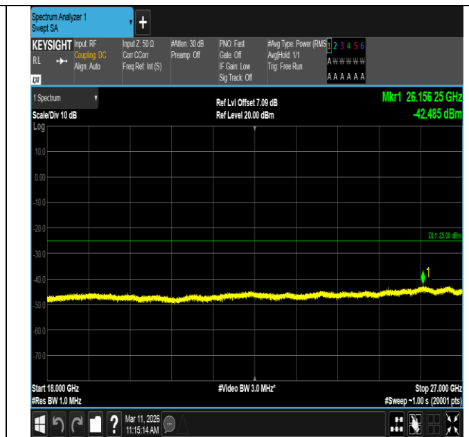
Band7-5MHz-16QAM-21425-1RB#0-18000~27000-PASS
