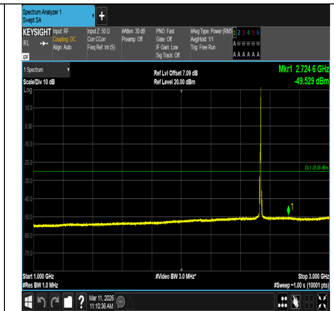
Band7-5MHz-16QAM-21100-1RB#24-1000~3000-PASS
