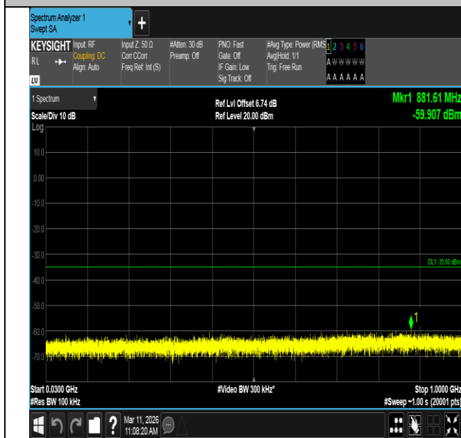
Band7-5MHz-16QAM-21100-1RB#0-30~1000-PASS
