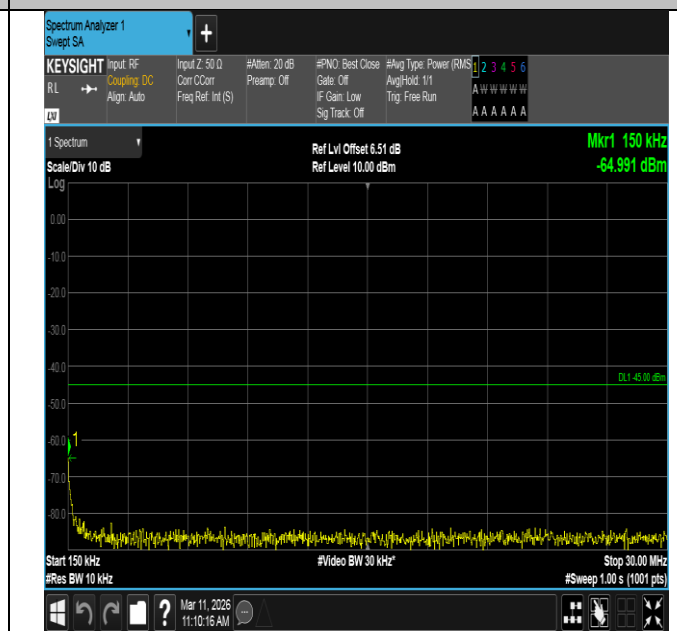
Band7-5MHz-16QAM-21100-1RB#24-0.15~30-PASS
