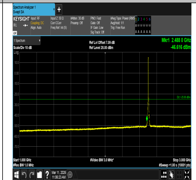
Band7-5MHz-16QAM-20775-25RB#0-1000~3000-PASS
