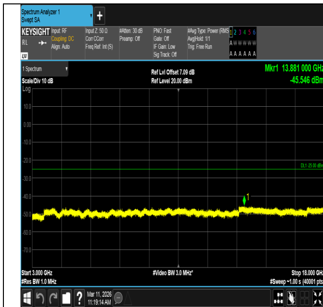
Band7-5MHz-16QAM-21425-25RB#0-3000~18000-PASS
