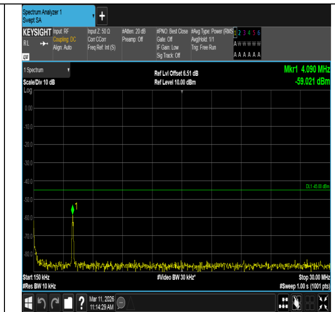
Band7-5MHz-16QAM-21425-1RB#0-0.15~30-PASS
