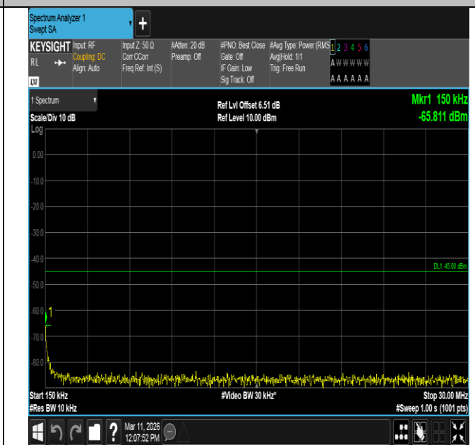
Band7-10MHz-QPSK-20800-1RB#0-0.15~30-PASS
