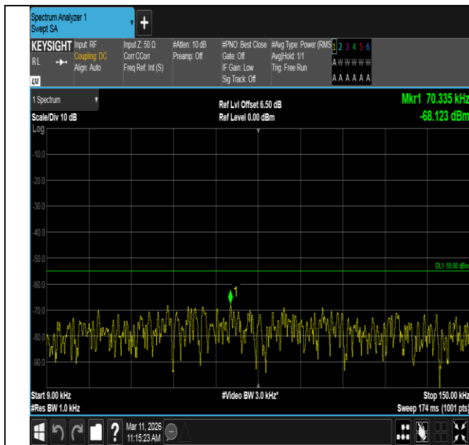
Band7-5MHz-QPSK-21425-1RB#24-0.009~0.15-PASS
