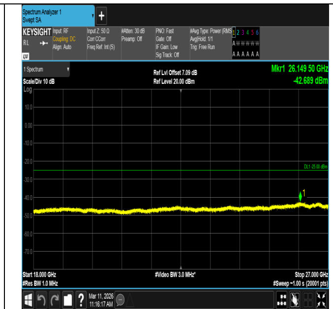
Band7-5MHz-QPSK-21425-1RB#24-18000~27000-PASS
