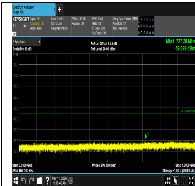
Band7-5MHz-16QAM-21425-1RB#24-30~1000-PASS
