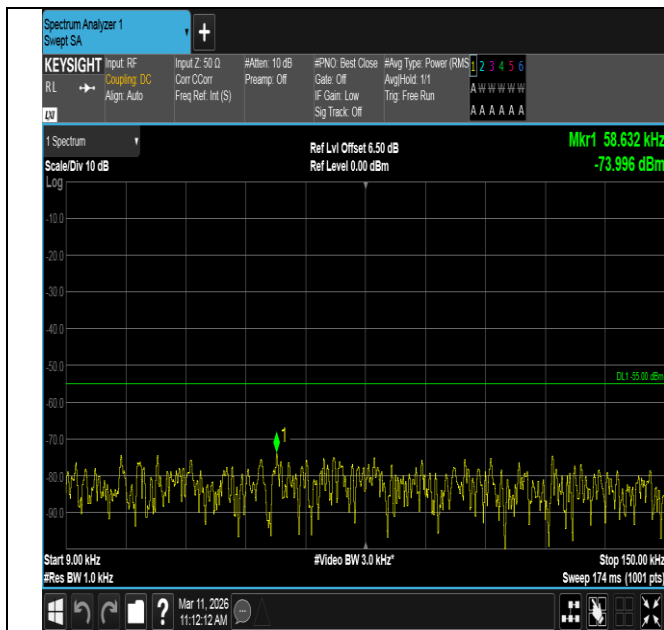
Band7-5MHz-16QAM-21100-25RB#0-0.009~0.15-PASS
