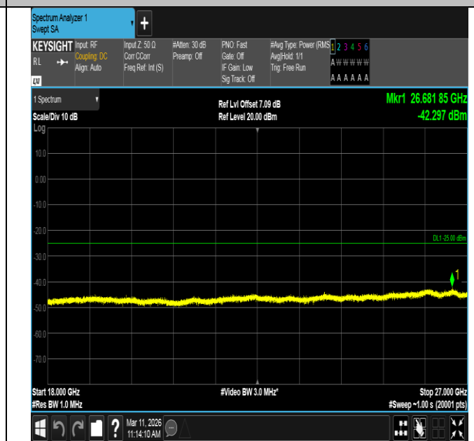
Band7-5MHz-QPSK-21425-1RB#0-18000~27000-PASS
