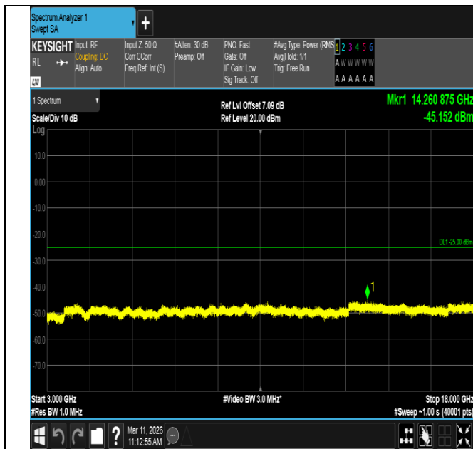
Band7-5MHz-16QAM-21100-25RB#0-3000~18000-PASS
