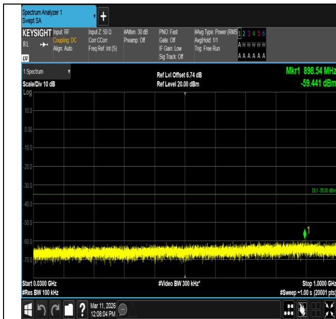
Band7-10MHz-QPSK-20800-1RB#0-30~1000-PASS
