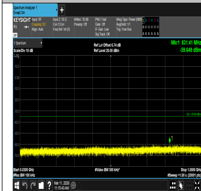
Band7-5MHz-QPSK-21425-1RB#24-30~1000-PASS
