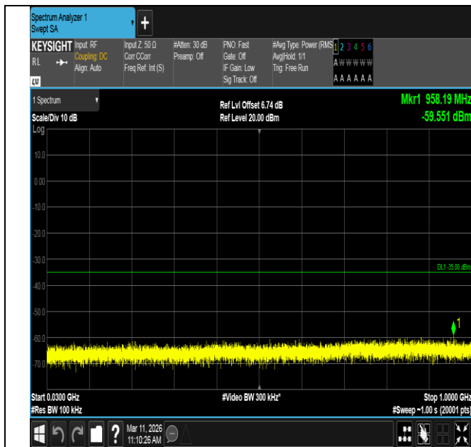
Band7-5MHz-16QAM-21100-1RB#24-30~1000-PASS
