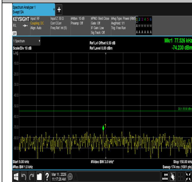
Band7-5MHz-QPSK-21425-25RB#0-0.009~0.15-PASS
