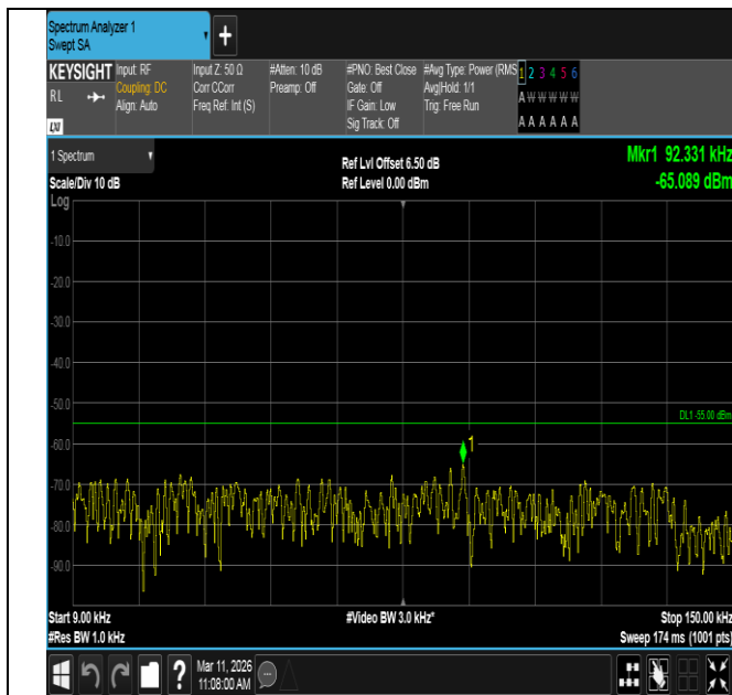
Band7-5MHz-16QAM-21100-1RB#0-0.009~0.15-PASS
