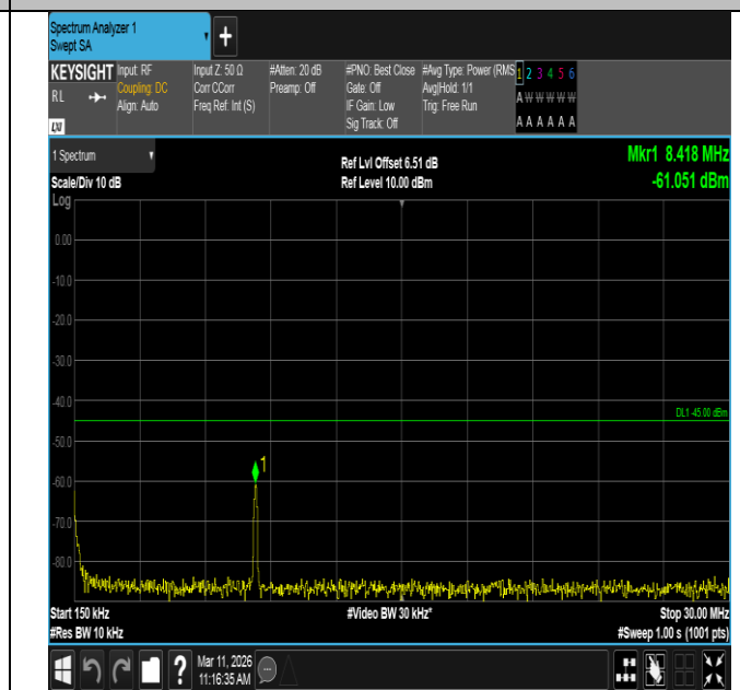
Band7-5MHz-16QAM-21425-1RB#24-0.15~30-PASS
