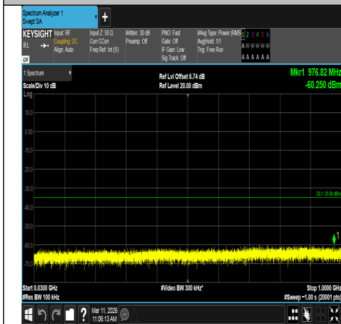
Band7-5MHz-16QAM-20775-25RB#0-30~1000-PASS
