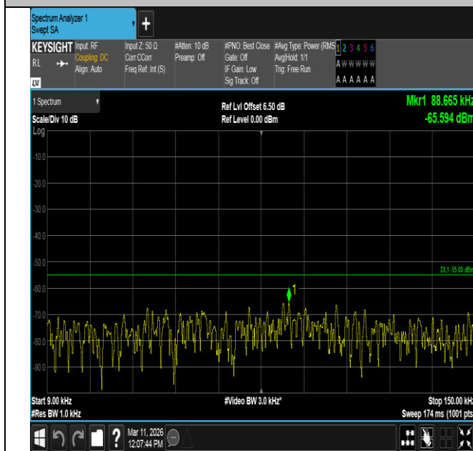
Band7-10MHz-QPSK-20800-1RB#0-0.009~0.15-PASS
