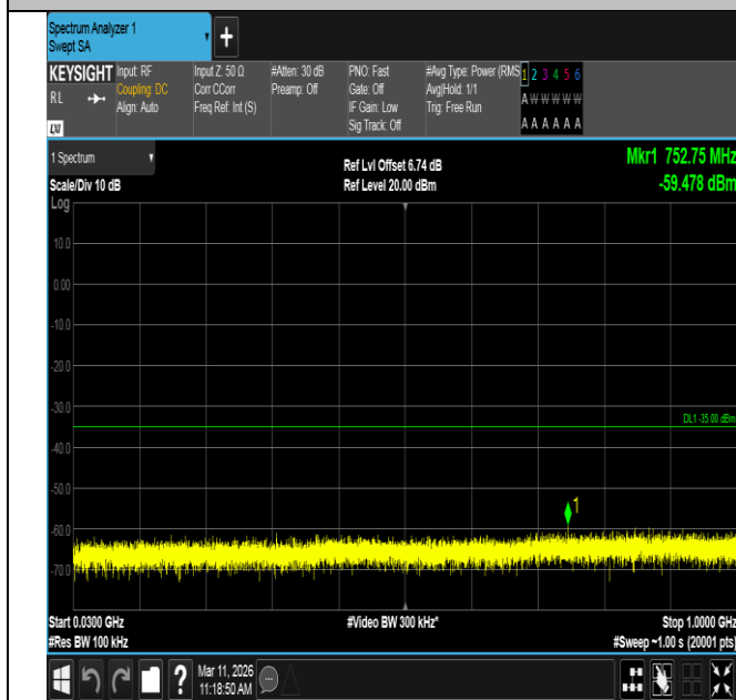
Band7-5MHz-16QAM-21425-25RB#0-30~1000-PASS
