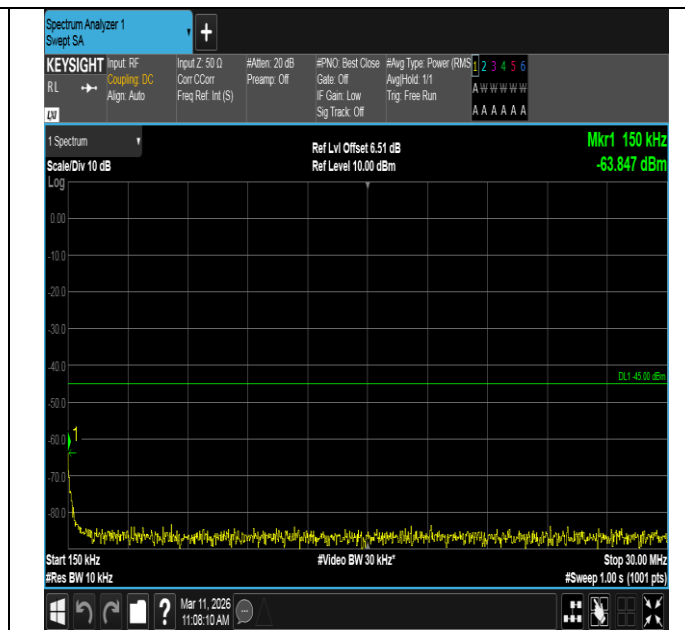
Band7-5MHz-16QAM-21100-1RB#0-0.15~30-PASS
