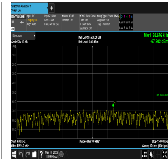
Band7-5MHz-QPSK-21100-1RB#24-0.009~0.15-PASS
