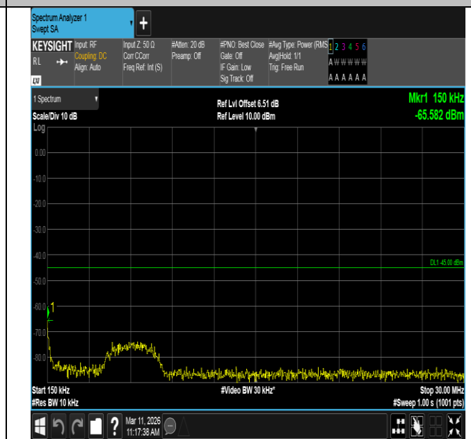
Band7-5MHz-QPSK-21425-25RB#0-0.15~30-PASS
