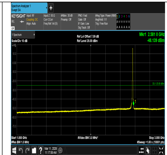
Band7-5MHz-QPSK-21425-25RB#0-1000~3000-PASS
