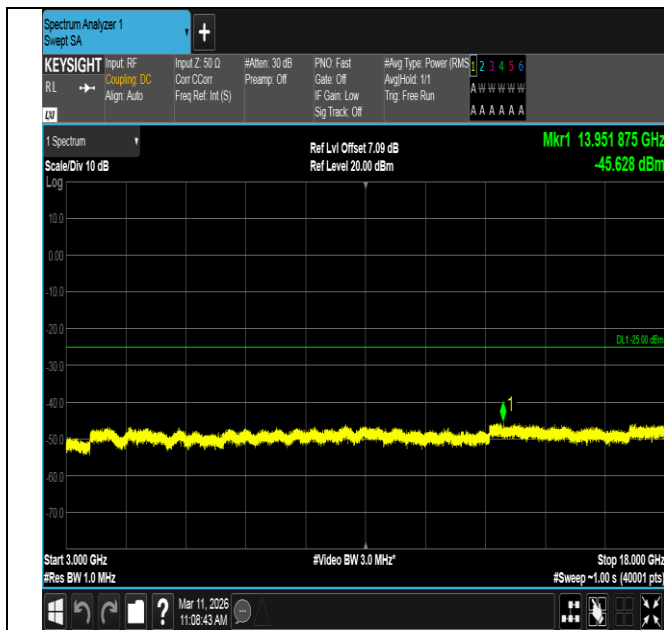
Band7-5MHz-16QAM-21100-1RB#0-3000~18000-PASS
