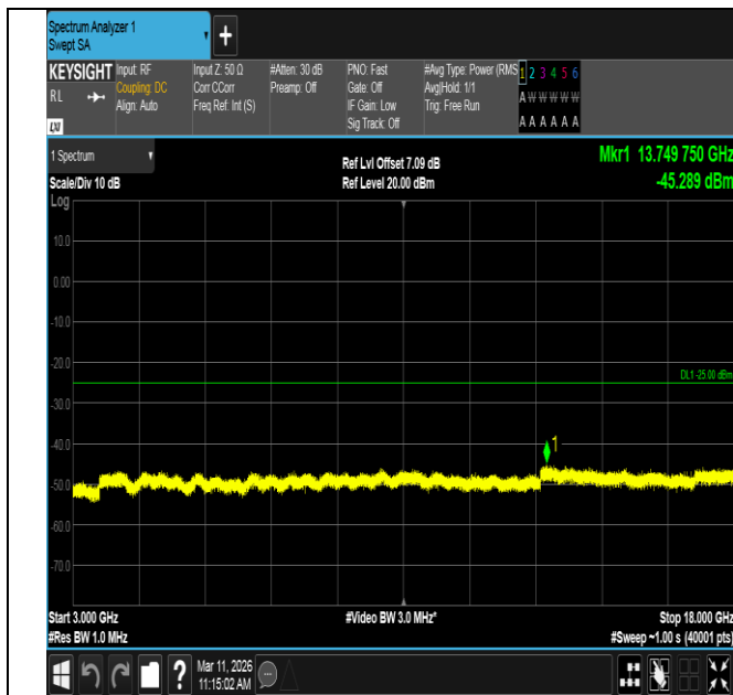
Band7-5MHz-16QAM-21425-1RB#0-3000~18000-PASS
