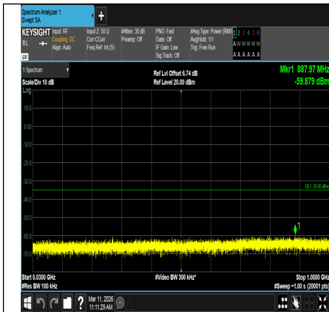
Band7-5MHz-QPSK-21100-25RB#0-30~1000-PASS
