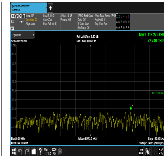
Band7-5MHz-16QAM-21425-25RB#0-0.009~0.15-PASS
