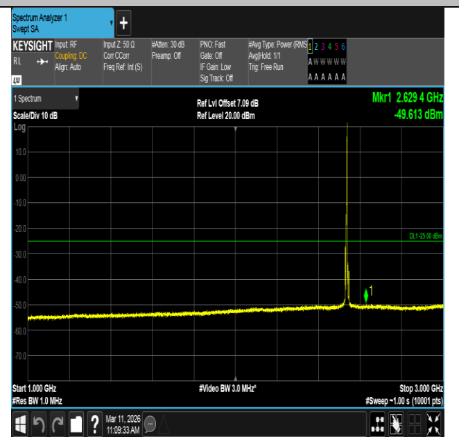
Band7-5MHz-QPSK-21100-1RB#24-1000~3000-PASS
