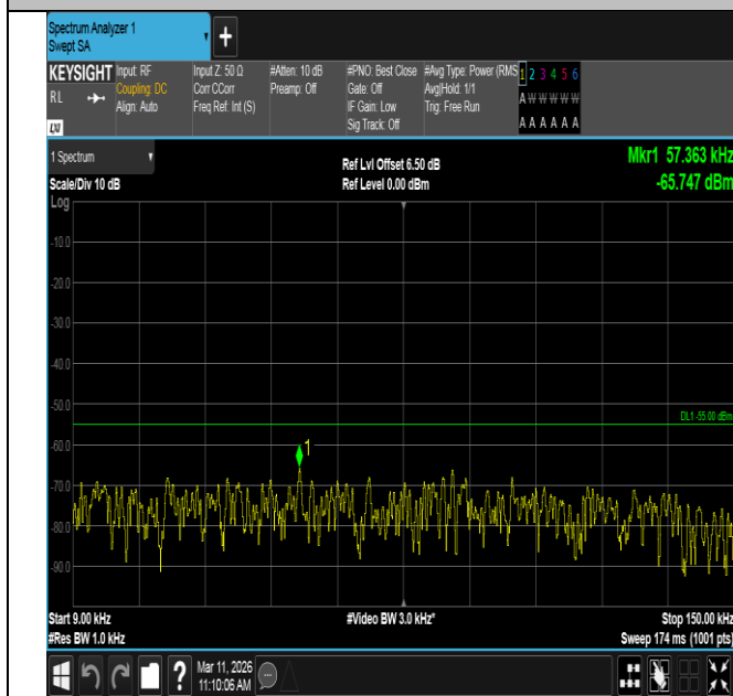
Band7-5MHz-16QAM-21100-1RB#24-0.009~0.15-PASS
