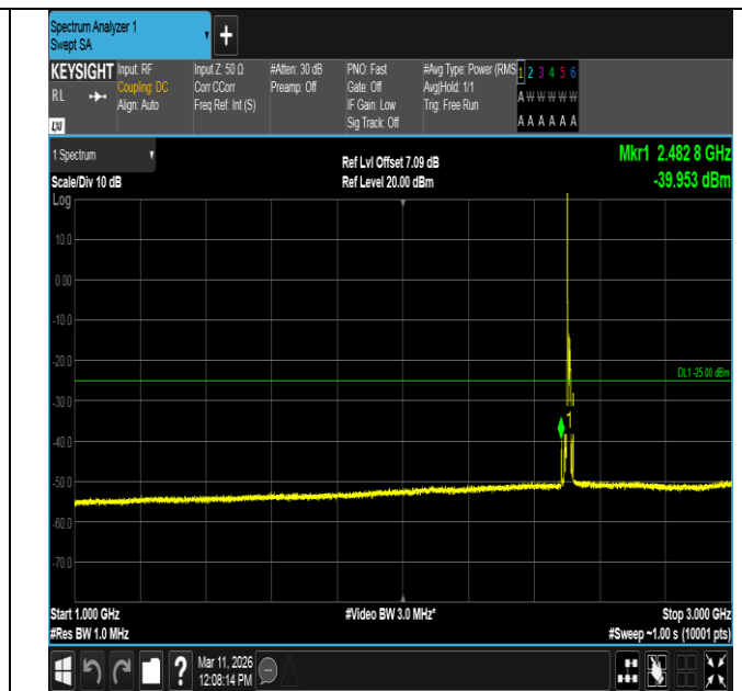
Band7-10MHz-QPSK-20800-1RB#0-1000~3000-PASS
