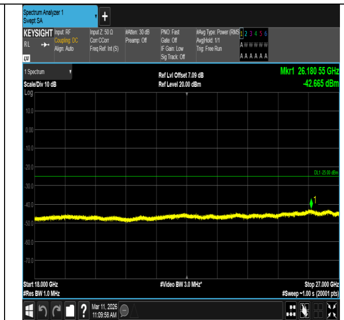
Band7-5MHz-QPSK-21100-1RB#24-18000~27000-PASS
