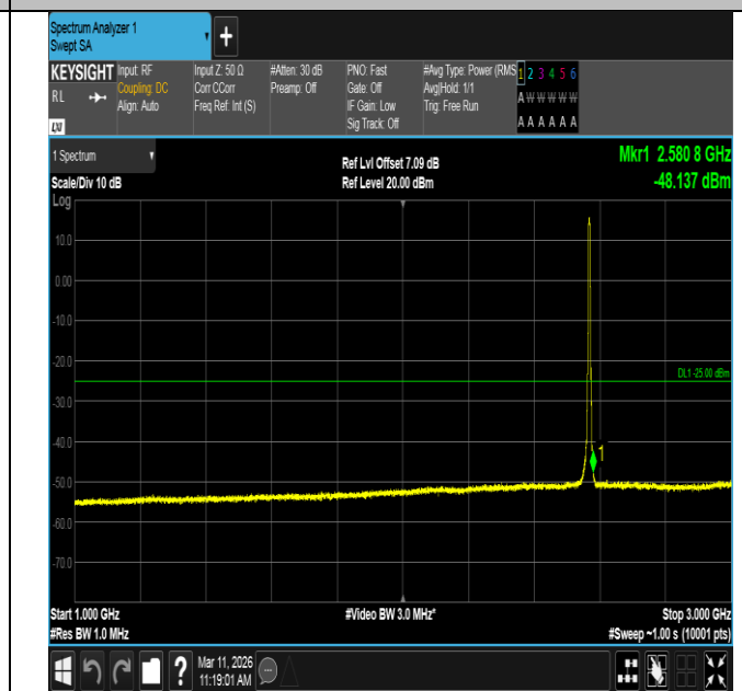
Band7-5MHz-16QAM-21425-25RB#0-1000~3000-PASS
