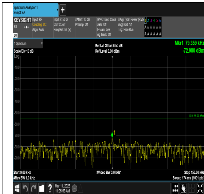
Band7-5MHz-16QAM-20775-25RB#0-0.009~0.15-PASS
