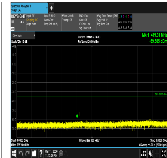
Band7-5MHz-QPSK-21425-1RB#0-30~1000-PASS
