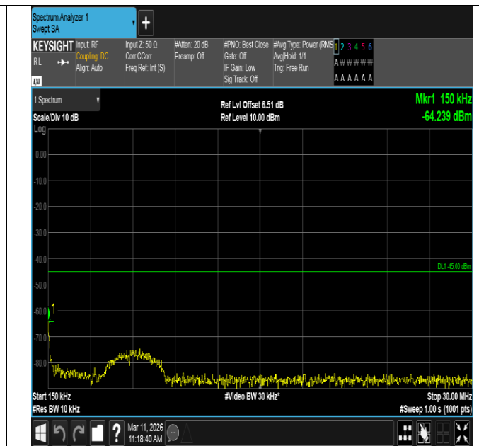
Band7-5MHz-16QAM-21425-25RB#0-0.15~30-PASS
