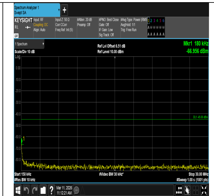
Band7-5MHz-16QAM-21100-25RB#0-0.15~30-PASS
