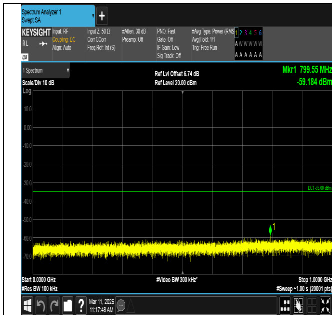
Band7-5MHz-QPSK-21425-25RB#0-30~1000-PASS
