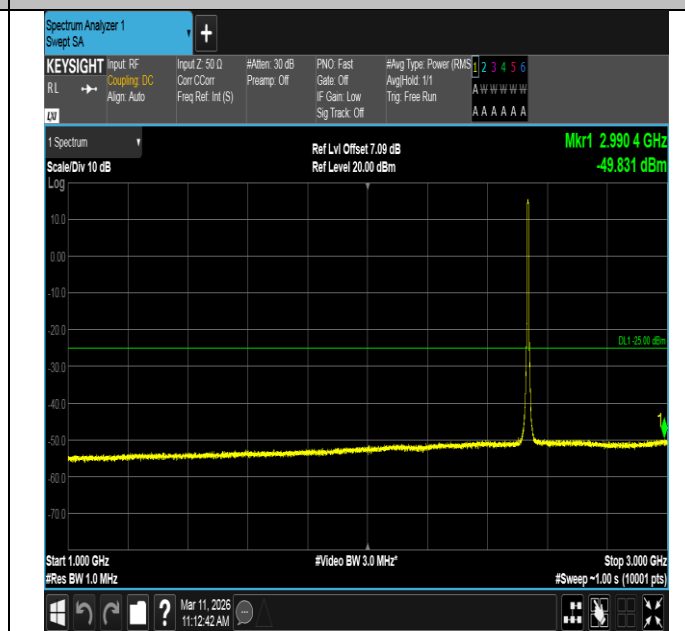
Band7-5MHz-16QAM-21100-25RB#0-1000~3000-PASS
