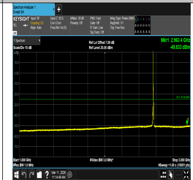
Band7-5MHz-16QAM-21425-1RB#0-1000~3000-PASS
