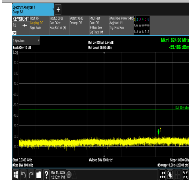
Band7-10MHz-QPSK-20800-1RB#49-30~1000-PASS
