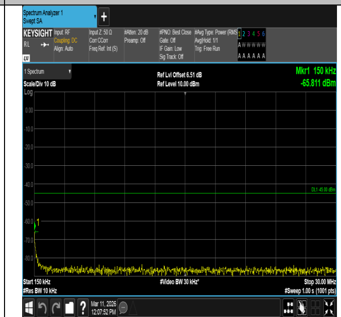
Band7-10MHz-QPSK-20800-1RB#0-0.15~30-PASS
