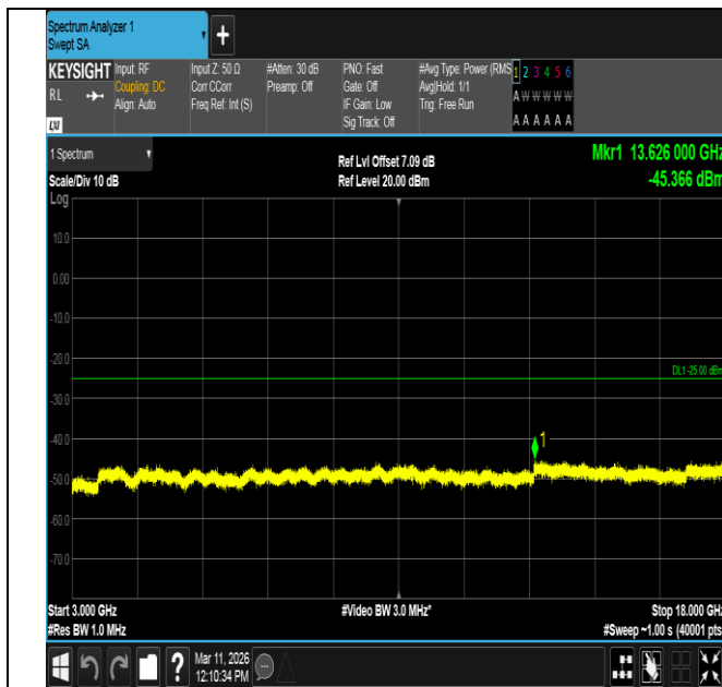
Band7-10MHz-QPSK-20800-1RB#49-3000~18000-PASS
