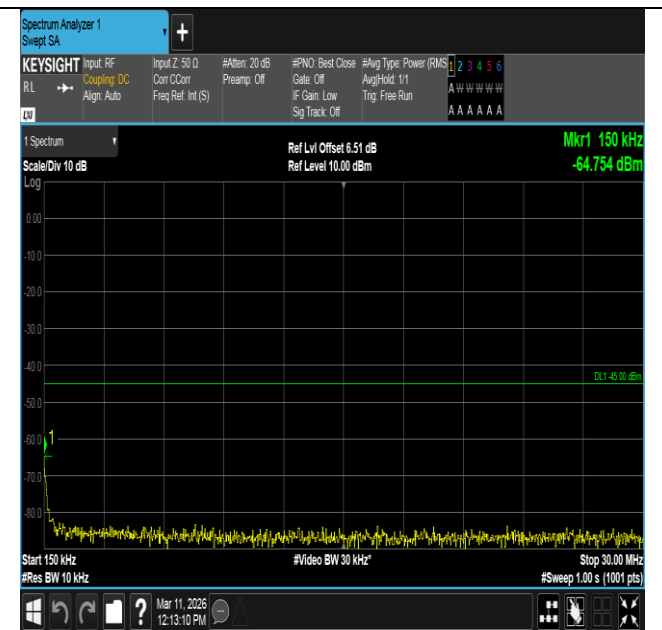
Band7-10MHz-16QAM-20800-50RB#0-0.15~30-PASS
