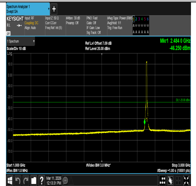
Band7-10MHz-16QAM-20800-50RB#0-1000~3000-PASS
