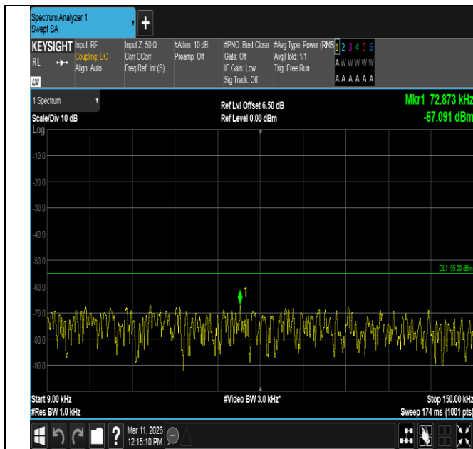
Band7-10MHz-16QAM-21100-1RB#0-0.009~0.15-PASS
