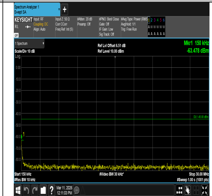
Band7-10MHz-16QAM-20800-1RB#49-0.15~30-PASS
