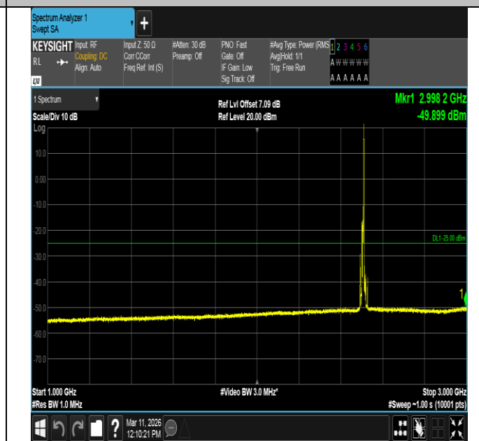
Band7-10MHz-QPSK-20800-1RB#49-1000~3000-PASS
