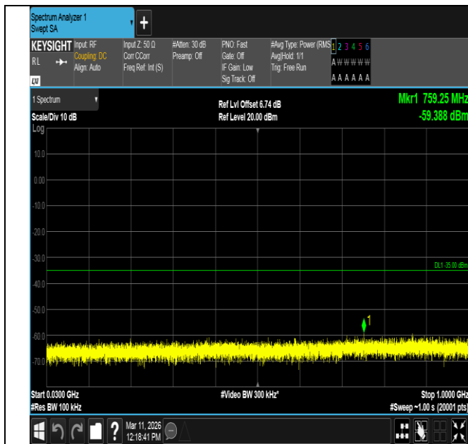
Band7-10MHz-QPSK-21100-50RB#0-30~1000-PASS
