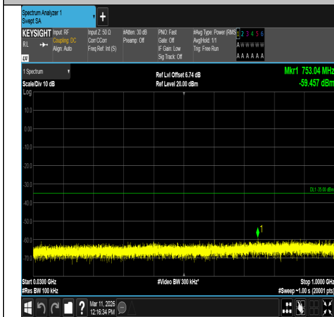
Band7-10MHz-QPSK-21100-1RB#49-30~1000-PASS
