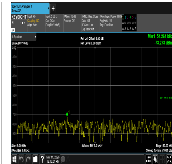
Band7-10MHz-16QAM-20800-50RB#0-0.009~0.15-PASS
