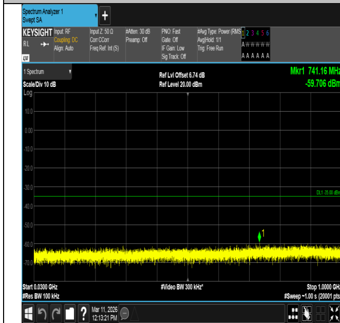
Band7-10MHz-16QAM-20800-50RB#0-30~1000-PASS
