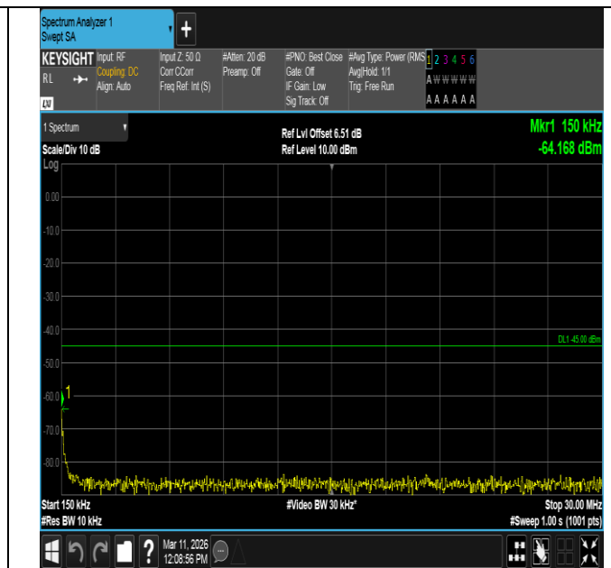
Band7-10MHz-16QAM-20800-1RB#0-0.15~30-PASS
