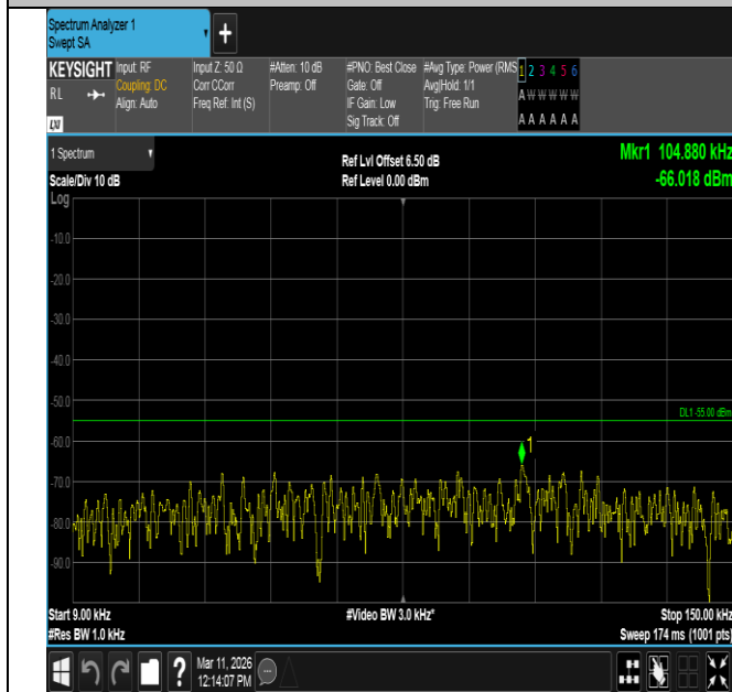
Band7-10MHz-QPSK-21100-1RB#0-0.009~0.15-PASS
