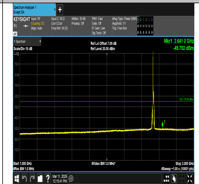
Band7-10MHz-16QAM-21100-1RB#0-1000~3000-PASS
