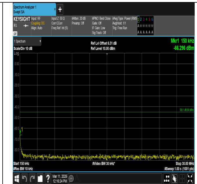
Band7-10MHz-QPSK-21100-1RB#49-0.15~30-PASS
