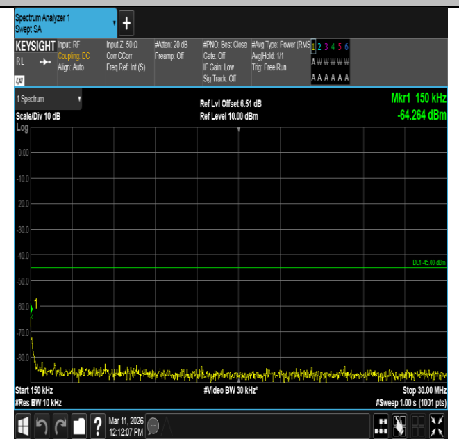
Band7-10MHz-QPSK-20800-50RB#0-0.15~30-PASS
