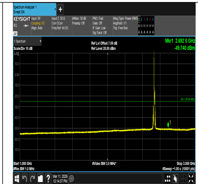
Band7-10MHz-QPSK-21100-1RB#0-1000~3000-PASS
