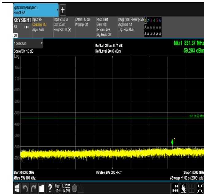
Band7-10MHz-16QAM-20800-1RB#49-30~1000-PASS
