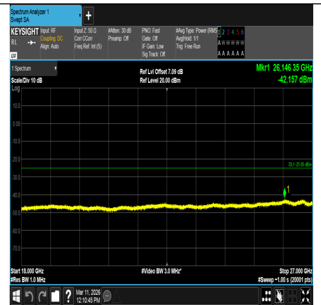
Band7-10MHz-QPSK-20800-1RB#49-18000~27000-PASS
