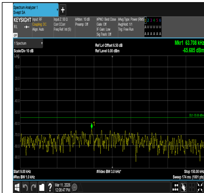
Band7-10MHz-16QAM-20800-1RB#0-0.009~0.15-PASS
