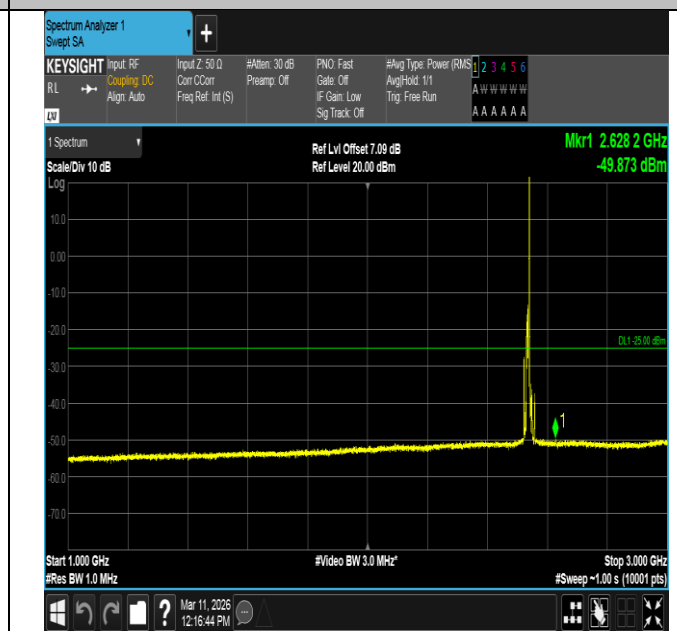
Band7-10MHz-QPSK-21100-1RB#49-1000~3000-PASS
