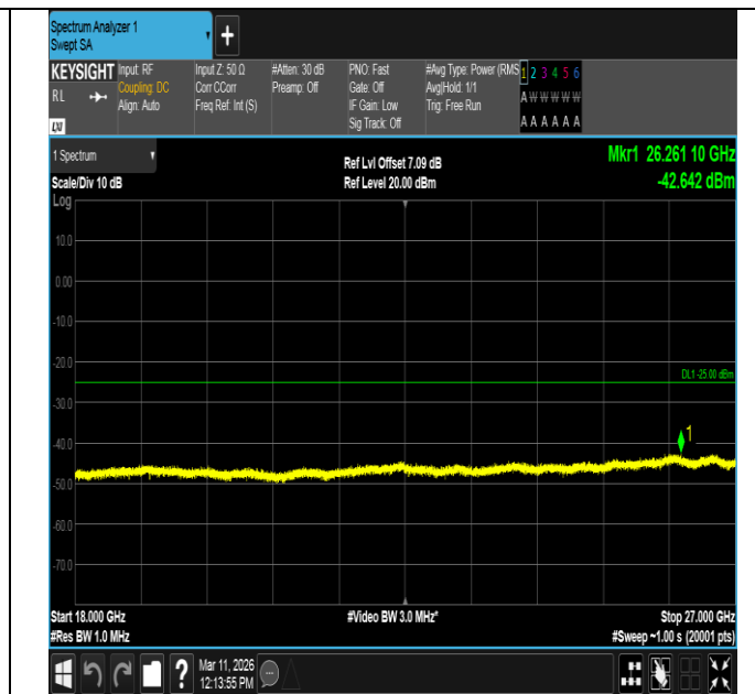
Band7-10MHz-16QAM-20800-50RB#0-18000~27000-PASS
