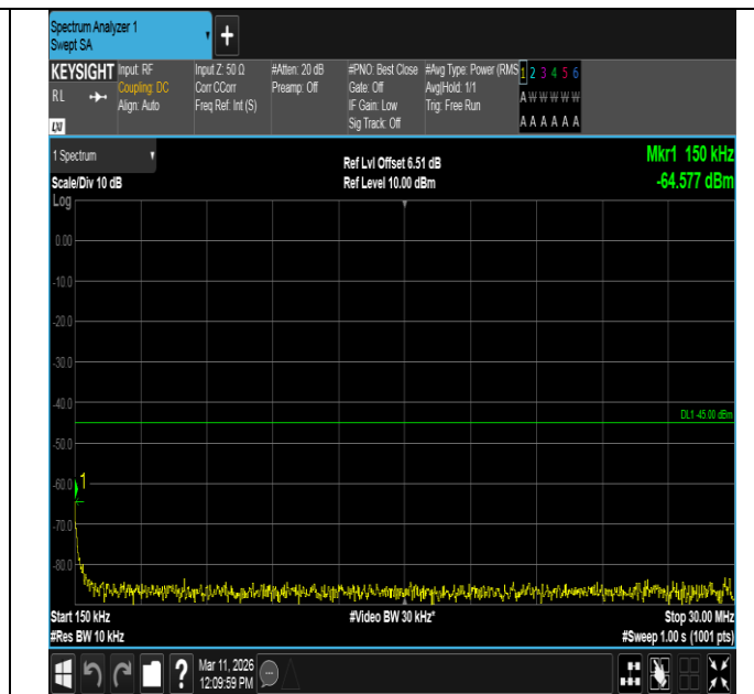
Band7-10MHz-QPSK-20800-1RB#49-0.15~30-PASS
