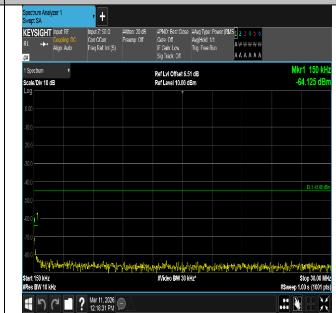
Band7-10MHz-QPSK-21100-50RB#0-0.15~30-PASS
