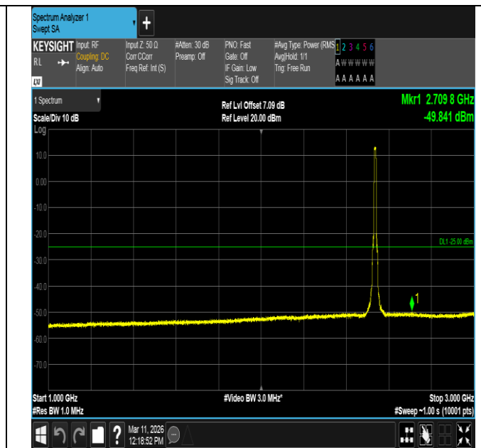
Band7-10MHz-QPSK-21100-50RB#0-1000~3000-PASS
