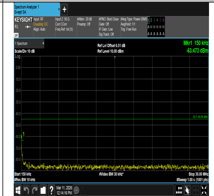
Band7-10MHz-QPSK-21100-1RB#0-0.15~30-PASS
