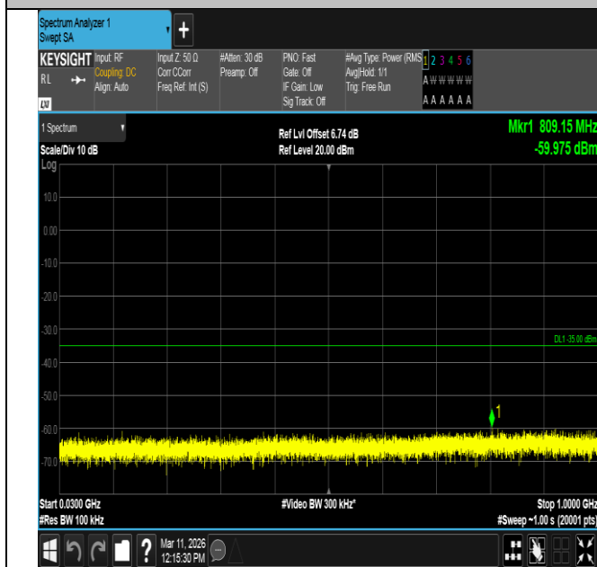
Band7-10MHz-16QAM-21100-1RB#0-30~1000-PASS
