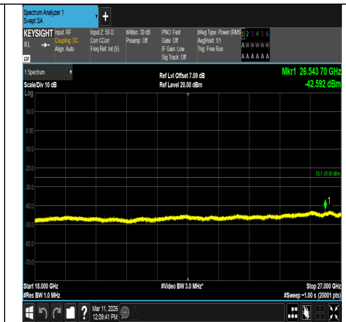
Band7-10MHz-16QAM-20800-1RB#0-18000~27000-PASS
