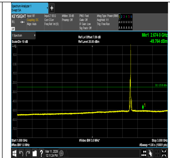
Band7-10MHz-16QAM-20800-1RB#49-1000~3000-PASS
