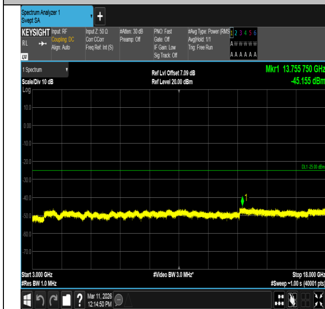
Band7-10MHz-QPSK-21100-1RB#0-3000~18000-PASS
