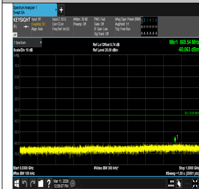
Band7-10MHz-16QAM-20800-1RB#0-30~1000-PASS
