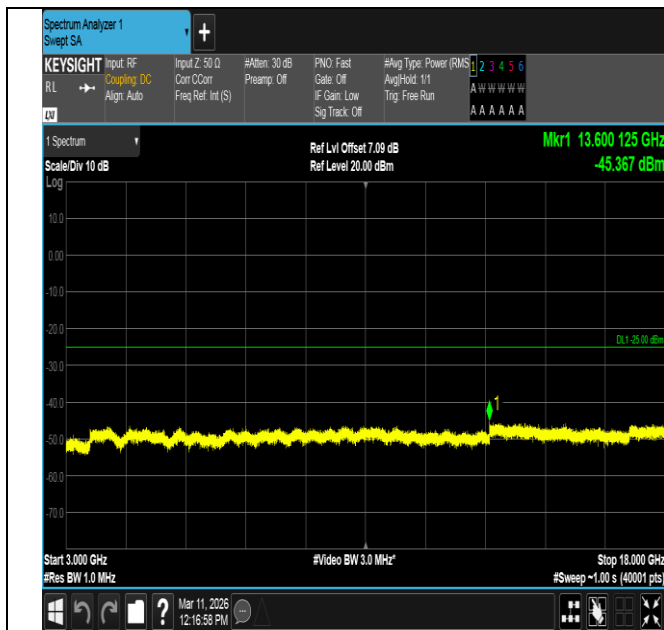
Band7-10MHz-QPSK-21100-1RB#49-3000~18000-PASS
