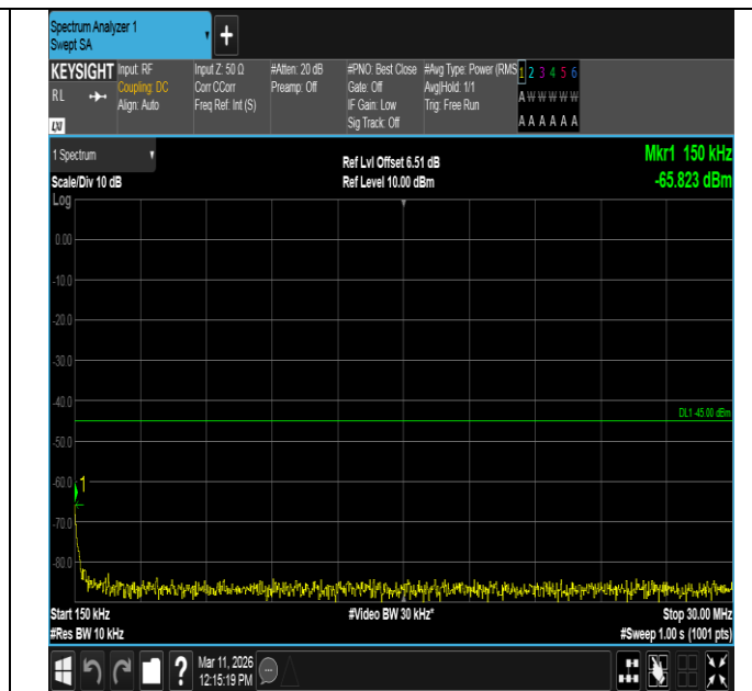
Band7-10MHz-16QAM-21100-1RB#0-0.15~30-PASS
