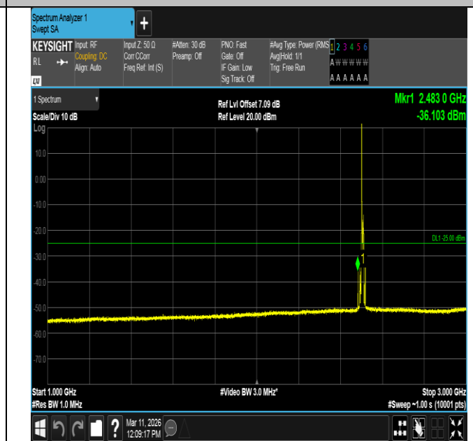
Band7-10MHz-16QAM-20800-1RB#0-1000~3000-PASS
