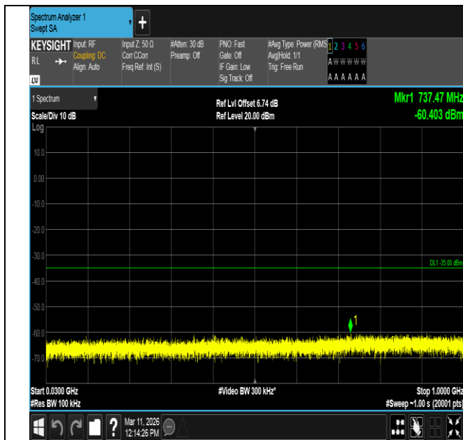
Band7-10MHz-QPSK-21100-1RB#0-30~1000-PASS
