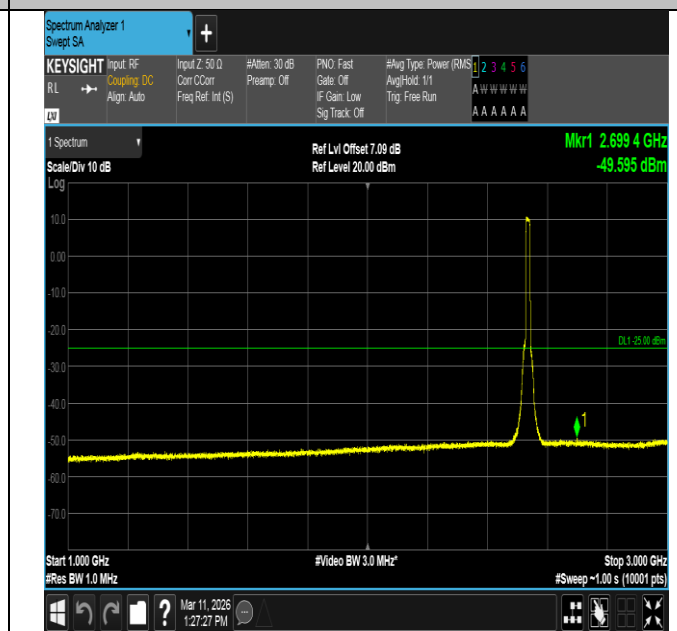
Band7-15MHz-16QAM-21100-75RB#0-1000~3000-PASS
