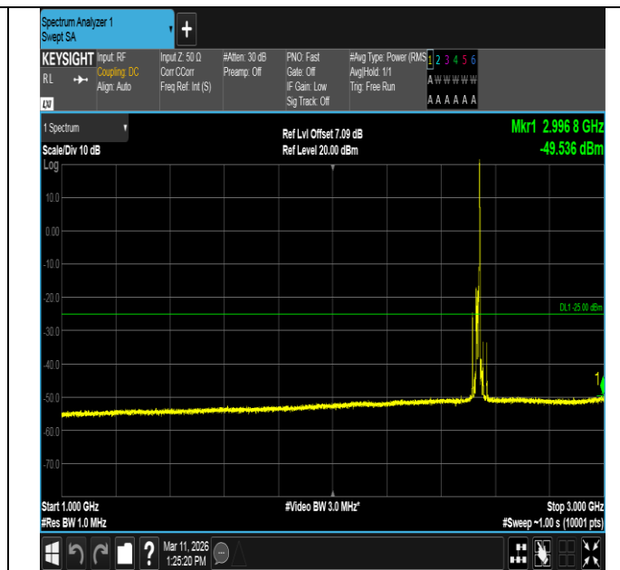
Band7-15MHz-16QAM-21100-1RB#74-1000~3000-PASS
