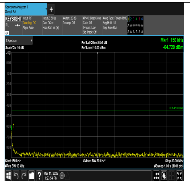
Band7-15MHz-QPSK-21100-1RB#74-0.15~30-PASS
