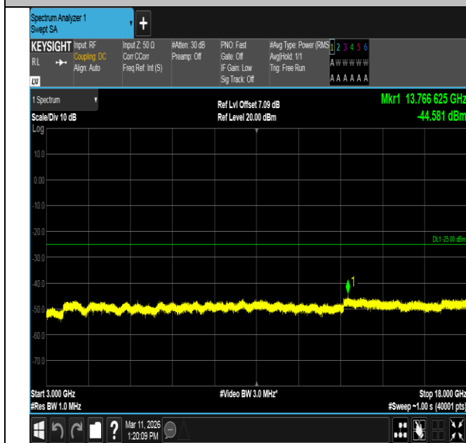
Band7-15MHz-QPSK-20825-75RB#0-3000~18000-PASS
