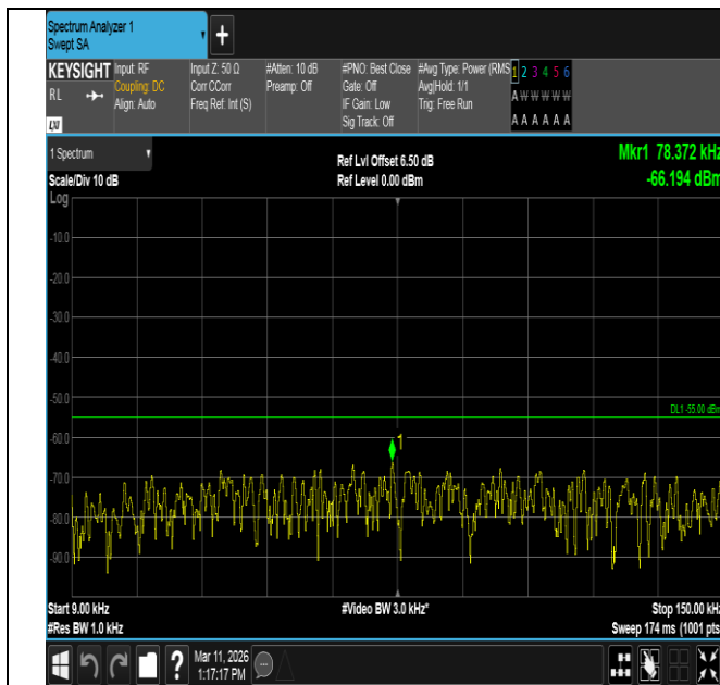
Band7-15MHz-QPSK-20825-1RB#74-0.009~0.15-PASS
