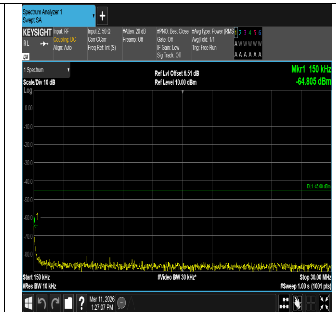
Band7-15MHz-16QAM-21100-75RB#0-0.15~30-PASS
