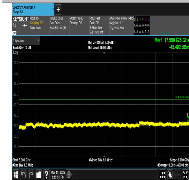
Band7-15MHz-QPSK-20825-1RB#0-3000~18000-PASS
