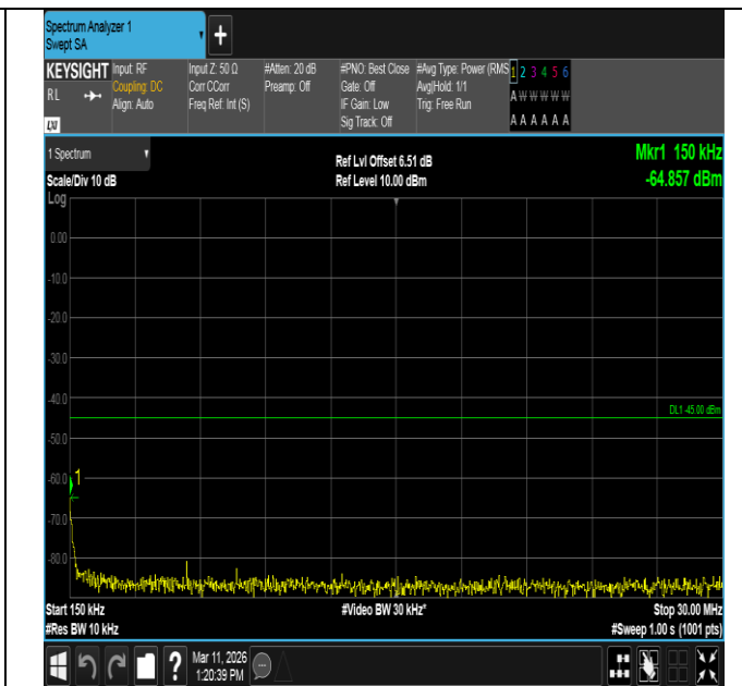
Band7-15MHz-16QAM-20825-75RB#0-0.15~30-PASS
