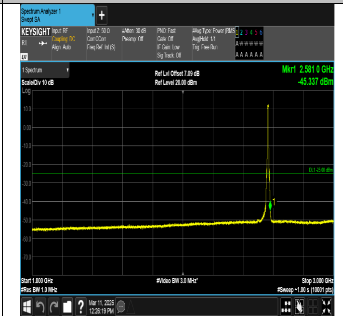
Band7-10MHz-16QAM-21400-50RB#0-1000~3000-PASS
