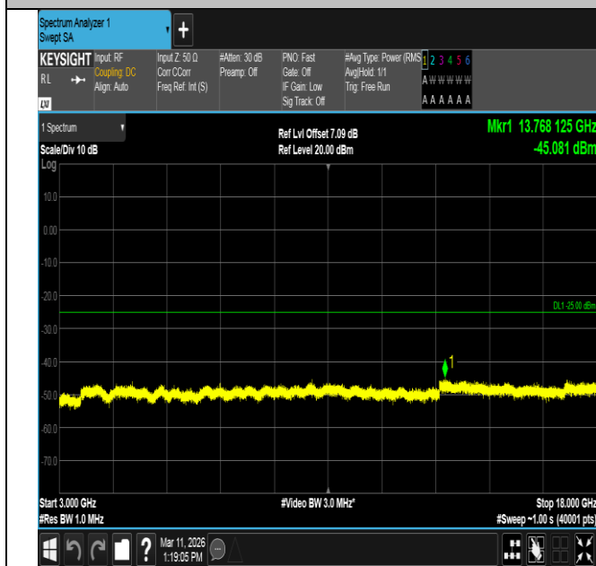
Band7-15MHz-16QAM-20825-1RB#74-3000~18000-PASS
