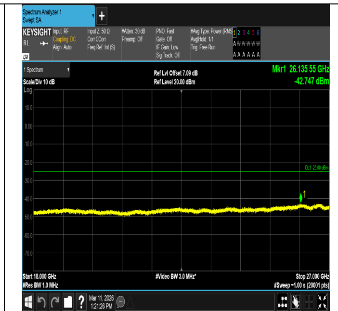
Band7-15MHz-16QAM-20825-75RB#0-18000~27000-PASS
