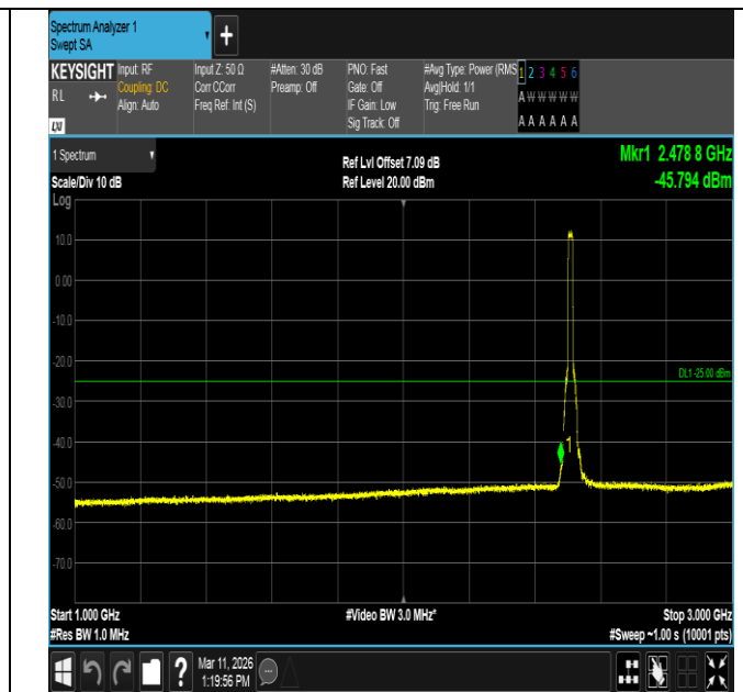
Band7-15MHz-QPSK-20825-75RB#0-1000~3000-PASS
