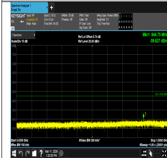
Band7-15MHz-16QAM-20825-75RB#0-30~1000-PASS
