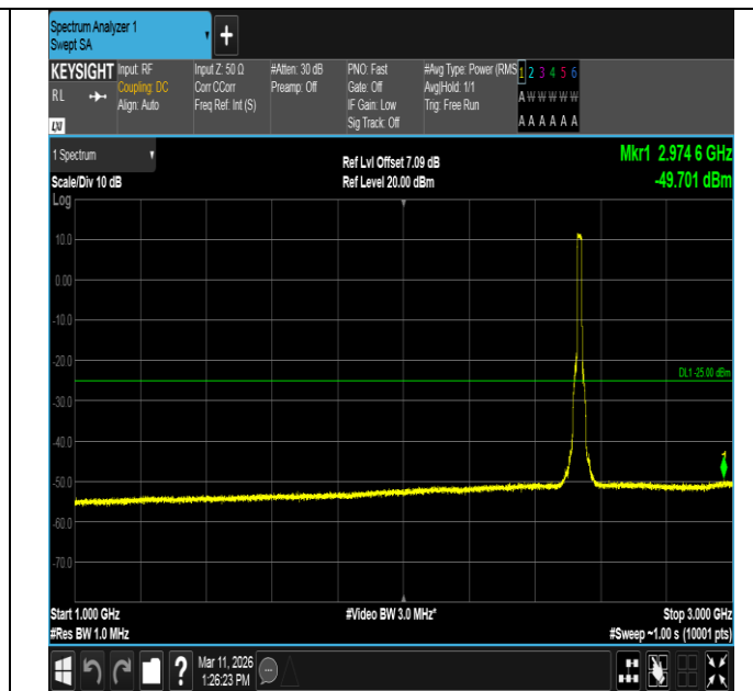
Band7-15MHz-QPSK-21100-75RB#0-1000~3000-PASS
