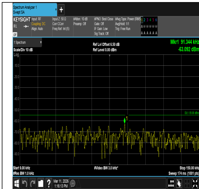
Band7-15MHz-16QAM-20825-1RB#0-0.009~0.15-PASS
