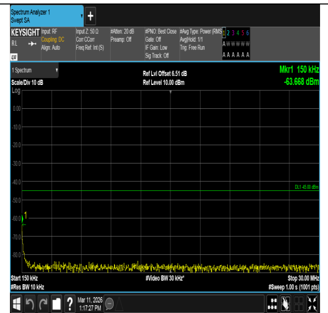
Band7-15MHz-QPSK-20825-1RB#74-0.15~30-PASS
