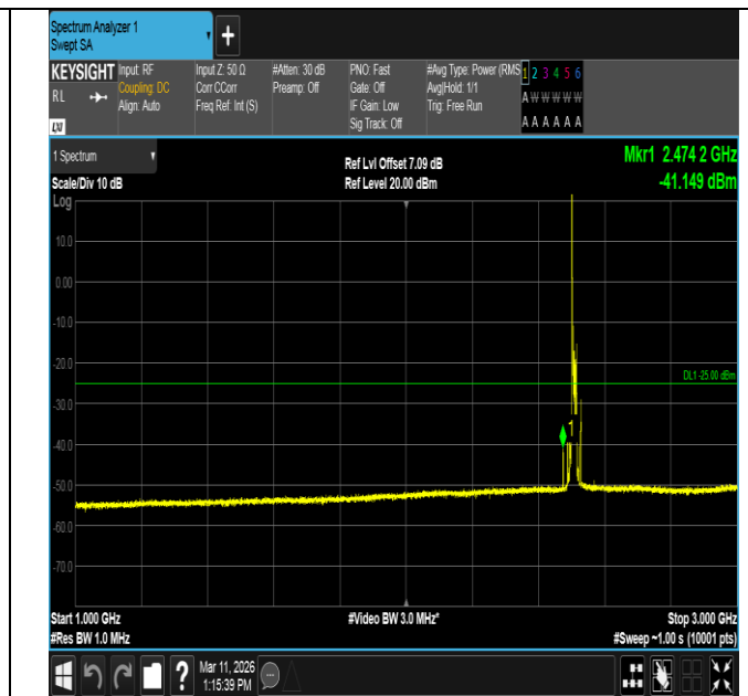
Band7-15MHz-QPSK-20825-1RB#0-1000~3000-PASS
