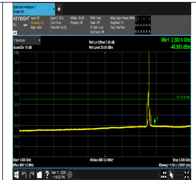
Band7-15MHz-16QAM-20825-1RB#74-1000~3000-PASS
