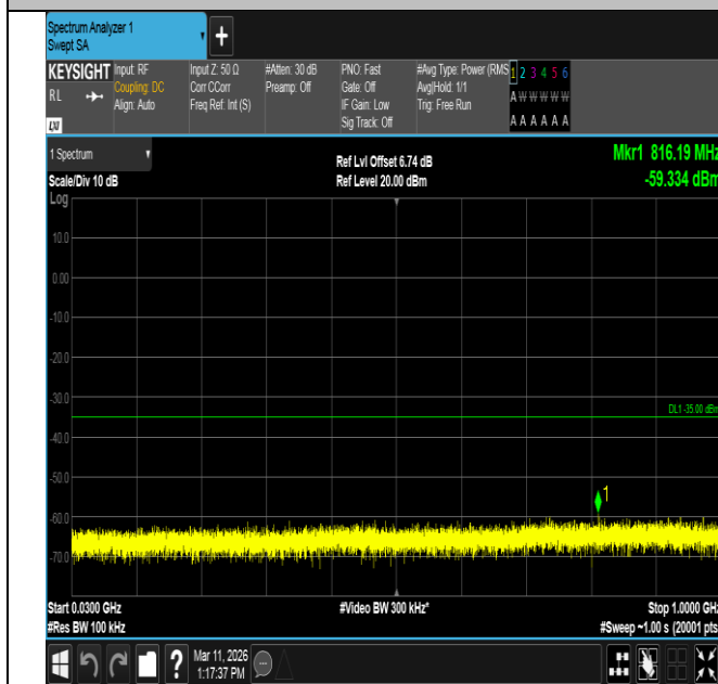
Band7-15MHz-QPSK-20825-1RB#74-30~1000-PASS
