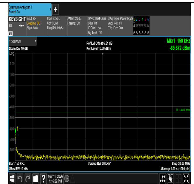
Band7-15MHz-16QAM-20825-1RB#0-0.15~30-PASS
