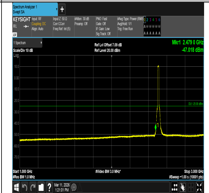
Band7-15MHz-16QAM-20825-75RB#0-1000~3000-PASS
