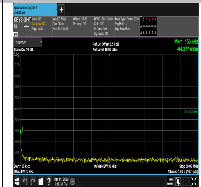
Band7-15MHz-16QAM-20825-1RB#74-0.15~30-PASS
