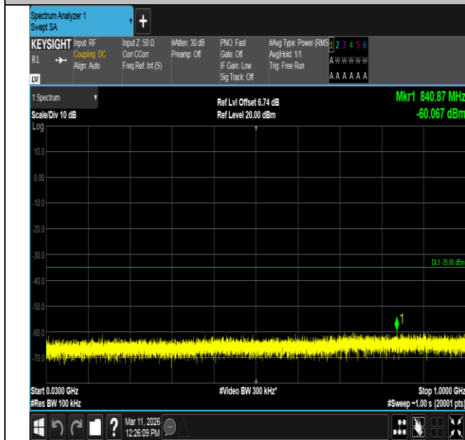
Band7-10MHz-16QAM-21400-50RB#0-30~1000-PASS
