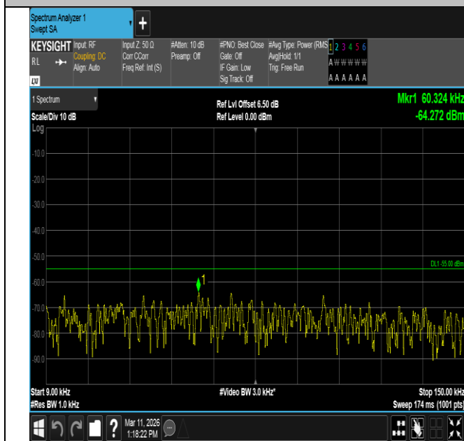
Band7-15MHz-16QAM-20825-1RB#74-0.009~0.15-PASS
