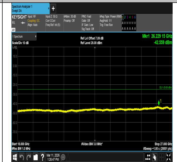
Band7-15MHz-QPSK-21100-75RB#0-18000~27000-PASS
