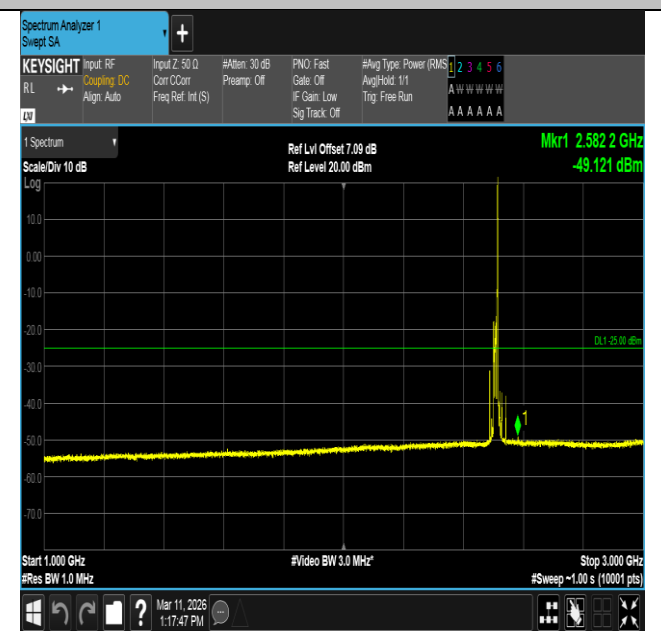
Band7-15MHz-QPSK-20825-1RB#74-1000~3000-PASS
