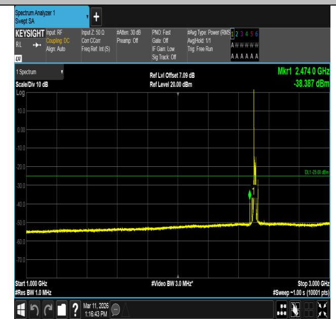
Band7-15MHz-16QAM-20825-1RB#0-1000~3000-PASS
