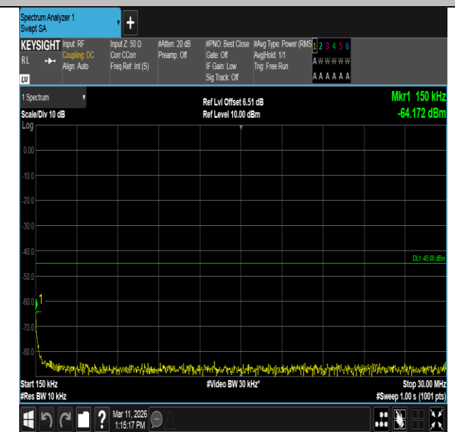
Band7-15MHz-QPSK-20825-1RB#0-0.15~30-PASS
