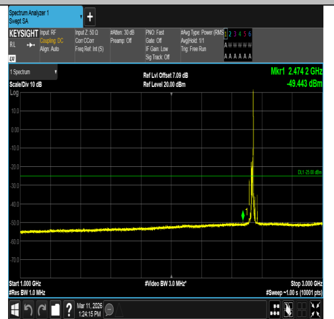
Band7-15MHz-QPSK-21100-1RB#74-1000~3000-PASS
