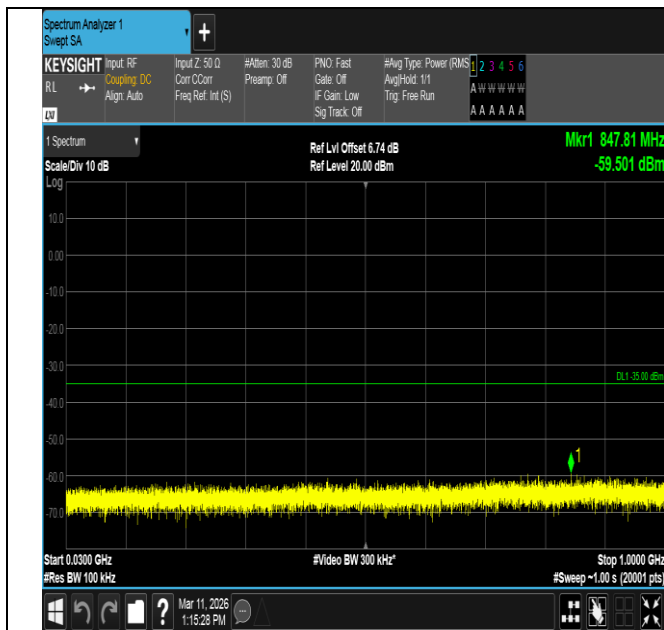
Band7-15MHz-QPSK-20825-1RB#0-30~1000-PASS
