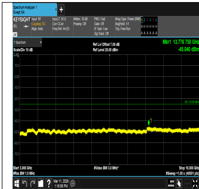
Band7-15MHz-16QAM-20825-1RB#0-3000~18000-PASS
