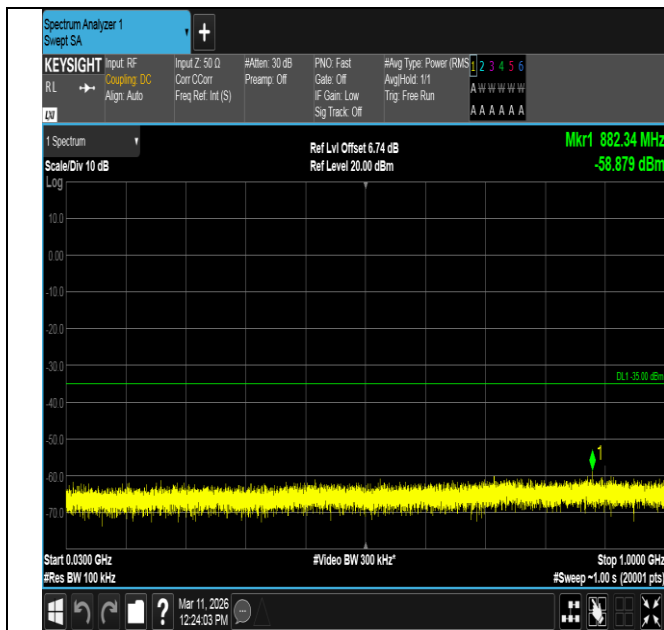
Band7-10MHz-16QAM-21400-1RB#49-30~1000-PASS
