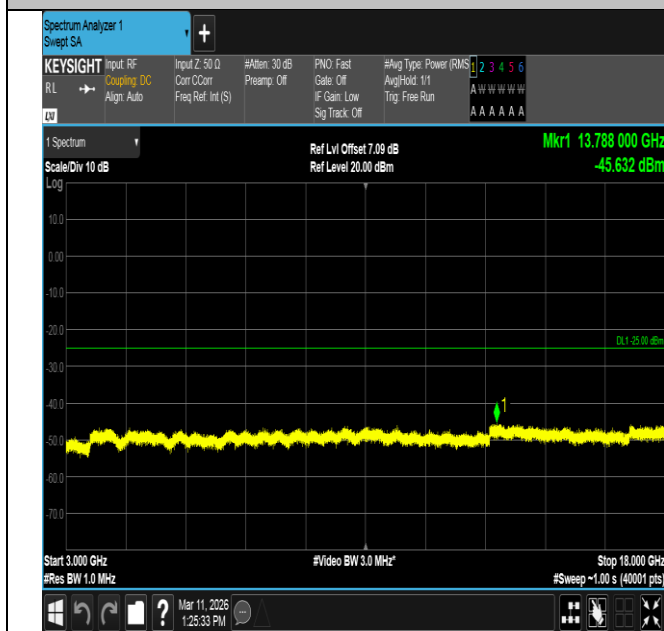
Band7-15MHz-16QAM-21100-1RB#74-3000~18000-PASS
