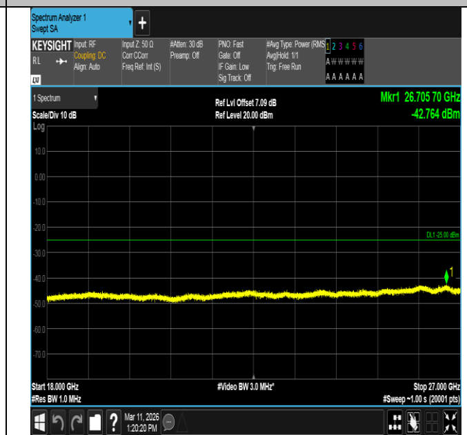
Band7-15MHz-QPSK-20825-75RB#0-18000~27000-PASS
