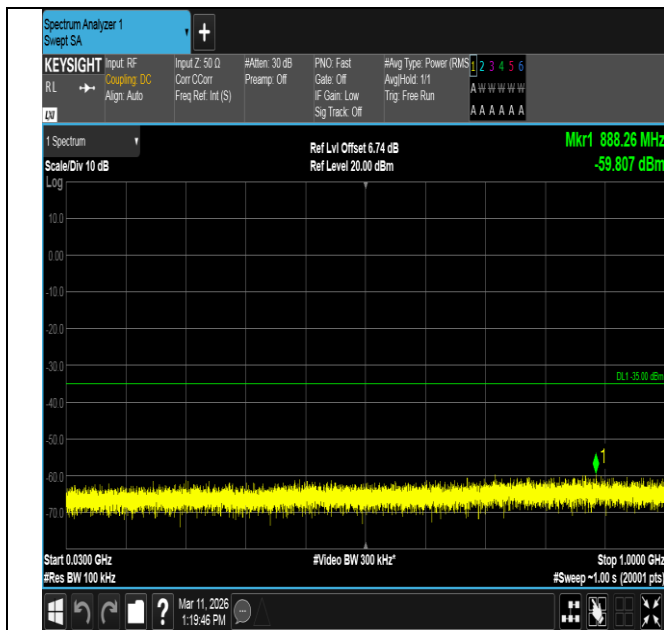
Band7-15MHz-QPSK-20825-75RB#0-30~1000-PASS
