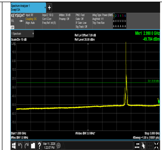
Band7-15MHz-QPSK-21100-1RB#0-1000~3000-PASS
