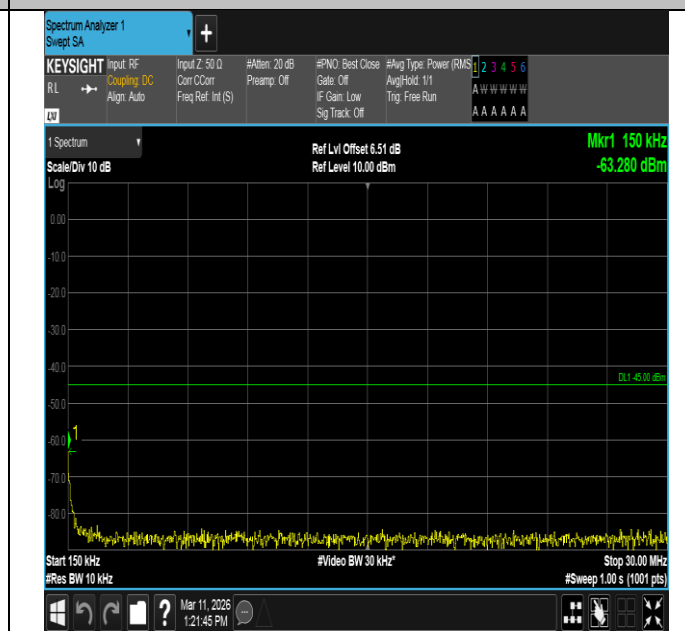
Band7-15MHz-QPSK-21100-1RB#0-0.15~30-PASS
