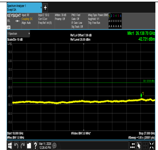
Band7-10MHz-16QAM-21400-50RB#0-18000~27000-PASS
