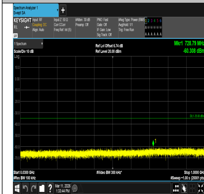
Band7-15MHz-16QAM-21375-75RB#0-30~1000-PASS
