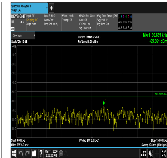
Band7-20MHz-QPSK-20850-1RB#99-0.009~0.15-PASS
