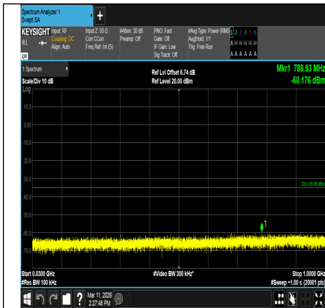
Band7-20MHz-QPSK-20850-100RB#0-30~1000-PASS
