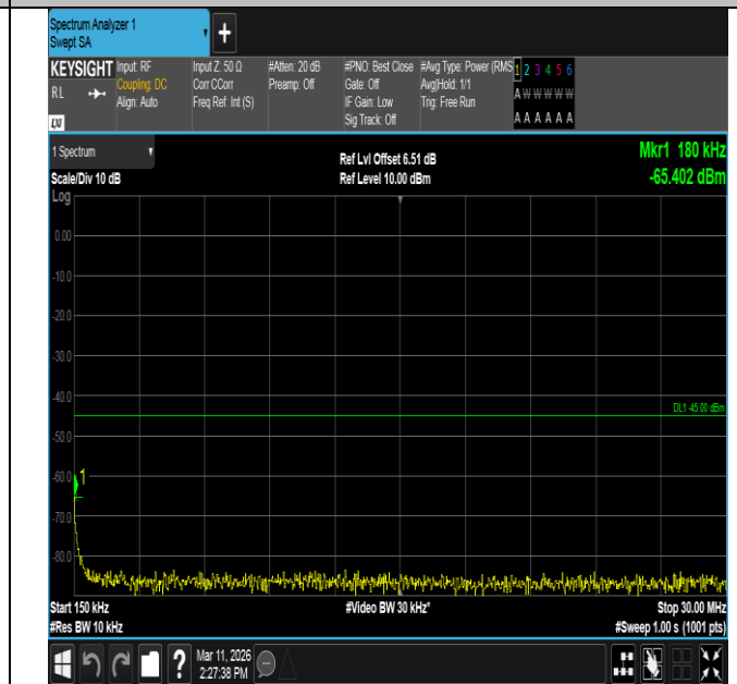
Band7-20MHz-QPSK-20850-100RB#0-0.15~30-PASS
