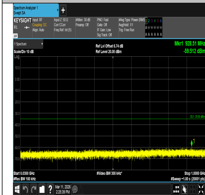
Band7-20MHz-QPSK-20850-1RB#99-30~1000-PASS
