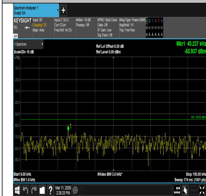
Band7-20MHz-16QAM-20850-1RB#99-0.009~0.15-PASS
