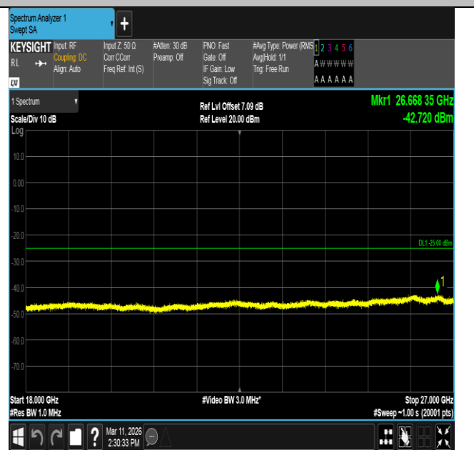
Band7-20MHz-QPSK-21100-1RB#0-18000~27000-PASS
