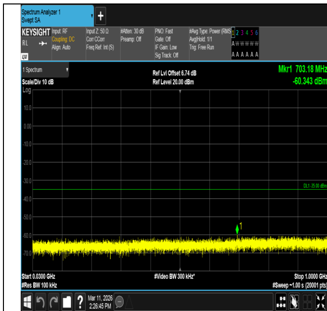
Band7-20MHz-16QAM-20850-1RB#99-30~1000-PASS
