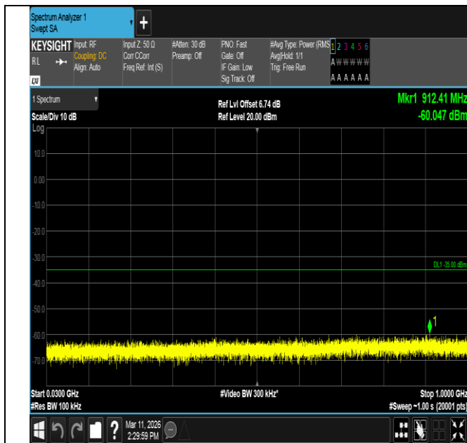
Band7-20MHz-QPSK-21100-1RB#0-30~1000-PASS
