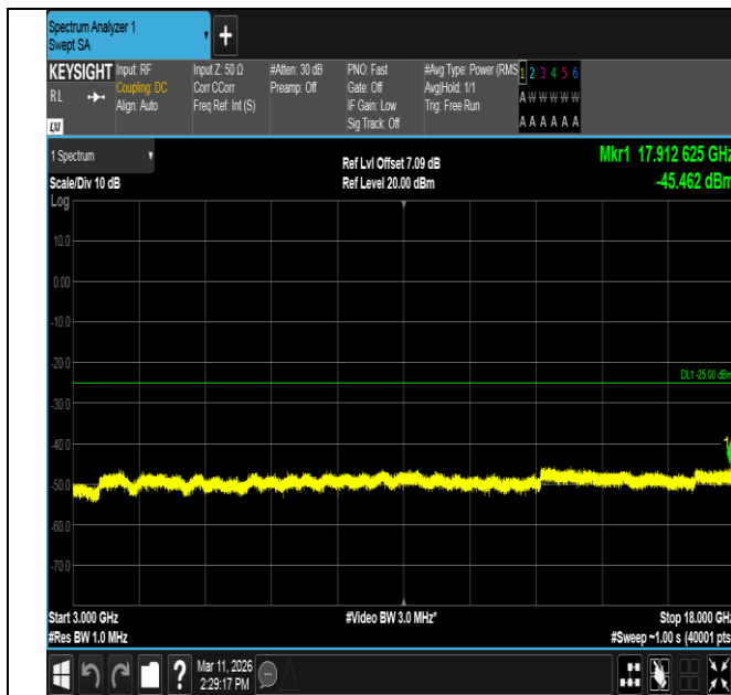
Band7-20MHz-16QAM-20850-100RB#0-3000~18000-PASS
