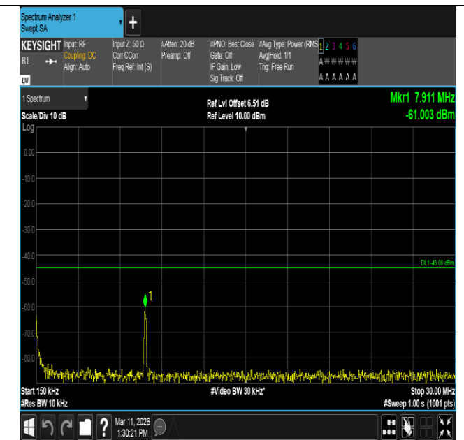
Band7-15MHz-QPSK-21375-1RB#74-0.15~30-PASS
