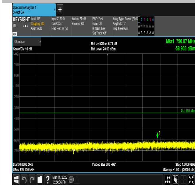
Band7-20MHz-16QAM-20850-1RB#0-30~1000-PASS
