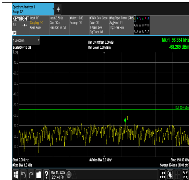
Band7-20MHz-QPSK-21100-1RB#99-0.009~0.15-PASS
