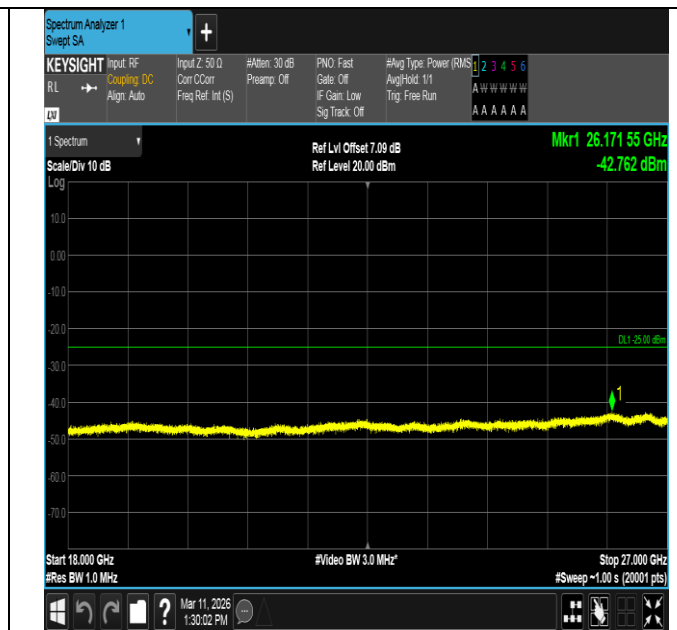
Band7-15MHz-16QAM-21375-1RB#0-18000~27000-PASS
