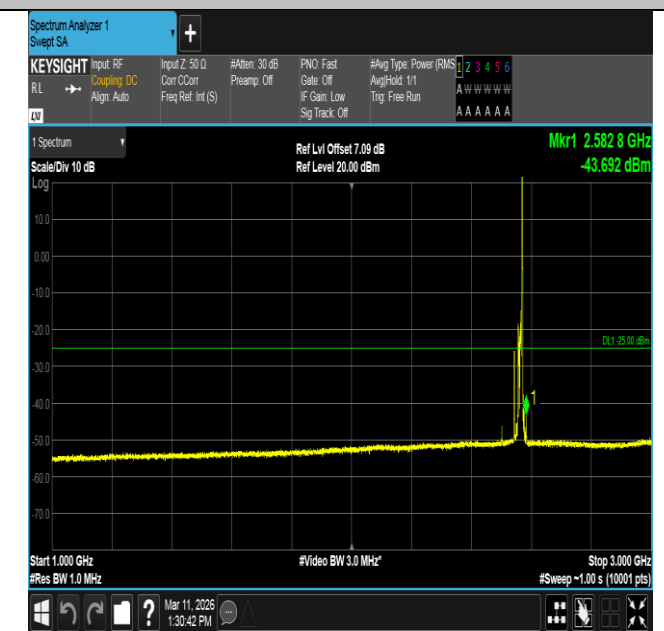
Band7-15MHz-QPSK-21375-1RB#74-1000~3000-PASS
