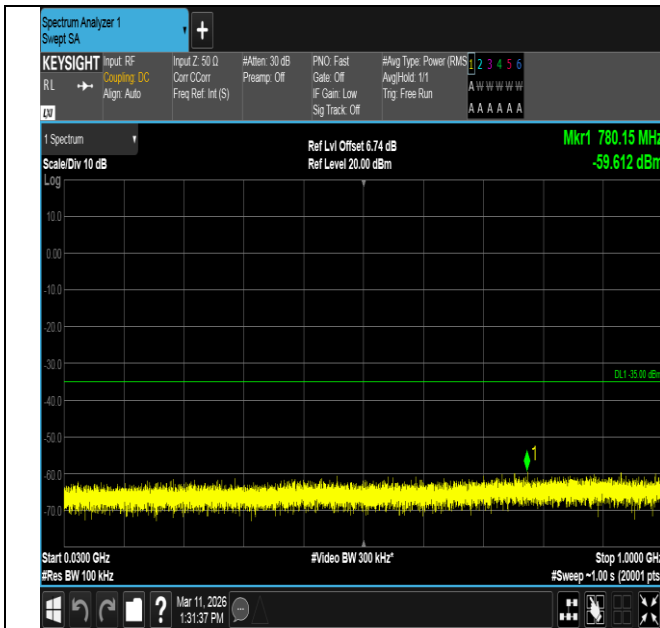
Band7-15MHz-16QAM-21375-1RB#74-30~1000-PASS
