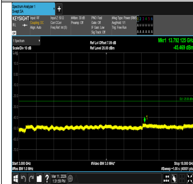
Band7-15MHz-16QAM-21375-1RB#74-3000~18000-PASS
