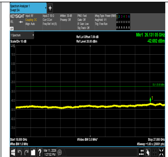
Band7-15MHz-16QAM-21100-75RB#0-18000~27000-PASS
