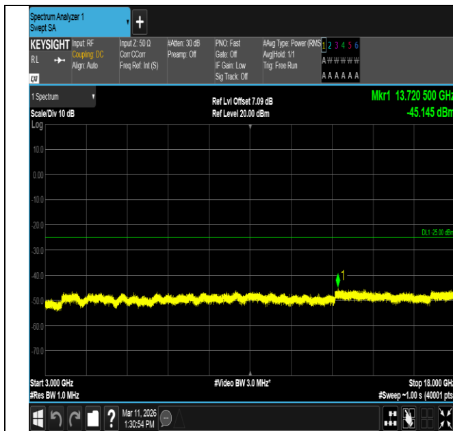
Band7-15MHz-QPSK-21375-1RB#74-3000~18000-PASS
