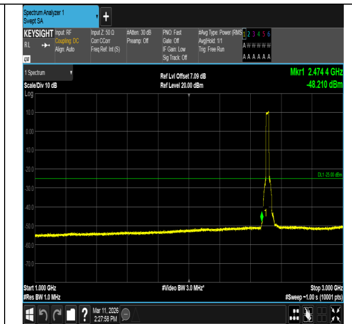
Band7-20MHz-QPSK-20850-100RB#0-1000~3000-PASS
