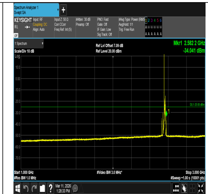
Band7-15MHz-QPSK-21375-1RB#0-1000~3000-PASS
