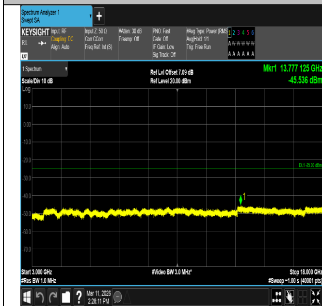
Band7-20MHz-QPSK-20850-100RB#0-3000~18000-PASS
