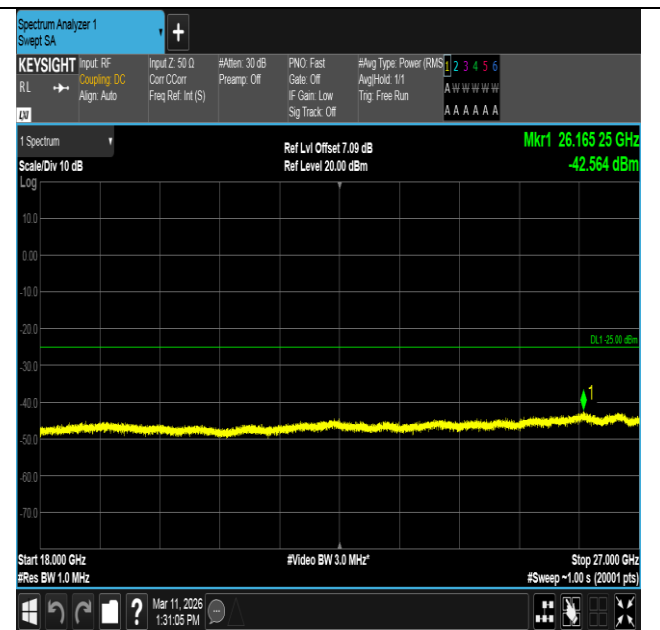
Band7-15MHz-QPSK-21375-1RB#74-18000~27000-PASS
