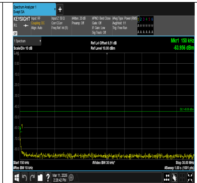
Band7-20MHz-16QAM-20850-100RB#0-0.15~30-PASS
