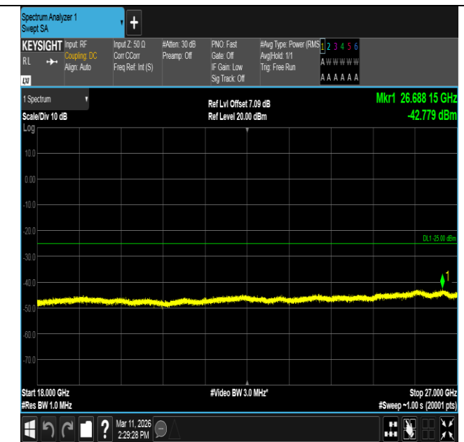
Band7-20MHz-16QAM-20850-100RB#0-18000~27000-PASS
