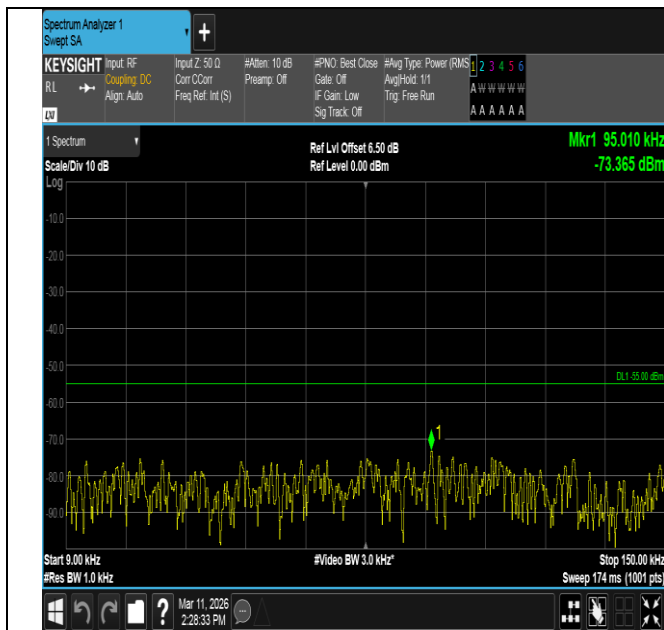
Band7-20MHz-16QAM-20850-100RB#0-0.009~0.15-PASS
