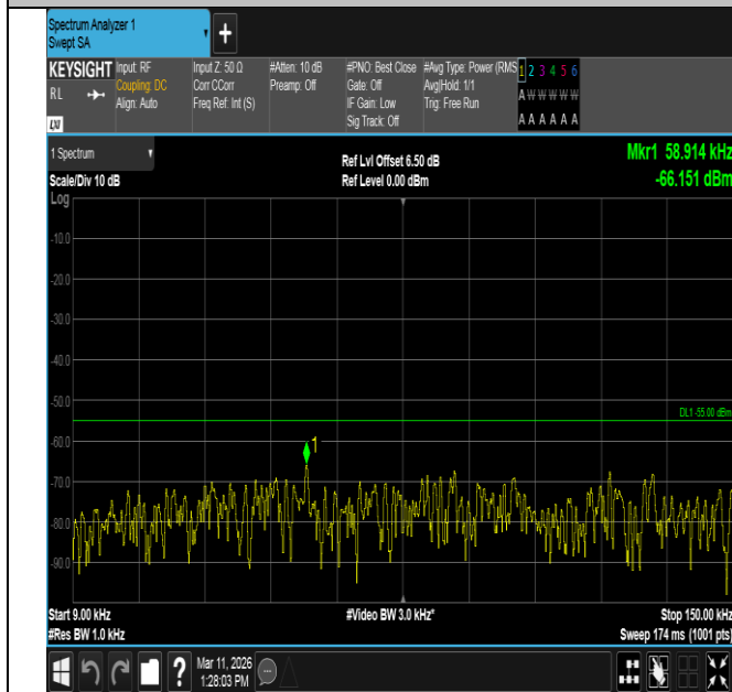
Band7-15MHz-QPSK-21375-1RB#0-0.009~0.15-PASS
