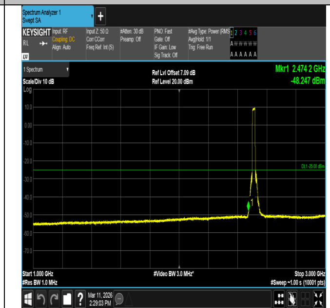
Band7-20MHz-16QAM-20850-100RB#0-1000~3000-PASS
