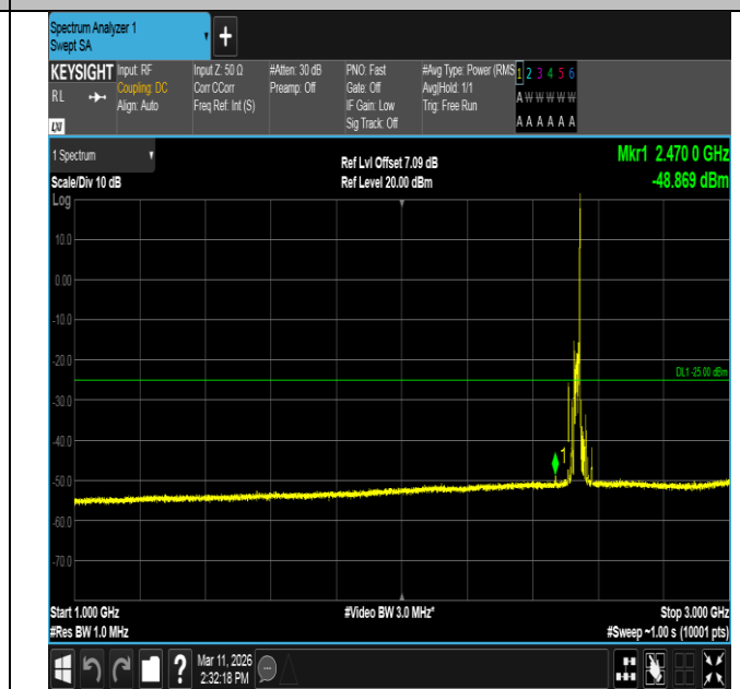
Band7-20MHz-QPSK-21100-1RB#99-1000~3000-PASS
