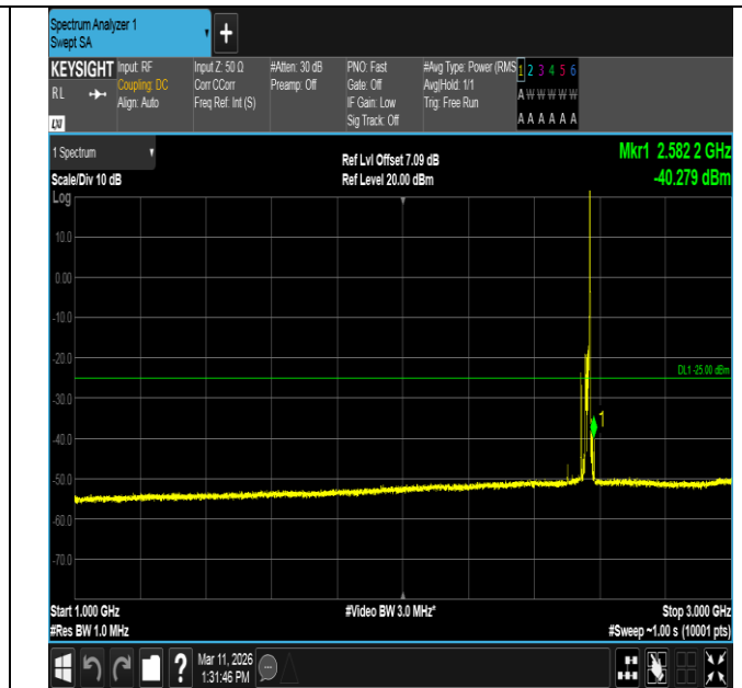
Band7-15MHz-16QAM-21375-1RB#74-1000~3000-PASS
