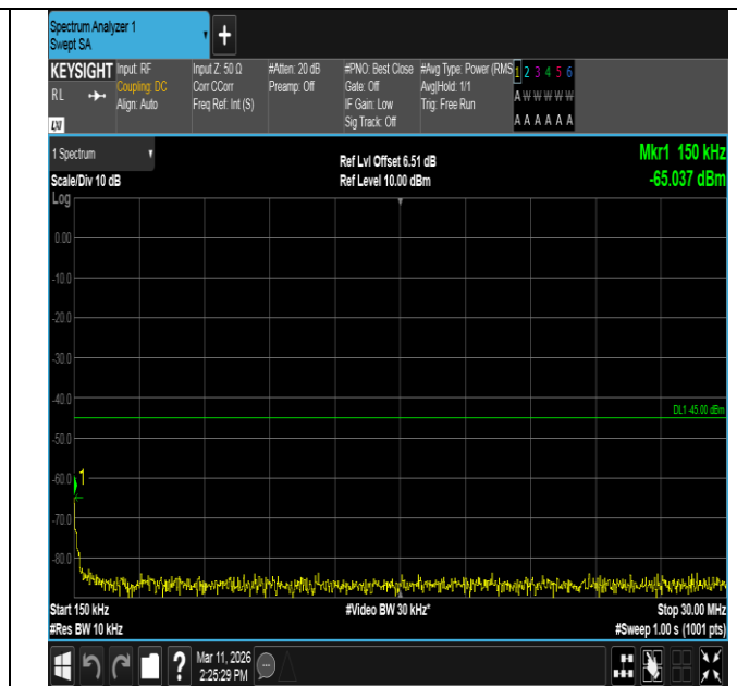
Band7-20MHz-QPSK-20850-1RB#99-0.15~30-PASS
