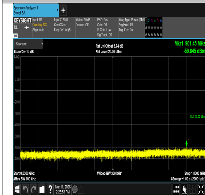
Band7-20MHz-16QAM-20850-100RB#0-30~1000-PASS
