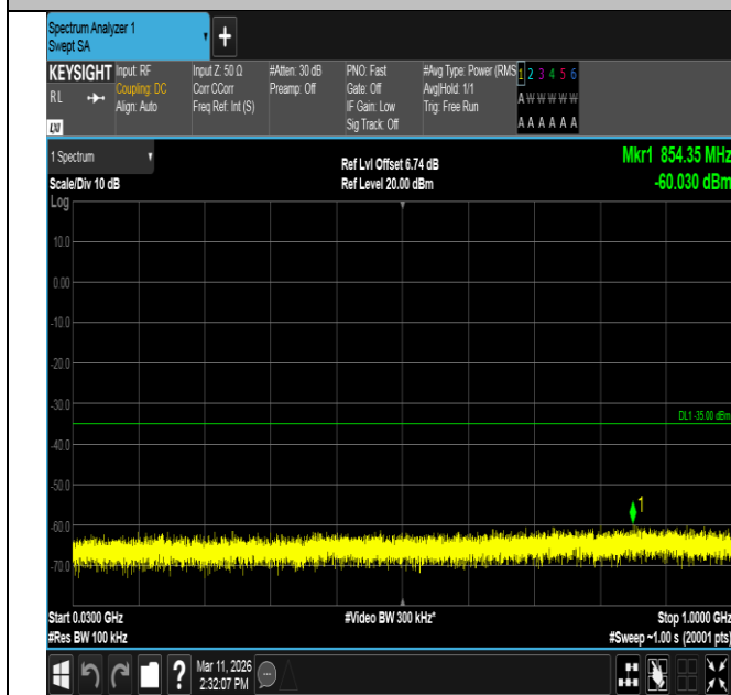
Band7-20MHz-QPSK-21100-1RB#99-30~1000-PASS
