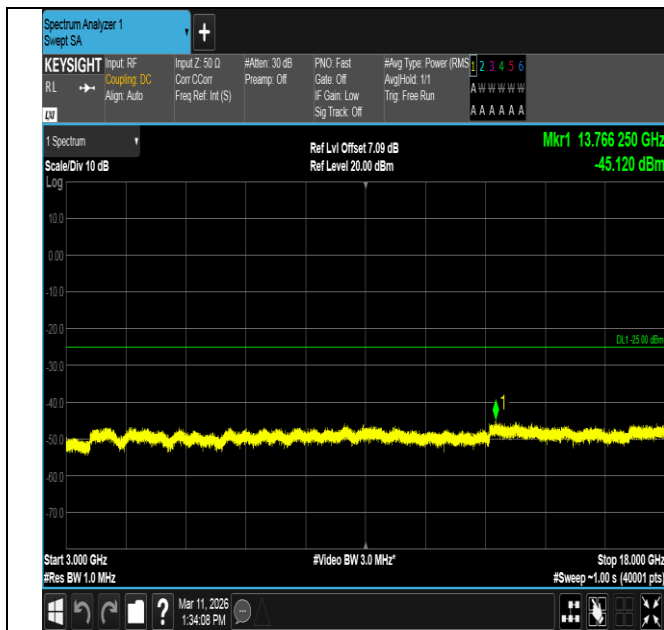
Band7-15MHz-16QAM-21375-75RB#0-3000~18000-PASS
