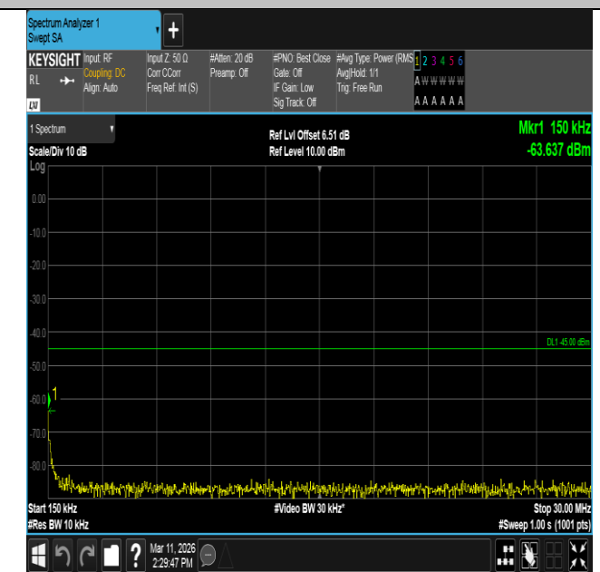
Band7-20MHz-QPSK-21100-1RB#0-0.15~30-PASS
