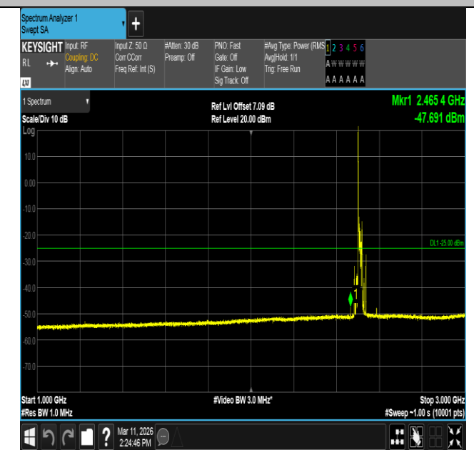
Band7-20MHz-16QAM-20850-1RB#0-1000~3000-PASS
