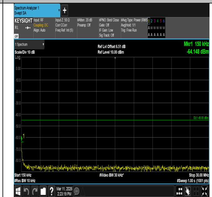
Band7-20MHz-QPSK-20850-1RB#0-0.15~30-PASS
