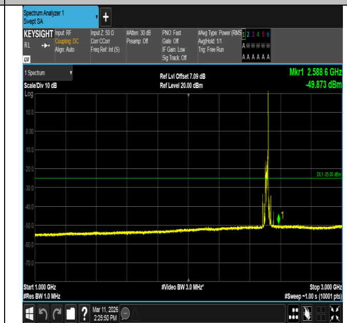
Band7-20MHz-QPSK-20850-1RB#99-1000~3000-PASS
