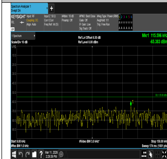
Band7-20MHz-QPSK-21100-1RB#0-0.009~0.15-PASS
