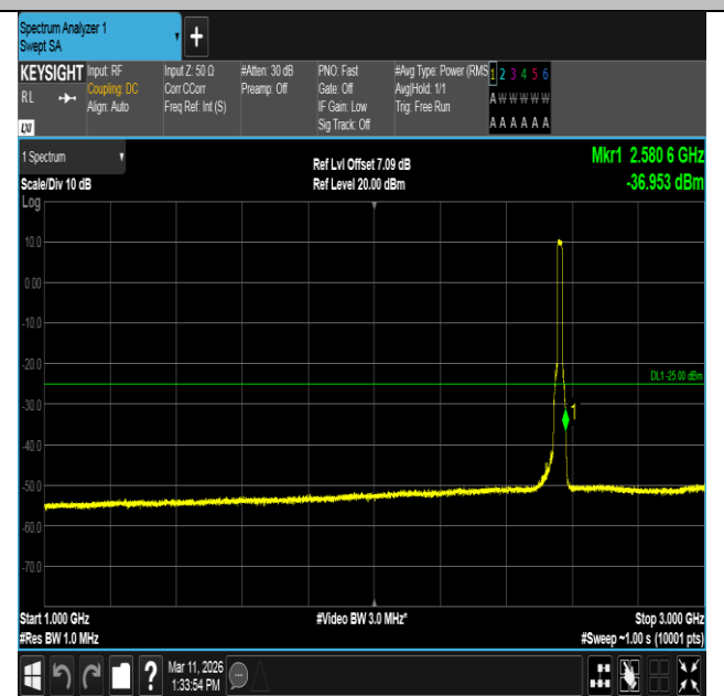
Band7-15MHz-16QAM-21375-75RB#0-1000~3000-PASS
