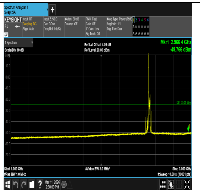
Band7-20MHz-QPSK-21100-1RB#0-1000~3000-PASS
