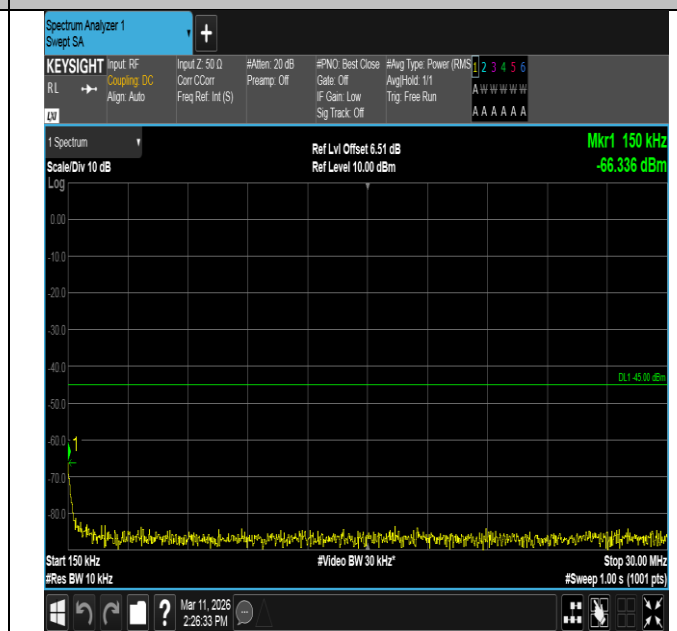
Band7-20MHz-16QAM-20850-1RB#99-0.15~30-PASS
