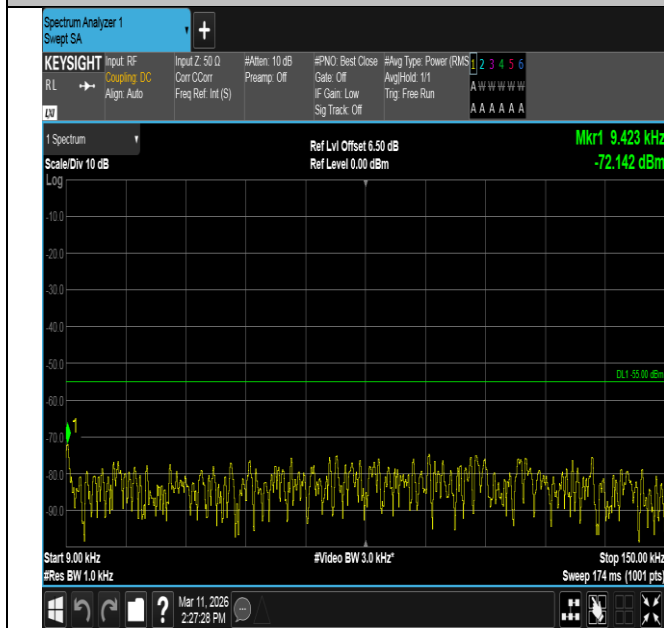
Band7-20MHz-QPSK-20850-100RB#0-0.009~0.15-PASS
