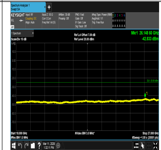
Band7-15MHz-16QAM-21375-1RB#74-18000~27000-PASS
