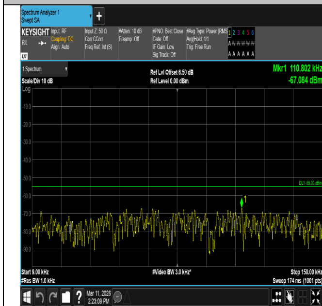
Band7-20MHz-QPSK-20850-1RB#0-0.009~0.15-PASS
