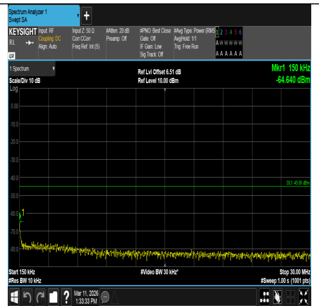
Band7-15MHz-16QAM-21375-75RB#0-0.15~30-PASS
