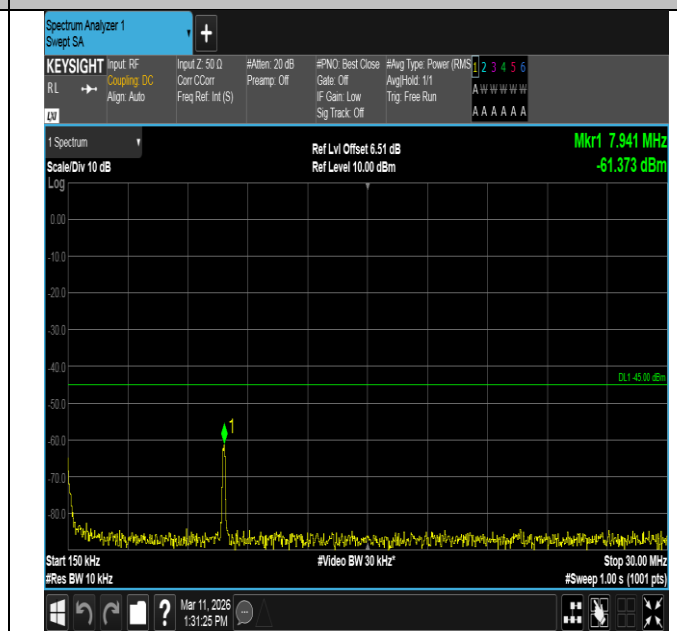
Band7-15MHz-16QAM-21375-1RB#74-0.15~30-PASS
