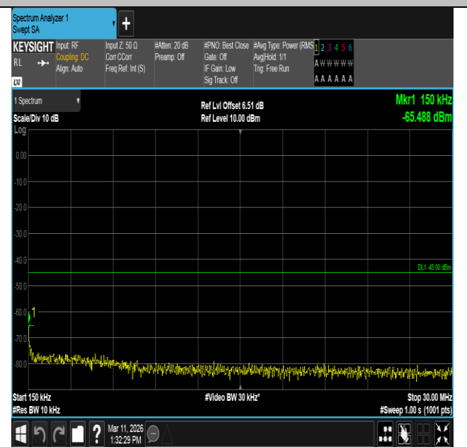
Band7-15MHz-QPSK-21375-75RB#0-0.15~30-PASS
