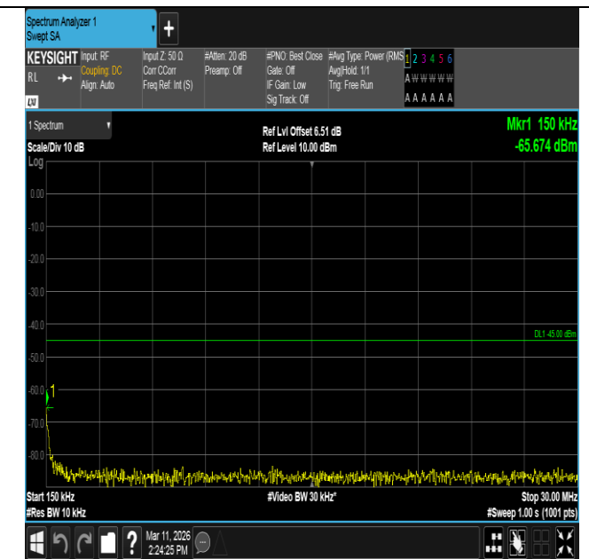
Band7-20MHz-16QAM-20850-1RB#0-0.15~30-PASS
