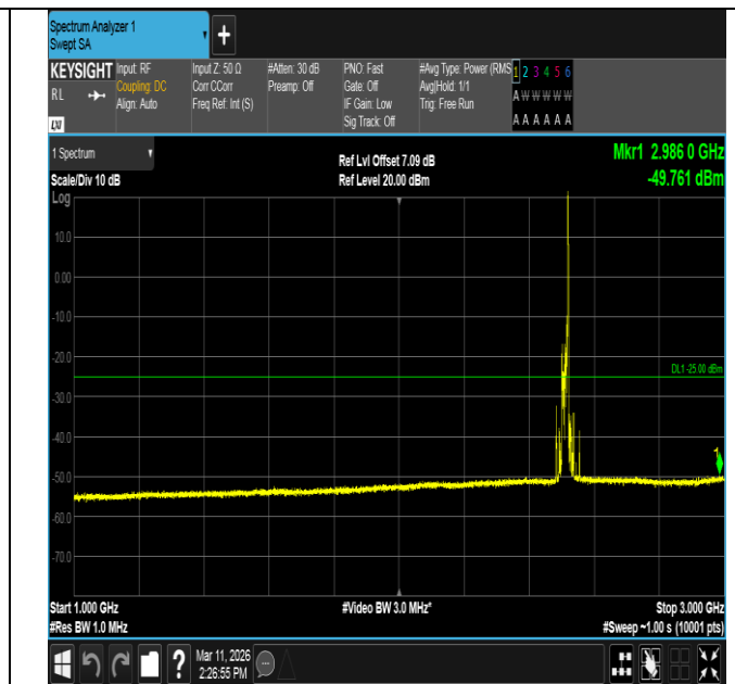
Band7-20MHz-16QAM-20850-1RB#99-1000~3000-PASS
