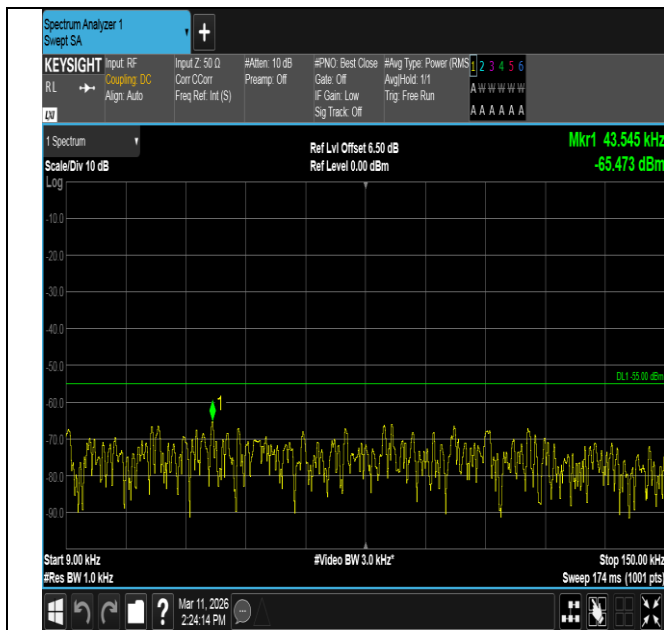
Band7-20MHz-16QAM-20850-1RB#0-0.009~0.15-PASS
