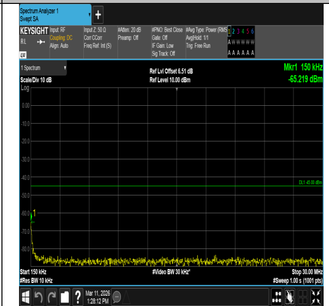
Band7-15MHz-QPSK-21375-1RB#0-0.15~30-PASS
