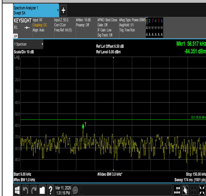
Band7-15MHz-16QAM-21375-1RB#74-0.009~0.15-PASS
