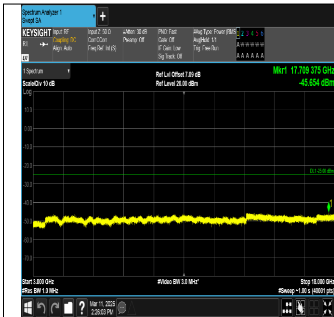
Band7-20MHz-QPSK-20850-1RB#99-3000~18000-PASS
