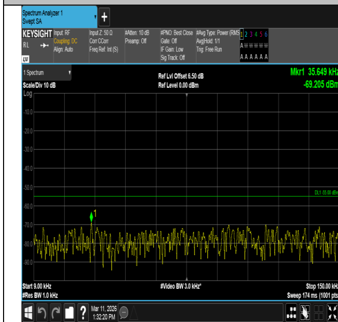
Band7-15MHz-QPSK-21375-75RB#0-0.009~0.15-PASS
