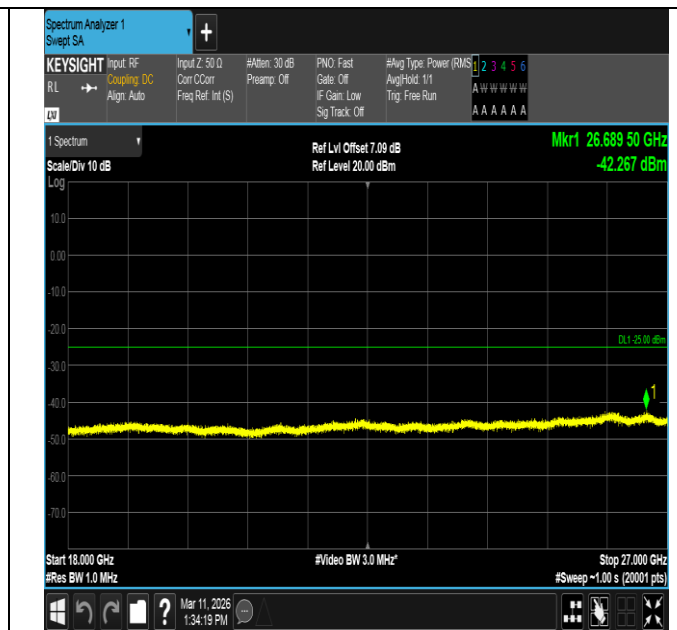
Band7-15MHz-16QAM-21375-75RB#0-18000~27000-PASS
