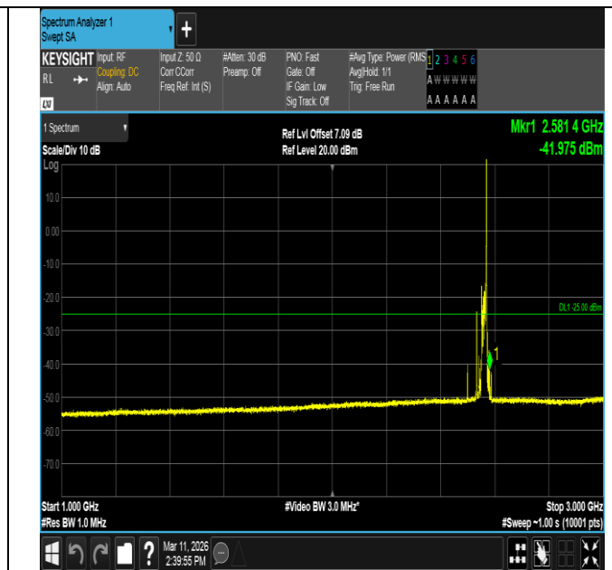
Band7-20MHz-16QAM-21350-1RB#99-1000~3000-PASS
