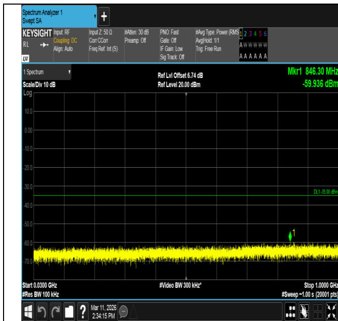
Band7-20MHz-QPSK-21100-100RB#0-30~1000-PASS
