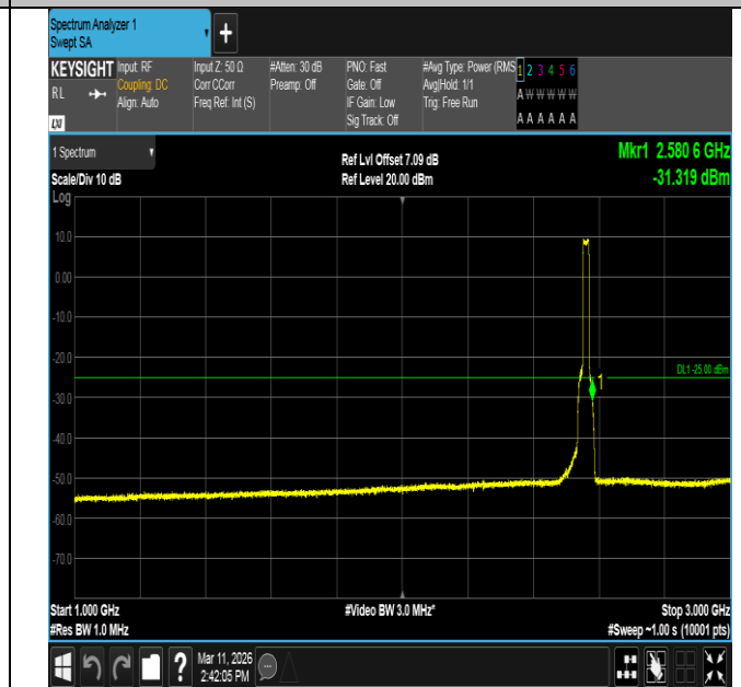
Band7-20MHz-16QAM-21350-100RB#0-1000~3000-PASS
