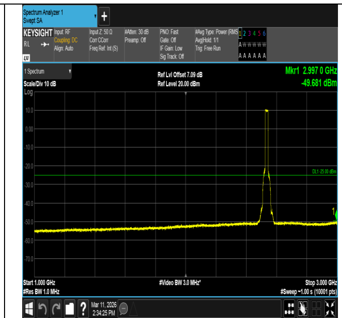
Band7-20MHz-QPSK-21100-100RB#0-1000~3000-PASS
