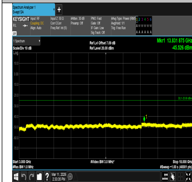
Band7-20MHz-16QAM-21100-1RB#99-3000~18000-PASS
