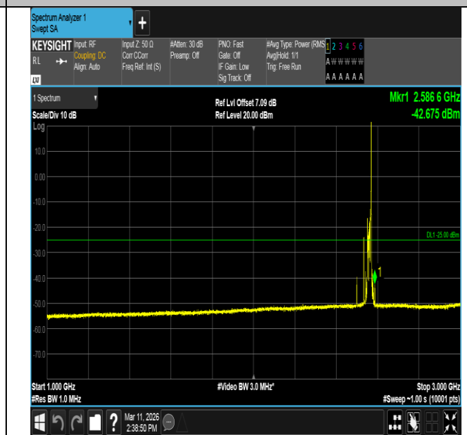
Band7-20MHz-QPSK-21350-1RB#99-1000~3000-PASS
