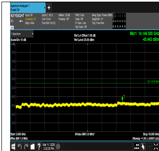
Band7-20MHz-QPSK-21100-1RB#99-3000~18000-PASS
