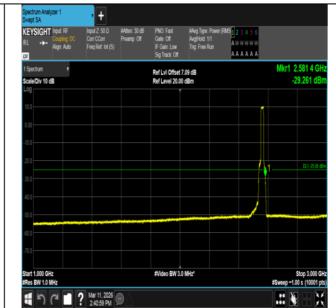
Band7-20MHz-QPSK-21350-100RB#0-1000~3000-PASS
