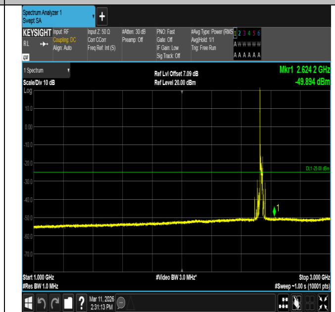
Band7-20MHz-16QAM-21100-1RB#0-1000~3000-PASS
