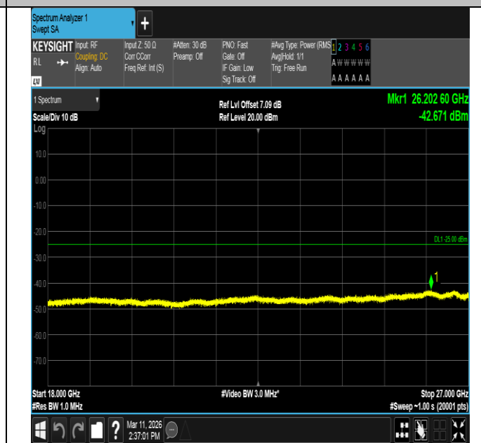
Band7-20MHz-QPSK-21350-1RB#0-18000~27000-PASS
