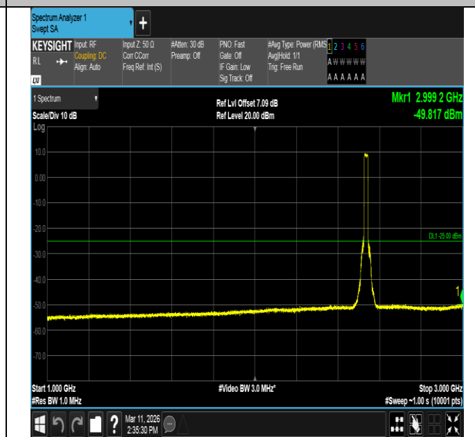
Band7-20MHz-16QAM-21100-100RB#0-1000~3000-PASS
