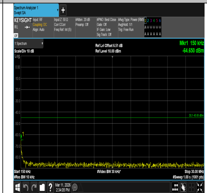
Band7-20MHz-QPSK-21100-100RB#0-0.15~30-PASS
