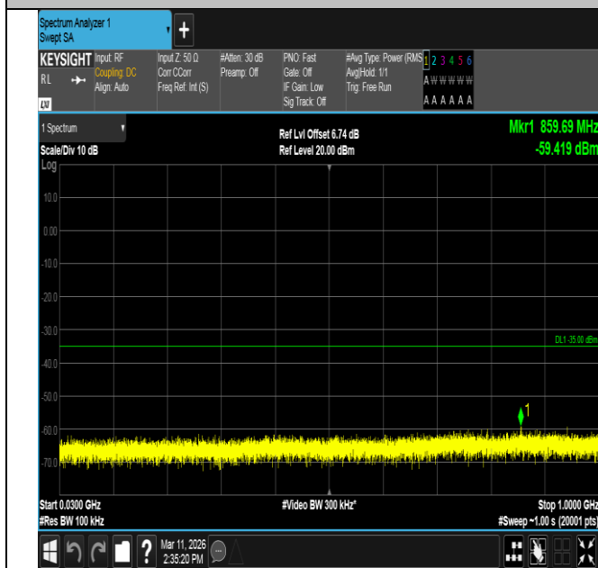
Band7-20MHz-16QAM-21100-100RB#0-30~1000-PASS
