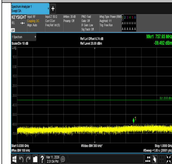
Band7-20MHz-16QAM-21100-1RB#0-30~1000-PASS
