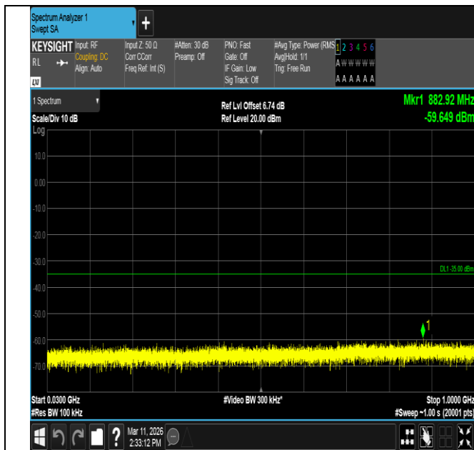
Band7-20MHz-16QAM-21100-1RB#99-30~1000-PASS
