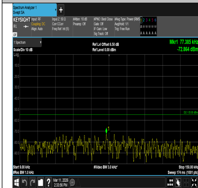
Band7-20MHz-QPSK-21100-100RB#0-0.009~0.15-PASS
