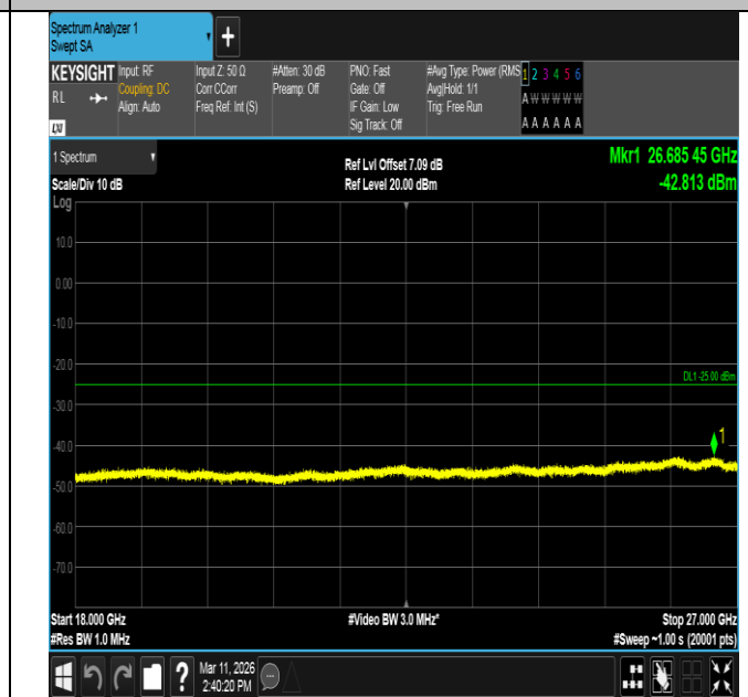
Band7-20MHz-16QAM-21350-1RB#99-18000~27000-PASS
