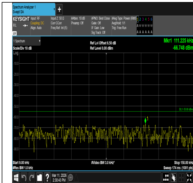
Band7-20MHz-16QAM-21100-1RB#0-0.009~0.15-PASS
