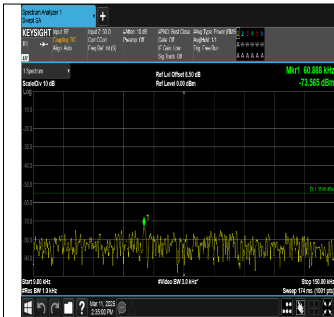
Band7-20MHz-16QAM-21100-100RB#0-0.009~0.15-PASS
