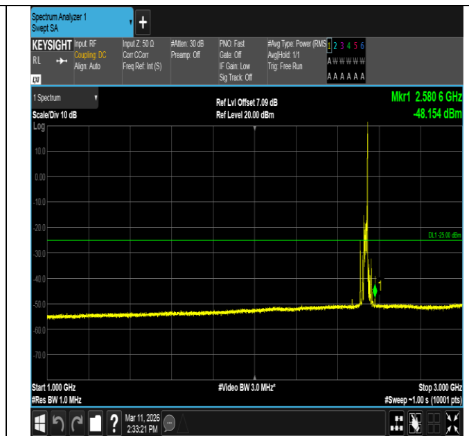
Band7-20MHz-16QAM-21100-1RB#99-1000~3000-PASS
