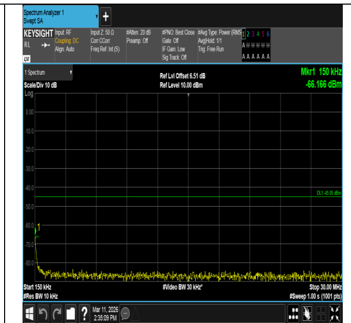
Band7-20MHz-16QAM-21100-100RB#0-0.15~30-PASS
