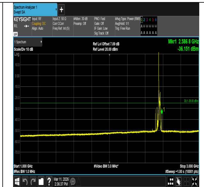
Band7-20MHz-QPSK-21350-1RB#0-1000~3000-PASS
