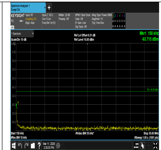
Band7-20MHz-16QAM-21100-1RB#0-0.15~30-PASS
