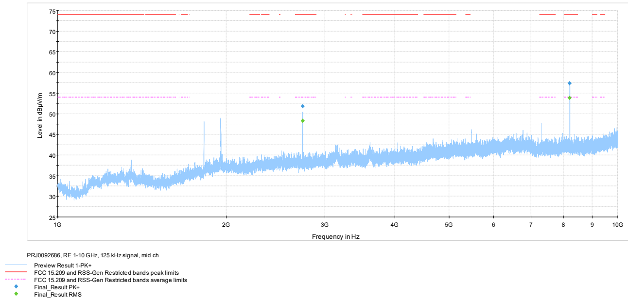
Figure 7.8-5: Radiated spurious emissions 1-10 GHz mid channel, 125 kHz signal
