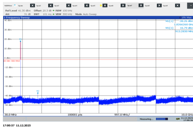
Figure 7.8-12: Conducted spurious emissions on high channel, 125 kHz signal
