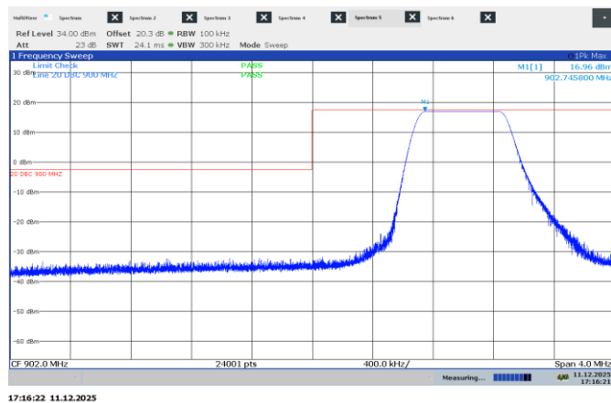
Figure 7.8-19: Conducted non-restricted band edge emissions at 902 MHz, 500 kHz signal
