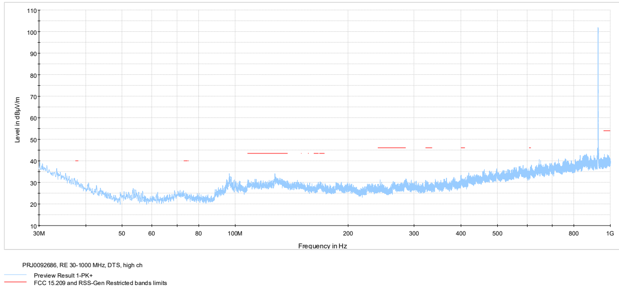
Figure 7.8-15: Radiated spurious emissions 30-1000 MHz high channel, 500 kHz signal
