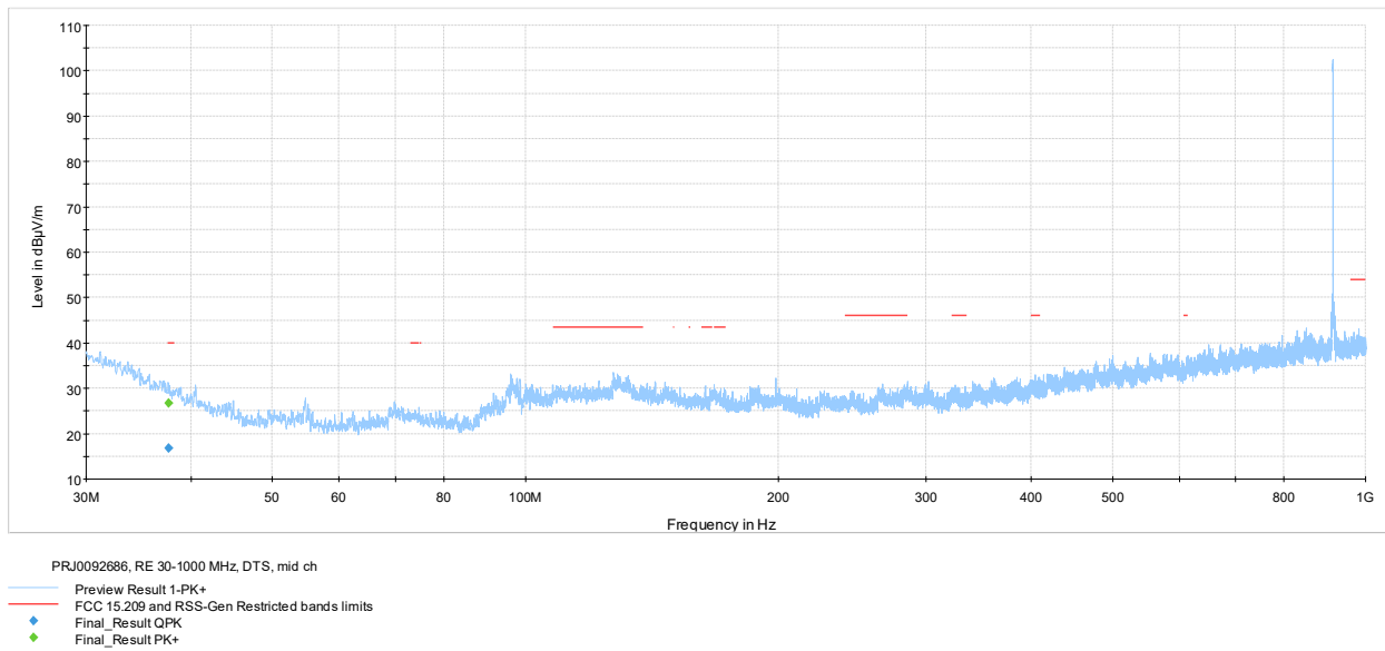
Figure 7.8-14: Radiated spurious emissions 30-1000 MHz mid channel, 500 kHz signal
