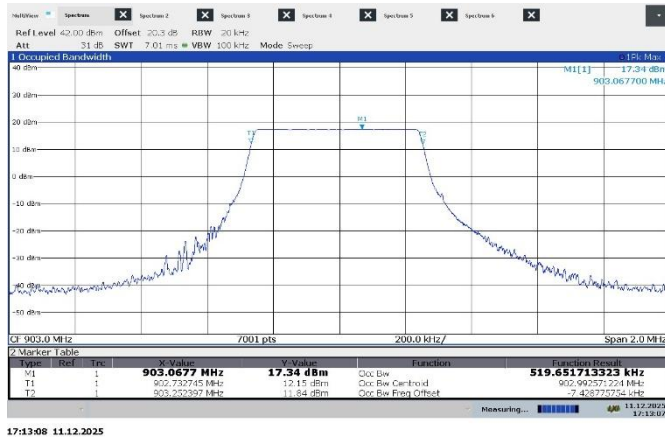
Figure 7.6-4: 99% occupied bandwidth on low ch
