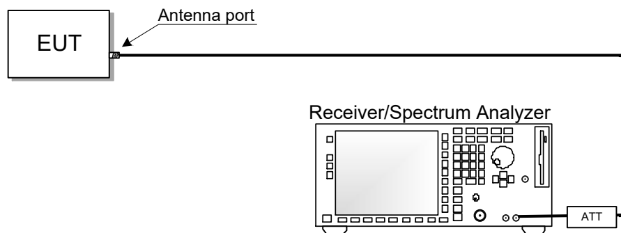
Figure 4.5-2: Antenna port testing block diagram
