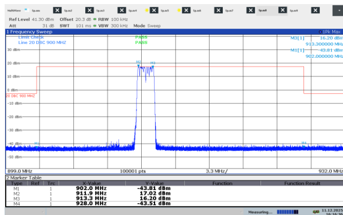
Figure 7.8-9: Conducted non-restricted band edge emissions, hopping on, 125 kHz signal
