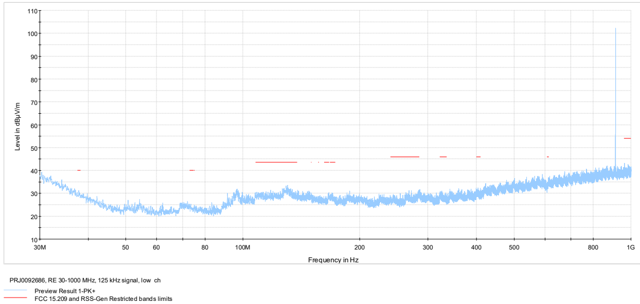
Figure 7.8-1: Radiated spurious emissions 30-1000 MHz low channel, 125 kHz signal
