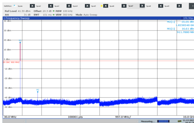
Figure 7.8-10: Conducted spurious emissions on low channel, 125 kHz signal
