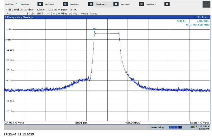
Figure 7.9-2: PSD on mid channel, 500 kHz
