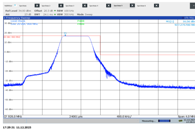
Figure 7.8-20: Conducted non-restricted band edge emissions at 928 MHz, 500 kHz signal
