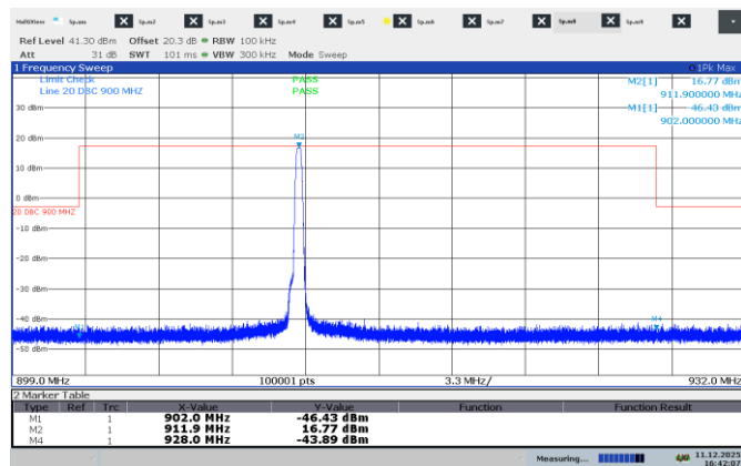
Figure 7.8-7: Conducted non-restricted band edge emissions at 902 MHz, hopping off, 125 kHz signal
