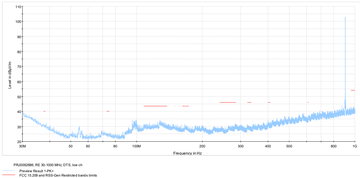
Figure 7.8-13: Radiated spurious emissions 30-1000 MHz low channel, 500 kHz signal
