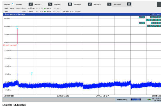
Figure 7.8-22: Conducted spurious emissions on mid channel, 500 kHz signal
