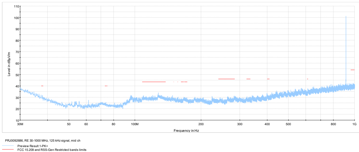
Figure 7.8-2: Radiated spurious emissions 30-1000 MHz mid channel, 125 kHz signal
