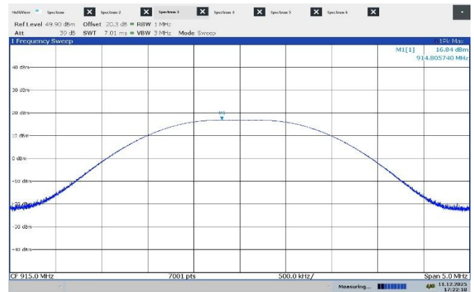
Figure 7.7-2: Output power on mid channel
