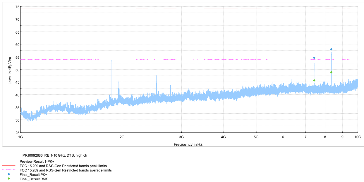
Figure 7.8-18: Radiated spurious emissions 1-10 GHz high channel, 500 kHz signal
