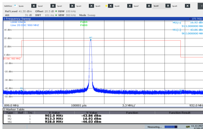
Figure 7.8-8: Conducted non-restricted band edge emissions at 928 MHz, hopping off, 125 kHz signal
