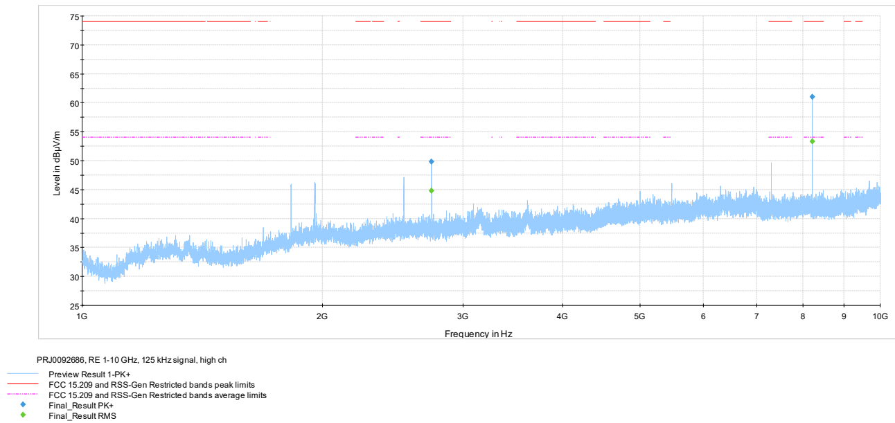
Figure 7.8-6: Radiated spurious emissions 1-10 GHz high channel, 125 kHz signal
