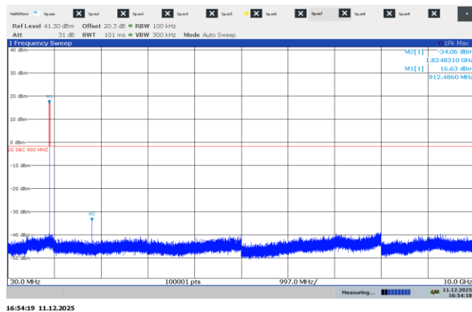
Figure 7.8-11: Conducted spurious emissions on mid channel, 125 kHz signal
