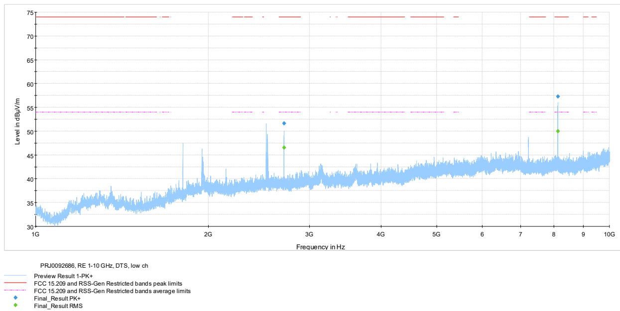
Figure 7.8-16: Radiated spurious emissions 1-10 GHz low channel, 500 kHz signal
