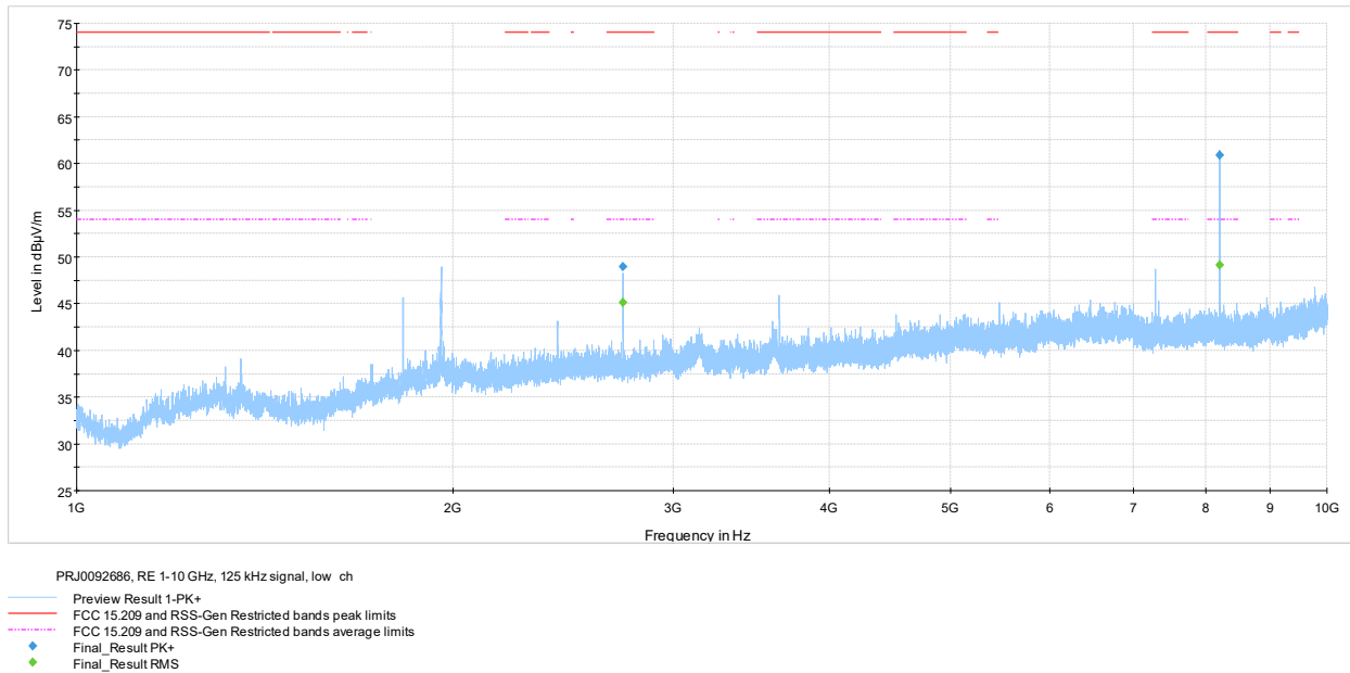
Figure 7.8-4: Radiated spurious emissions 1-10 GHz low channel, 125 kHz signal
