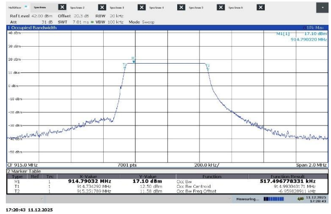
Figure 7.6-5: 99% occupied bandwidth on mid ch
