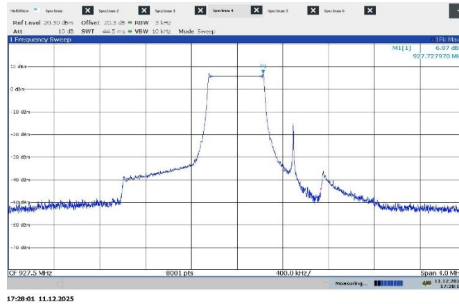
Figure 7.9-3: PSD on high channel, 500 kHz
