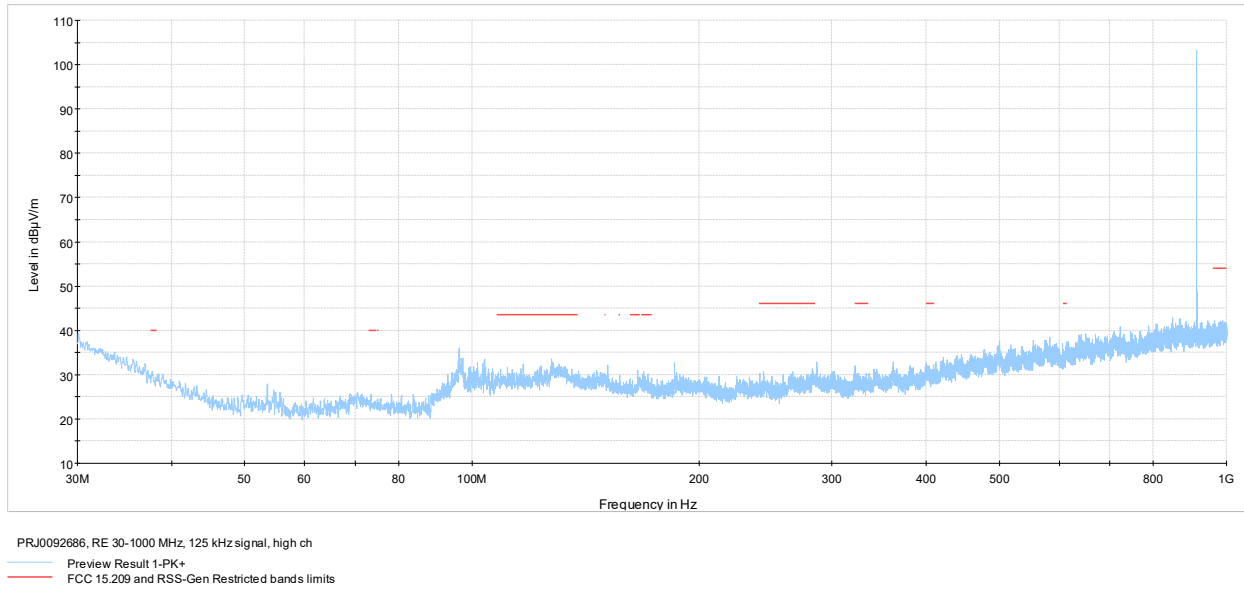
Figure 7.8-3: Radiated spurious emissions 30-1000 MHz high channel, 125 kHz signal
