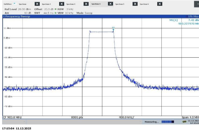
Figure 7.9-1: PSD on low channel, 500 kHz
