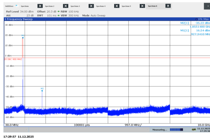
Figure 7.8-23: Conducted spurious emissions on high channel, 500 kHz signal
