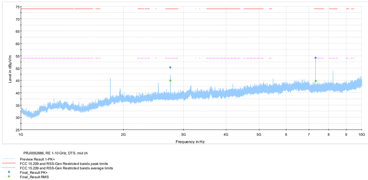
Figure 7.8-17: Radiated spurious emissions 1-10 GHz mid channel, 500 kHz signal
