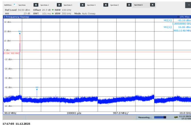
Figure 7.8-21: Conducted spurious emissions on low channel, 500 kHz signal
