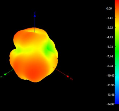
Freq:2450MHz
