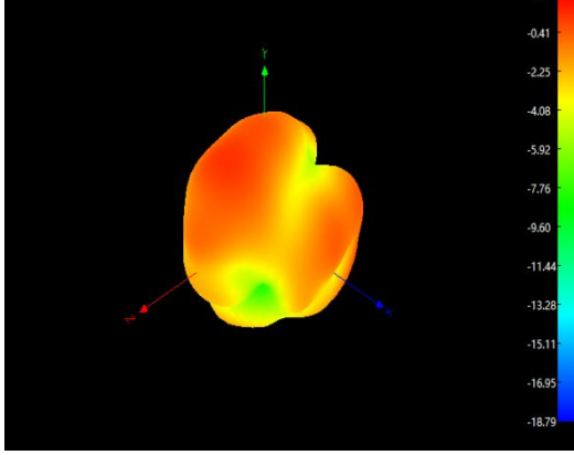
Freq:2400MHz
