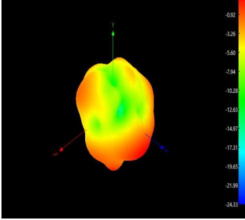
Freq:2480MHz
