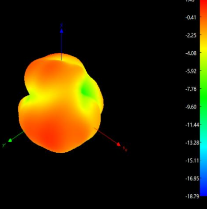
Freq:2400MHz
