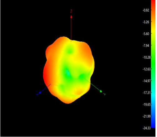
Freq:2480MHz
