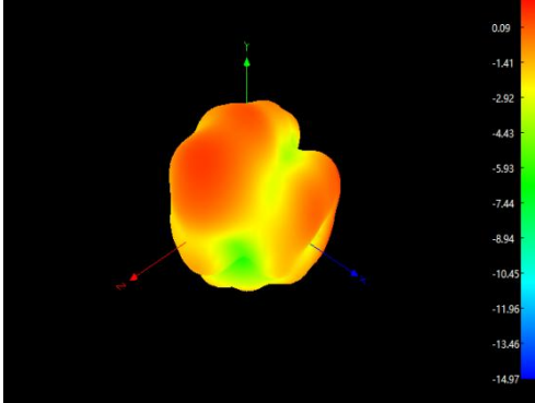
Freq:2450MHz
