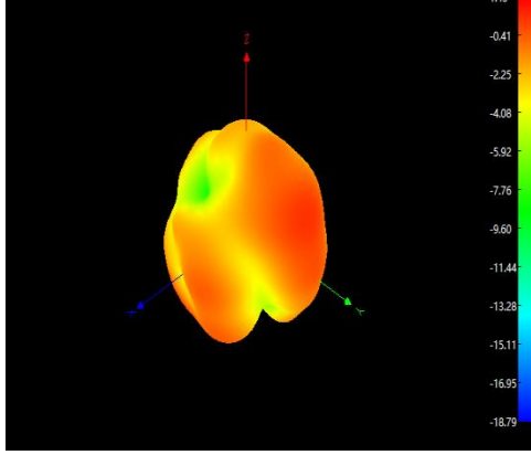
Freq:2400MHz
