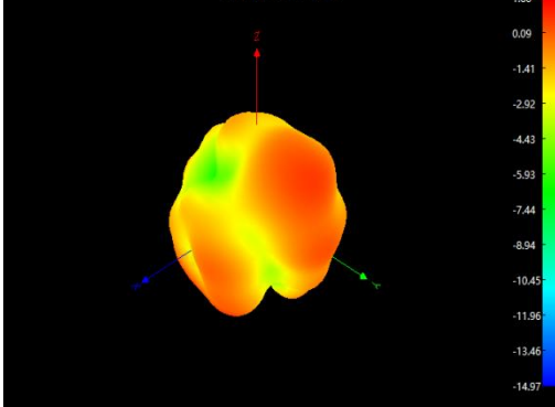
Freq:2450MHz
