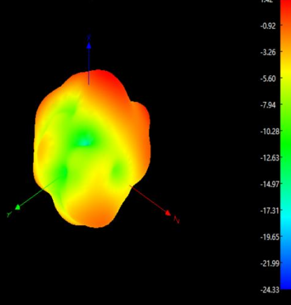
Freq:2480MHz
