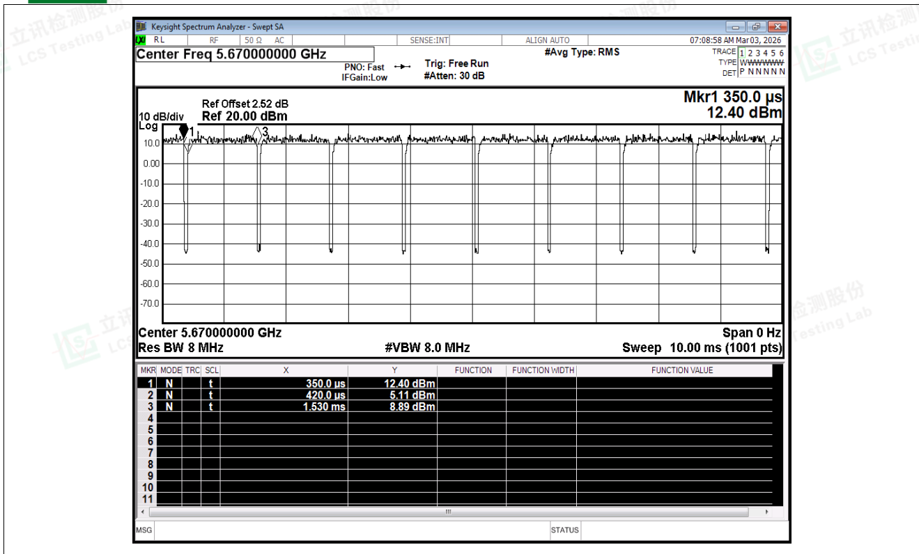
Duty Cycle NVNT n40 5670MHz Ant1
