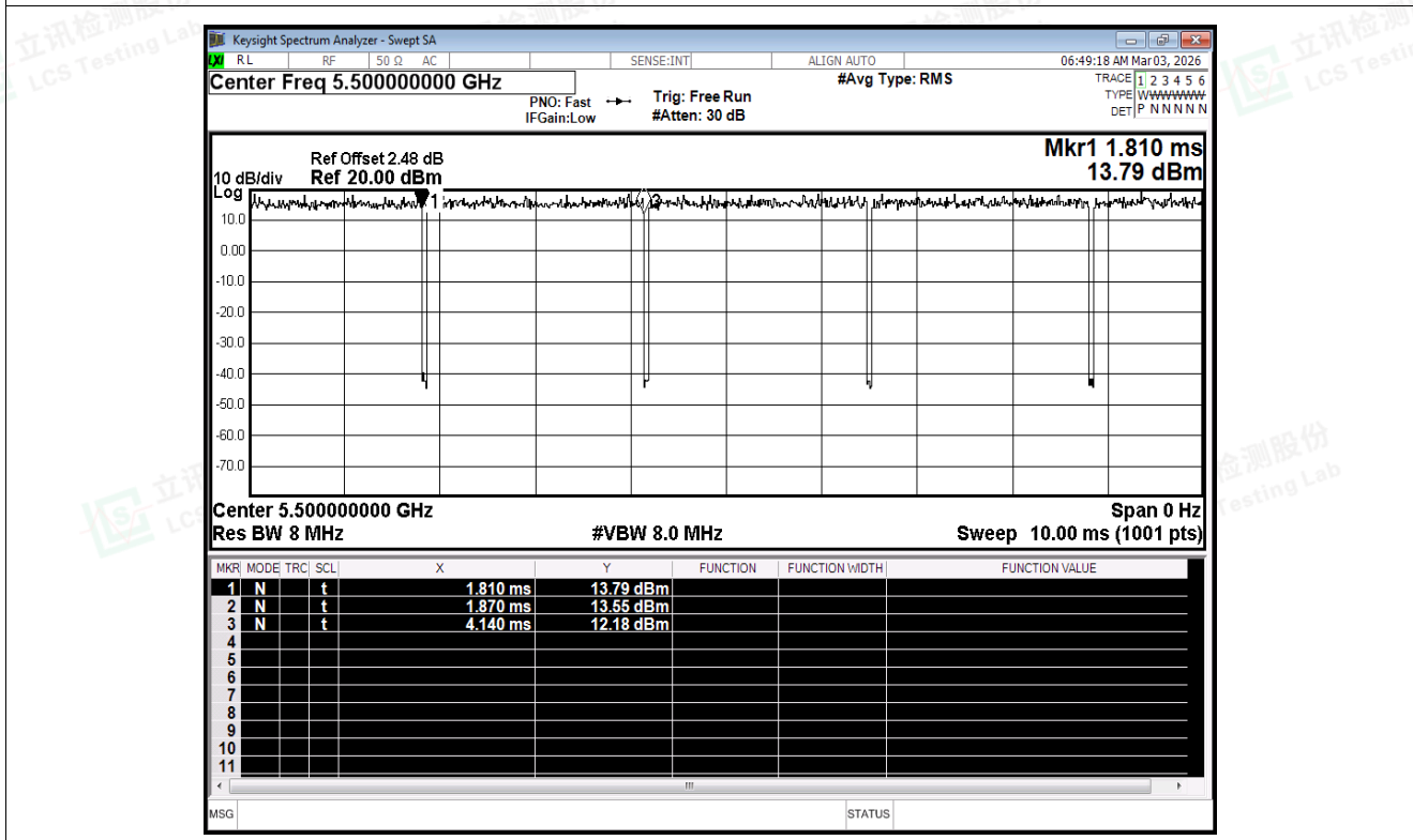
Duty Cycle NVNT ac20 5500MHz Ant1
