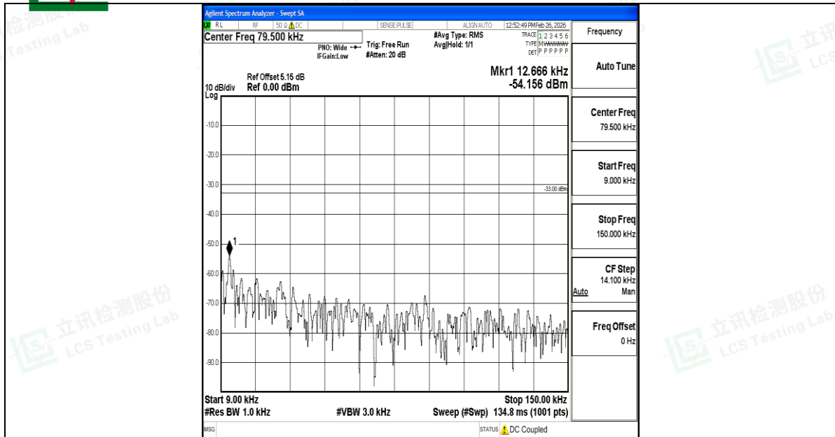
Band5_1.4MHz_QPSK_20525_1RB#0_0.009~0.15_0.009~0.15
