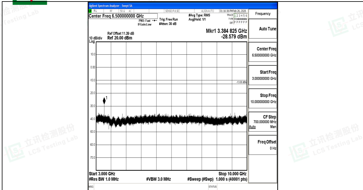
Band5_3MHz_QPSK_20635_1RB#0_3000~10000_3000~10000
