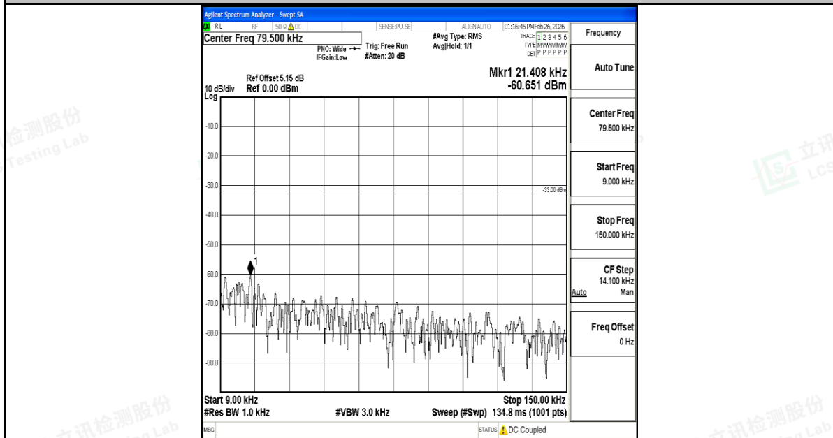
Band5_3MHz_16QAM_20635_1RB#0_0.009~0.15_0.009~0.15
