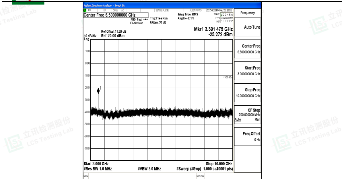
Band5_1.4MHz_QPSK_20643_1RB#0_3000~10000_3000~10000
