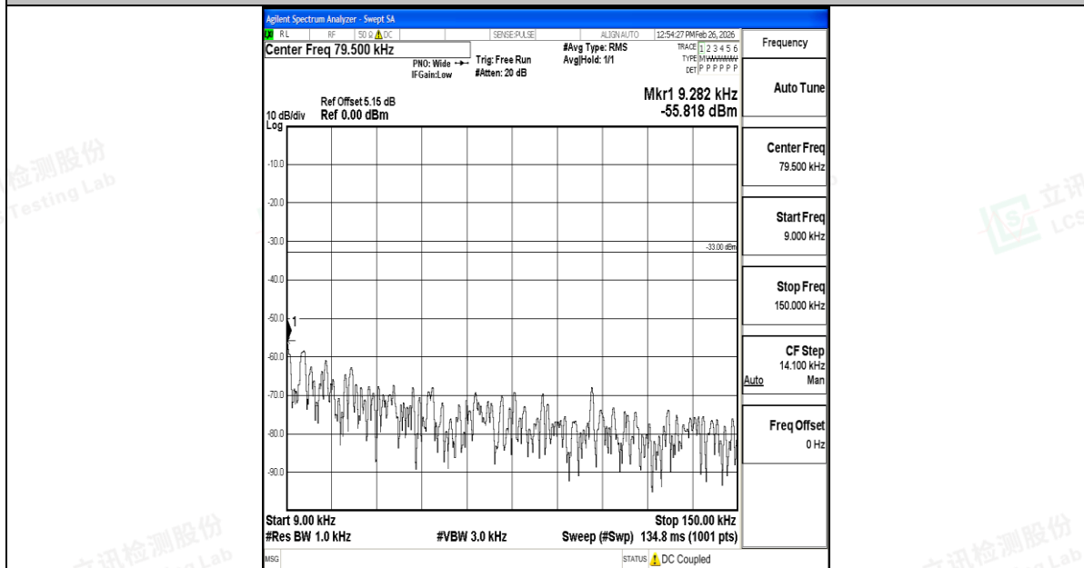
Band5_1.4MHz_16QAM_20643_1RB#0_0.009~0.15_0.009~0.15
