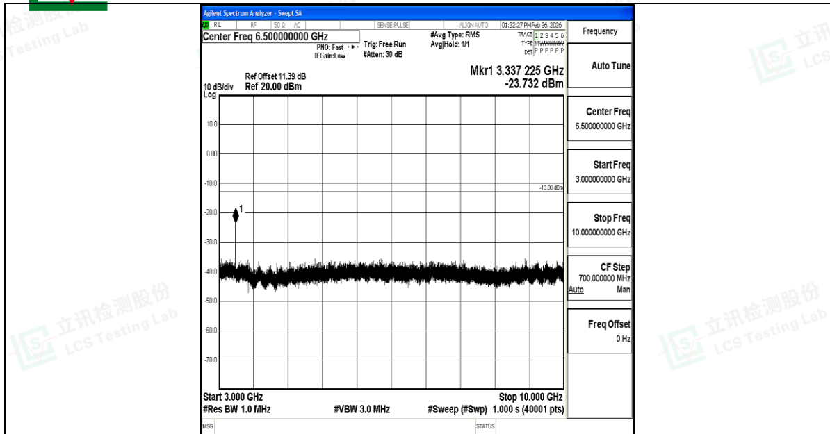
Band5_5MHz_QPSK_20525_1RB#0_3000~10000_3000~10000
