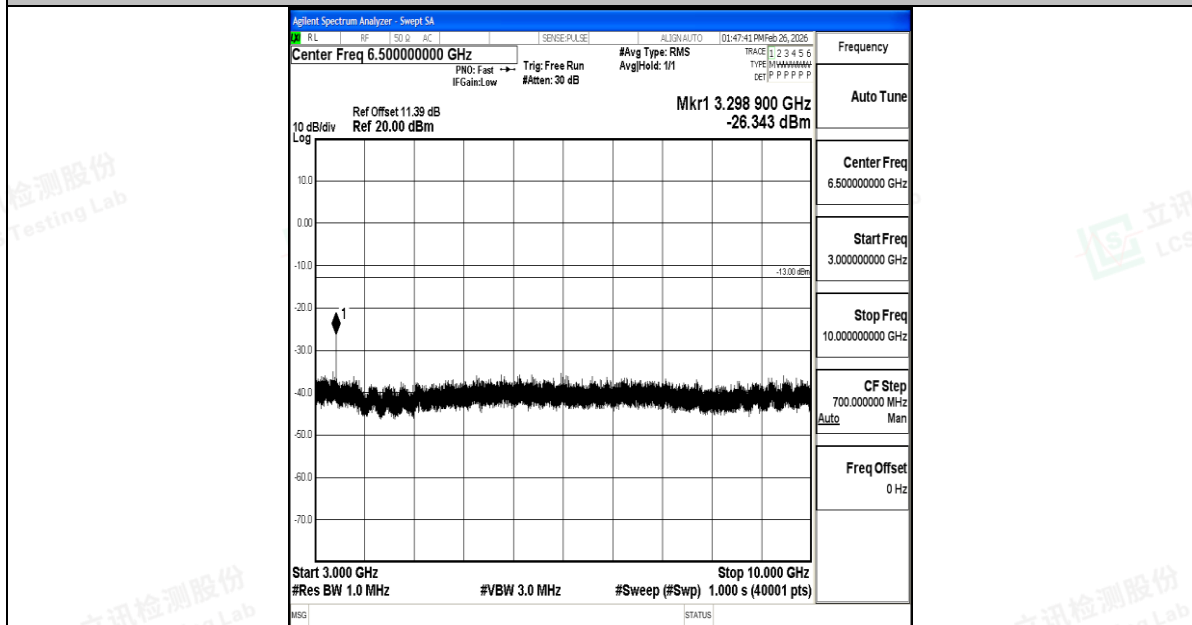
Band5_10MHz_16QAM_20450_1RB#0_3000~10000_3000~10000
