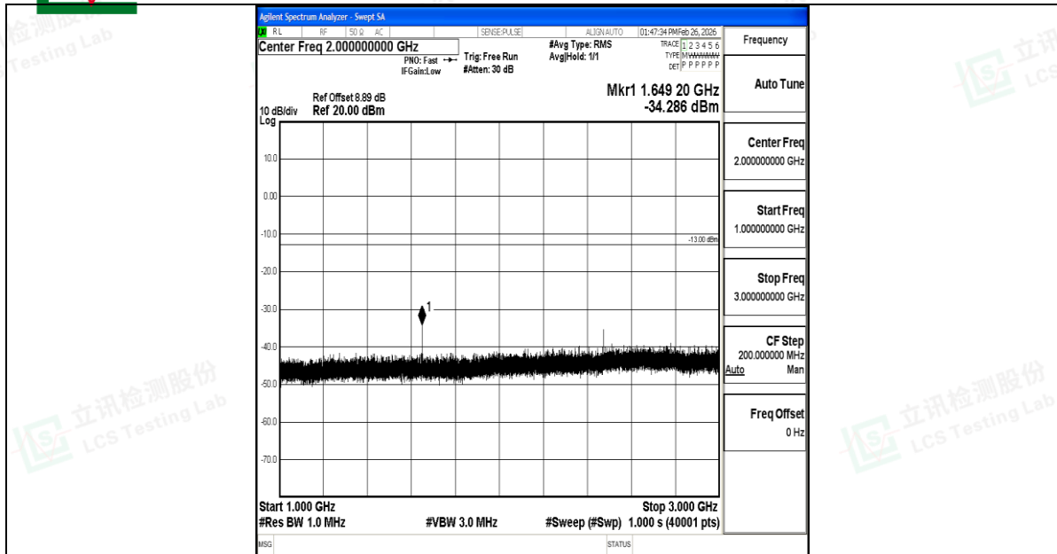
Band5_10MHz_16QAM_20450_1RB#0_1000~3000_1000~3000
