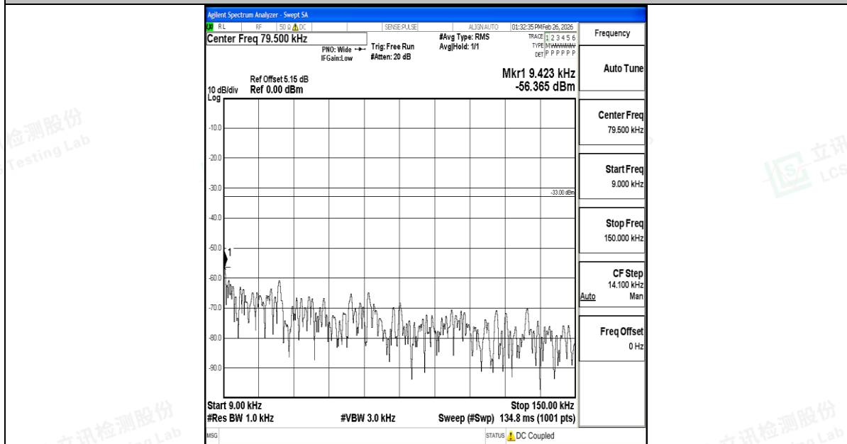
Band5_5MHz_16QAM_20525_1RB#0_0.009~0.15_0.009~0.15
