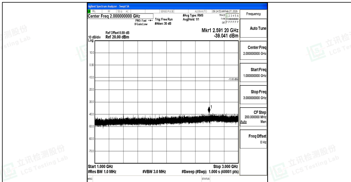
Band12_1.4MHz_16QAM_23017_1RB#0_1000~3000_1000~3000
