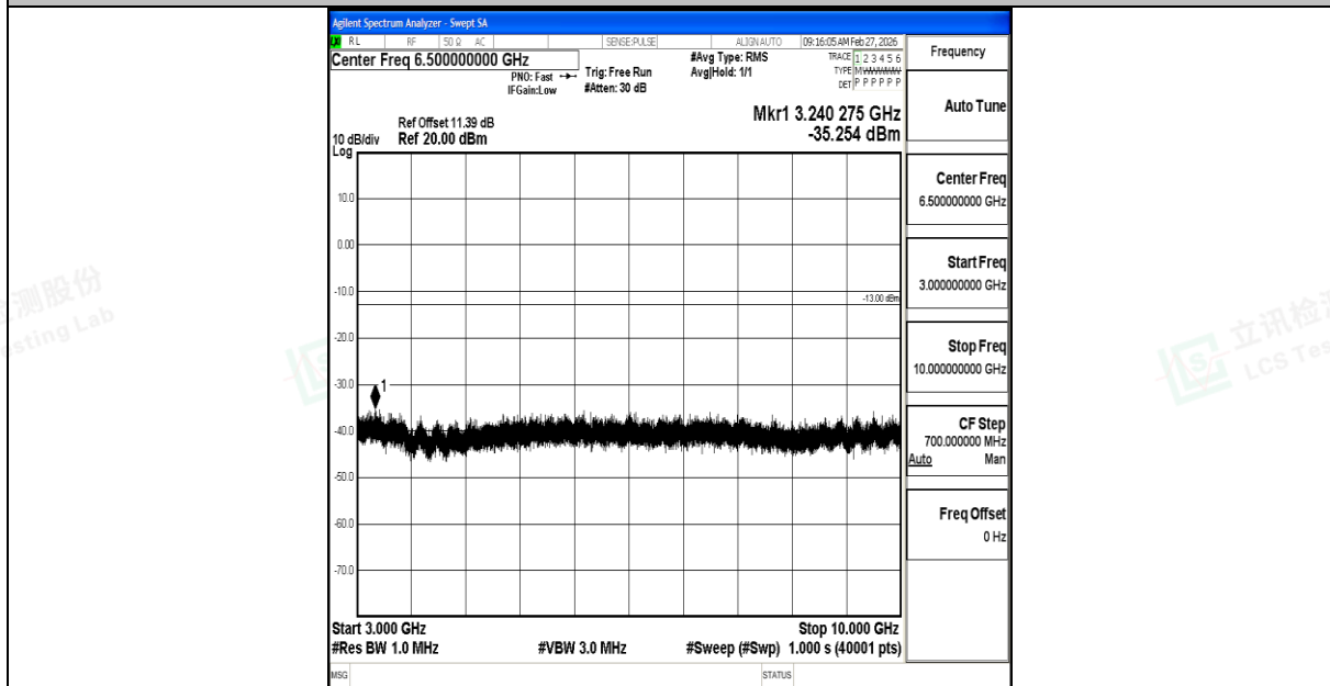
Band12_1.4MHz_16QAM_23095_1RB#0_3000~10000_3000~10000
