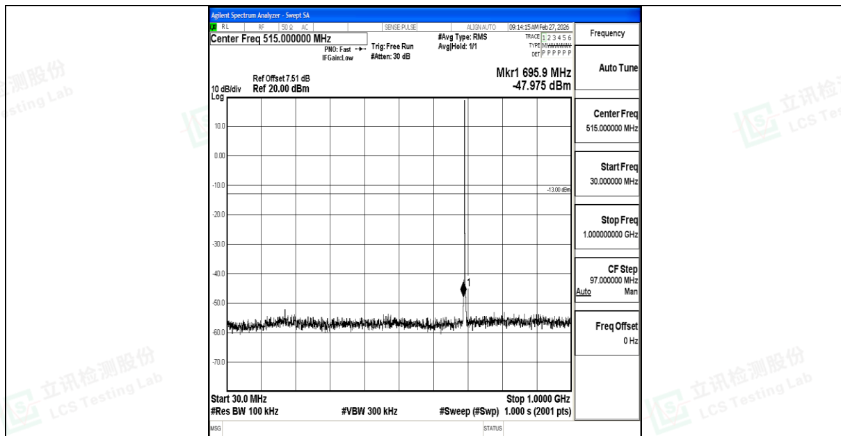
Band12_1.4MHz_QPSK_23017_1RB#0_30~1000_30~1000
