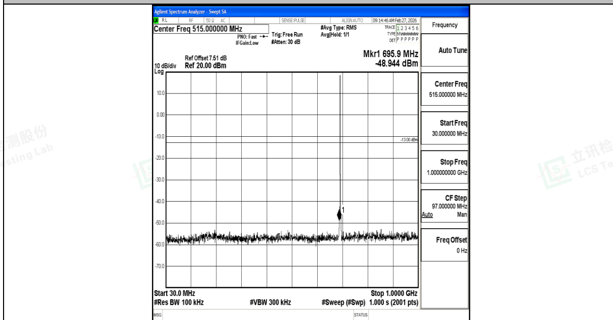
Band12_1.4MHz_16QAM_23017_1RB#0_30~1000_30~1000
