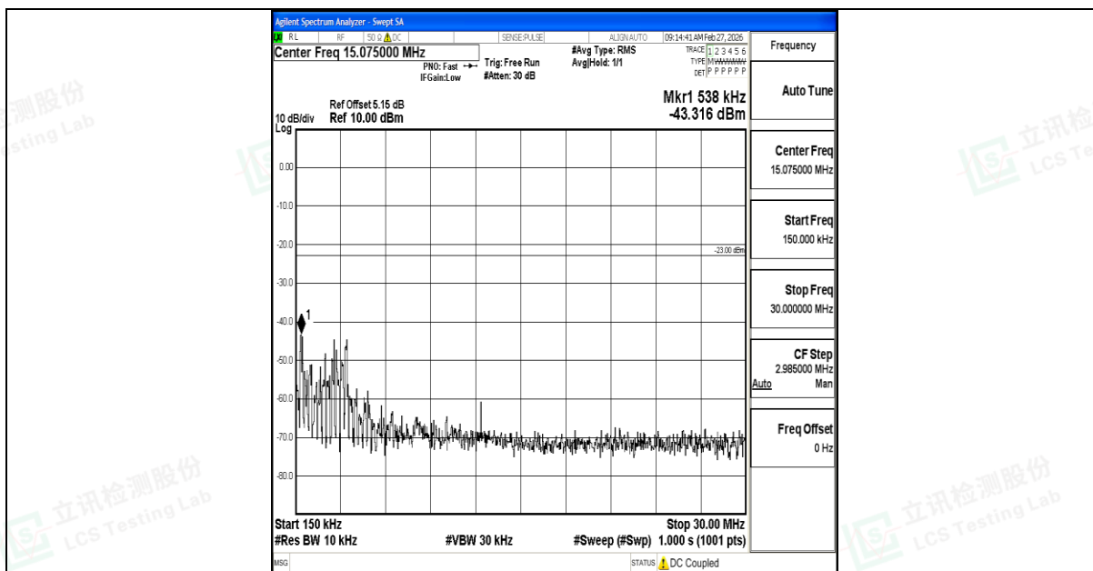
Band12_1.4MHz_16QAM_23017_1RB#0_0.15~30_0.15~30
