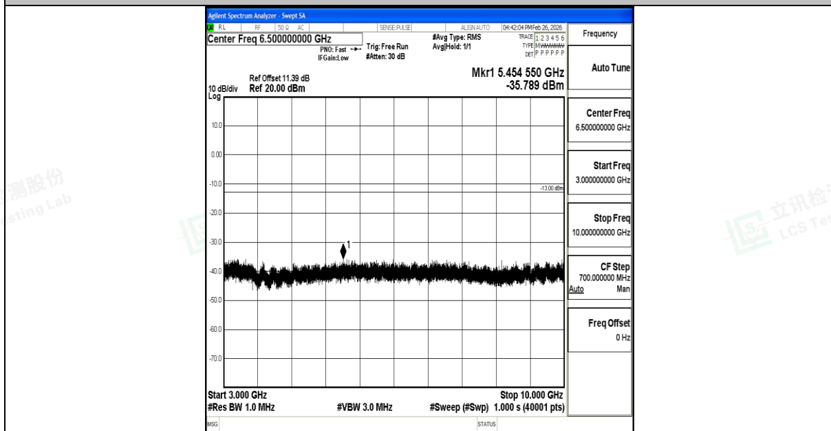
Band12_3MHz_QPSK_23095_1RB#0_3000~10000_3000~10000
