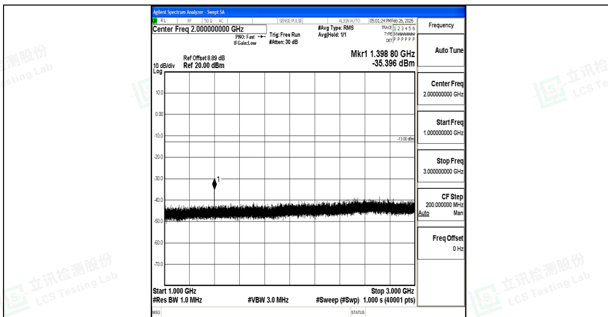
Band12_5MHz_QPSK_23035_1RB#0_1000~3000_1000~3000
