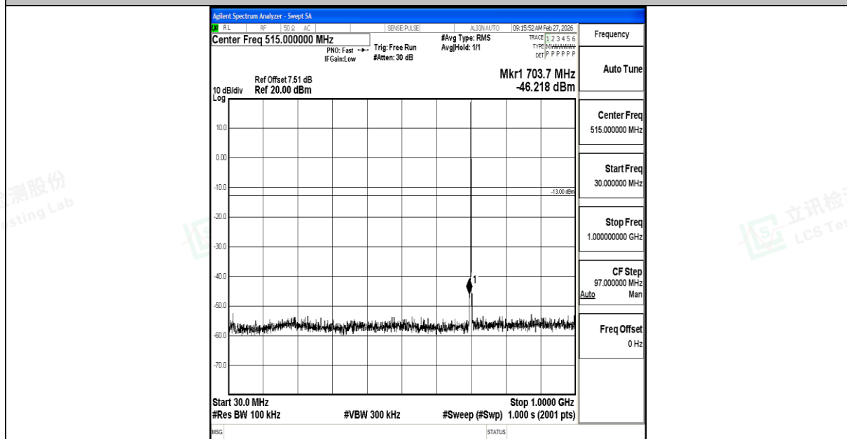
Band12_1.4MHz_16QAM_23095_1RB#0_30~1000_30~1000
