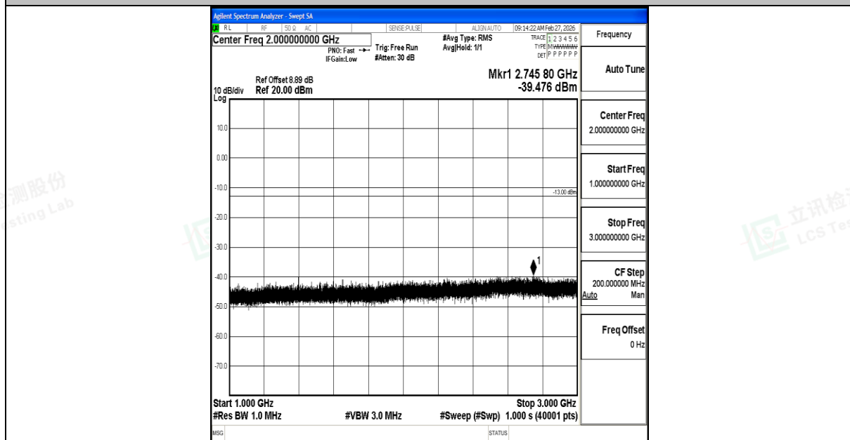
Band12_1.4MHz_QPSK_23017_1RB#0_1000~3000_1000~3000
