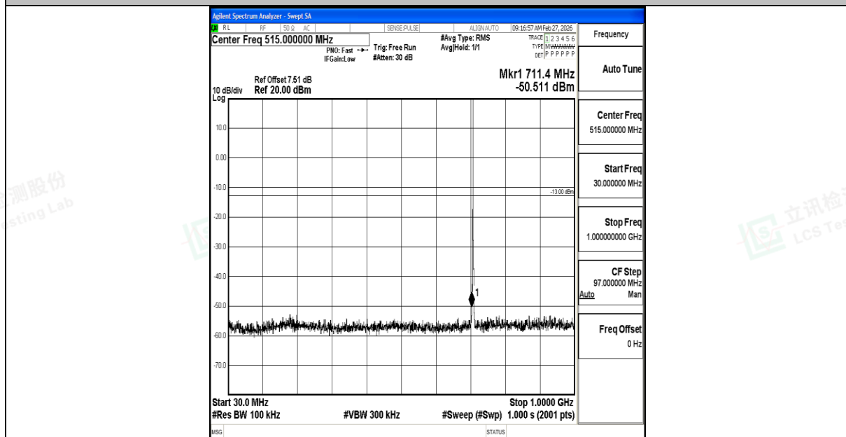
Band12_1.4MHz_16QAM_23173_1RB#0_30~1000_30~1000
