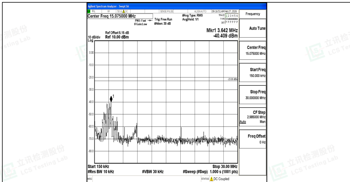
Band12_1.4MHz_16QAM_23173_1RB#0_0.15~30_0.15~30
