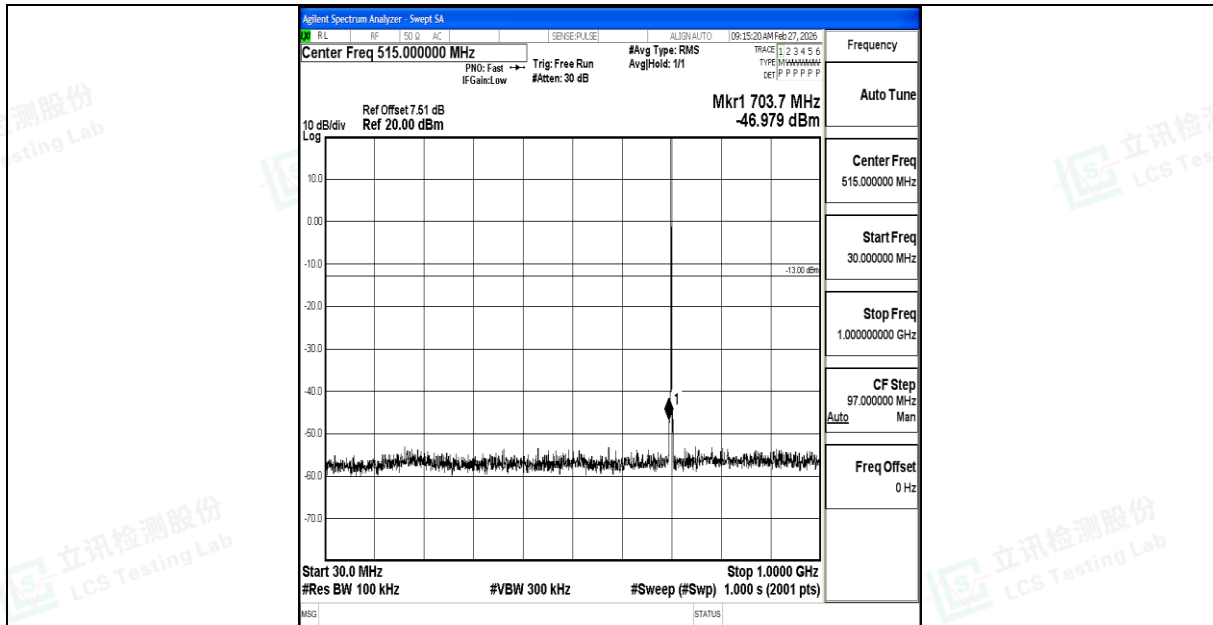
Band12_1.4MHz_QPSK_23095_1RB#0_30~1000_30~1000
