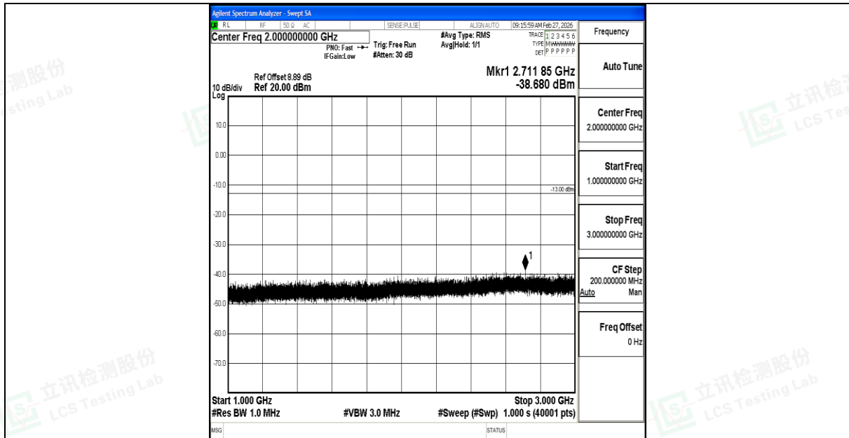
Band12_1.4MHz_16QAM_23095_1RB#0_1000~3000_1000~3000
