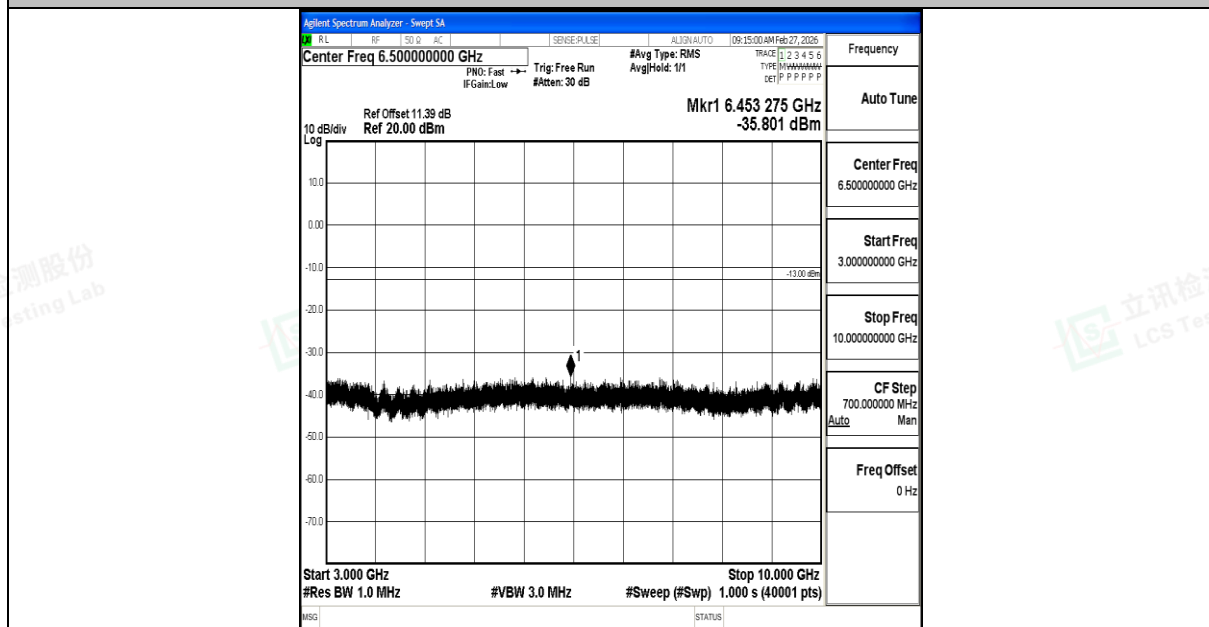
Band12_1.4MHz_16QAM_23017_1RB#0_3000~10000_3000~10000
