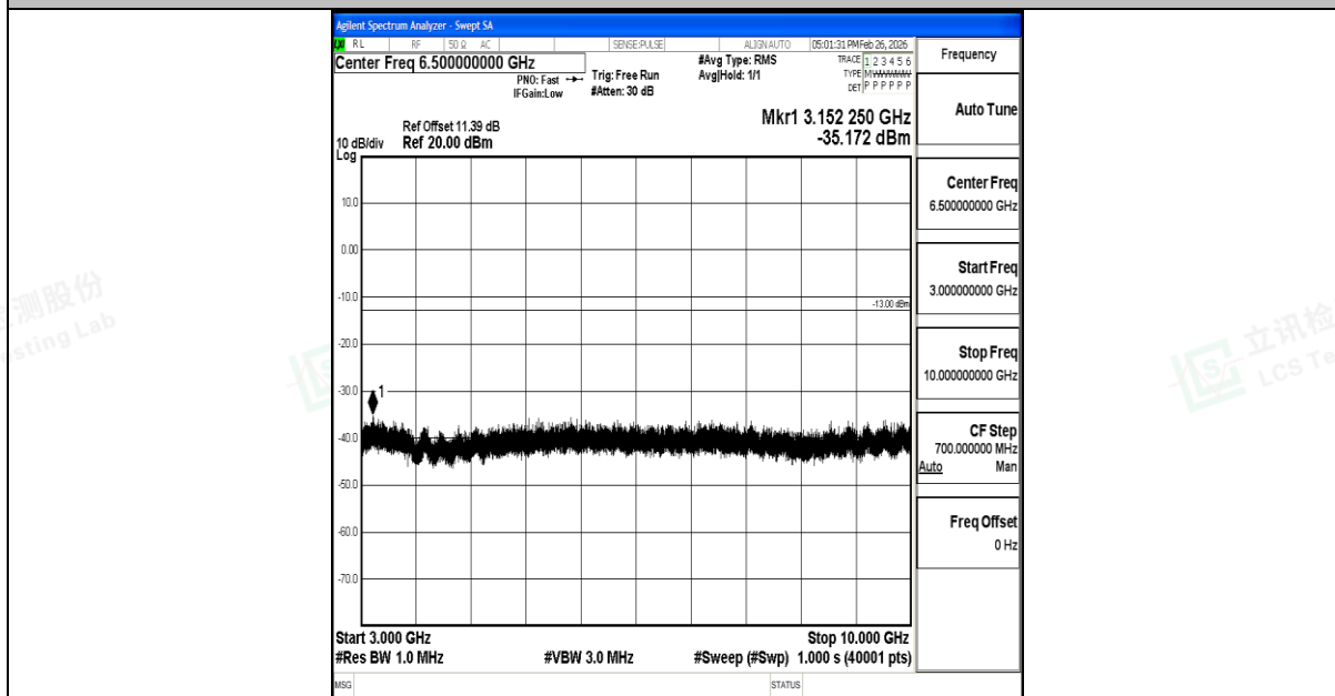
Band12_5MHz_QPSK_23035_1RB#0_3000~10000_3000~10000
