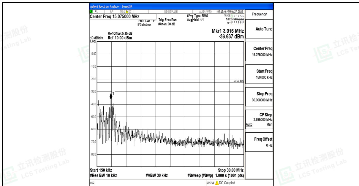
Band12_1.4MHz_16QAM_23095_1RB#0_0.15~30_0.15~30
