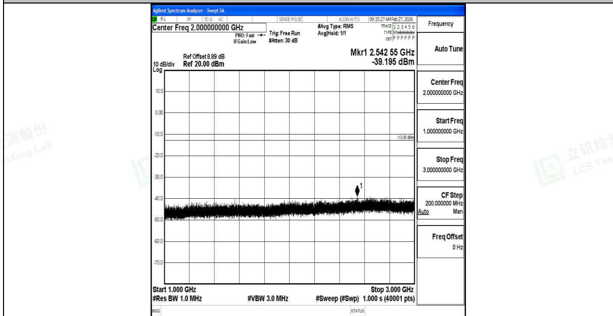
Band12_1.4MHz_QPSK_23095_1RB#0_1000~3000_1000~3000
