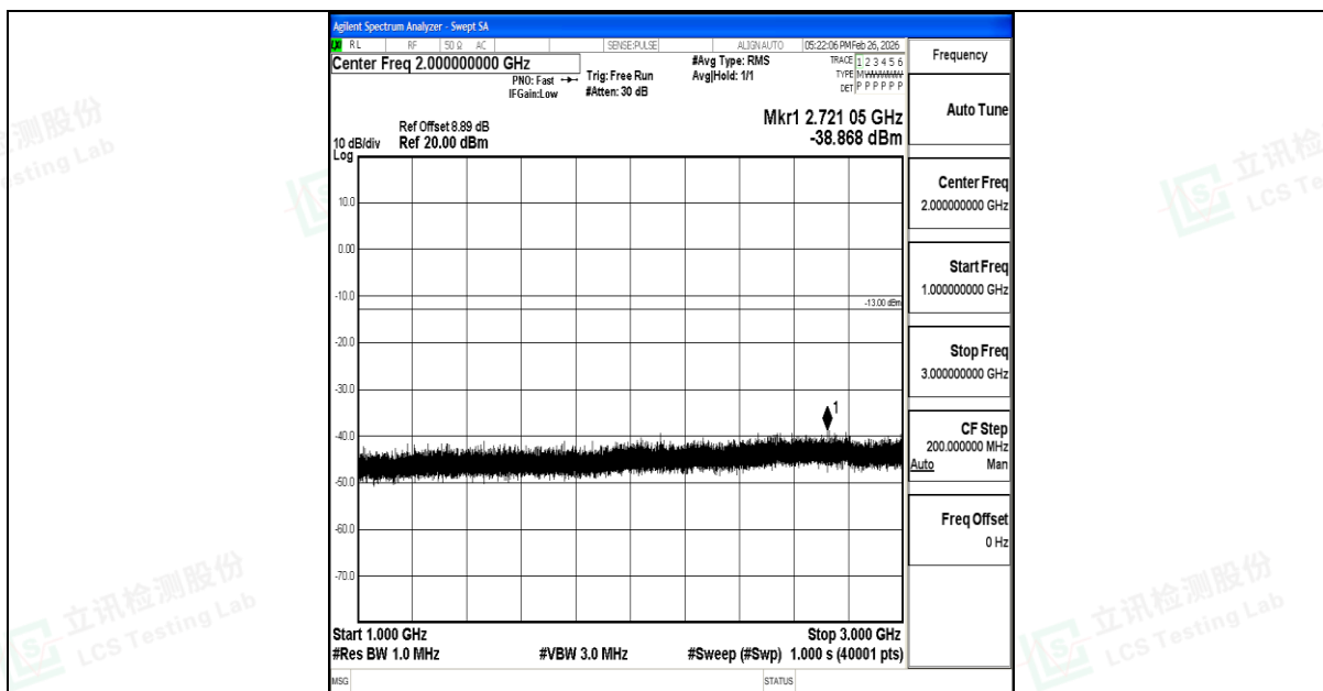
Band12_10MHz_16QAM_23095_1RB#0_1000~3000_1000~3000
