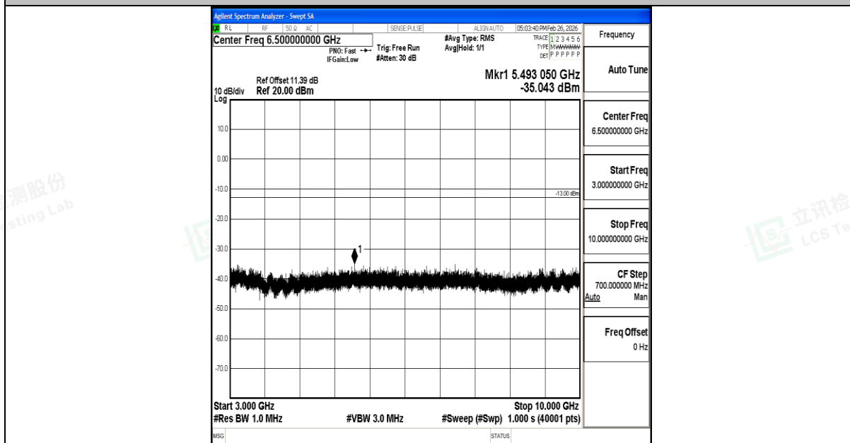
Band12_5MHz_QPSK_23155_1RB#0_3000~10000_3000~10000
