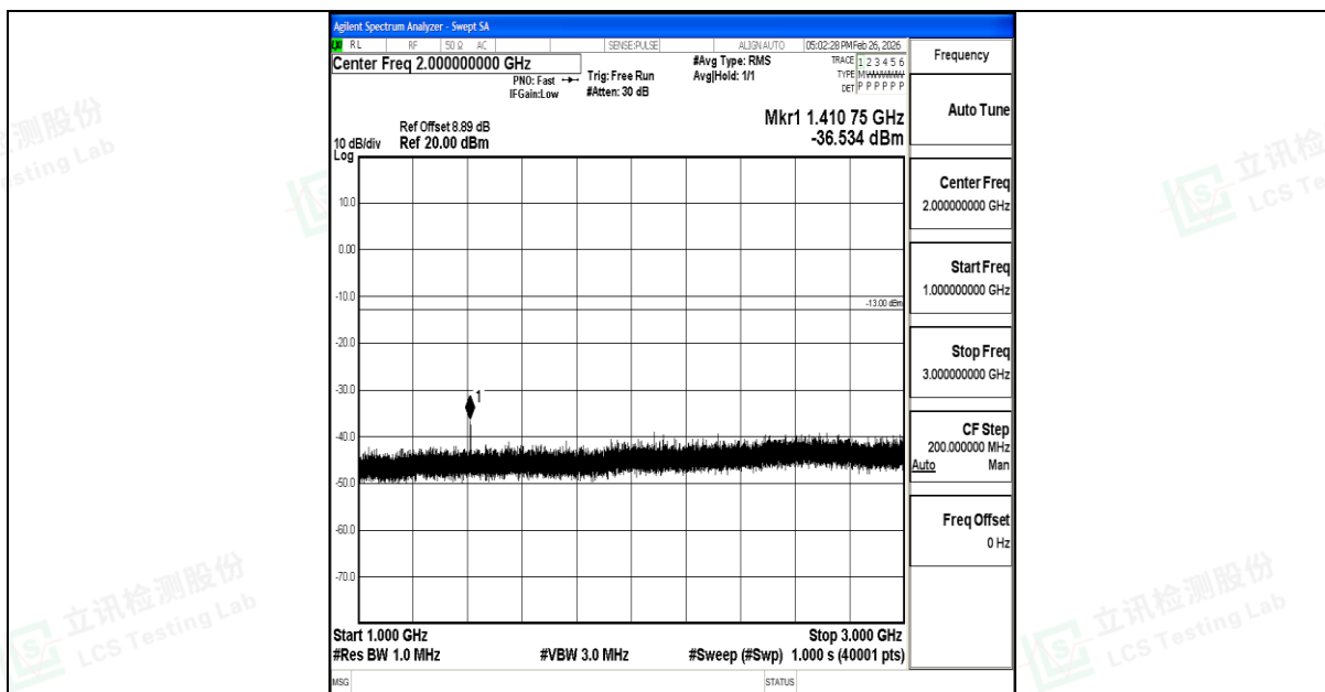
Band12_5MHz_QPSK_23095_1RB#0_1000~3000_1000~3000
