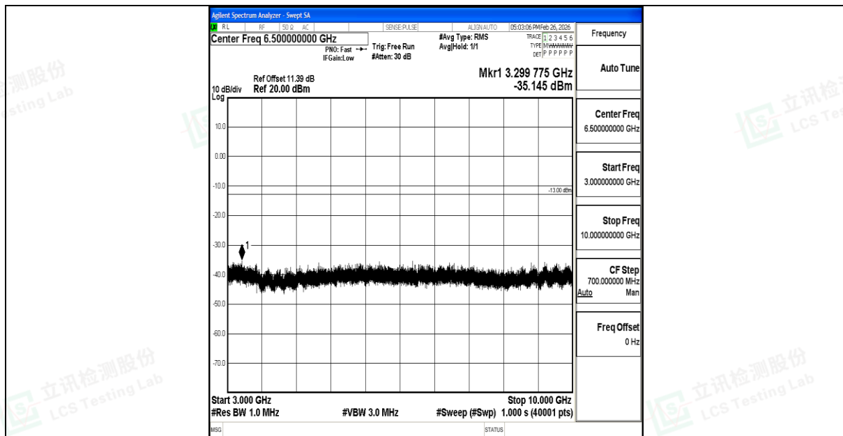
Band12_5MHz_16QAM_23095_1RB#0_3000~10000_3000~10000
