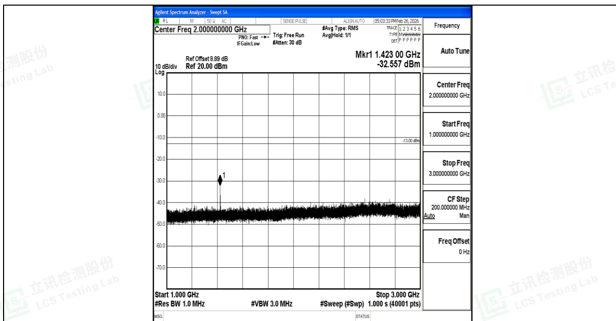
Band12_5MHz_QPSK_23155_1RB#0_1000~3000_1000~3000
