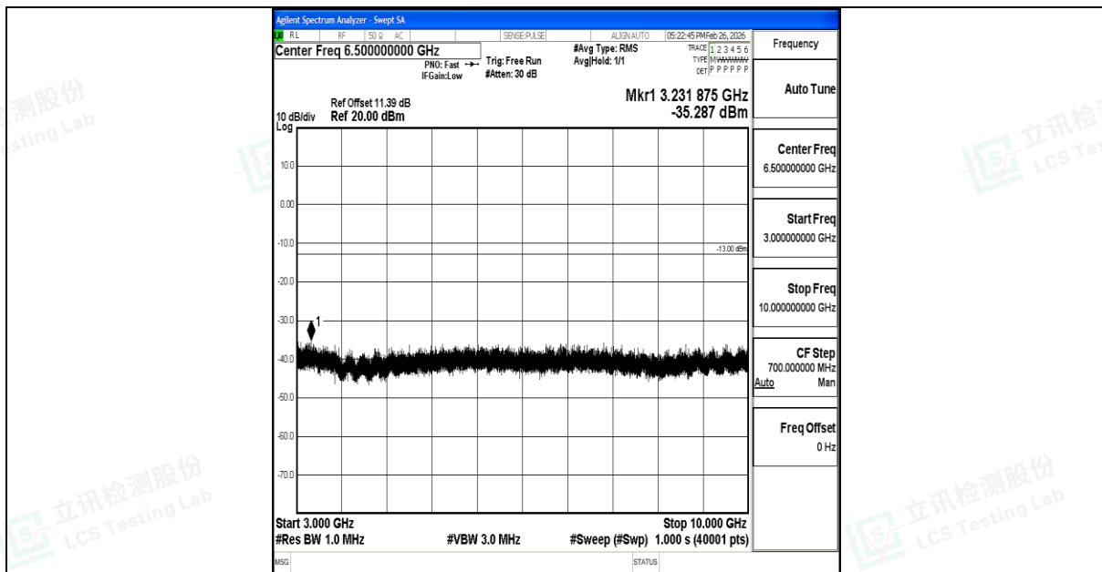
Band12_10MHz_QPSK_23130_1RB#0_3000~10000_3000~10000
