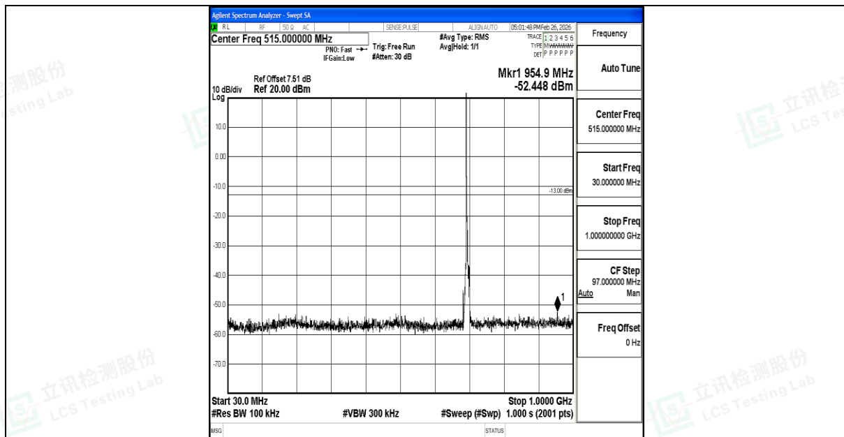
Band12_5MHz_16QAM_23035_1RB#0_30~1000_30~1000
