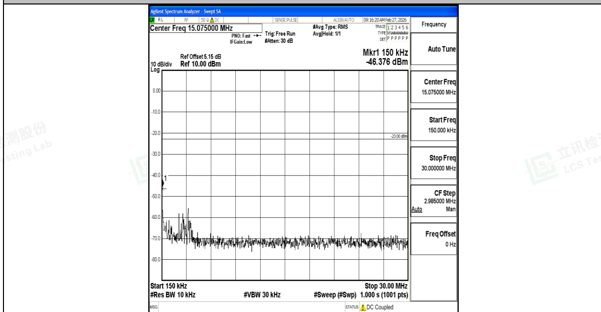
Band12_1.4MHz_QPSK_23173_1RB#0_0.15~30_0.15~30
