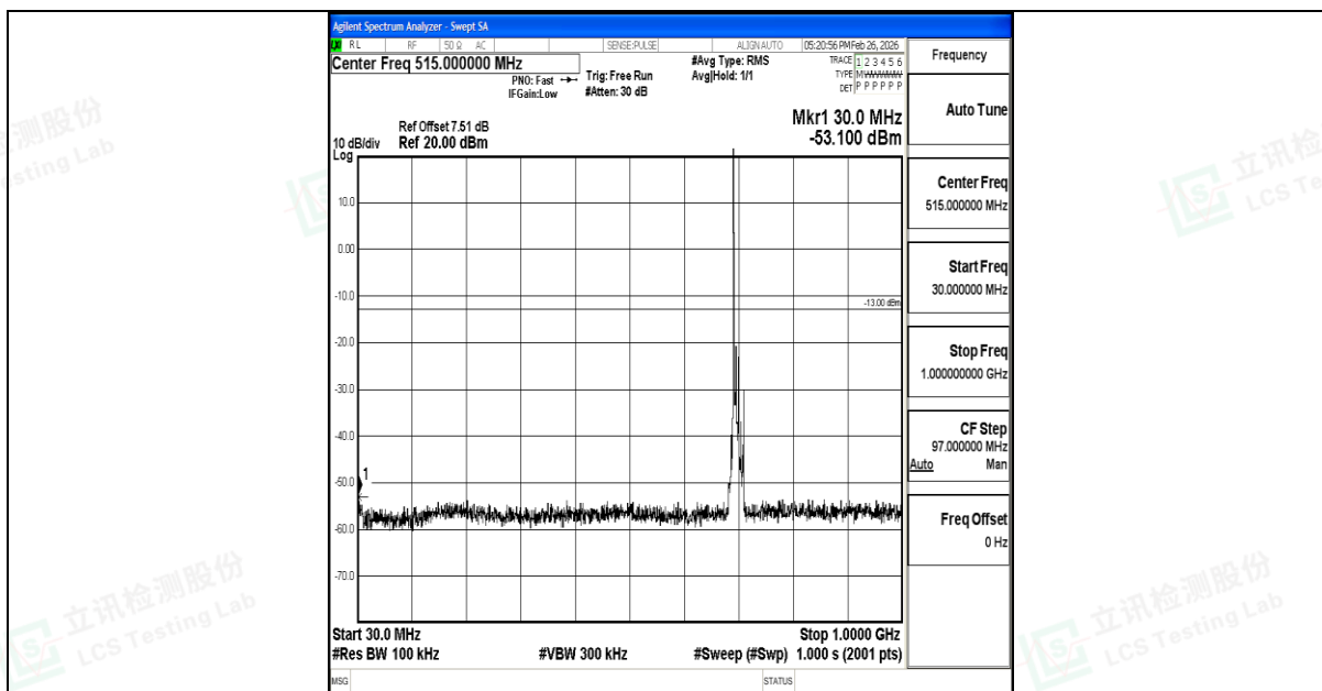
Band12_10MHz_16QAM_23060_1RB#0_30~1000_30~1000
