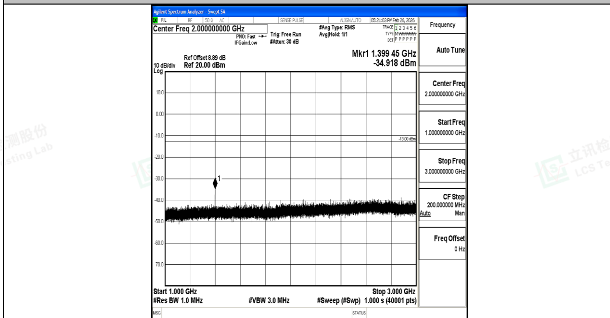
Band12_10MHz_16QAM_23060_1RB#0_1000~3000_1000~3000
