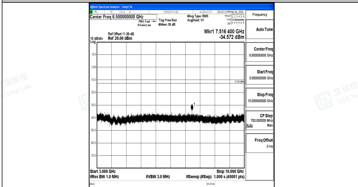
Band12_10MHz_16QAM_23095_1RB#0_3000~10000_3000~10000
