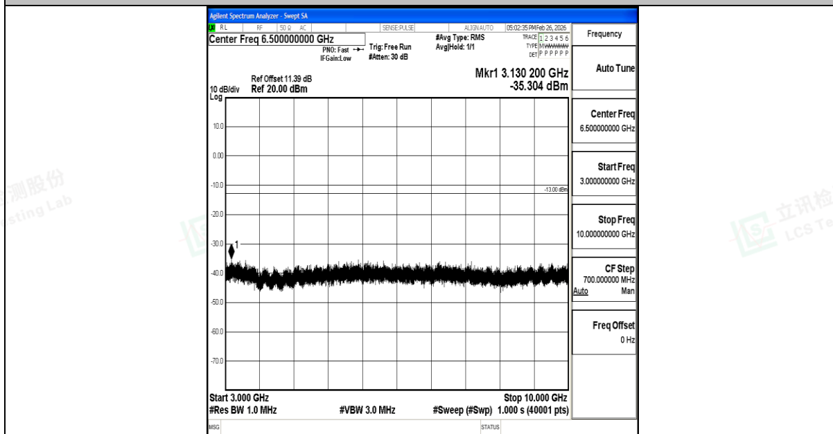
Band12_5MHz_QPSK_23095_1RB#0_3000~10000_3000~10000
