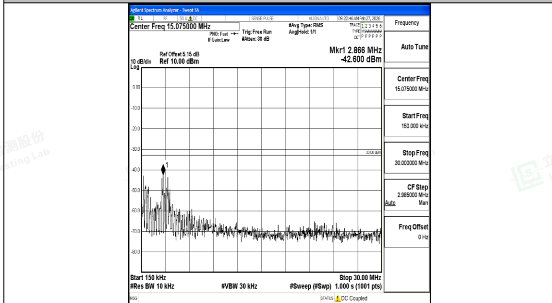
Band66_3MHz_16QAM_131987_1RB#0_0.15~30_0.15~30
