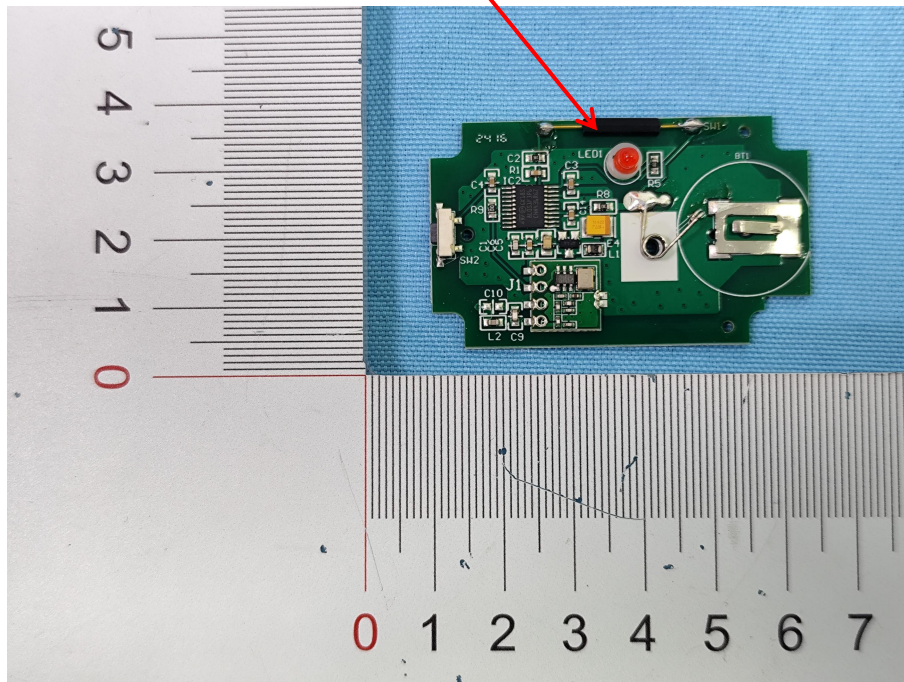
ANT(DOOR SENSOR)
