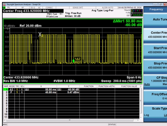
T period
