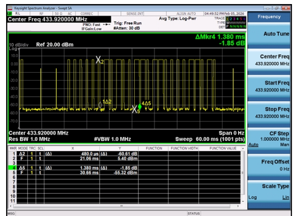
T on
