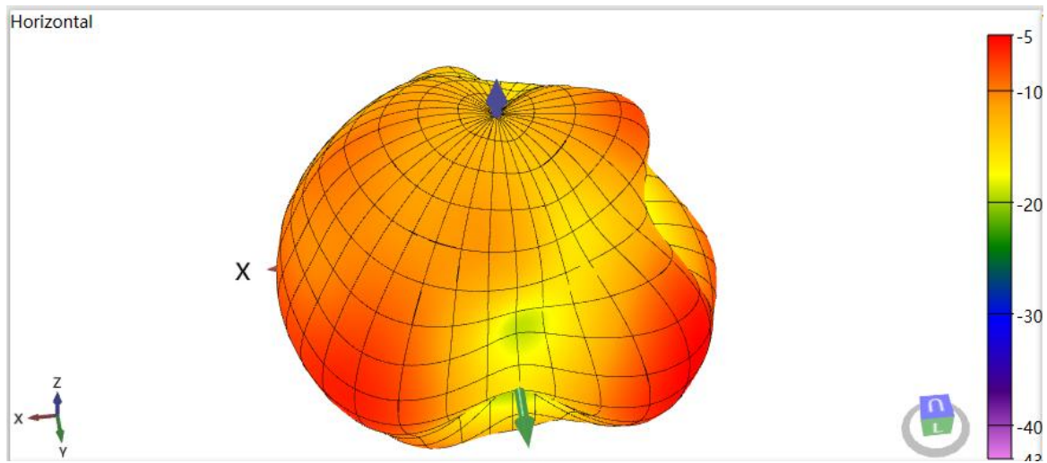
Antenna 2400MHz 3D
