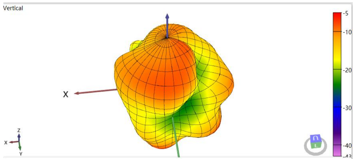
Antenna 2440MHz 3D
