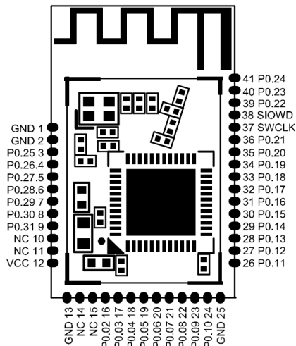
PCB Antenna
