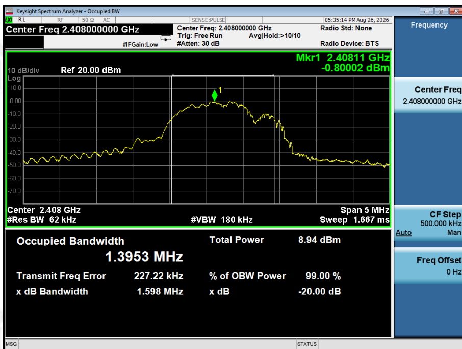
-20dB Bandwidth-GFSK 2408MHz
