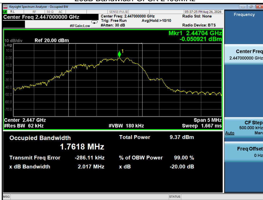
-20dB Bandwidth-GFSK 2447MHz
