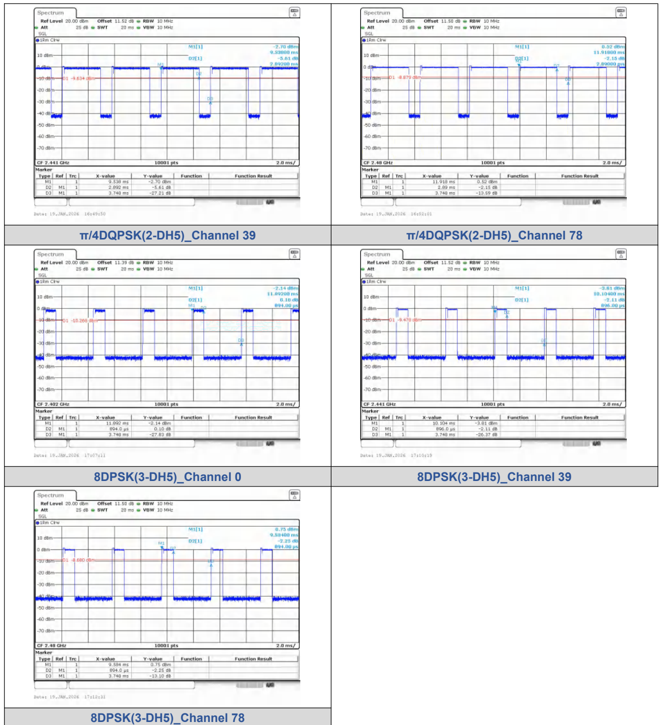
8DPSK(3-DH5)_Channel 78
