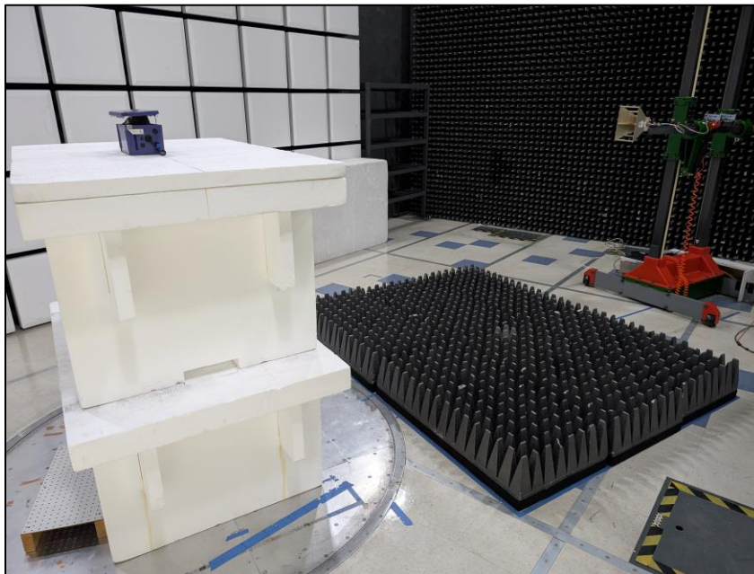
1-18 GHz Setup
