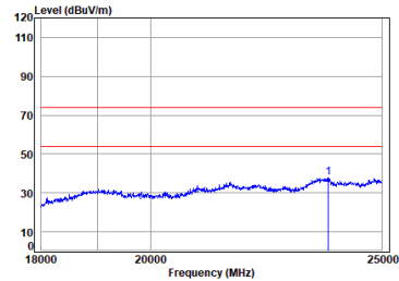
BLE_1M_TX_CH_39_Vertical
