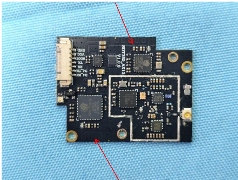
BT&WiFi(ESP32-PICO-D4)-ANT
