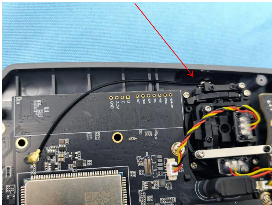
WiFi(XY8788WA)-ANT
