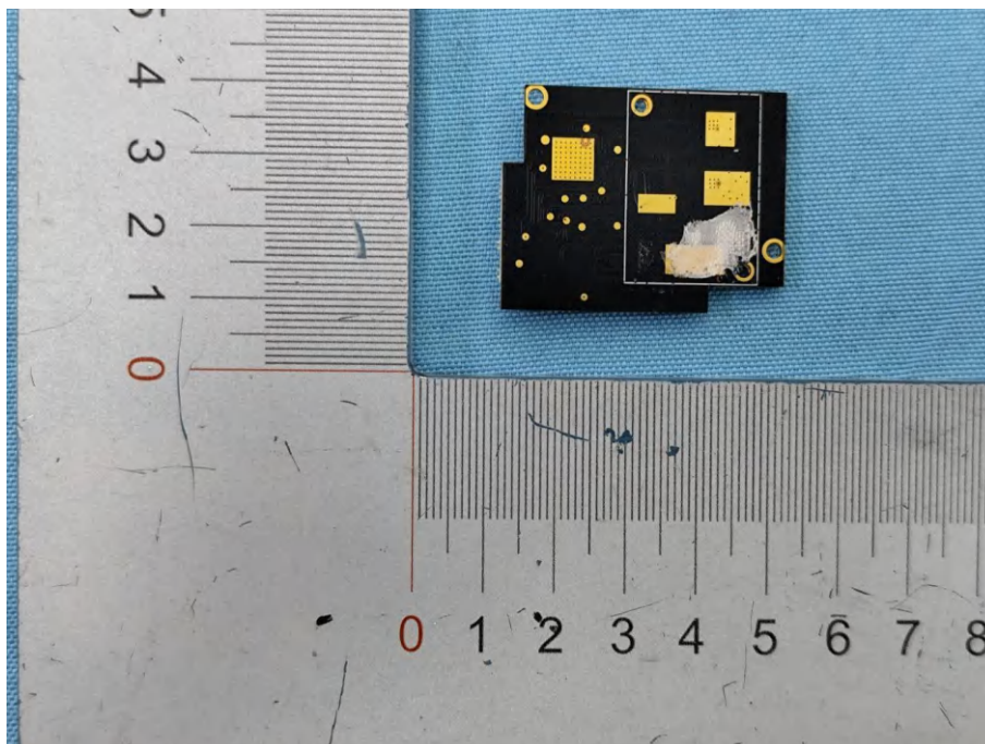
BT&WiFi(ESP32-PICO-D4)-ANT
