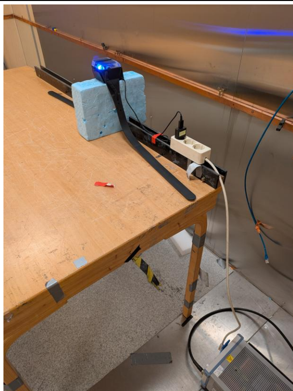
Power-Line Conducted Emissions
