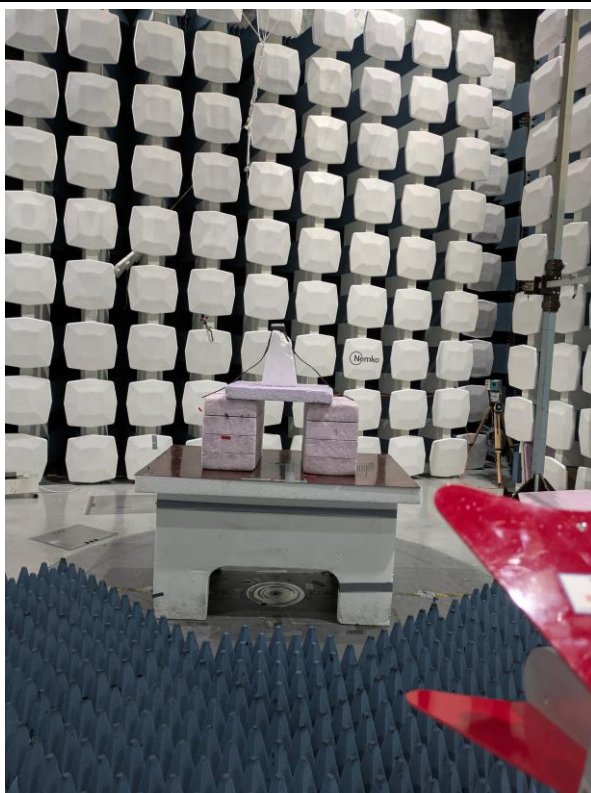
Radiated Emissions 1 – 18 GHz
