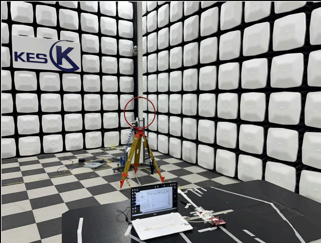
Radiated test
