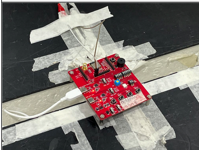
Radiated test close-up
