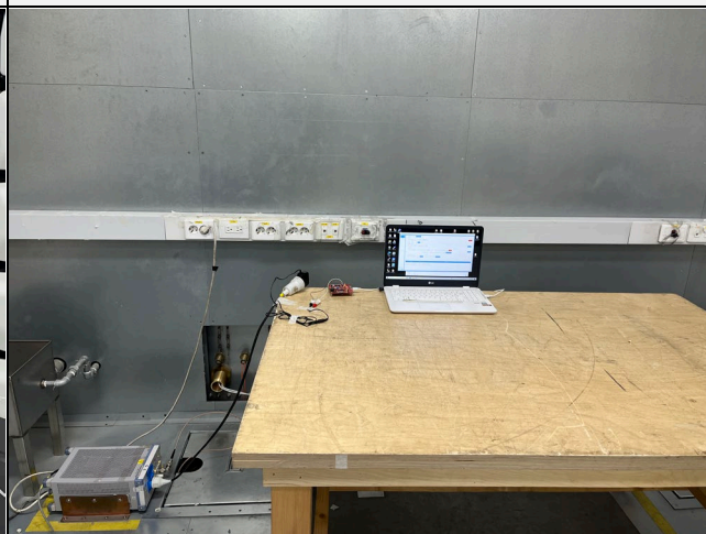
AC conducted test
