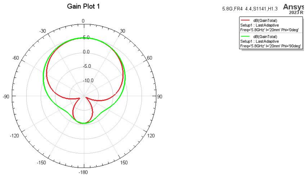
Realized Gain Plot 1
