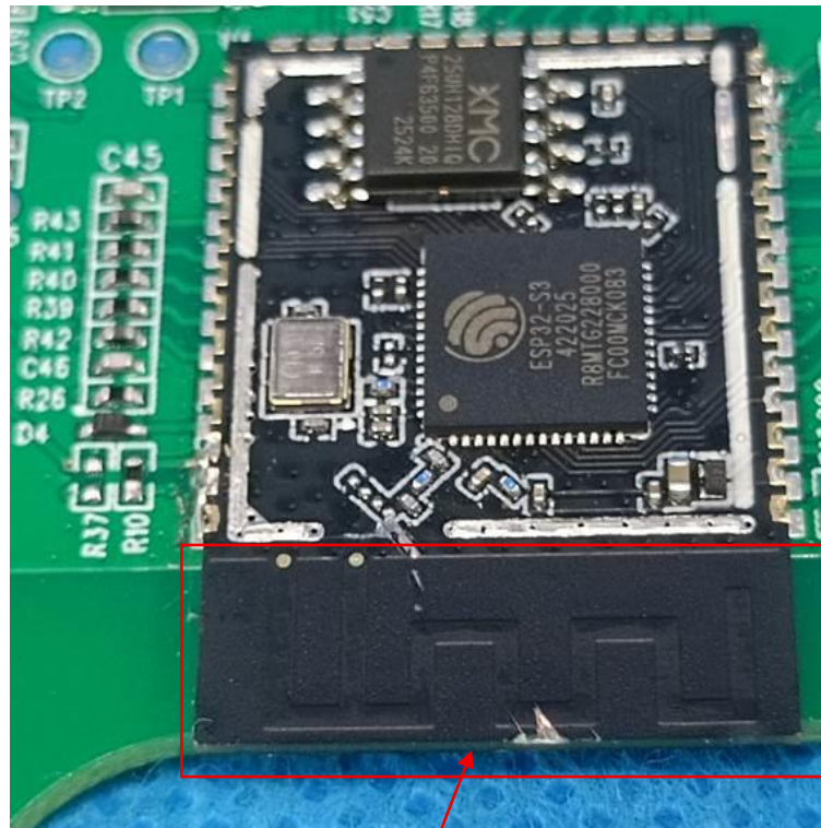
RF antenna
