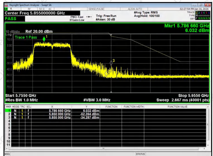
(802.11ax20) Band Edge, Right Side
