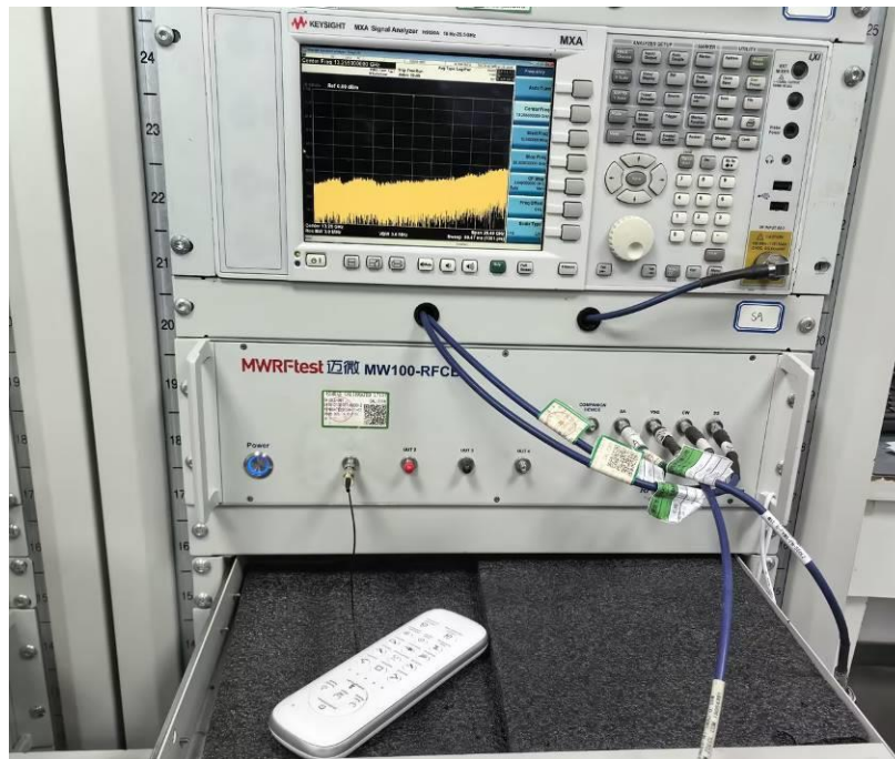
RF conducted test Photos
