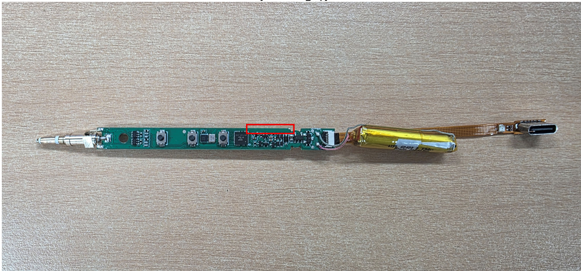
[Main board_Top]
