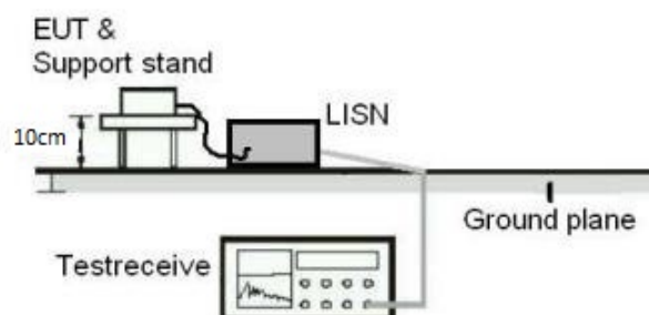
Diagram of Measurement Configuration for Mains Conduction Measurement
