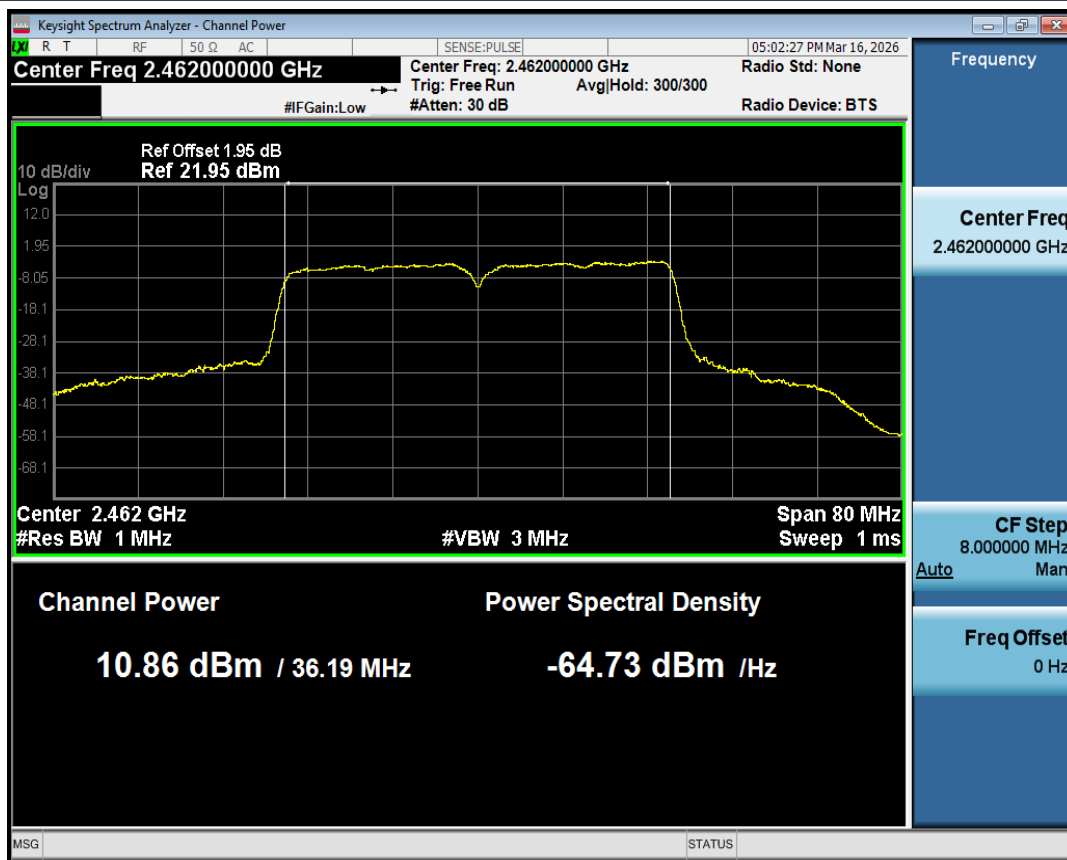
Average Power NVNT n40 2462MHz Ant1
