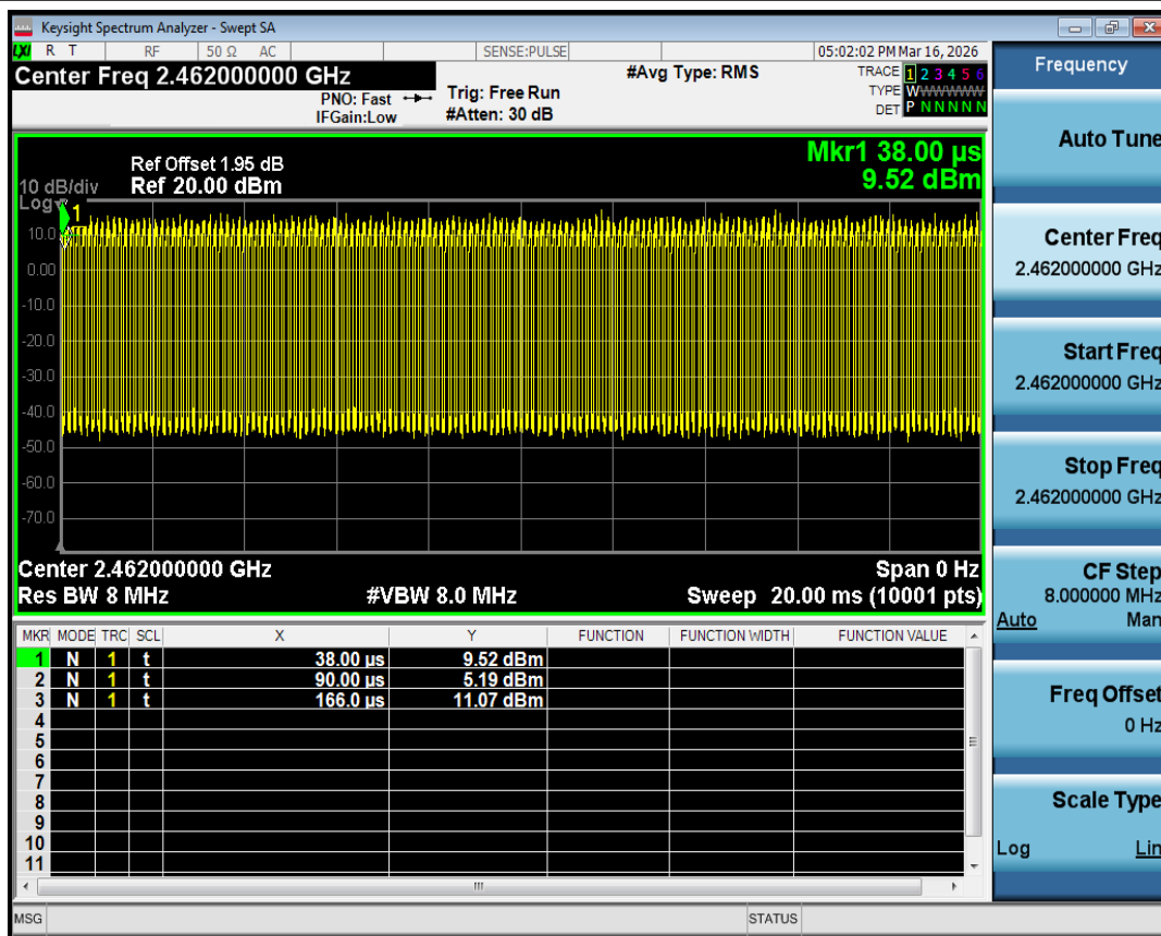
Duty Cycle NVNT n40 2462MHz Ant1
