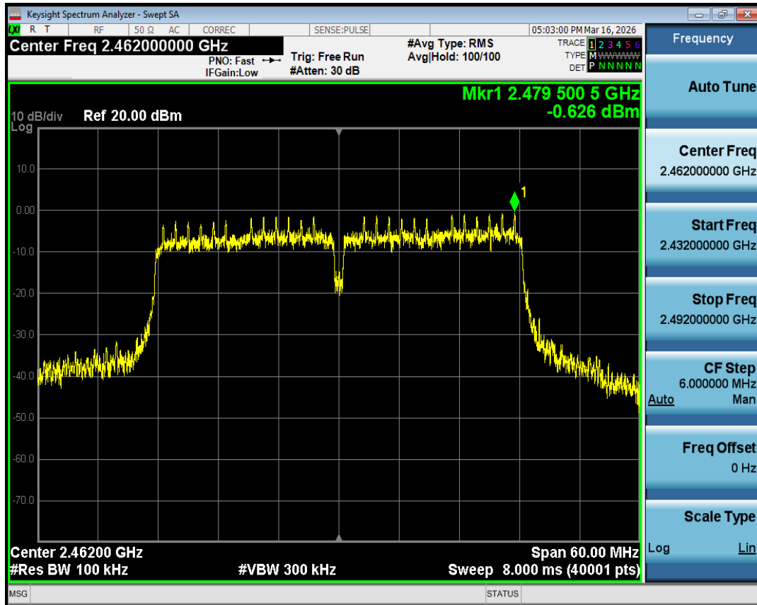
Tx. Spurious NVNT n40 2462MHz Ant1 Ref
