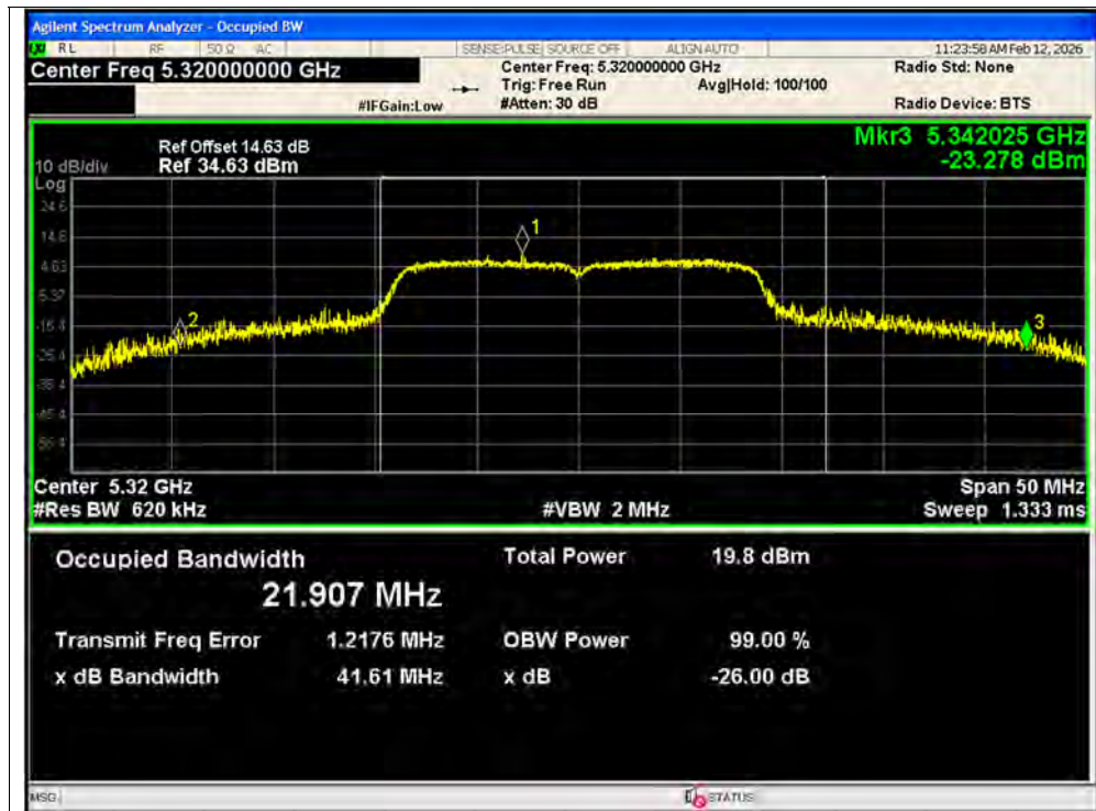
-26dB Bandwidth NVNT n20 5320MHz Ant1
